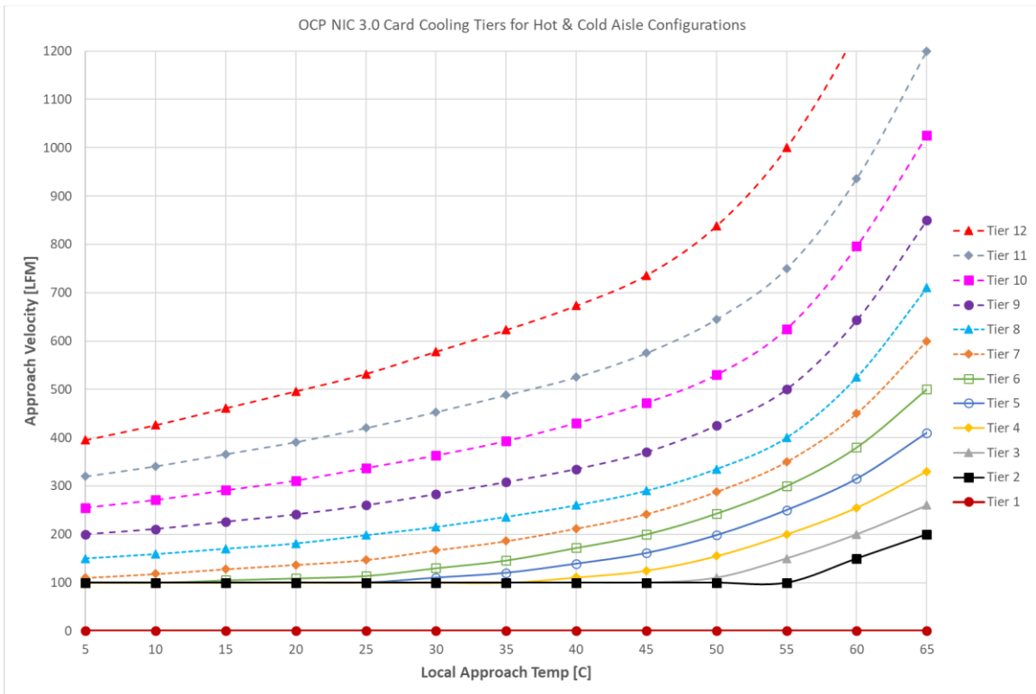
Figure 143: Graphical View of Card Cooling Tiers
