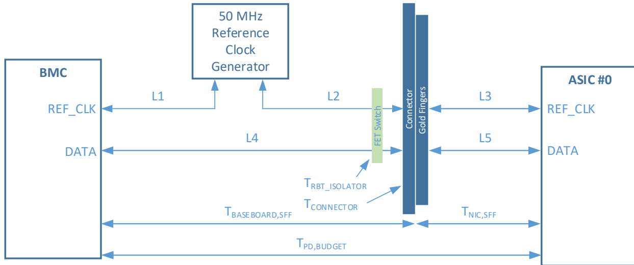
Figure 113: NC-SI over RBT Timing Budget Topology
