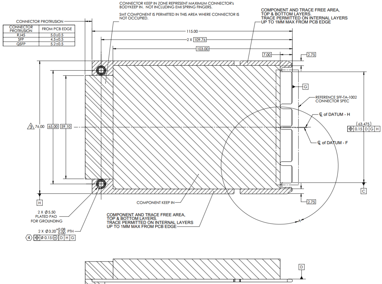
Figure 24: SFF Keep Out Zone – Top View
