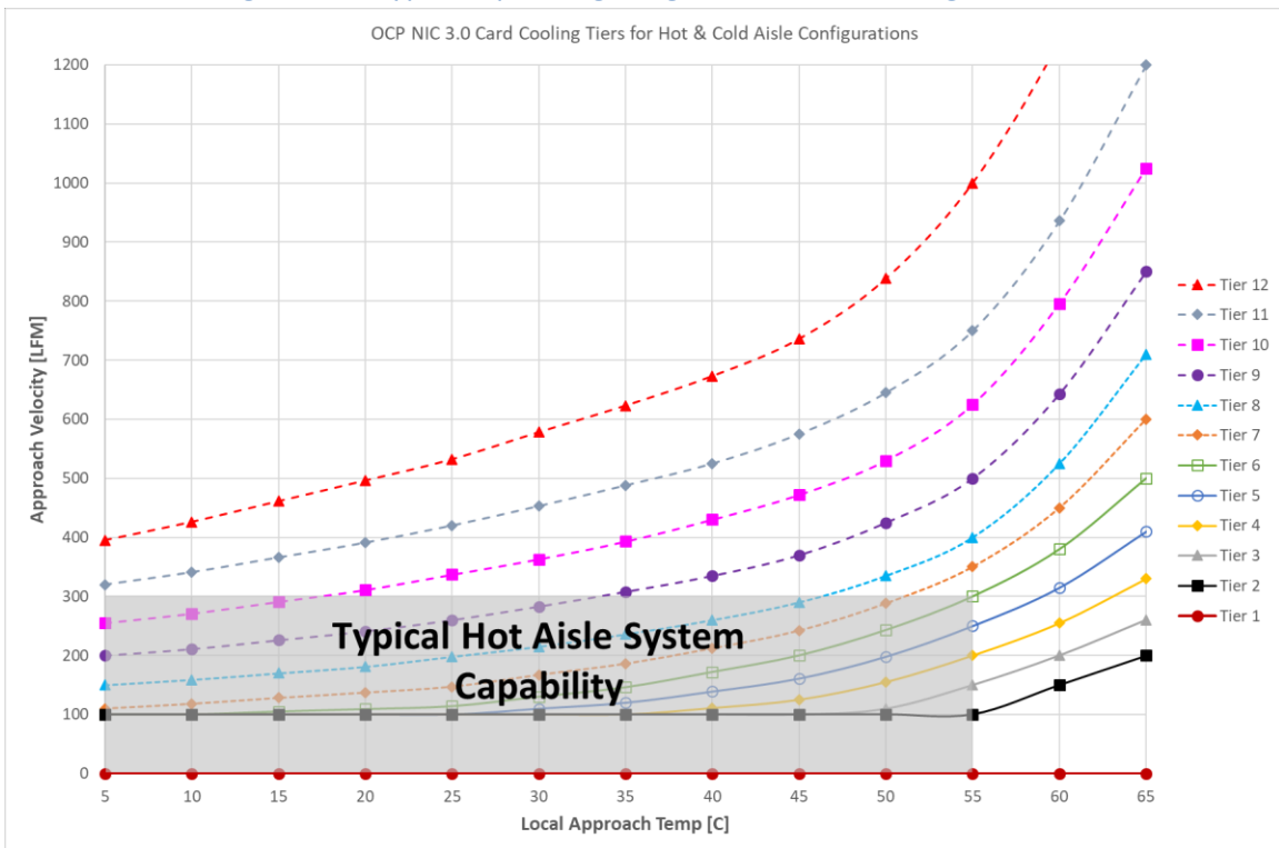
Figure 144: Typical Operating Range for Hot Aisle Configurations
