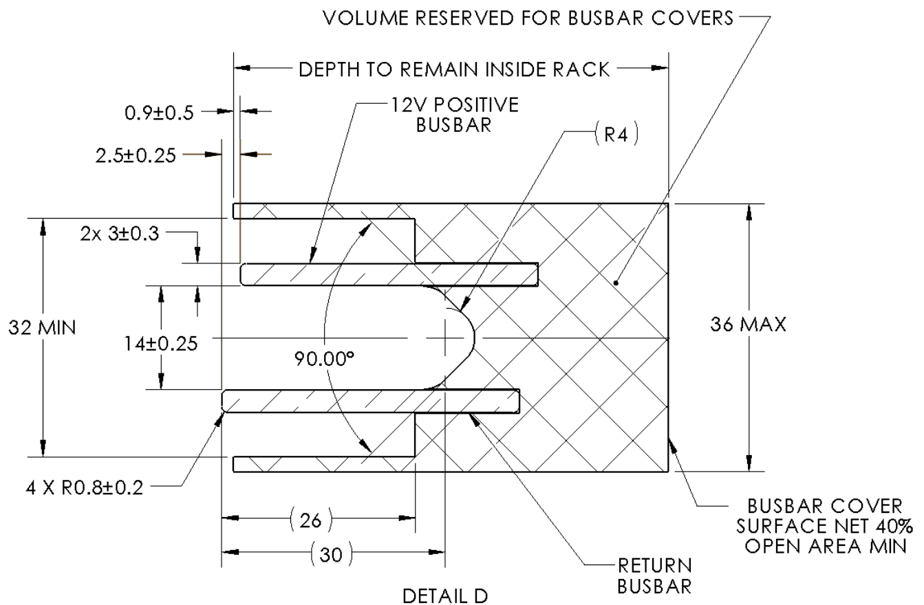
Figure 8: Bus bar Detail
