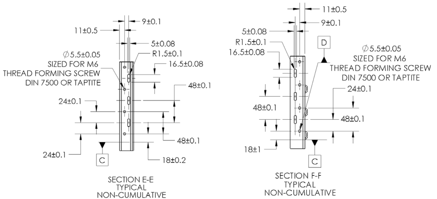
Figure 4. Front and rear Vertical Post Detail
