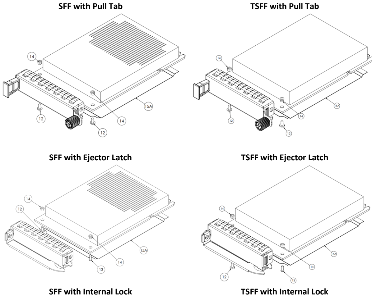
Figure 14: PBA Exploded Views (SFF, TSFF and LFF)
