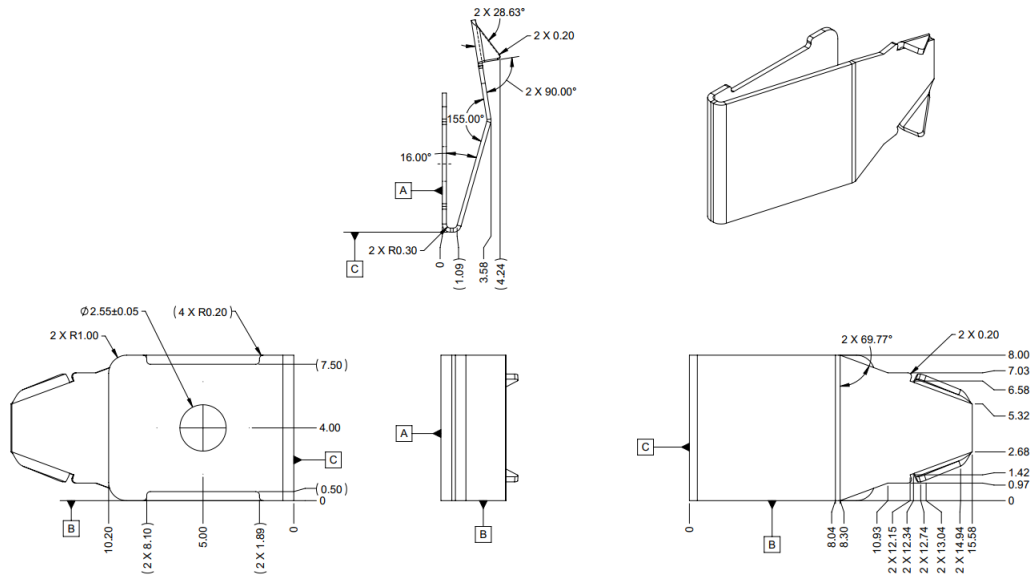
Figure 25: Ejector Lock
