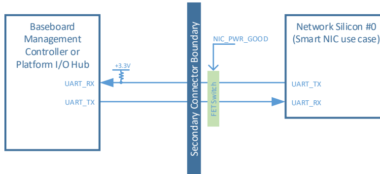
Figure 102: UART Connection Example
