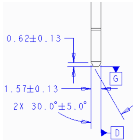
Figure 77: SFF, TSFF Primary Connector Card Profile Dimensions
