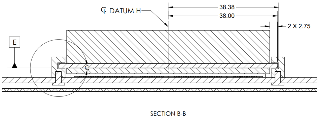
Figure 57: SFF Baseboard Chassis CTF Dimensions (Rear Rail Guide View)
