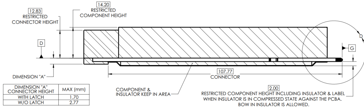
Figure 33: TSFF Keep Out Zone – Side View
