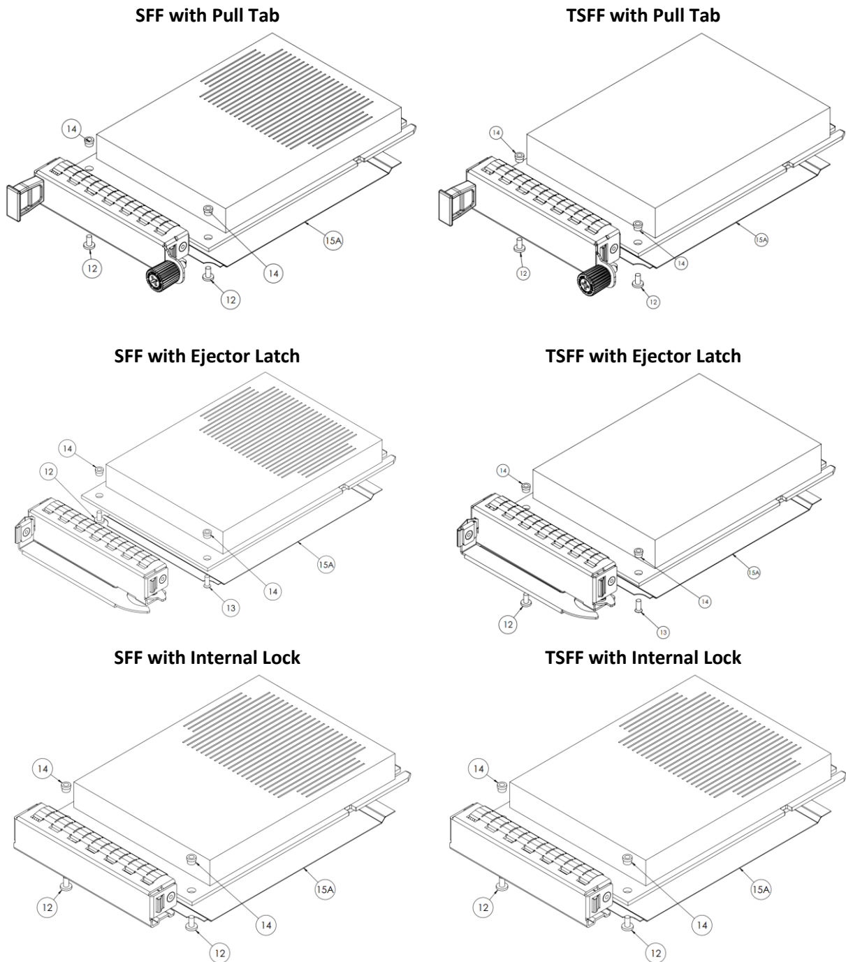
Figure 14: PBA Exploded Views (SFF, TSFF and LFF)
