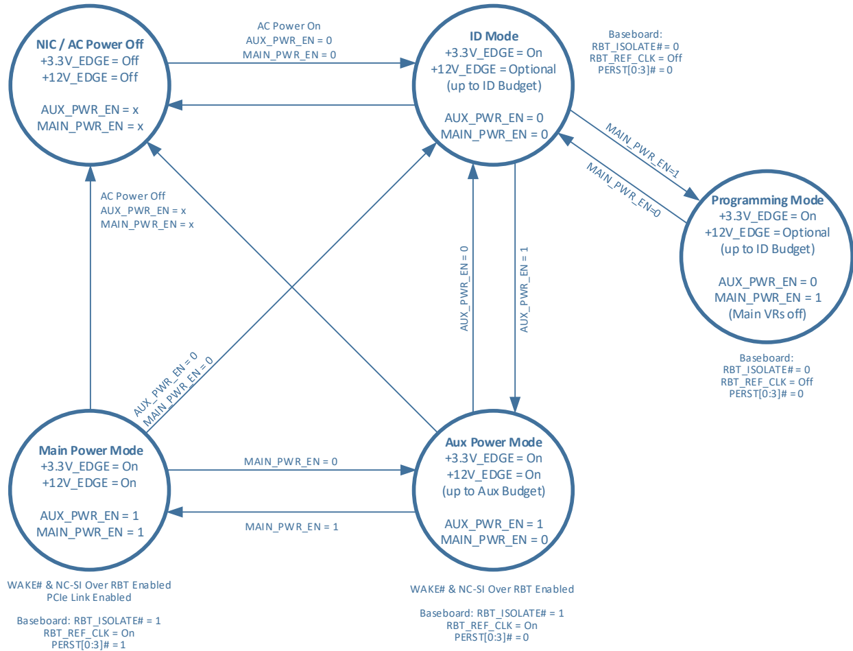
Figure 115: Baseboard Power States
