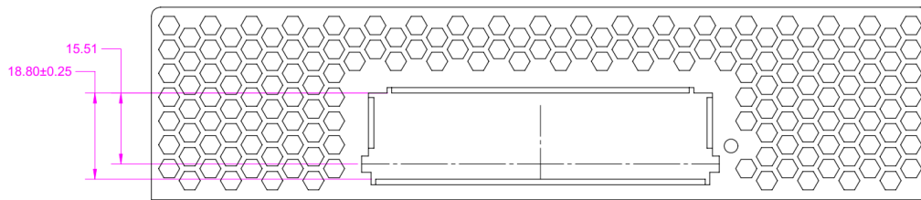
Figure 62: TSFF Baseboard Chassis CTF Dimensions (Rear View)
