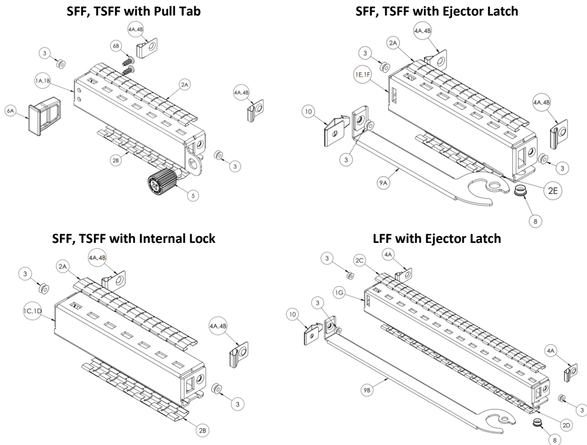
Figure 15: Faceplate Assembly Exploded Views (SFF, TSFF and LFF)
