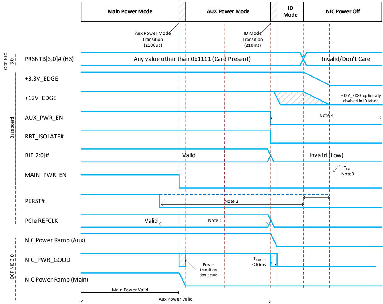
Figure 117: Power-Down Sequencing – Normal Operation
