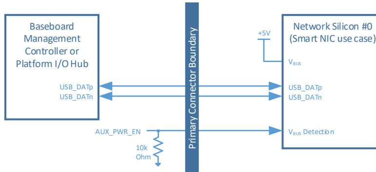
Figure 100: USB 2.0 Connection Example – Basic Connectivity
