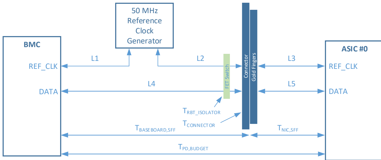
Figure 122: NC-SI over RBT Timing Budget Topology
