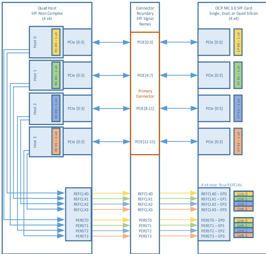
Figure 110: SFF/TSFF PCIe REFCLK Mapping – Quad Host – 4 Links
