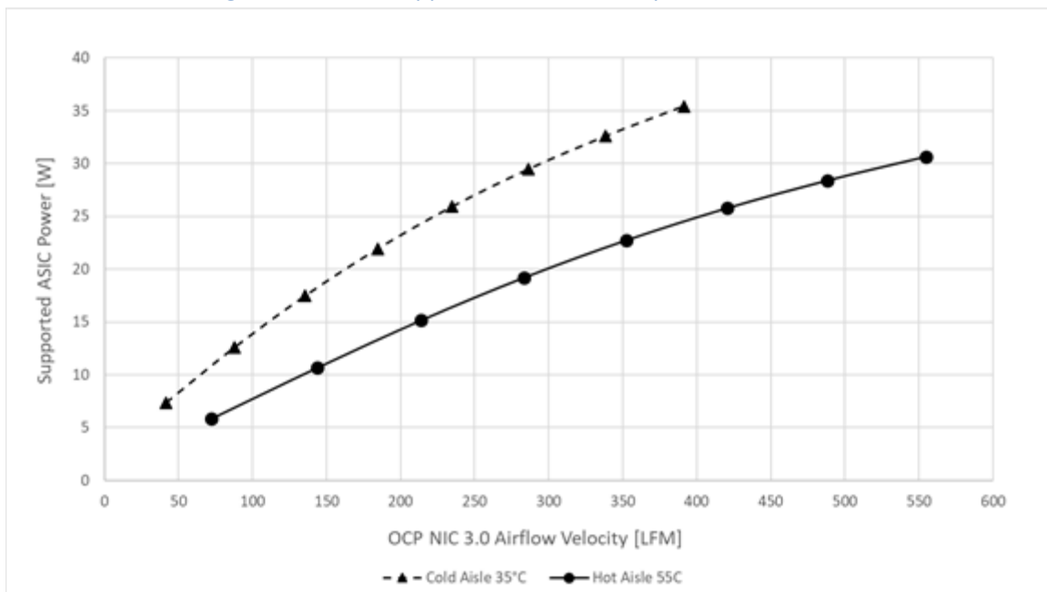
Figure 138: ASIC Supportable Power Comparison – SFF Card
