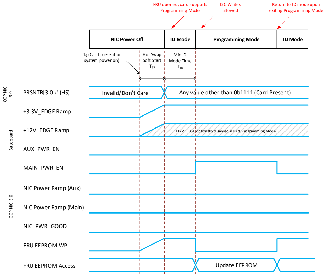
Figure 118: Programming Mode Sequencing
