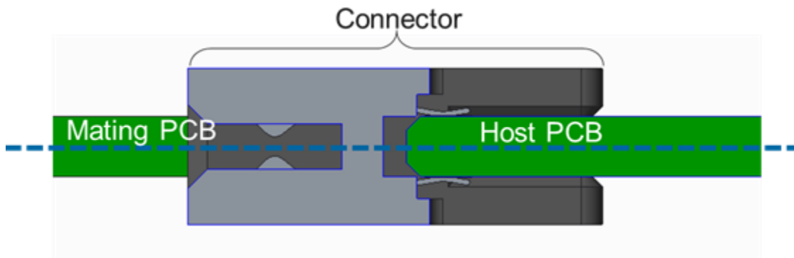
Figure 87: 0 mm Offset (Coplanar) for 0.062" Thick Baseboards
