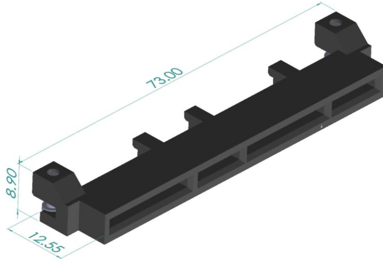
Figure 84: 168-pin Base Board Primary Connector – Straddle Mount
