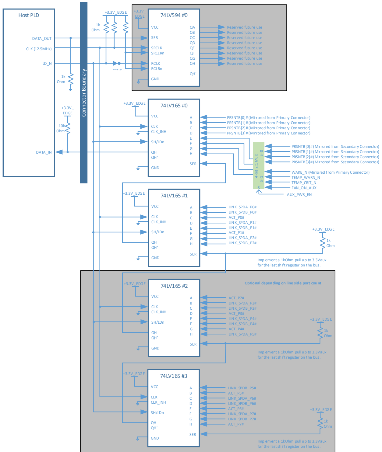
Figure 98: Scan Chain Connection Example
