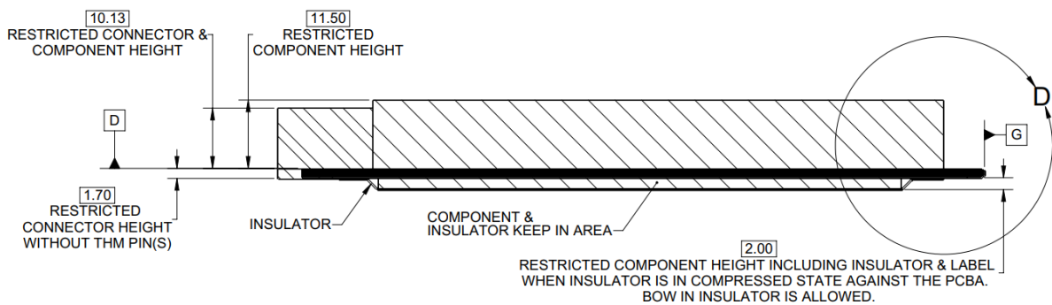
Figure 37: LFF Keep Out Zone – Side View
