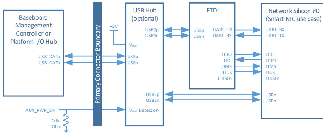
Figure 101: USB 2.0 Connection Example – USB-Serial / USB-JTAG Connectivity
