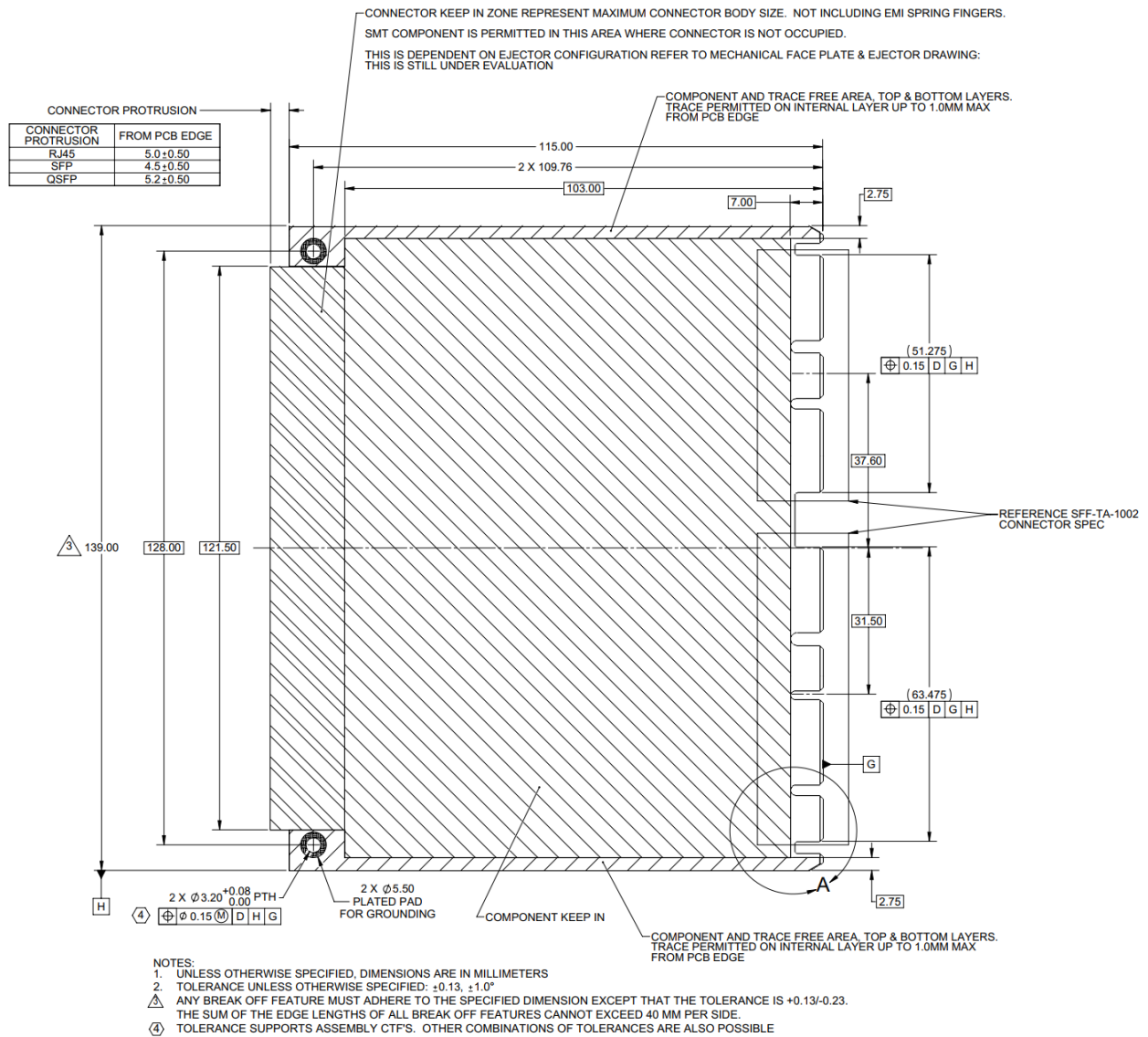
Figure 34: LFF Keep Out Zone – Top View
