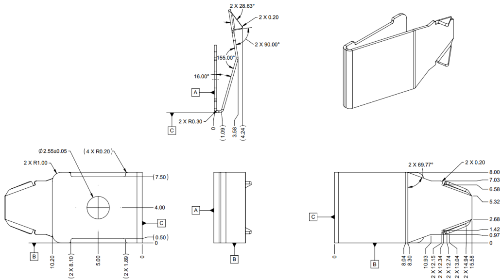
Figure 25: Ejector Lock
