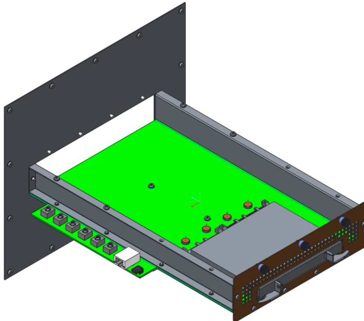
Figure 146: LFF Card Thermal Test Fixture Design – Cover Removed
