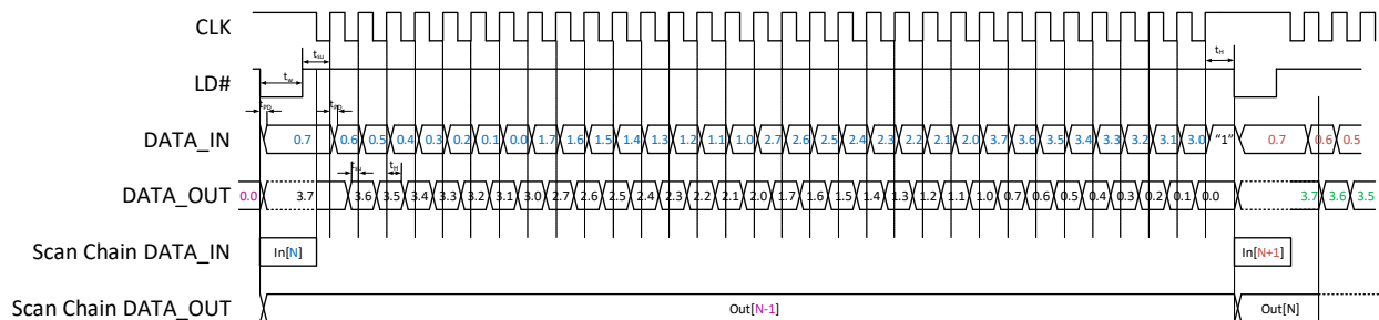
Figure 97: Scan Chain Timing Diagram Example 2
