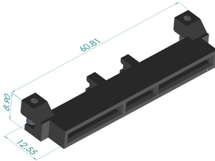
Figure 85: 140-pin Base Board Secondary Connector – Straddle Mount
