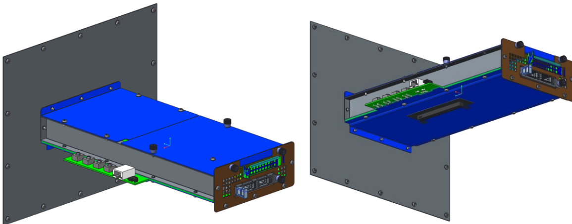
Figure 142: SFF Thermal Test Fixture Preliminary Design
