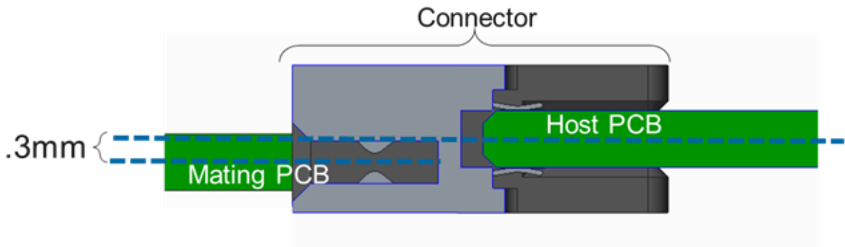
Figure 88: 0.3 mm Offset for 0.076" Thick Baseboards
