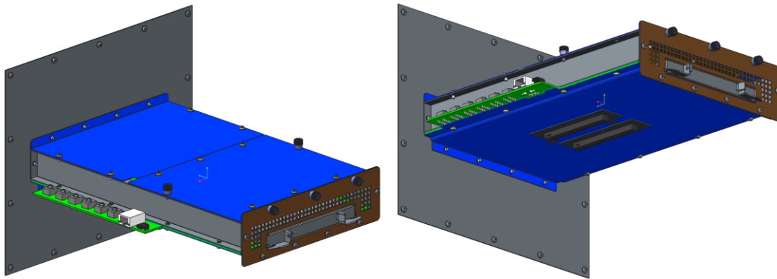
Figure 145: LFF Card Thermal Test Fixture Design
