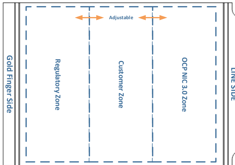
Figure 70: SFF, TSFF Label Area Example
