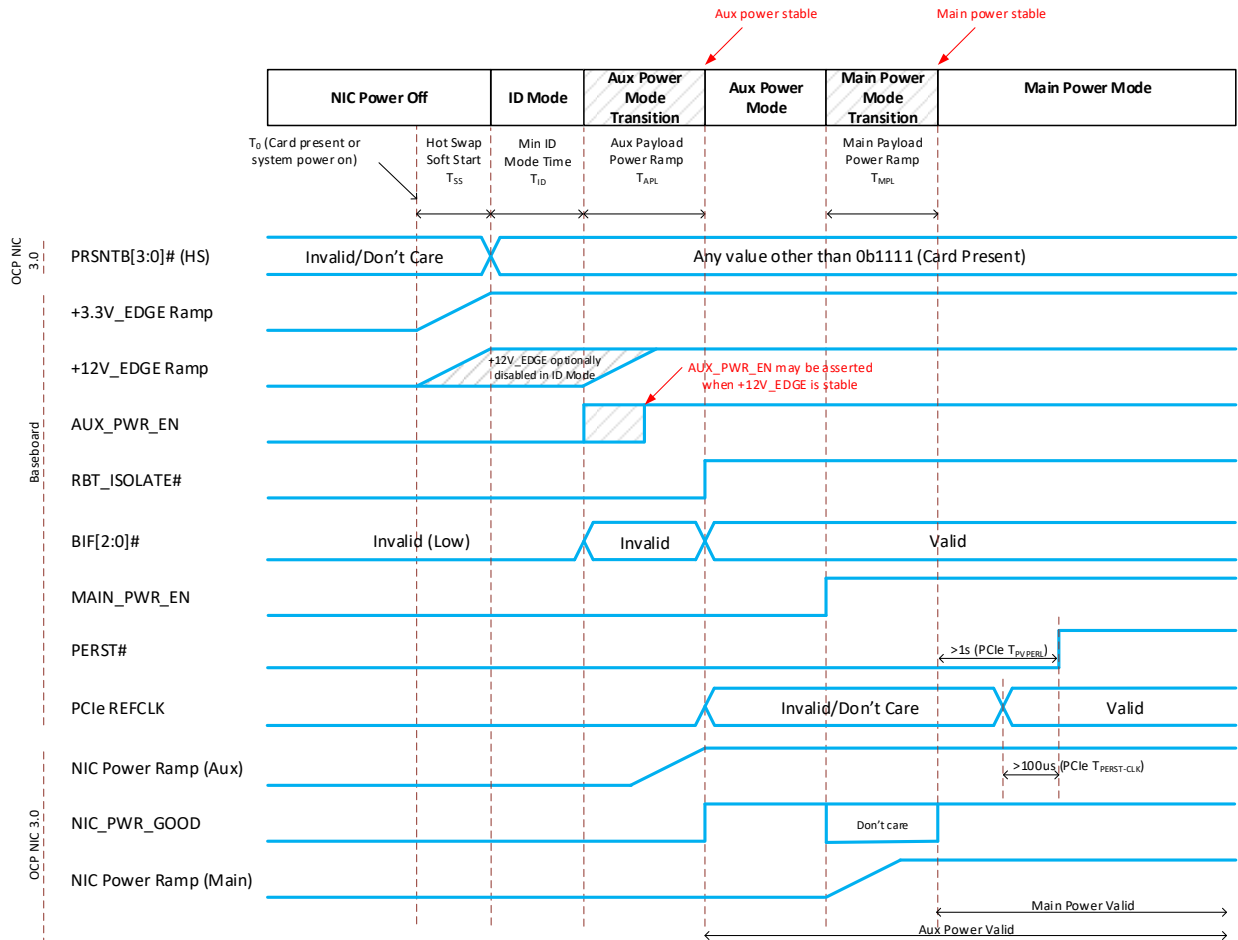
Figure 116: Power-Up Sequencing – Normal Operation
