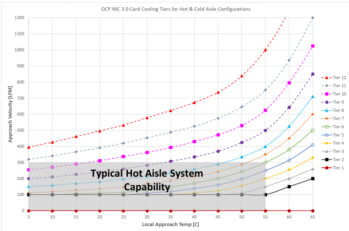
Figure 154: Typical Operating Range for Hot Aisle Configurations
