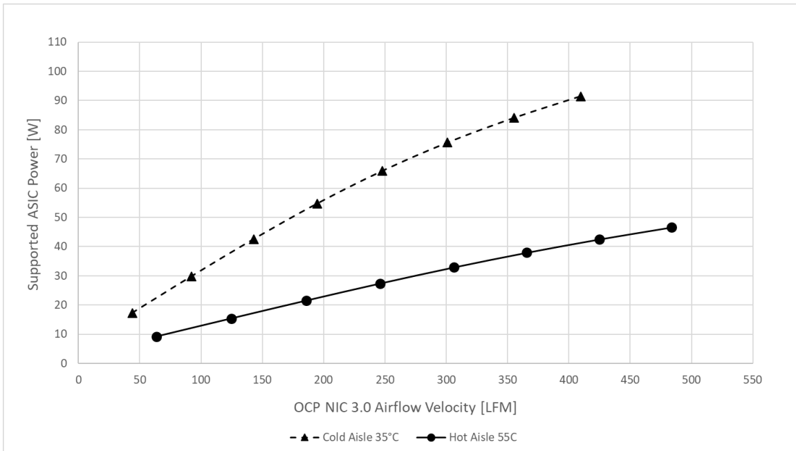
Figure 141: ASIC Supportable Power Comparison – LFF Card
