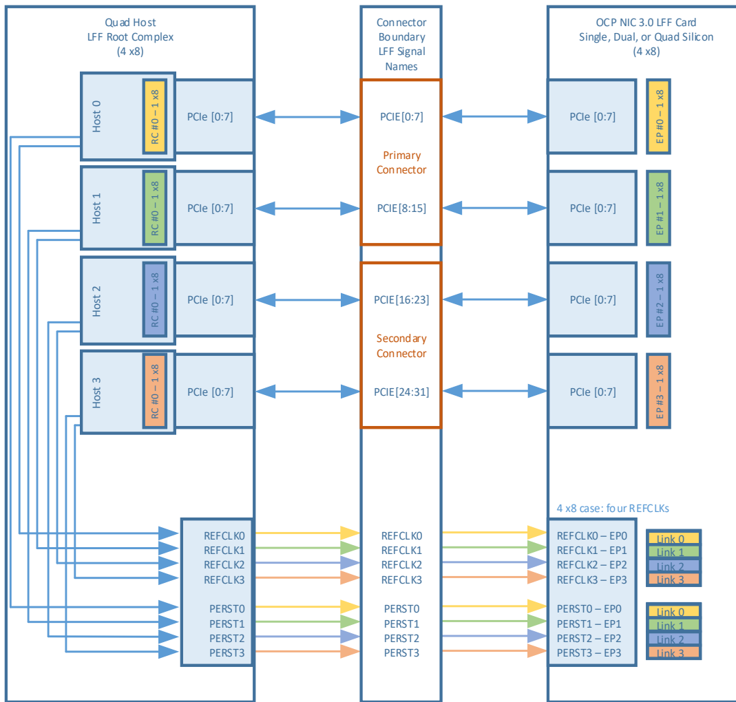
Figure 113: LFF PCIe REFCLK Mapping – Quad Host – 4 Links
