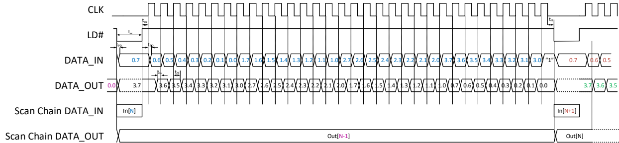
Figure 96: Scan Chain Timing Diagram Example 1
