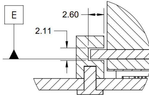
Figure 58: SFF Baseboard Chassis CTF Dimensions (Rail Guide Detail) – Detail C
