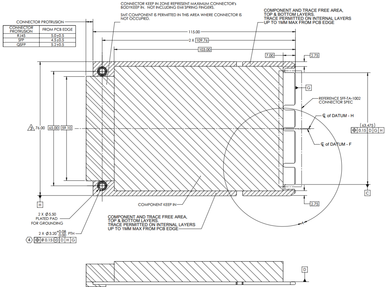
Figure 28: SFF Keep Out Zone – Top View
