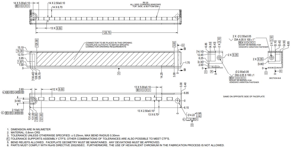
Figure 22: LFF Generic I/O Faceplate – Ejector Version (2D View)
