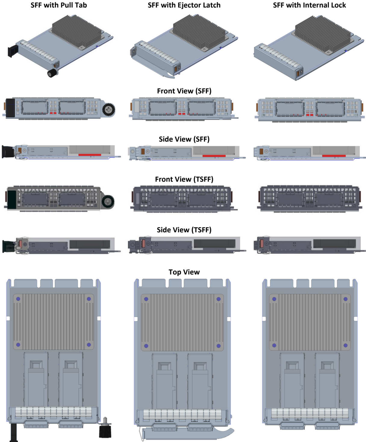
Figure 8: SFF/TSFF NIC Configuration Views
