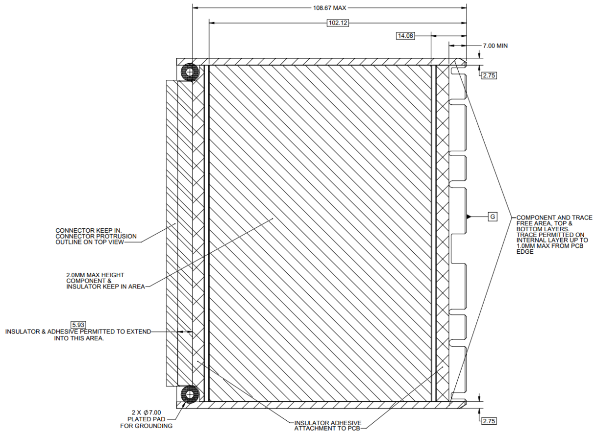
Figure 36: LFF Keep Out Zone – Bottom View
