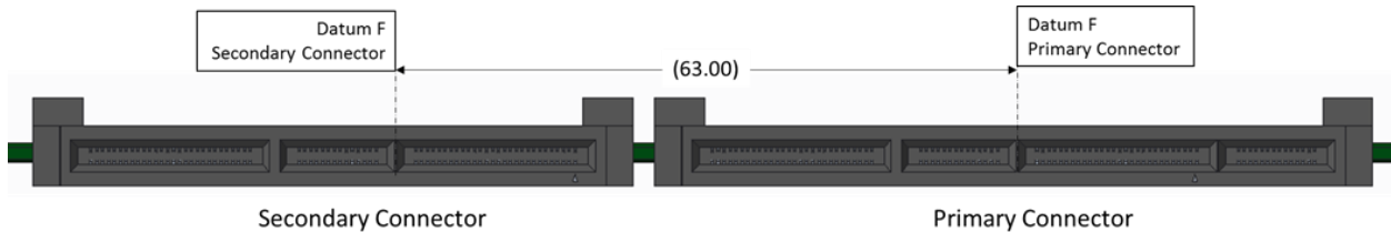
Figure 90: Primary and Secondary Connector Locations for LFF Support with Straddle Mount Connectors
