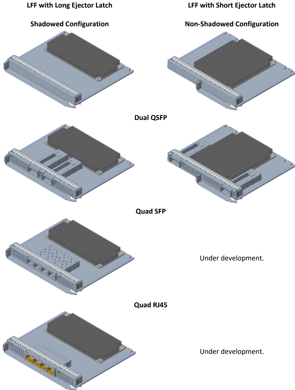
Figure 12: LFF NIC Line Side 3D Views
