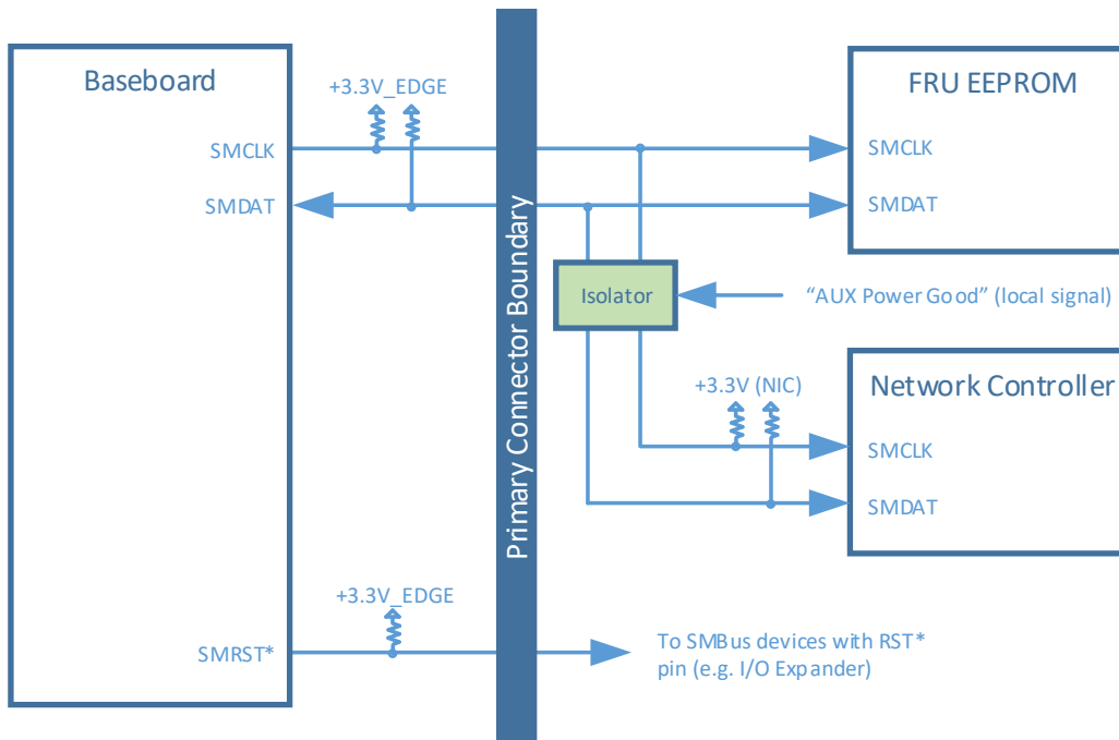
Figure 93: Example SMBus Connections
