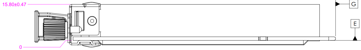
Figure 59: TSFF OCP NIC 3.0 Card with Pull Tab CTF Dimensions (Top View)
