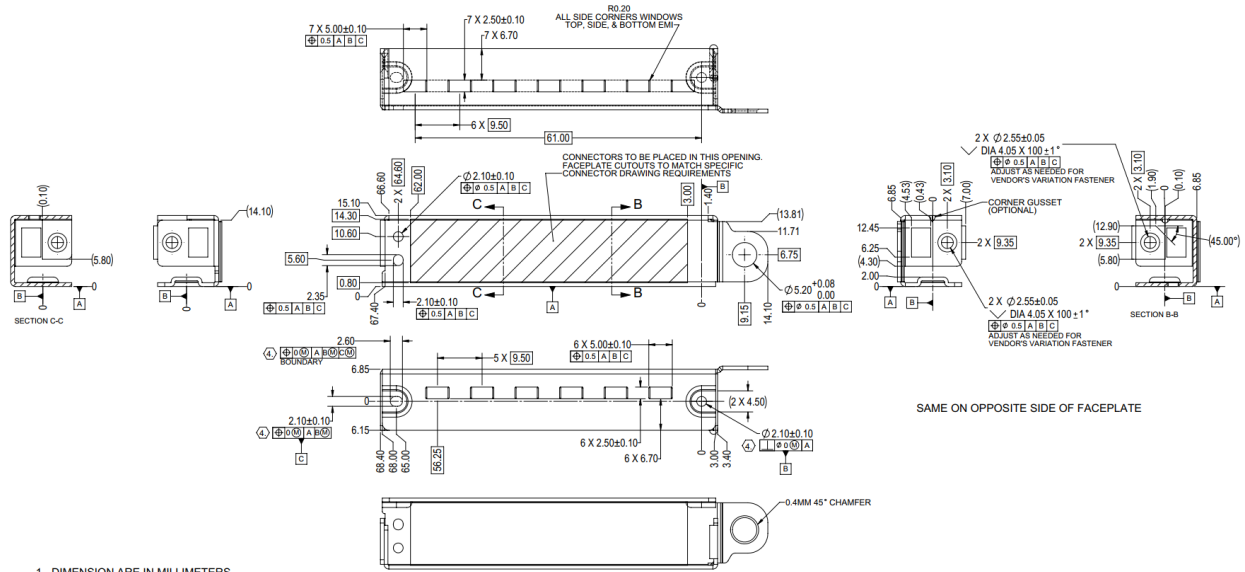
Figure 16: SFF Generic I/O Faceplate – Pull Tab Version (2D View)
