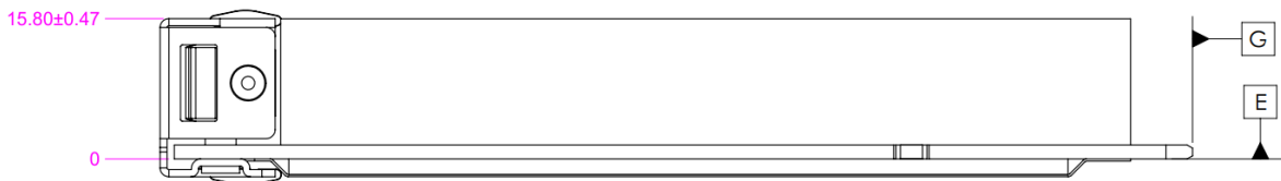
Figure 61: TSFF OCP NIC 3.0 Card with Internal Lock CTF Dimensions (Top View)
