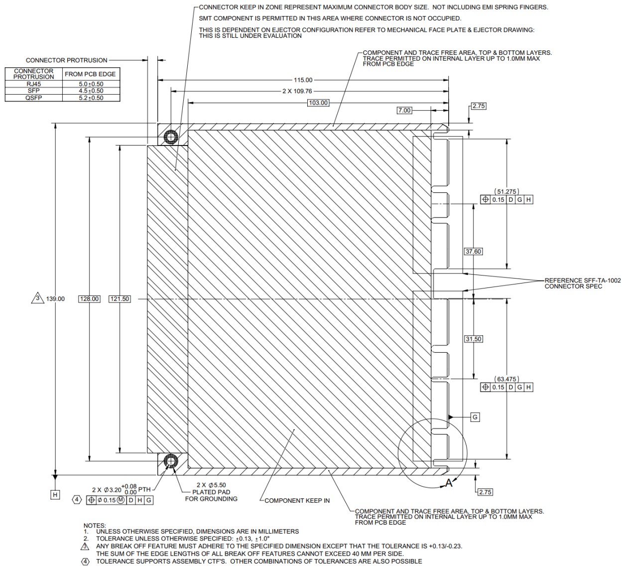
Figure 34: LFF Keep Out Zone – Top View
