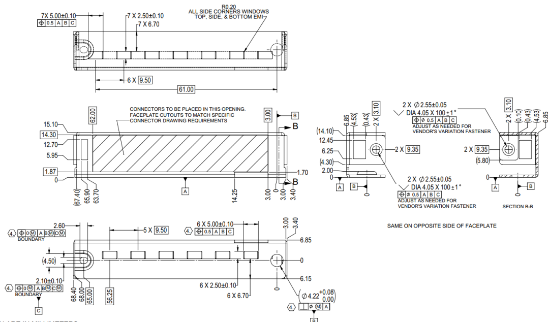
Figure 17: SFF Generic I/O Faceplate – Ejector Version (2D View)
