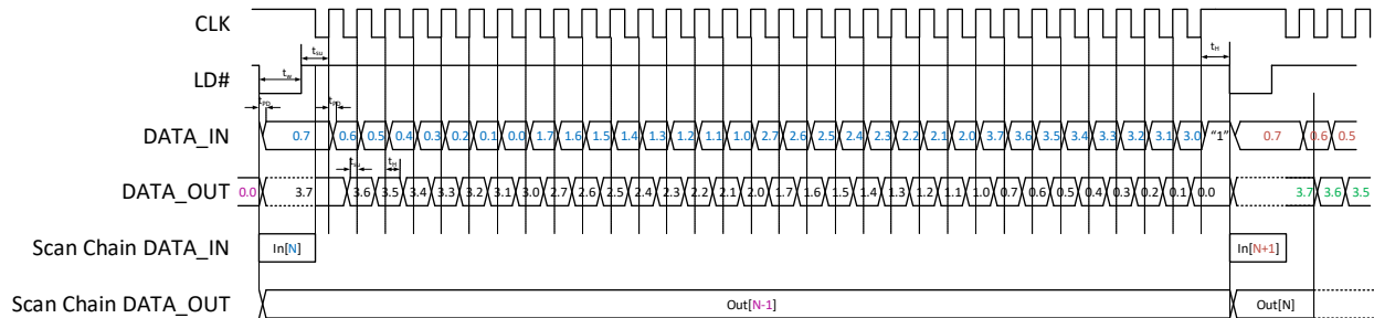
Figure 97: Scan Chain Timing Diagram Example 2
