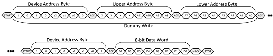
Figure 120: FRU EEPROM Reads with Double Byte Addressing
