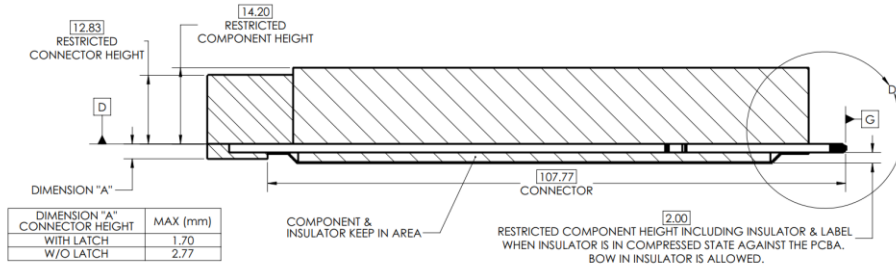
Figure 33: TSFF Keep Out Zone – Side View
