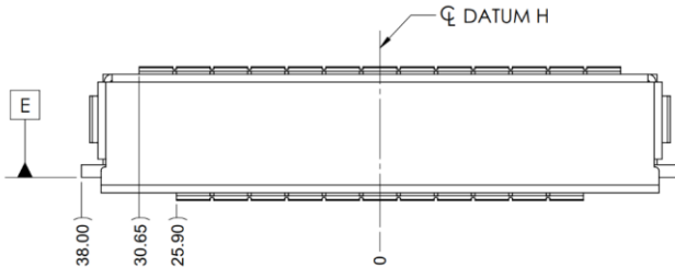
Figure 53: SFF OCP NIC 3.0 Card with Internal Lock CTF Dimensions (Side View)
