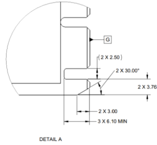
Figure 35: LFF Keep Out Zone – Top View – Detail A
