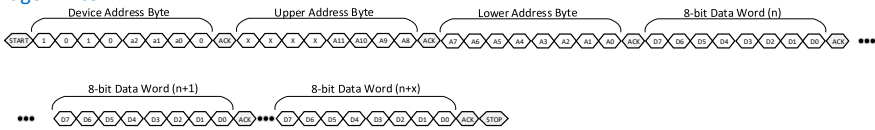
Figure 120: FRU EEPROM Reads with Double Byte Addressing
