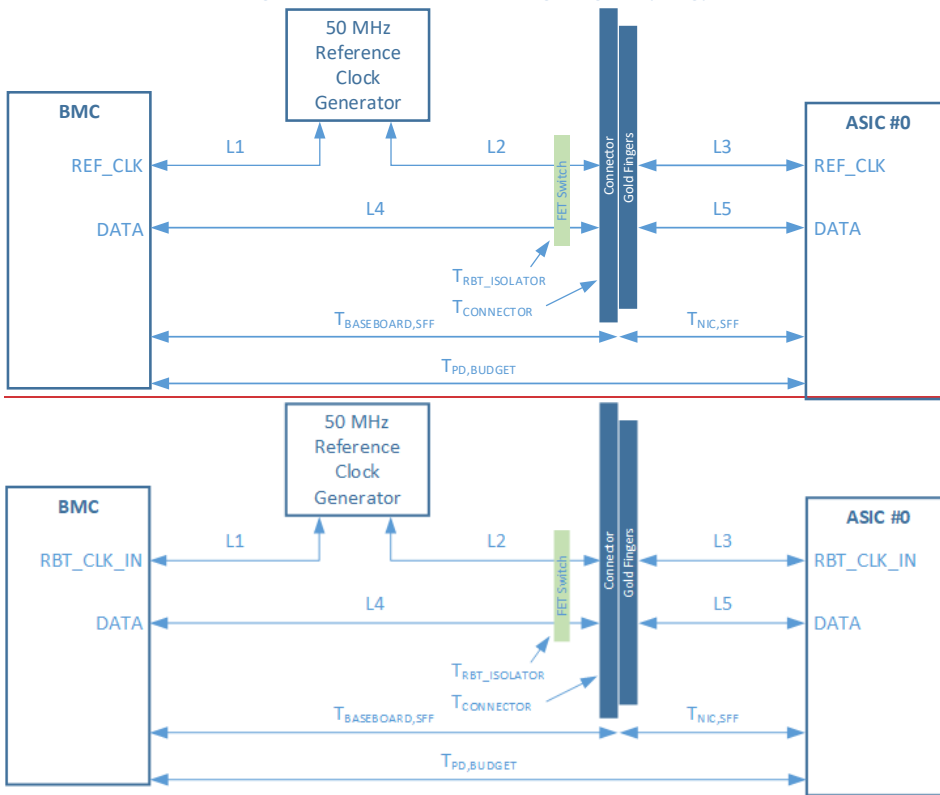
Figure 122: NC-SI over RBT Timing Budget Topology
