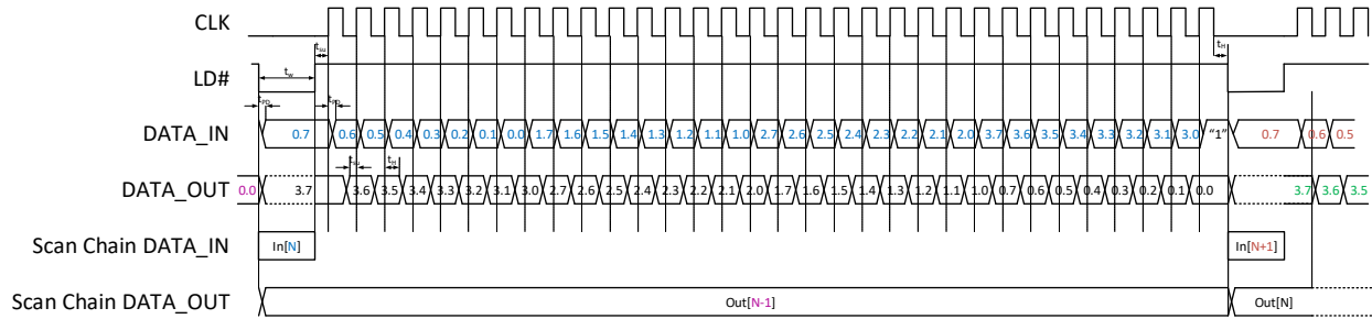
Figure 96: Scan Chain Timing Diagram Example 1
