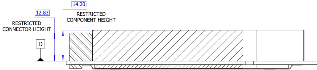
Figure 33: TSFF Keep Out Zone – Side View
