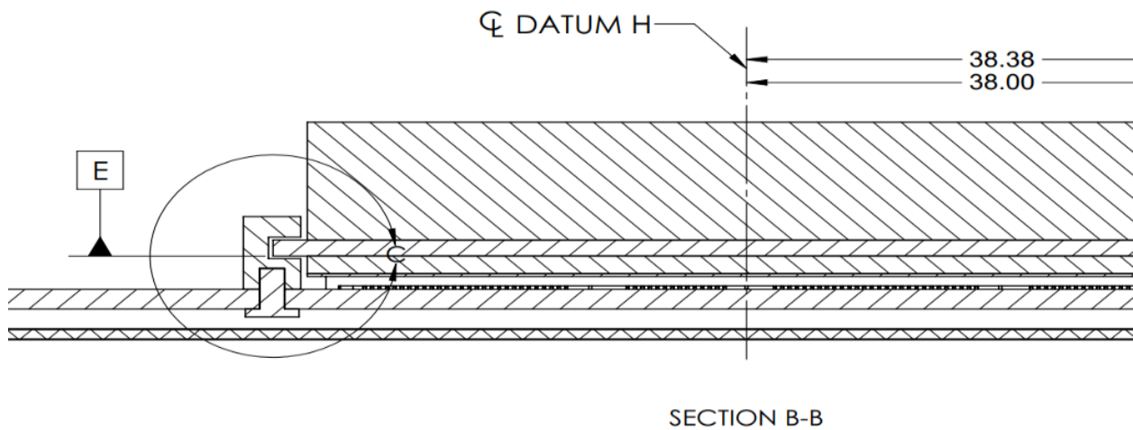
Figure 57: SFF Baseboard Chassis CTF Dimensions (Rear Rail Guide View)
