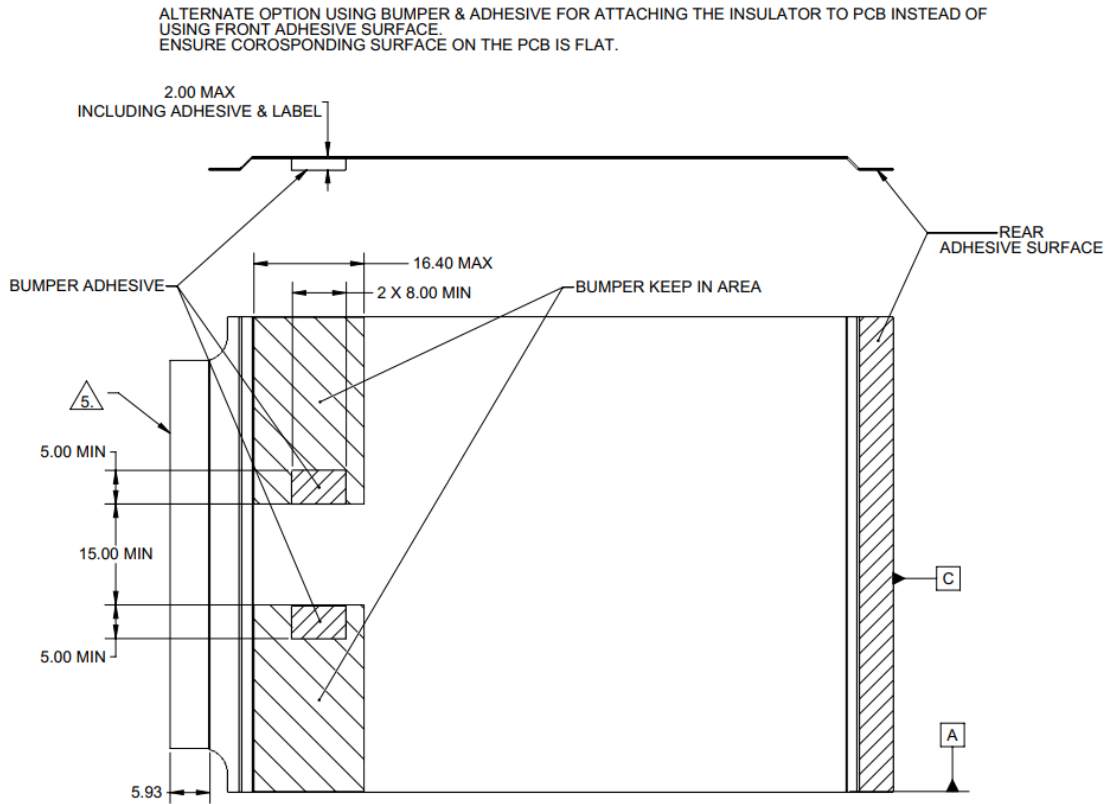
Figure 41: SFF, TSFF Bottom Side Insulator (alternate) (Top and Side View)
