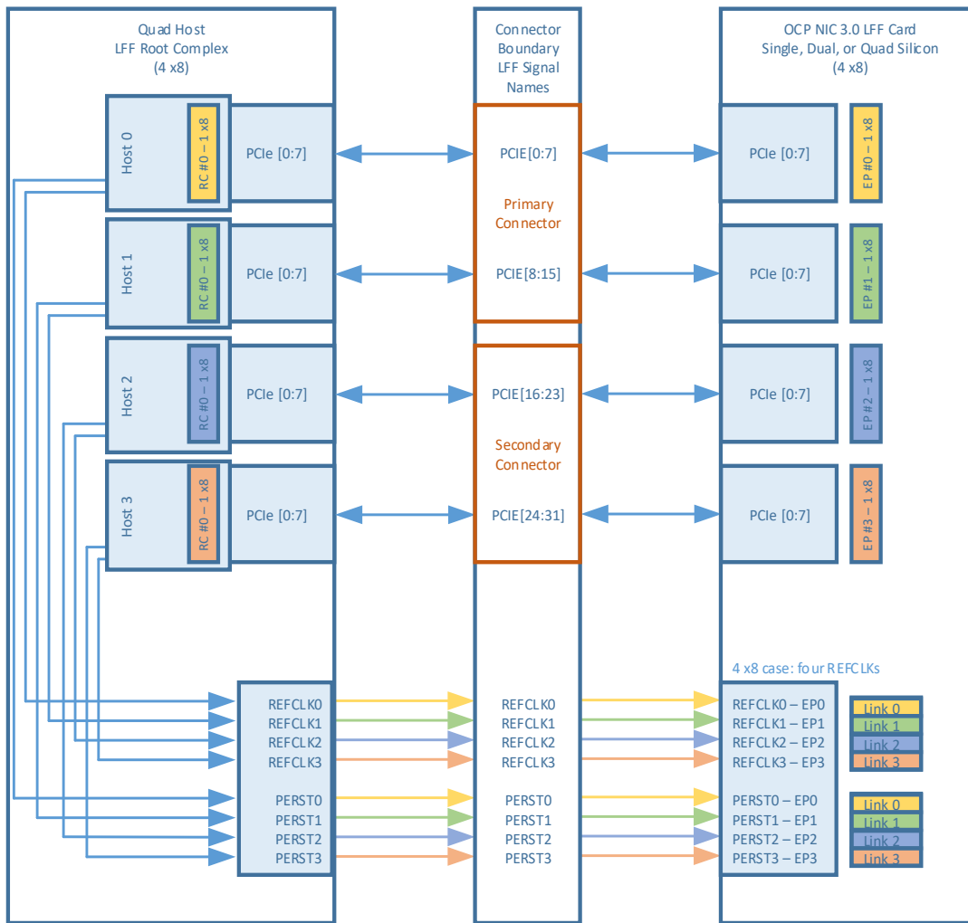
Figure 112: LFF PCIe REFCLK Mapping – Quad Host – 4 Links
