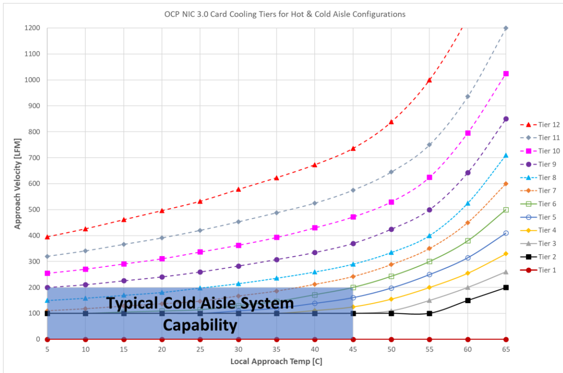
Figure 154: Typical Operating Range for Cold Aisle Configurations
