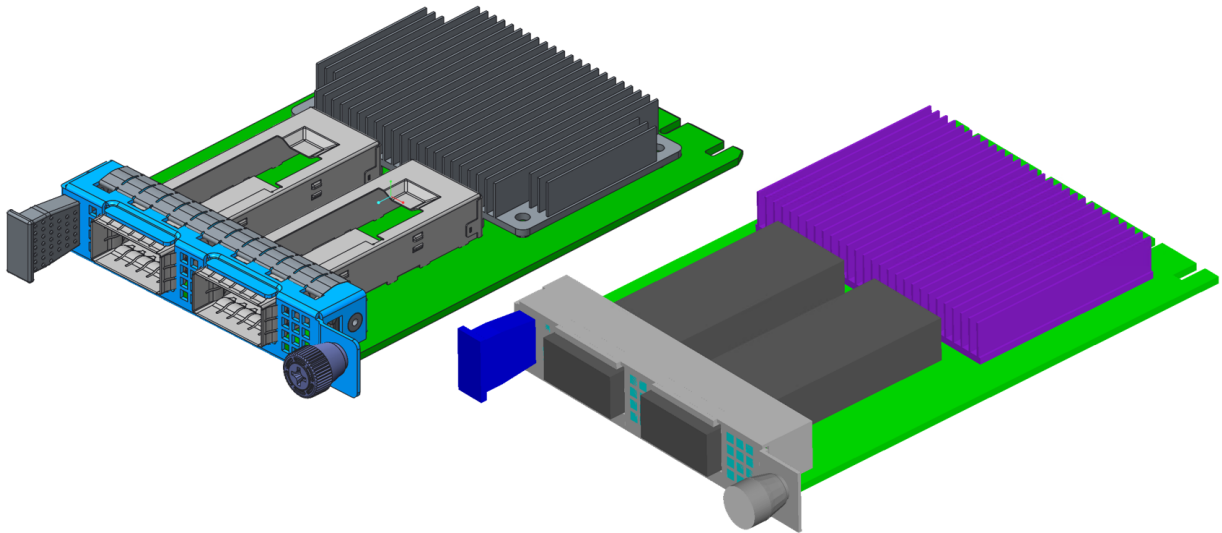
Figure 129: OCP NIC 3.0 SFF Reference Design and CFD Geometry
