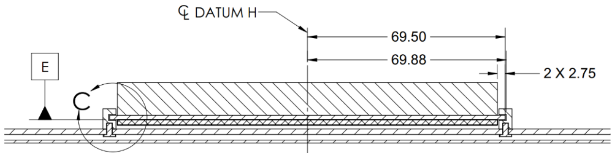
Figure 67: LFF Baseboard Chassis CTF Dimensions (Rail Guide View)
