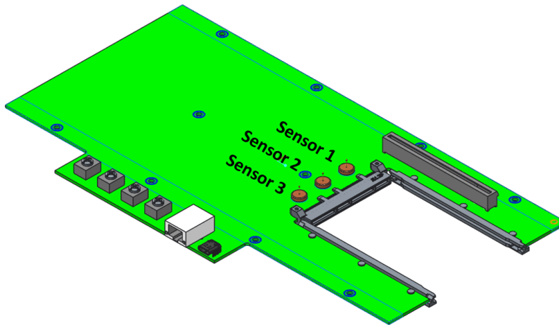
Figure 143: SFF Card Thermal Test Fixture PCB
