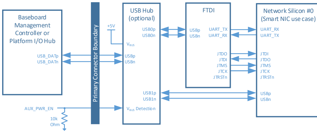
Figure 100: USB 2.0 Connection Example – USB-Serial / USB-JTAG Connectivity
