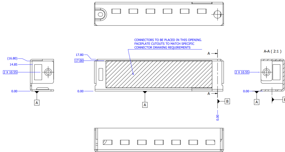
Figure 19: TSFF Generic I/O Faceplate – Ejector Version (2D View)
