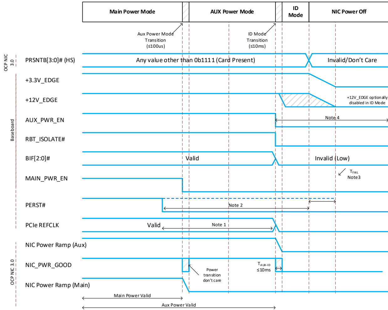
Figure 116: Power-Down Sequencing – Normal Operation
