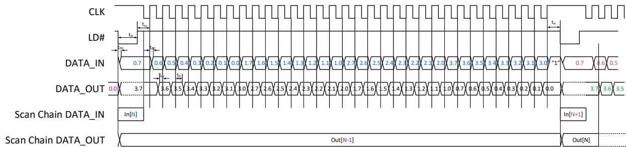
Figure 96: Scan Chain Timing Diagram Example 2
