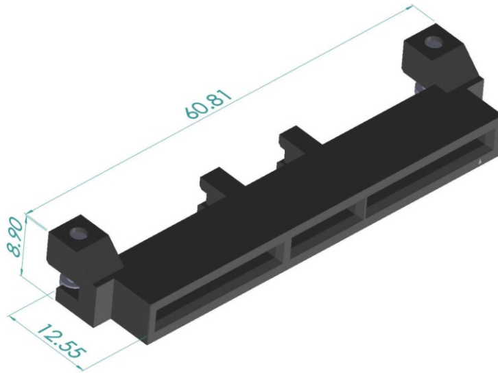
Figure 84: 140-pin Base Board Secondary Connector – Straddle Mount
