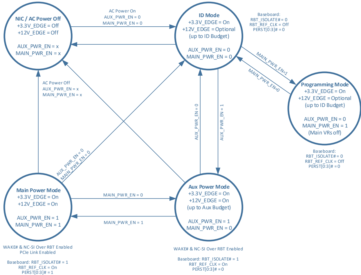
Figure 114: Baseboard Power States
