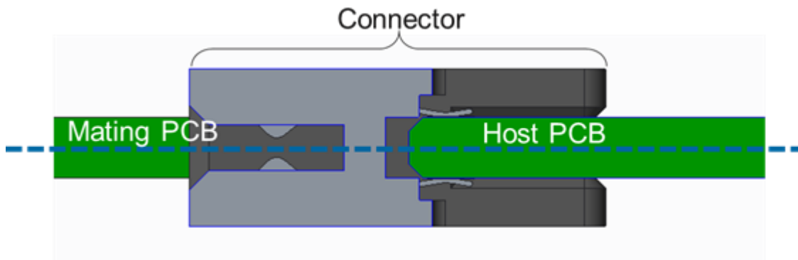
Figure 86: 0 mm Offset (Coplanar) for 0.062" Thick Baseboards
