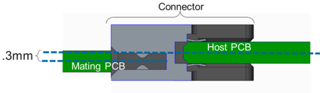
Figure 87: 0.3 mm Offset for 0.076" Thick Baseboards
