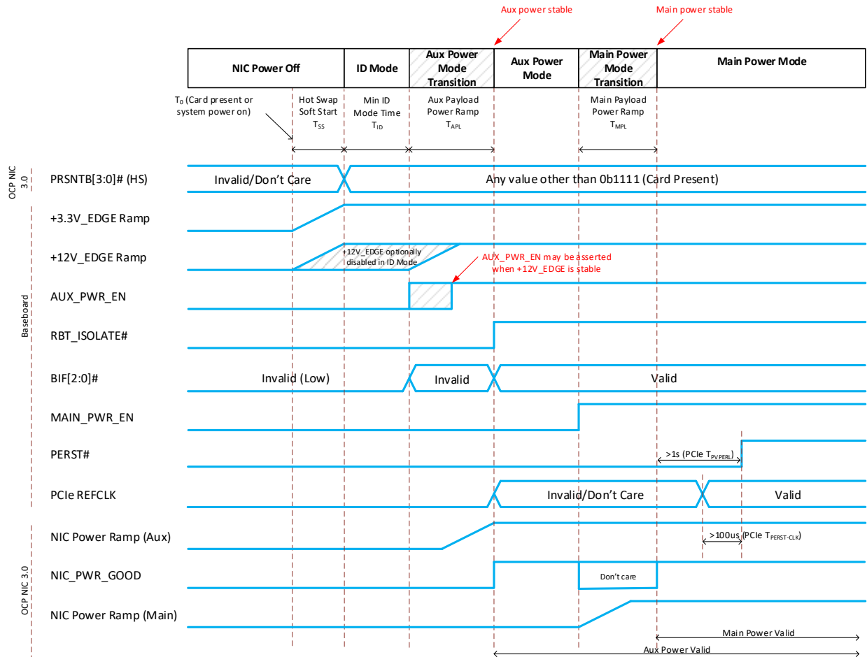
Figure 115: Power-Up Sequencing – Normal Operation
