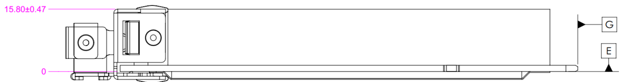
Figure 59: TSFF OCP NIC 3.0 Card with Ejector Latch CTF Dimensions (Top View)
