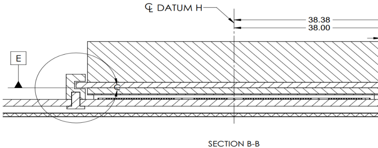
Figure 56: SFF Baseboard Chassis CTF Dimensions (Rear Rail Guide View)
