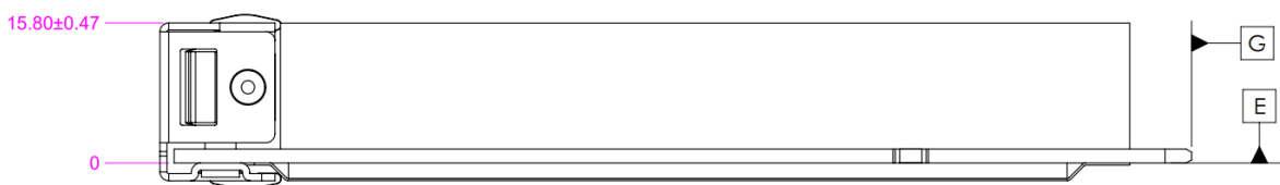
Figure 60: TSFF OCP NIC 3.0 Card with Internal Lock CTF Dimensions (Top View)
