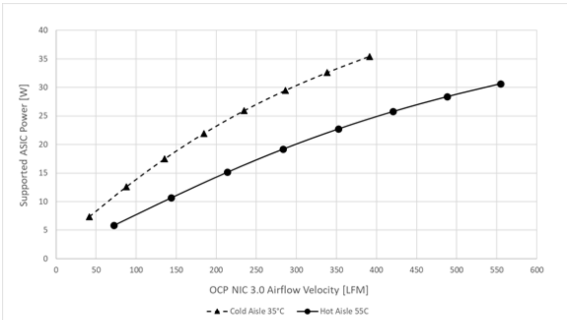
Figure 137: ASIC Supportable Power Comparison – SFF Card
