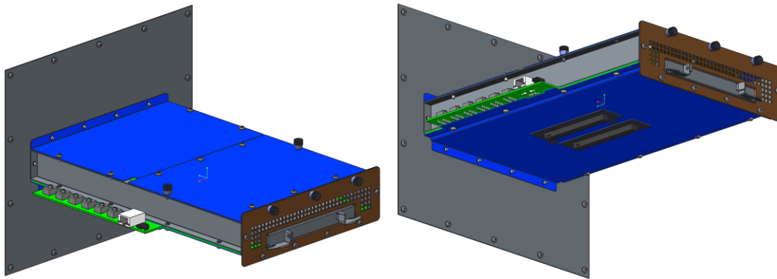
Figure 144: LFF Card Thermal Test Fixture Design
