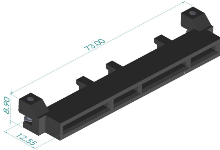
Figure 83: 168-pin Base Board Primary Connector – Straddle Mount
