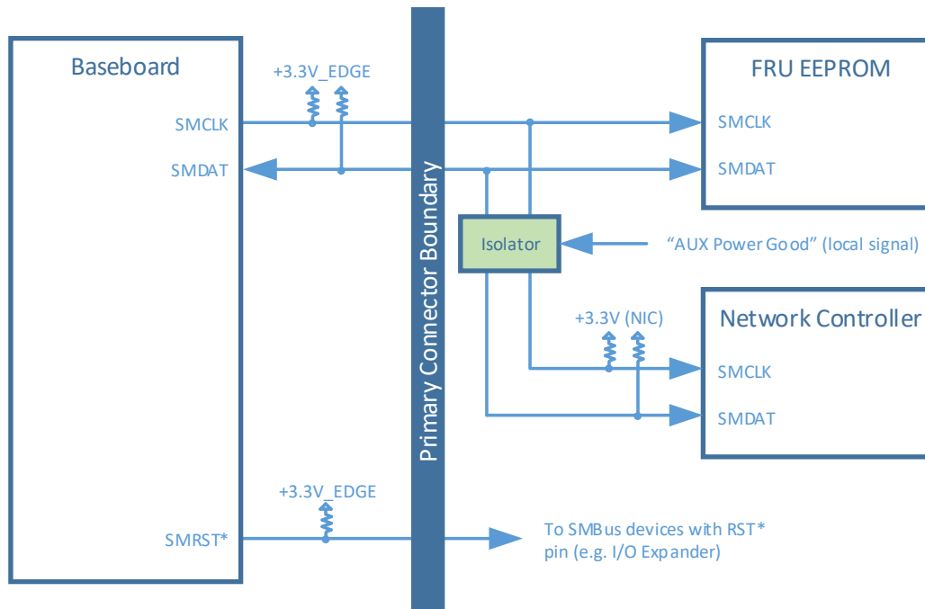
Figure 92: Example SMBus Connections
