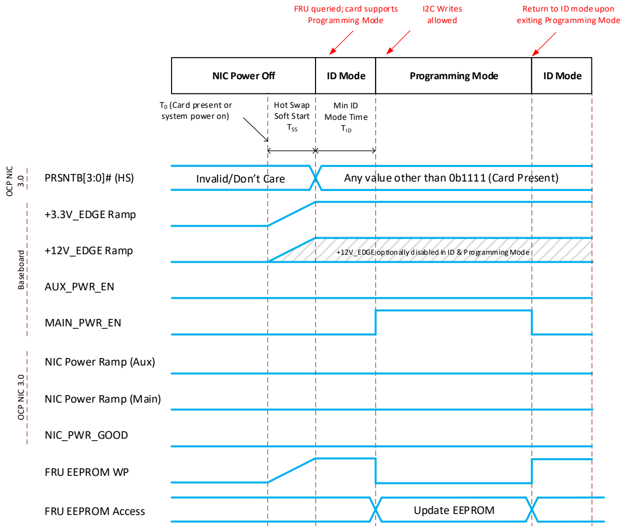
Figure 117: Programming Mode Sequencing
