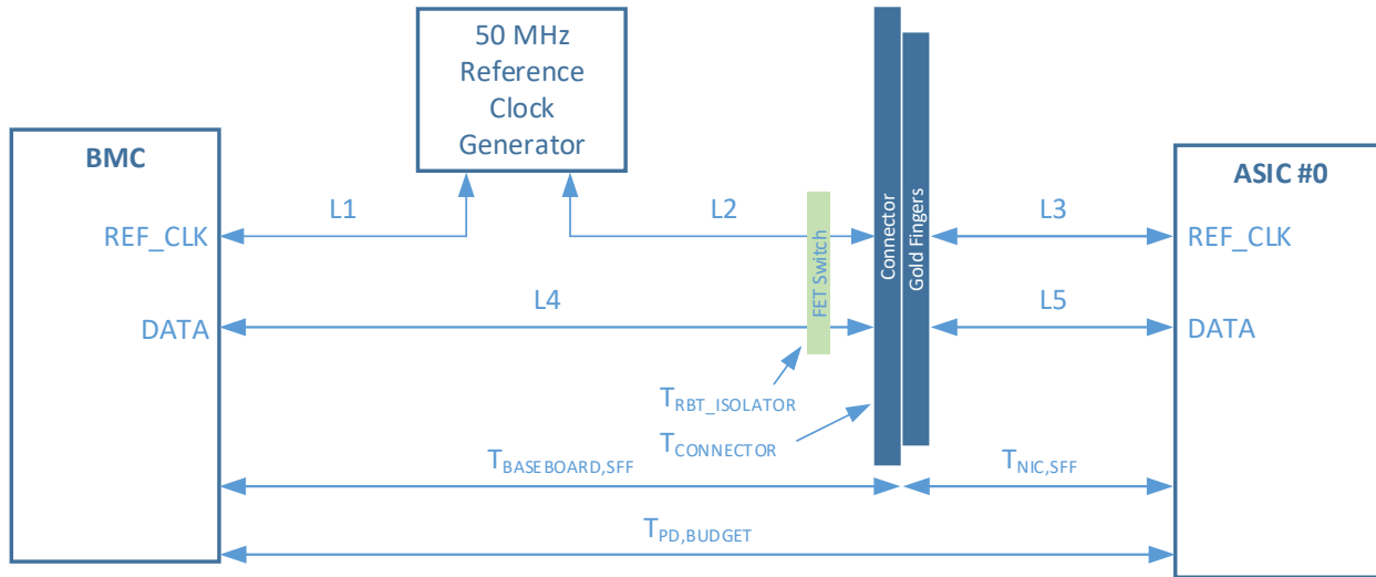
Figure 121: NC-SI over RBT Timing Budget Topology
