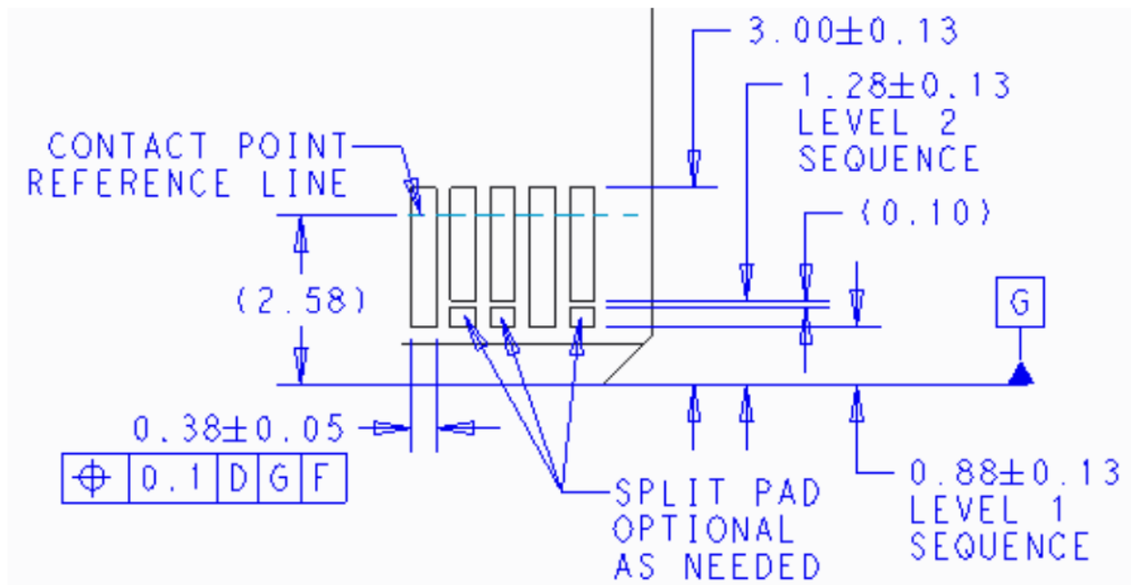
Figure 77: SFF, TSFF Primary Connector Gold Finger - Detail D
