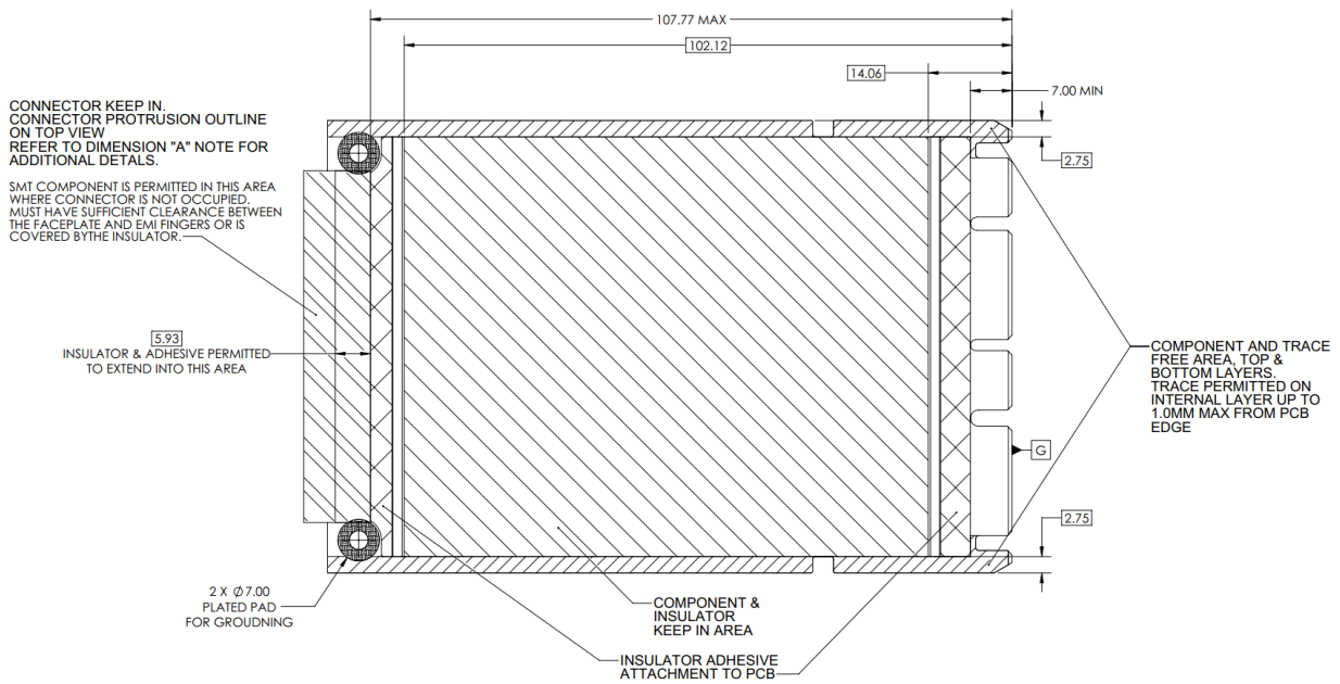
Figure 29: SFF Keep Out Zone – Bottom View
