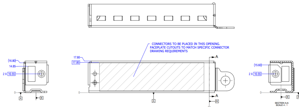
Figure 18: TSFF Generic I/O Faceplate – Pull Tab Version (2D View)
