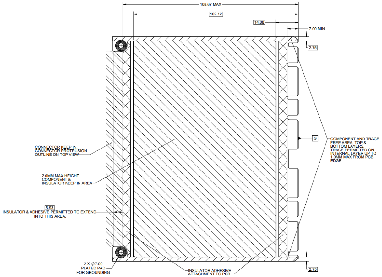
Figure 35: LFF Keep Out Zone – Bottom View
