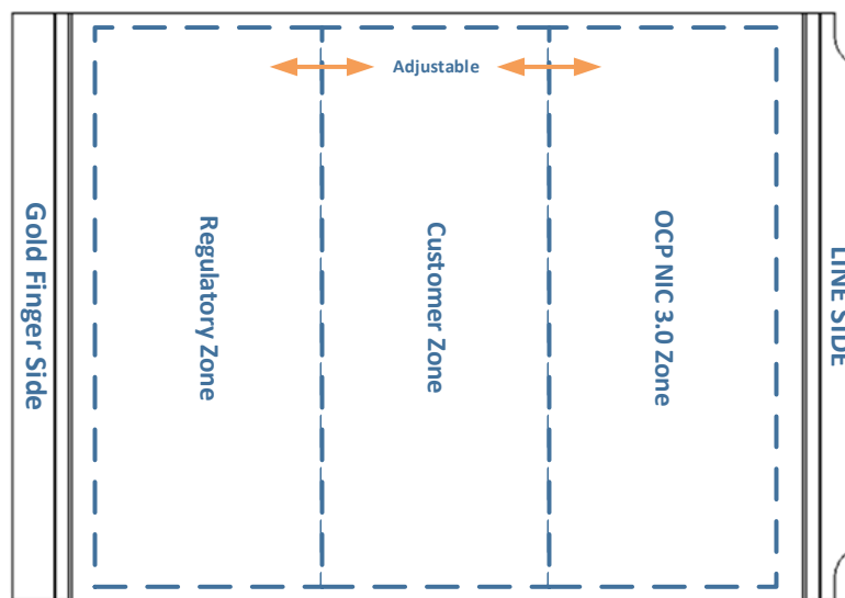
Figure 69: SFF, TSFF Label Area Example
