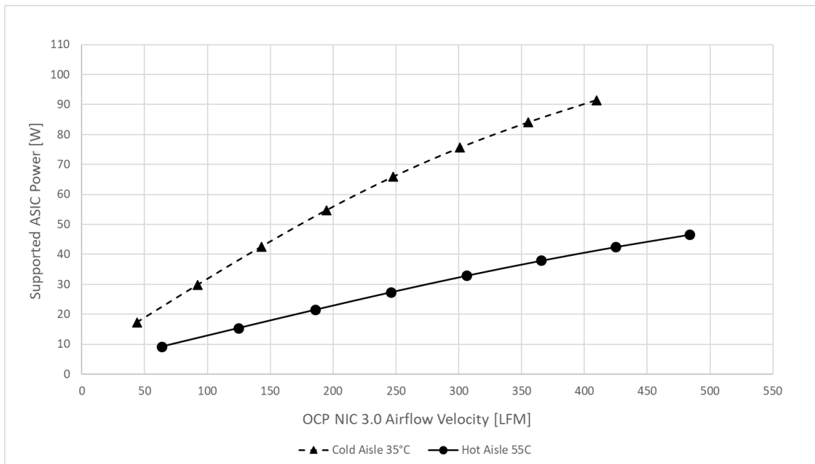
Figure 140: ASIC Supportable Power Comparison – LFF Card
