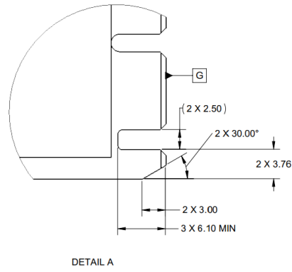
Figure 34: LFF Keep Out Zone – Top View – Detail A
