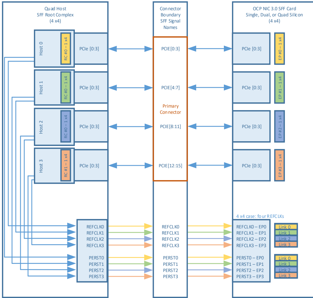
Figure 109: SFF/TSFF PCIe REFCLK Mapping – Quad Host – 4 Links
