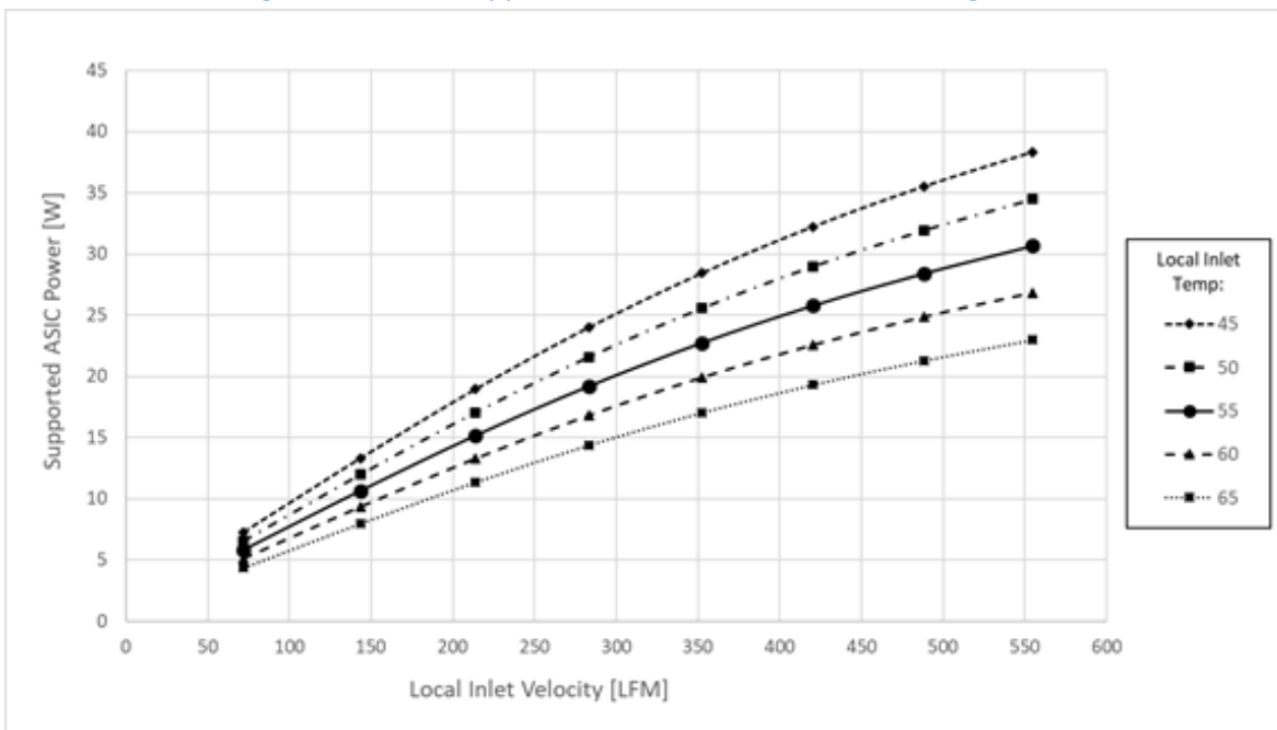
Figure 128: ASIC Supportable Power for Hot Aisle Cooling – SFF
