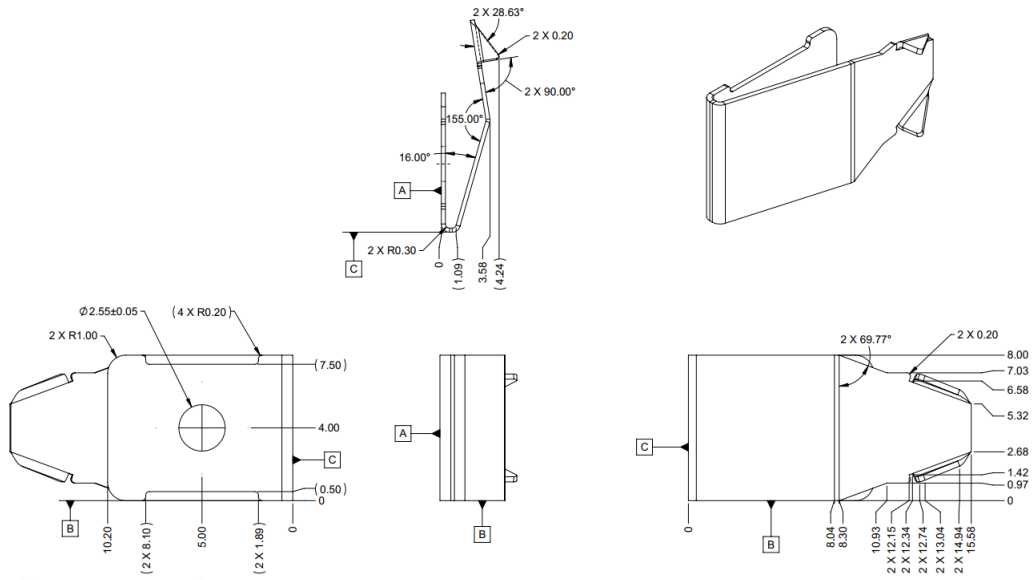
Figure 24: Ejector Lock
