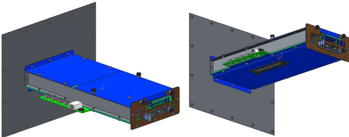
Figure 141: SFF Thermal Test Fixture Preliminary Design
