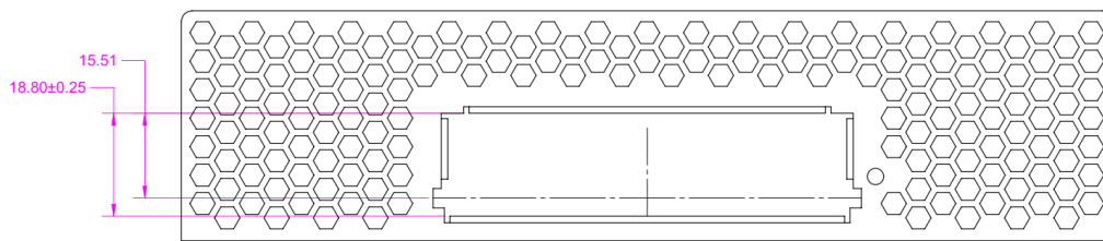
Figure 61: TSFF Baseboard Chassis CTF Dimensions (Rear View)
