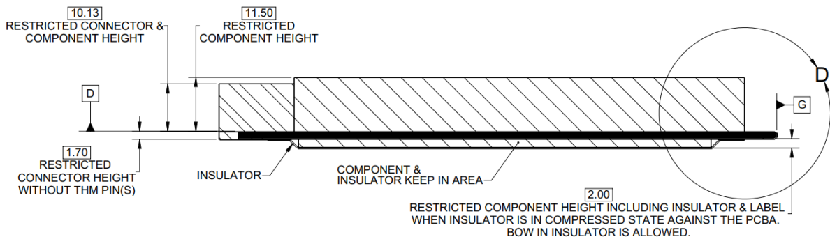
Figure 36: LFF Keep Out Zone – Side View
