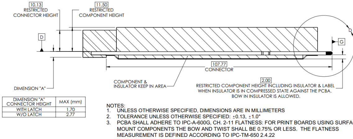
Figure 30: SFF Keep Out Zone – Side View
