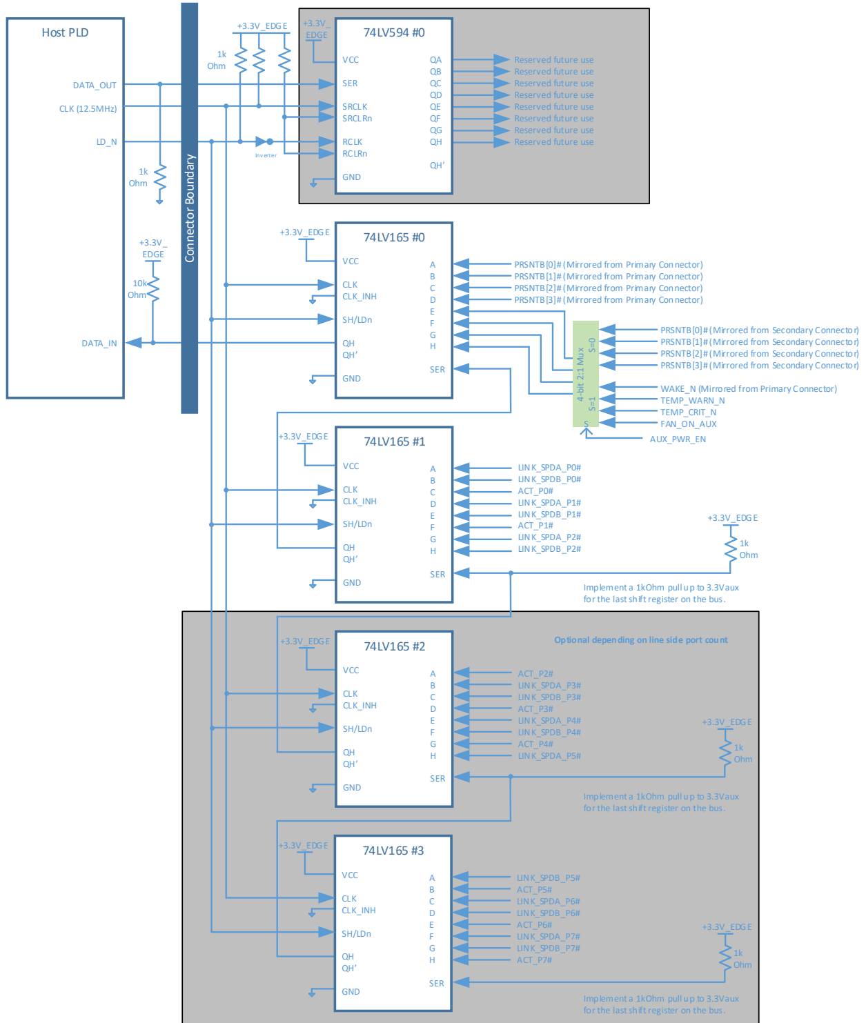
Figure 97: Scan Chain Connection Example
