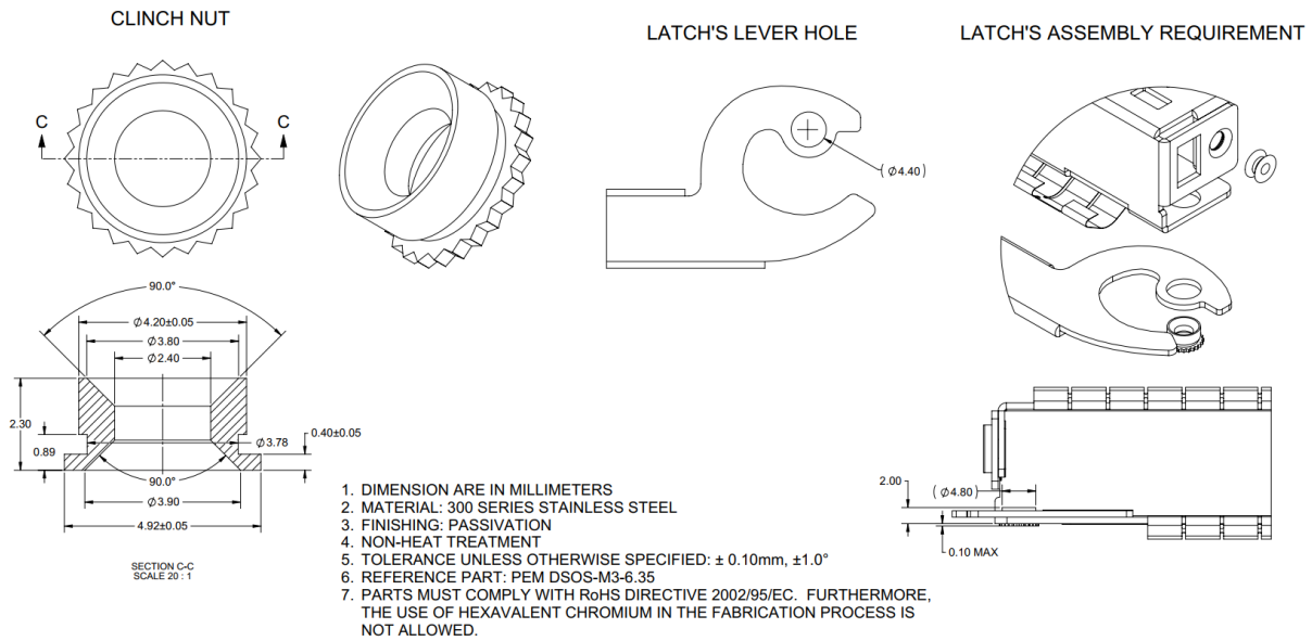
Figure 25: Clinch Nut Option A
