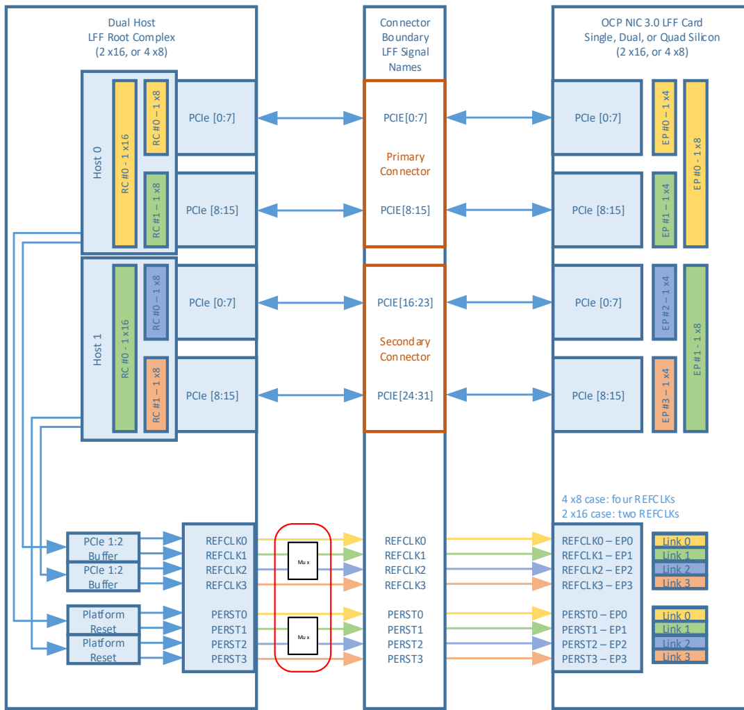
Figure 111: LFF PCIe REFCLK Mapping – Dual Host – 2 and 4 links
