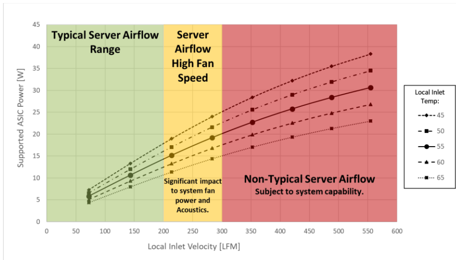
Figure 130: Server System Airflow Capability – SFF Card Hot Aisle Cooling
