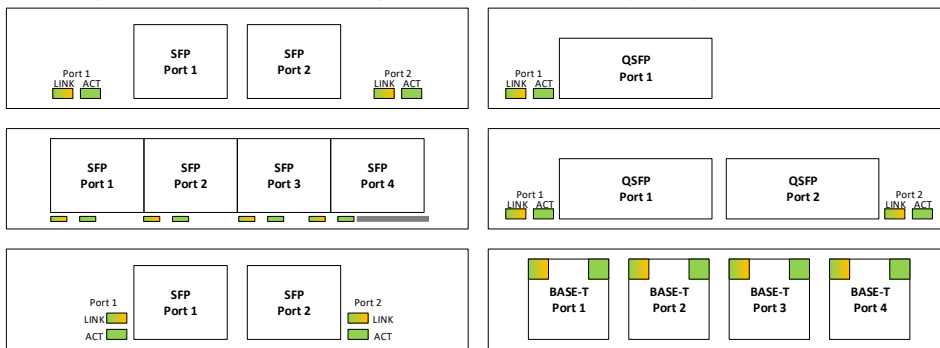
Figure 113: Port and LED Ordering – Example SFF Link/Activity and Speed LED Placement
