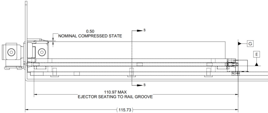
Figure 67: LFF Baseboard Chassis CTF Dimensions (Rail Guide View)
