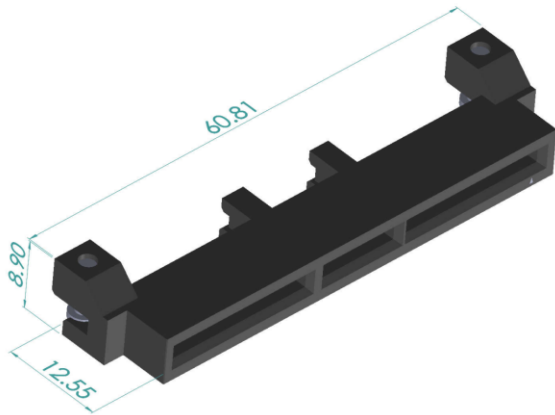
Figure 84: 140-pin Base Board Secondary Connector – Straddle Mount
