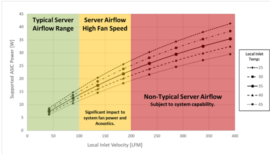
Figure 136: Server System Airflow Capability – SFF Cold Aisle Cooling
