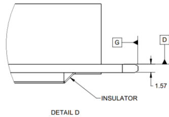
Figure 37: LFF Keep Out Zone – Side View – Detail D
