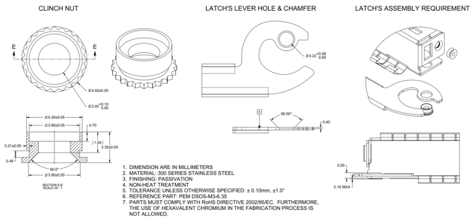
Figure 26: Clinch Nut Option B
