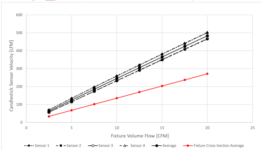
Figure 151: LFF Fixture, Hot Aisle Flow – Candlestick Air Velocity vs. Volume Flow
