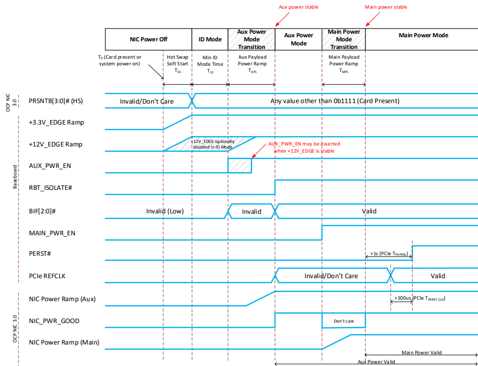
Figure 115: Power-Up Sequencing – Normal Operation
