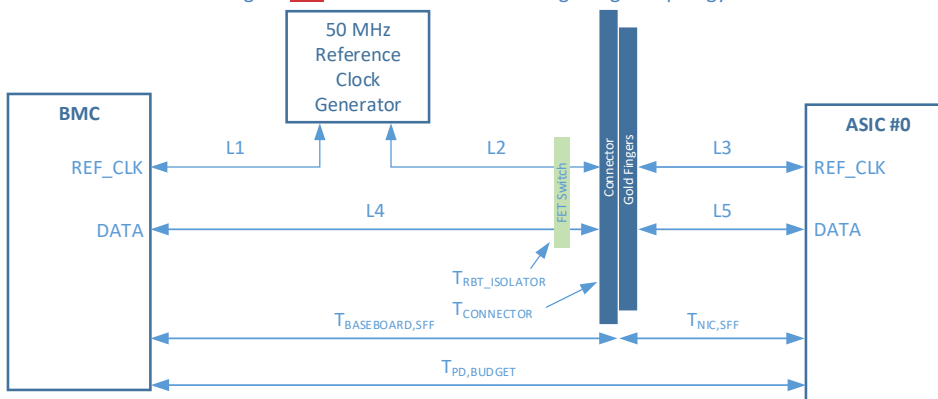
Figure 121413: NC-SI over RBT Timing Budget Topology
