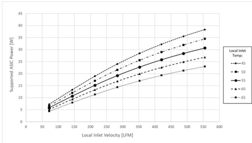
Figure 128120: ASIC Supportable Power for Hot Aisle Cooling – SFF
