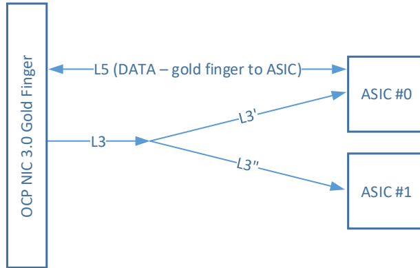
Figure 122: NC-SI over RBT Propagation Delay Matching for Two Target ASICs – No Clock Buffer
