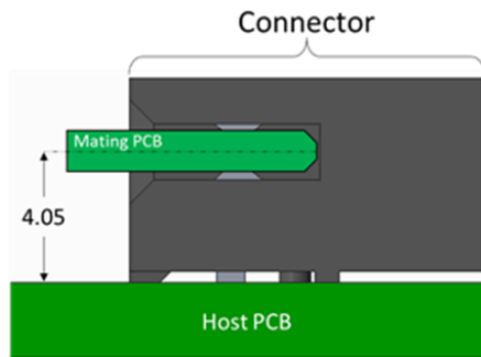
Figure 82: OCP NIC 3.0 Card and Host Offset for Right Angle Connectors
