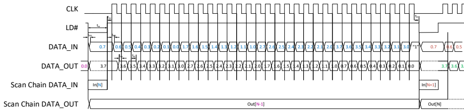
Figure 95: Scan Chain Timing Diagram Example 1
