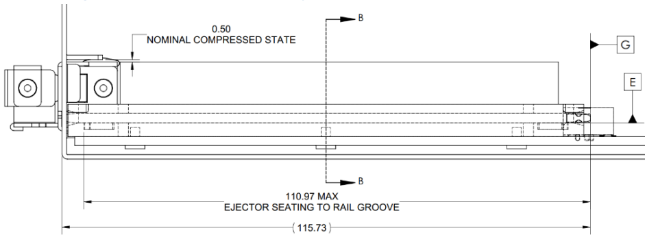
Figure 55: SFF Baseboard Chassis to Ejector lever Card CTF Dimensions (Side View)
