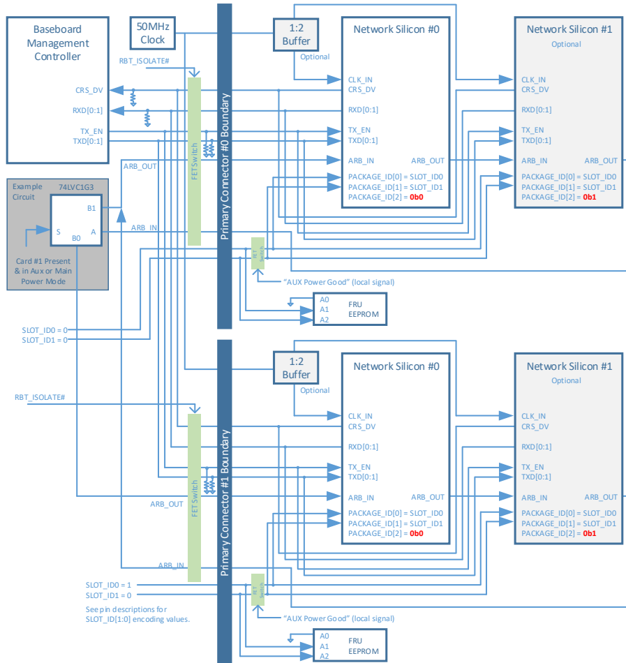
Figure 94: NC-SI over RBT Connection Example – Dual Primary Connectors
