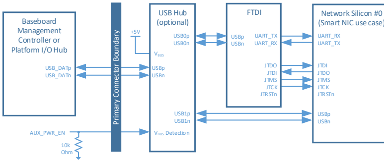
Figure 100: USB 2.0 Connection Example – USB-Serial / USB-JTAG Connectivity
