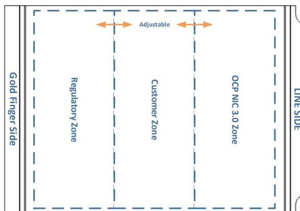
Figure 69: SFF, TSFF Label Area Example
