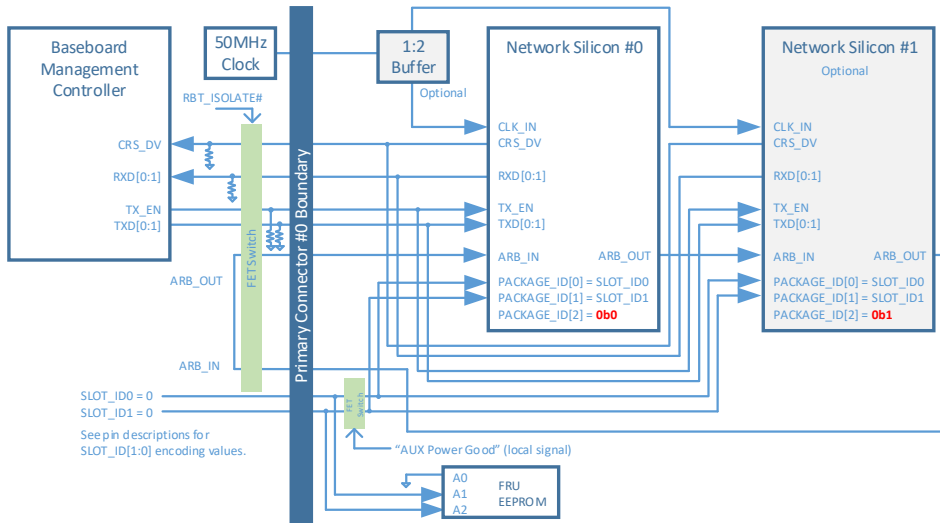
Figure 93: NC-SI over RBT Connection Example – Single Primary Connector
