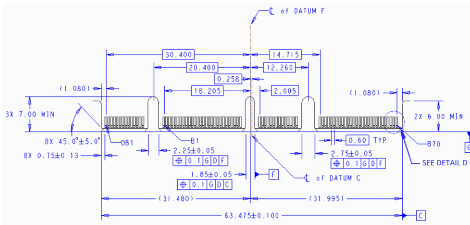
Figure 75: SFF, TSFF Primary Connector Gold Finger Dimensions – x16 – Top Side (“B” Pins)
