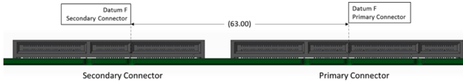
Figure 88: Primary and Secondary Connector Locations for LFF Support with Right Angle Connectors
