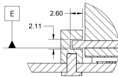
Figure 68: LFF Baseboard Chassis CTF Dimensions (Rail Guide – Detail C)
