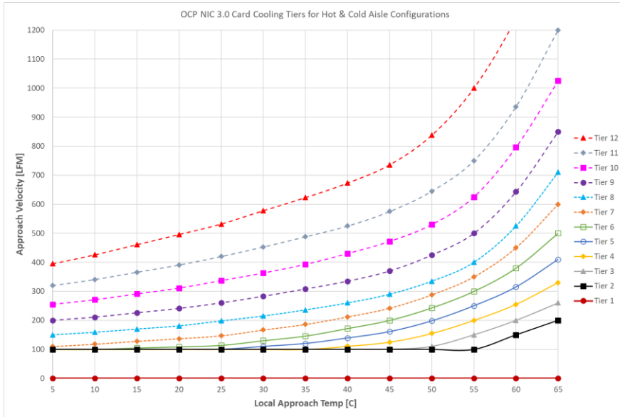
Figure 153: Typical Operating Range for Hot Aisle Configurations
