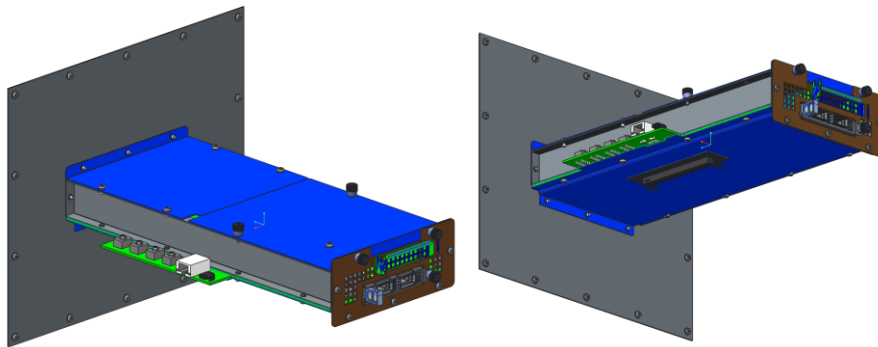
Figure 141: SFF Thermal Test Fixture Preliminary Design
