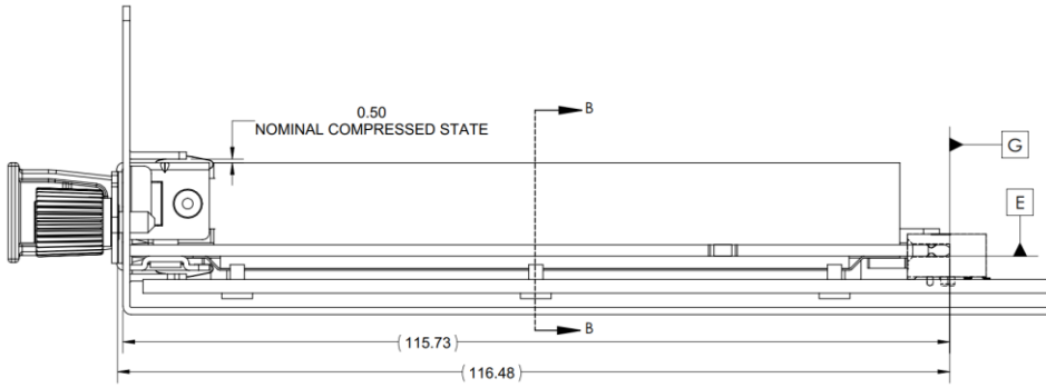
Figure 54: SFF Baseboard Chassis to Card Thumb Screw CTF Dimensions (Side View)
