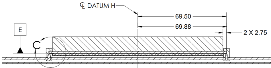
Figure 67: LFF Baseboard Chassis CTF Dimensions (Rail Guide View)
