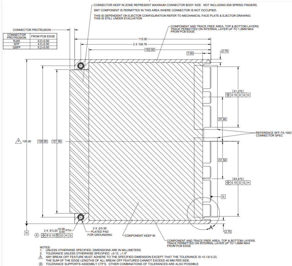
Figure 33: LFF Keep Out Zone – Top View
