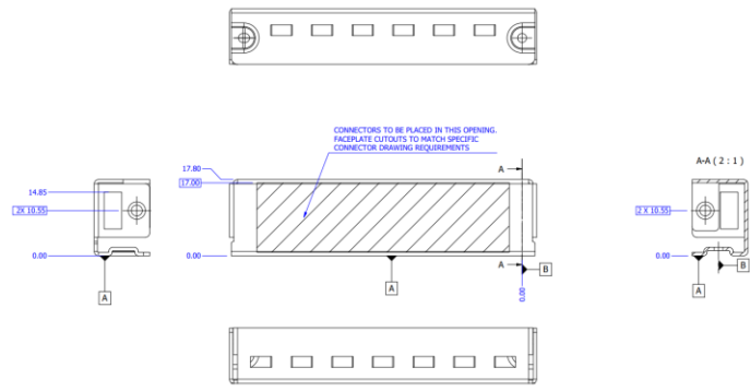
Figure 20: TSFF Generic I/O Faceplate – Internal Lock Version (2D View)
