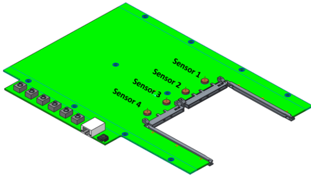
Figure 146: LFF Card Thermal Test Fixture PCB
