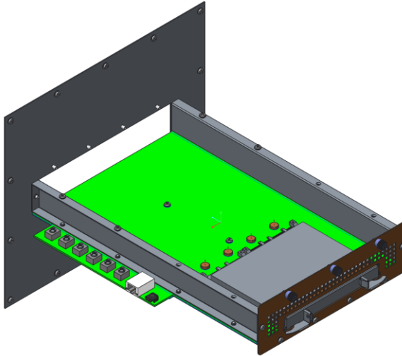
Figure 145 : LFF Card Thermal Test Fixture Design – Cover Removed
