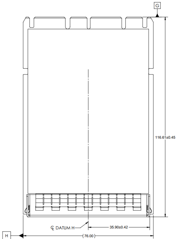
Figure 50: SFF OCP NIC 3.0 Card with Internal Lock CTF Dimensions (Top View)
