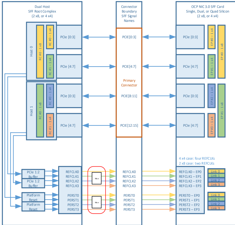
Figure 108: SFF/TSFF PCIe REFCLK Mapping – Dual Host – 2 and 4 links
