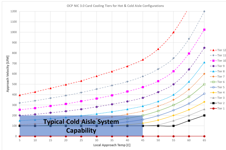
Figure 154: Typical Operating Range for Cold Aisle Configurations
