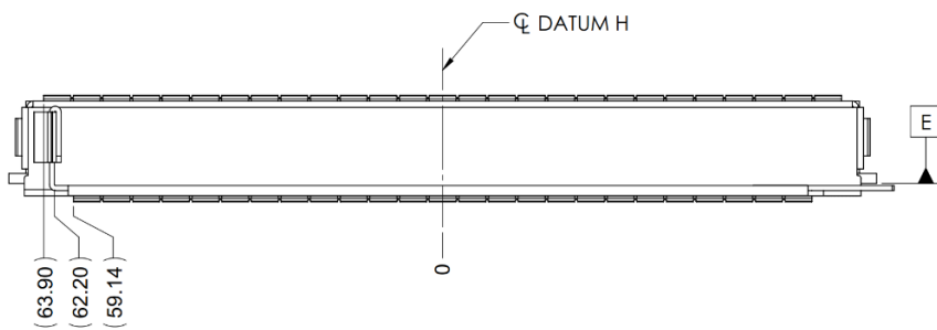
Figure 63: LFF OCP NIC 3.0 Card with Ejector CTF Dimensions (Front View)
