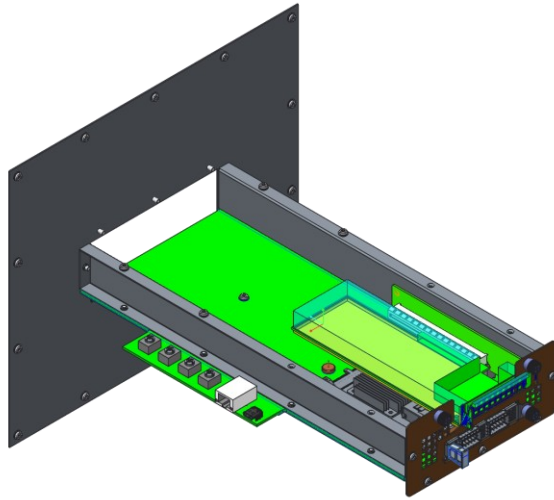
Figure 142: SFF Thermal Test Fixture Preliminary Design – Cover Removed
