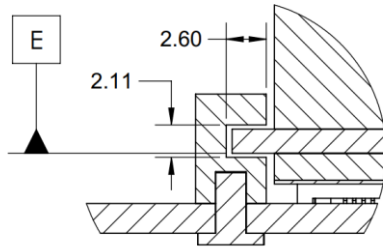
Figure 57: SFF Baseboard Chassis CTF Dimensions (Rail Guide Detail) – Detail C
