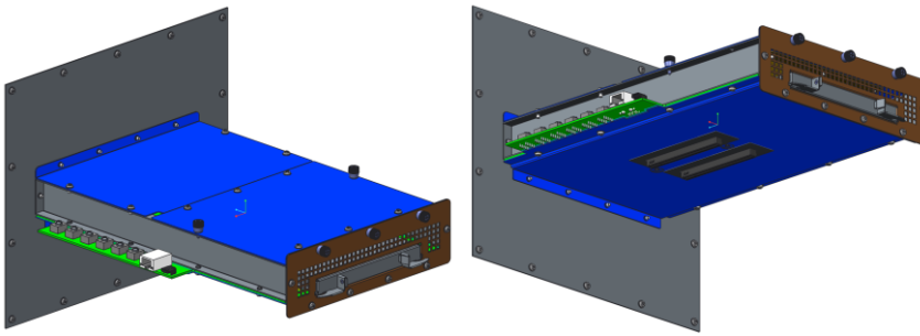
Figure 144 : LFF Card Thermal Test Fixture Design
