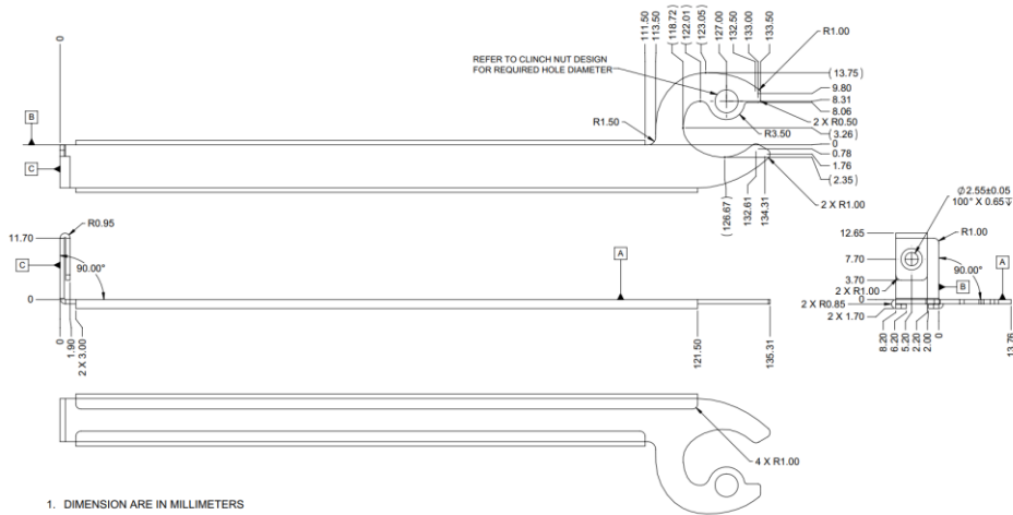
Figure 23: LFF I/O Faceplate – Ejector Lever (2D View)
