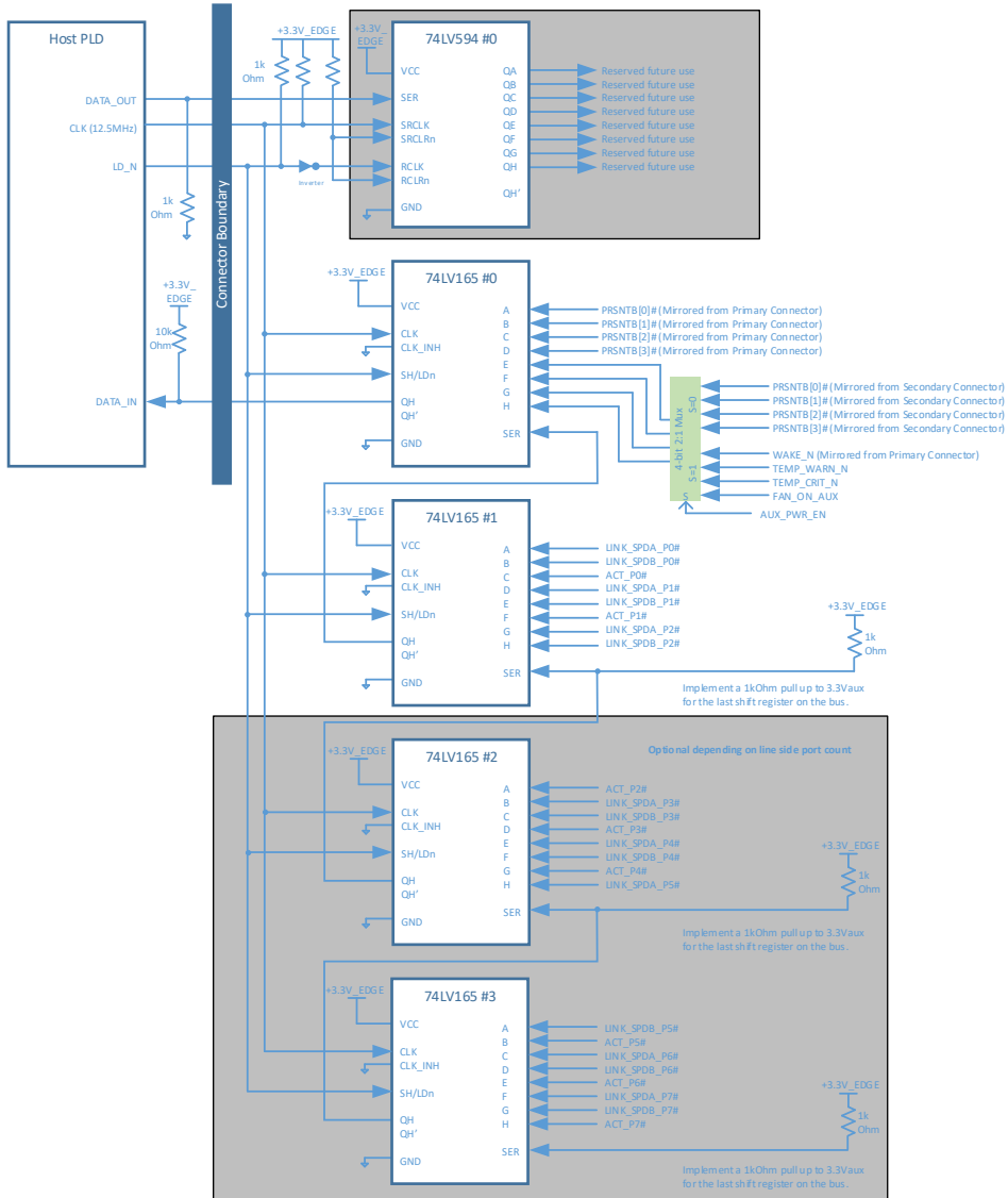
Figure 97: Scan Chain Connection Example
