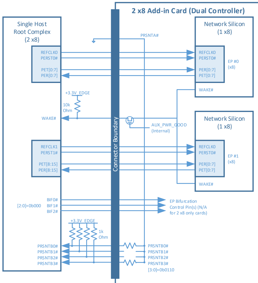
Figure 103: Single Host (2 x8) and 2 x8 OCP NIC 3.0 Card (Dual Controllers)
