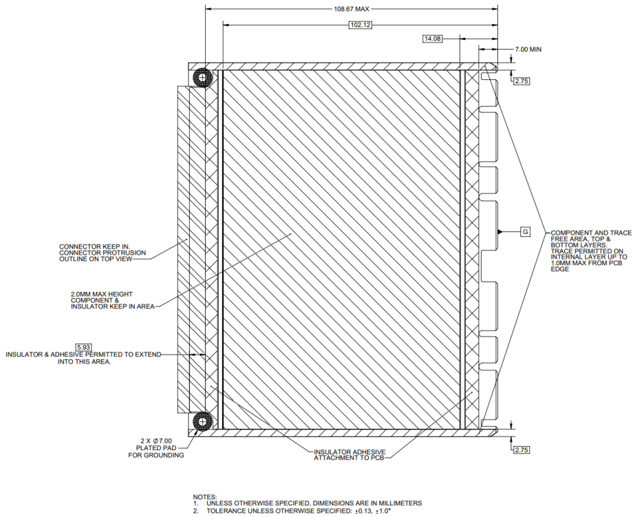
Figure 35: LFF Keep Out Zone – Bottom View
