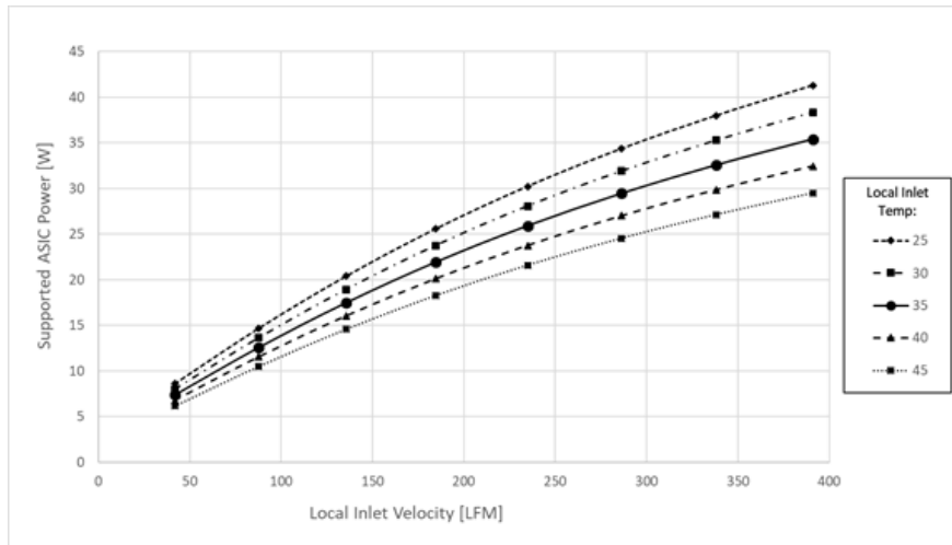
Figure 135: ASIC Supportable Power for Cold Aisle Cooling – SFF Card
