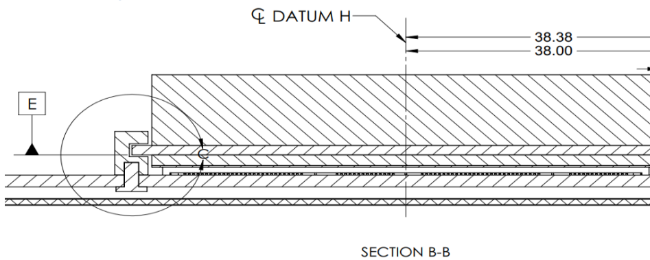
Figure 56: SFF Baseboard Chassis CTF Dimensions (Rear Rail Guide View)
