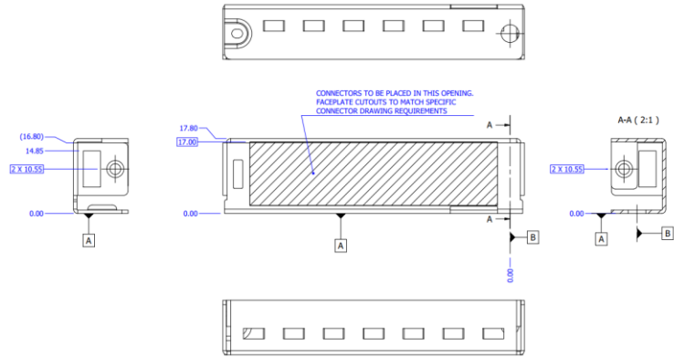
Figure 19: TSFF Generic I/O Faceplate – Ejector Version (2D View)
