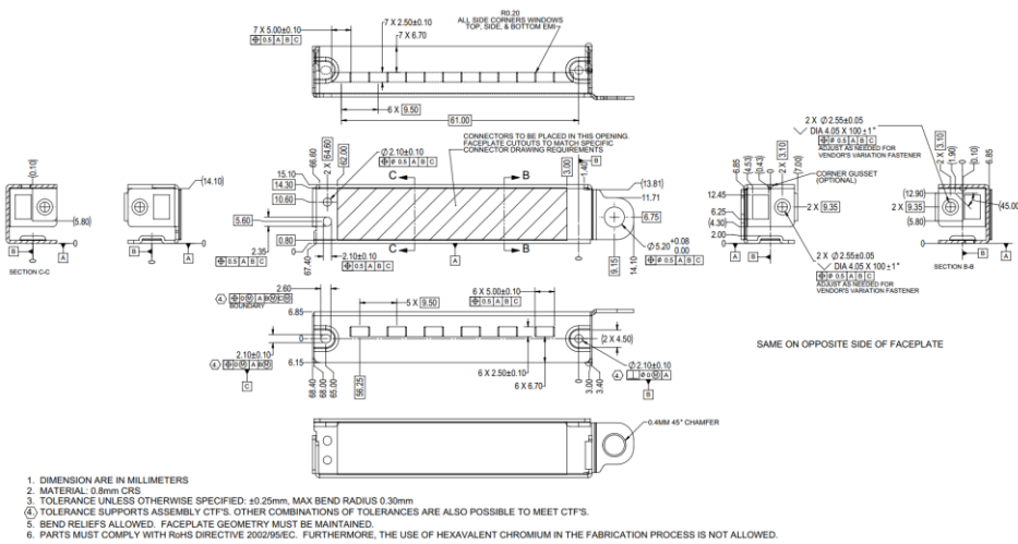
Figure 15: SFF Generic I/O Faceplate – Pull Tab Version (2D View)
