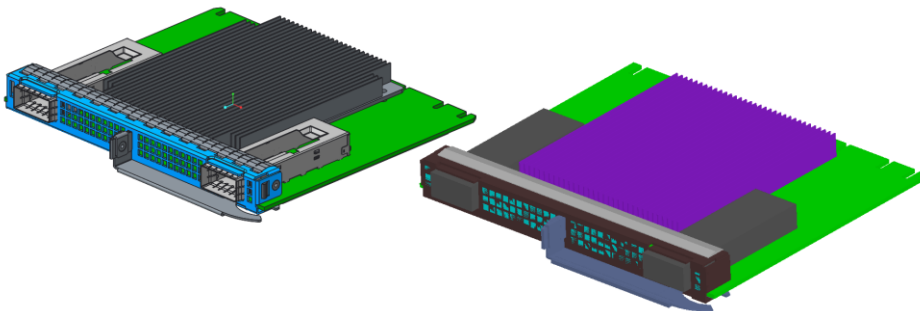
Figure 133: OCP NIC 3.0 LFF Reference Design and CFD Geometry
