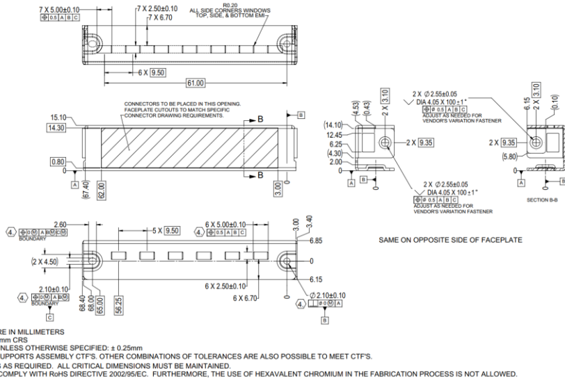
Figure 17: SFF Generic I/O Faceplate – Internal Lock Version (2D View)
