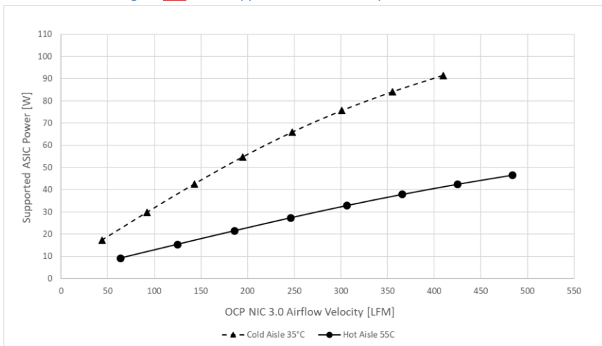
Figure 140: ASIC Supportable Power Comparison – LFF Card
