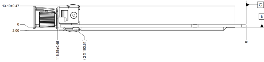
Figure 46: SFF OCP NIC 3.0 Card with Pull Tab CTF Dimensions (Side View)
