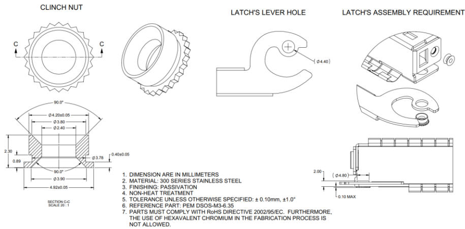
Figure 25: Clinch Nut Option A
