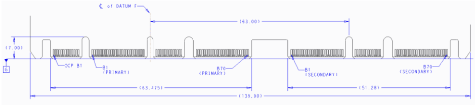
Figure 78: LFF Gold Finger Dimensions – x32 – Top Side (“B” Pins)
