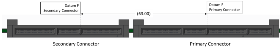
Figure 89: Primary and Secondary Connector Locations for LFF Support with Straddle Mount Connectors
