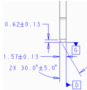
Figure 77: SFF, TSFF Primary Connector Gold Finger - Detail D
