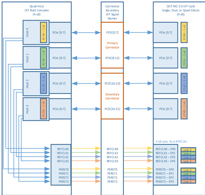
Figure 112: LFF PCIe REFCLK Mapping – Quad Host – 4 Links
