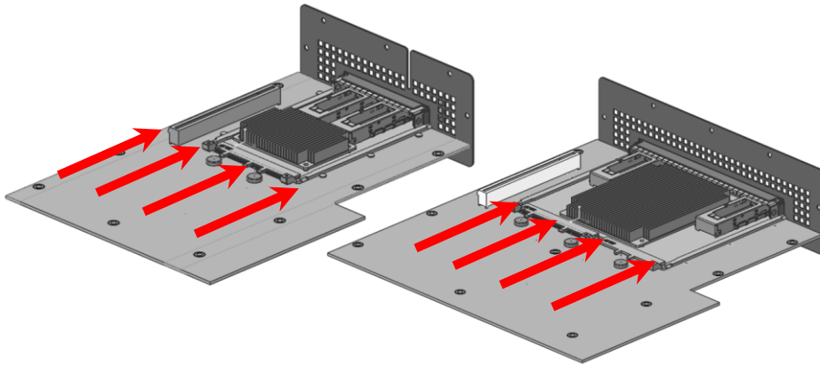
Figure 126: Airflow Direction for Hot Aisle Cooling (SFF/TSFF and LFF)
