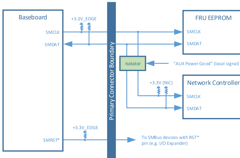
Figure 92: Example SMBus Connections
