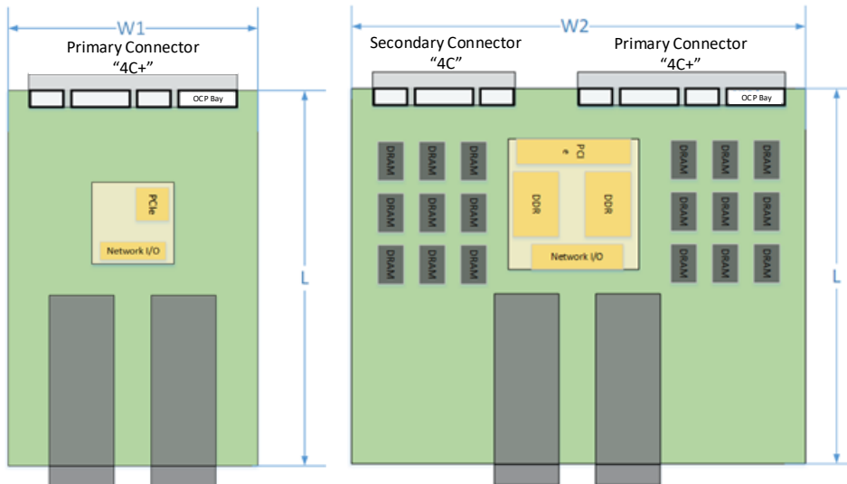
Figure 3: SFF/ TSFF and LFF Block Diagrams (not to scale)
