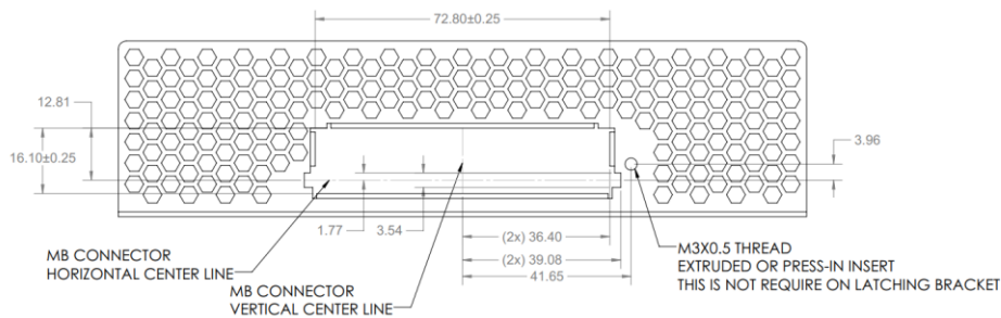
Figure 53: SFF Baseboard Chassis CTF Dimensions (Rear View)
