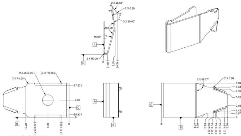
Figure 24: Ejector Lock
