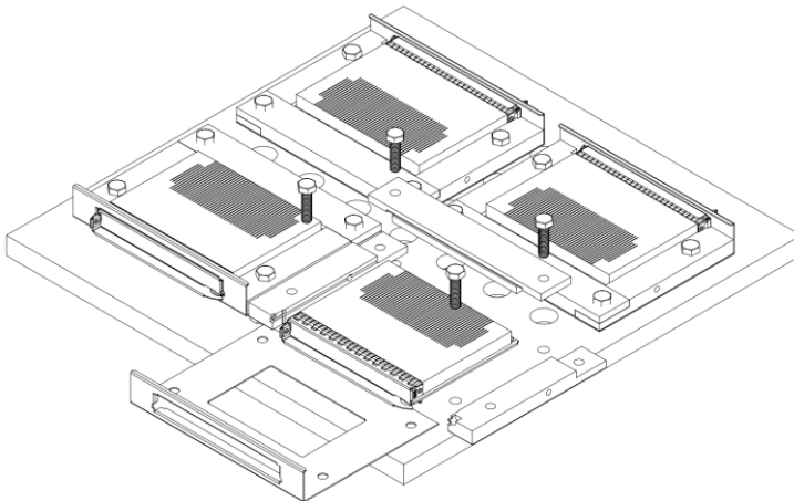
Figure 156: LFF Shock and Vibe Fixture
