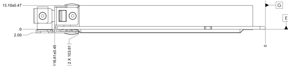
Figure 49: SFF OCP NIC 3.0 Card with Ejector CTF Dimensions (Side View)
