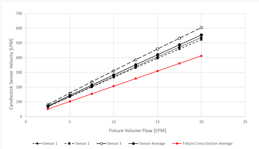
Figure 149: SFF Fixture, Hot Aisle Flow – Candlestick Air Velocity vs. Volume Flow
