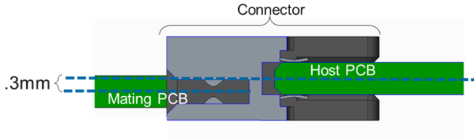
Figure 87: 0.3 mm Offset for 0.076" Thick Baseboards
