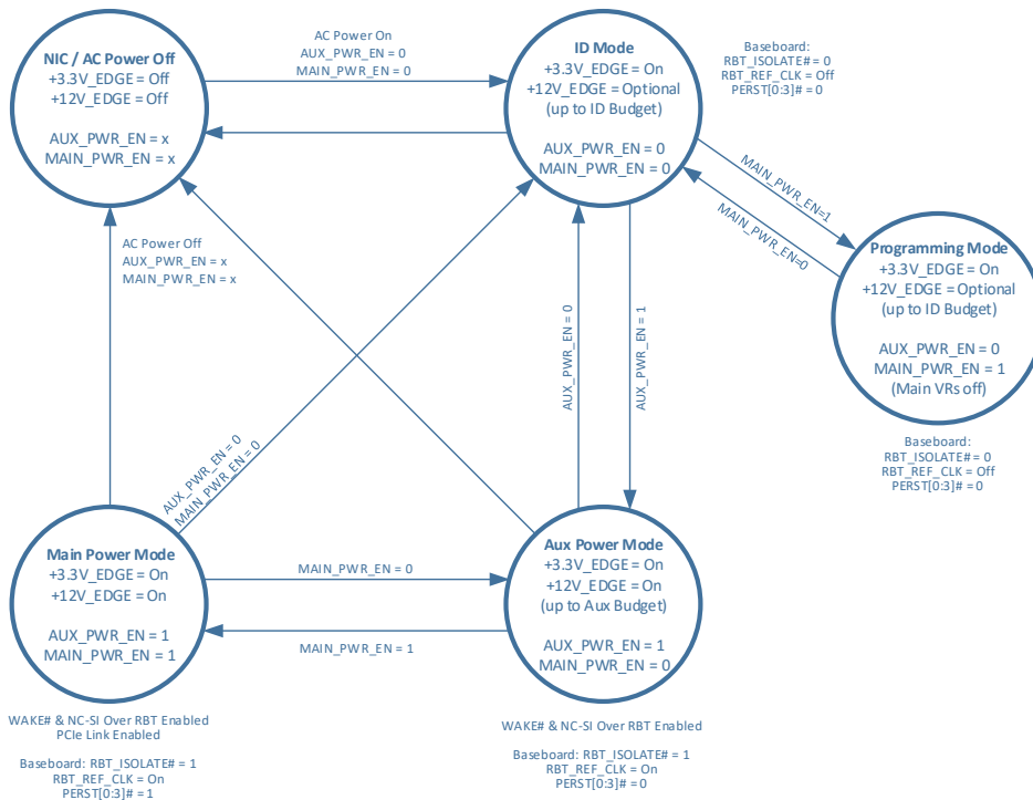
Figure 114: Baseboard Power States
