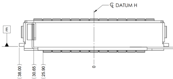
Figure 48: SFF OCP NIC 3.0 Card with Ejector CTF Dimensions (Front View)
