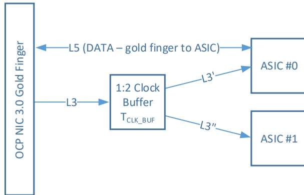
Figure 123: NC-SI over RBT Propagation Delay Matching for Two Target ASICs – Clock Buffer
