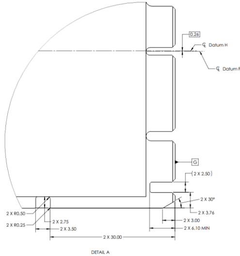
Figure 28: SFF Keep Out Zone – Top View – Detail A
