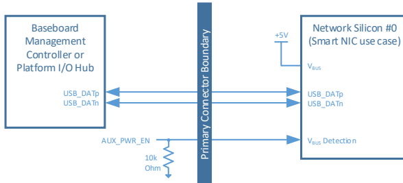
Figure 99: USB 2.0 Connection Example – Basic Connectivity
