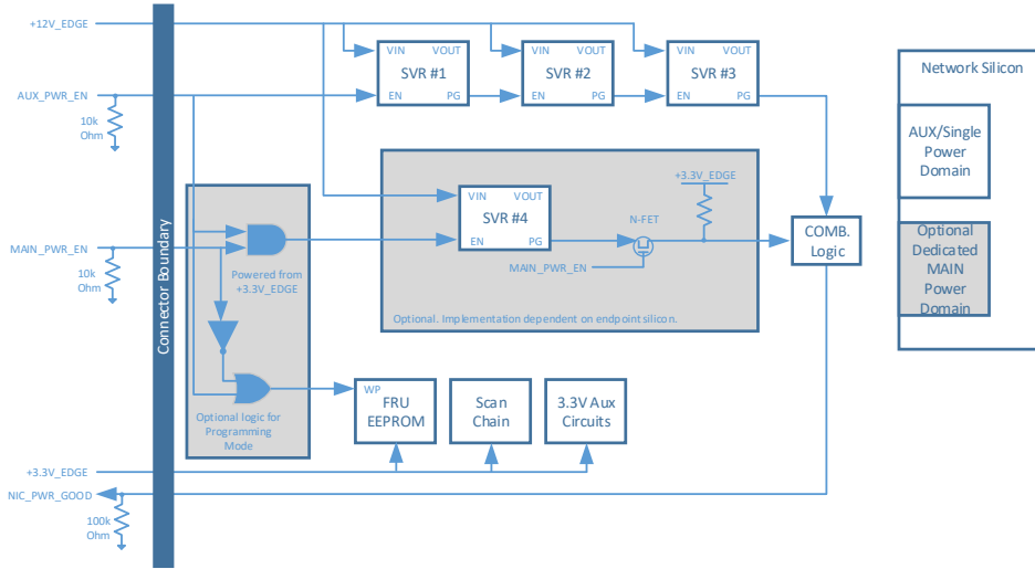
Figure 98: Example Power Supply Topology
