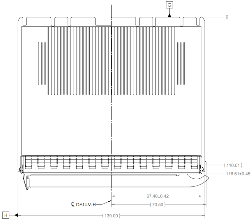
Figure 62: LFF OCP NIC 3.0 Card with Ejector Latch CTF Dimensions (Top View)
