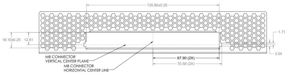
Figure 65: LFF Baseboard Chassis CTF Dimensions (Rear View)
