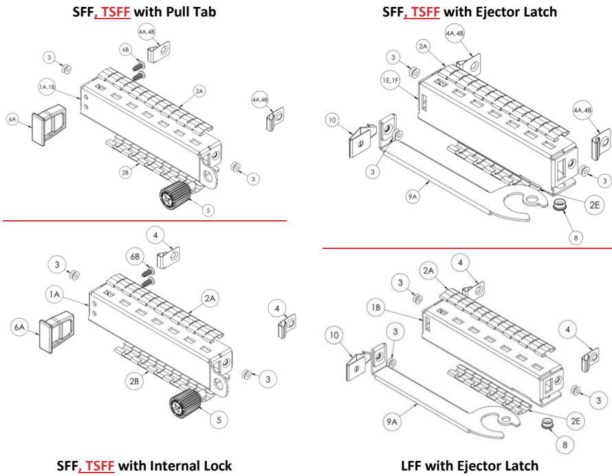
Figure 14: Faceplate Assembly Exploded Views (SFF, TSFF and LFF)
