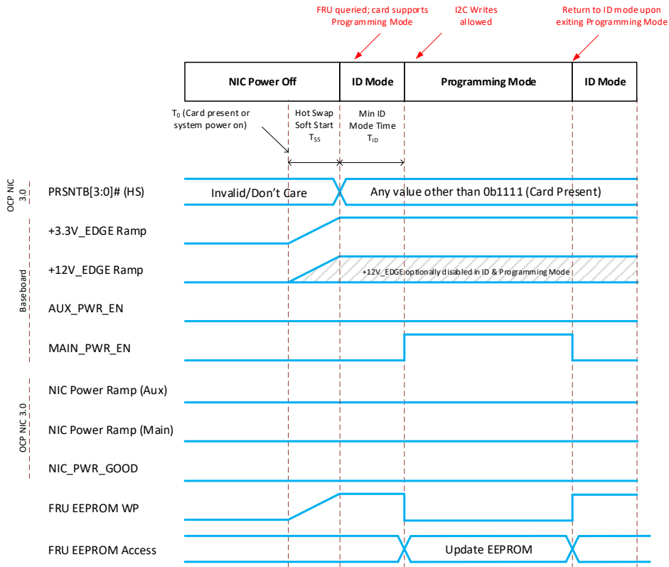
Figure 117: Programming Mode Sequencing
