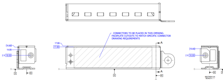
Figure 18: TSFF Generic I/O Faceplate – Pull Tab Version (2D View)
