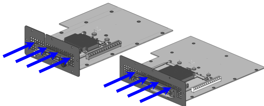
Figure 127 149: Airflow Direction for Cold Aisle Cooling (SFF/TSFF and LFF)
