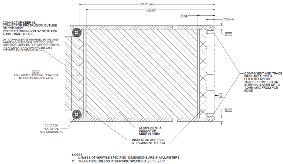
Figure 29: SFF Keep Out Zone – Bottom View
