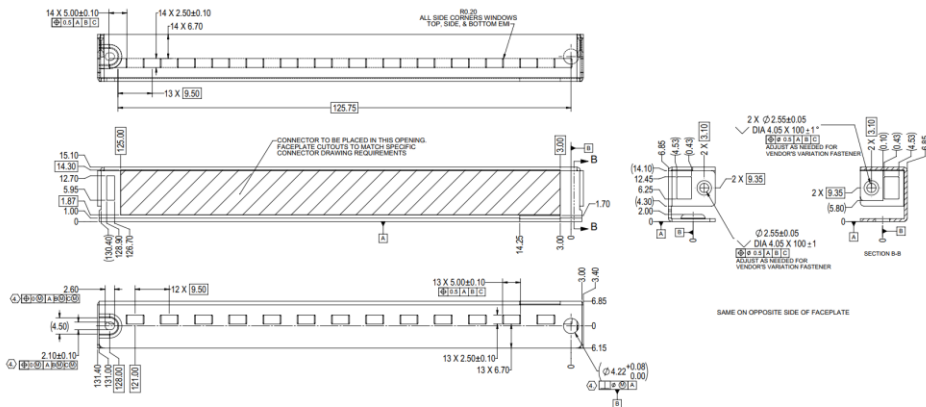
Figure 21: LFF Generic I/O Faceplate – Ejector Version (2D View)
