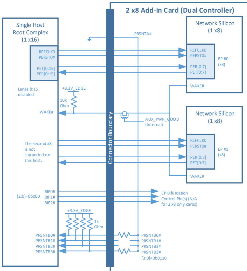
Figure 106: Single Host with no Bifurcation (1 x16) and 2 x8 OCP NIC 3.0 Card (Dual Controllers)
