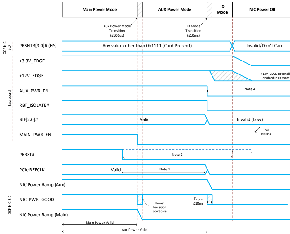
Figure 116: Power-Down Sequencing – Normal Operation
