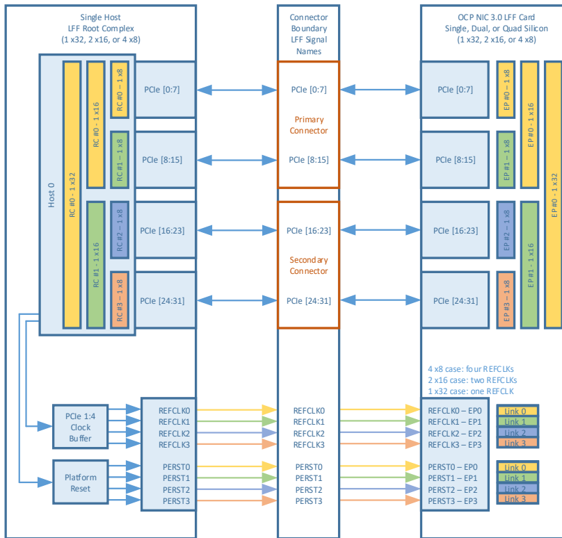
Figure 110: LFF PCIe REFCLK Mapping – Single Host – 1, 2 and 4 links
