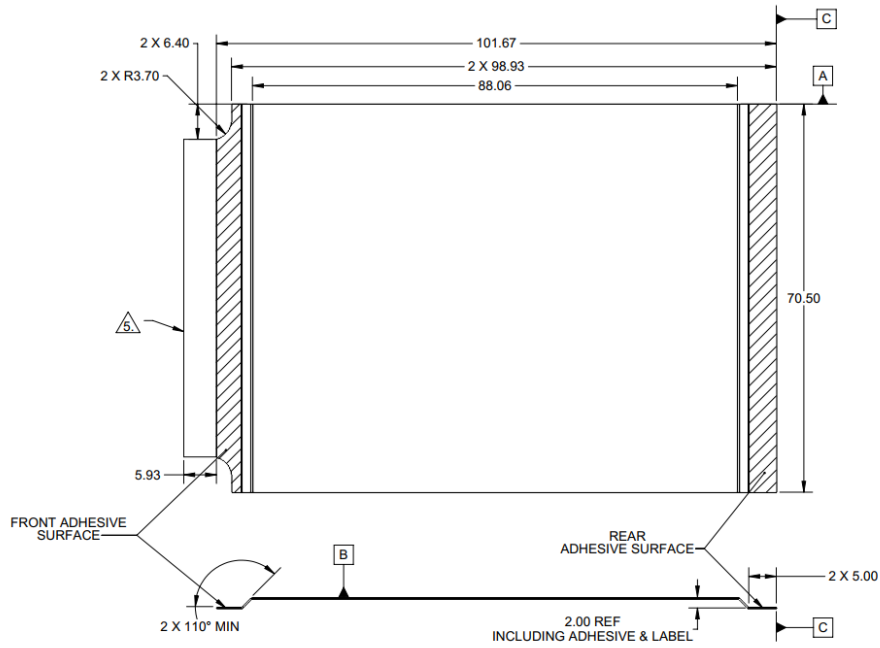
Figure 39: SFF, TSFF Bottom Side Insulator (Top and Side View)
