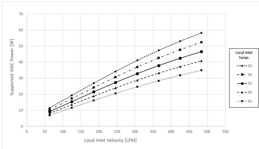
Figure 132: ASIC Supportable Power for Hot Aisle Cooling – LFF Card
