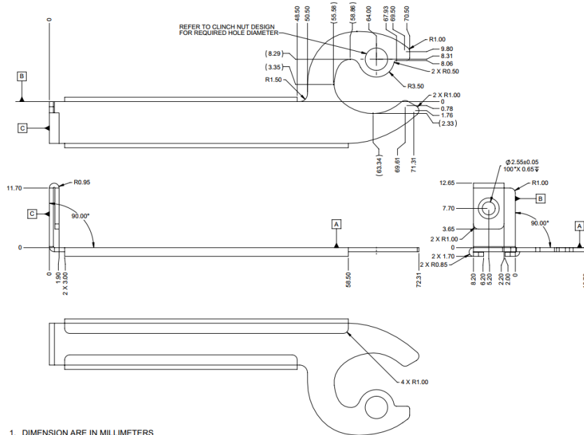
Figure 22: SFF I/O Faceplate – Ejector Lever (2D View)
