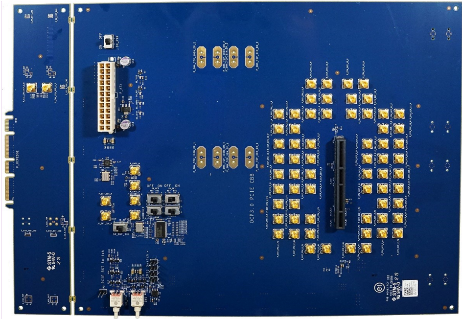
Figure 125: PCIe Base Board Test Fixture for OCP NIC 3.0 SFF/TSFF
