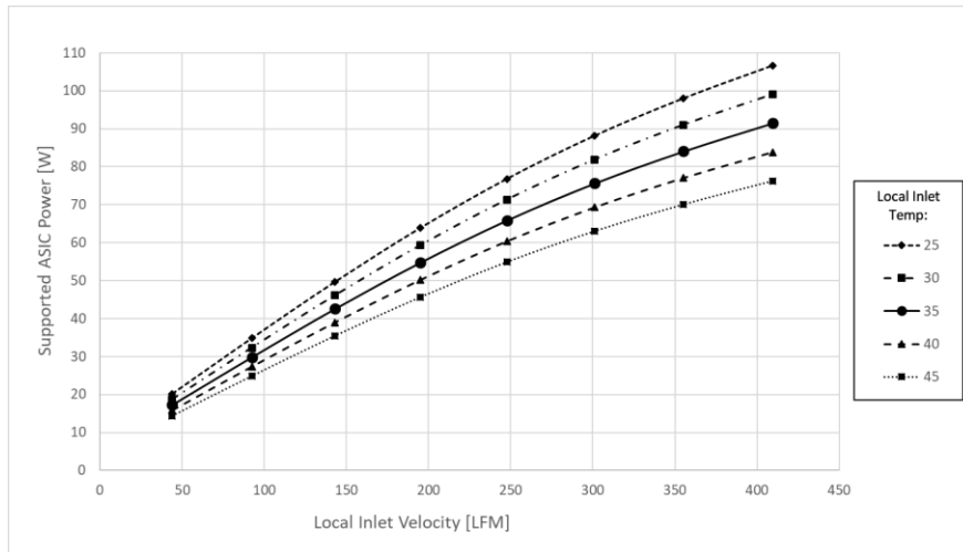
Figure 138: ASIC Supportable Power for Cold Aisle Cooling – LFF Card
