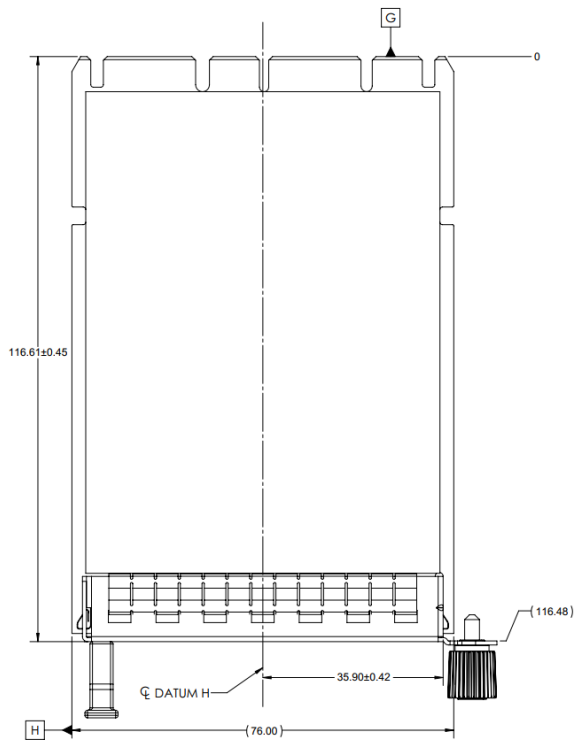
Figure 44: SFF OCP NIC 3.0 Card with Pull Tab CTF Dimensions (Top View)
