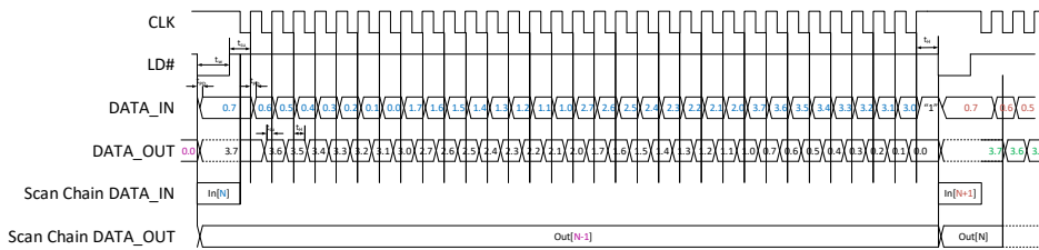
Figure 96: Scan Chain Timing Diagram Example 2
