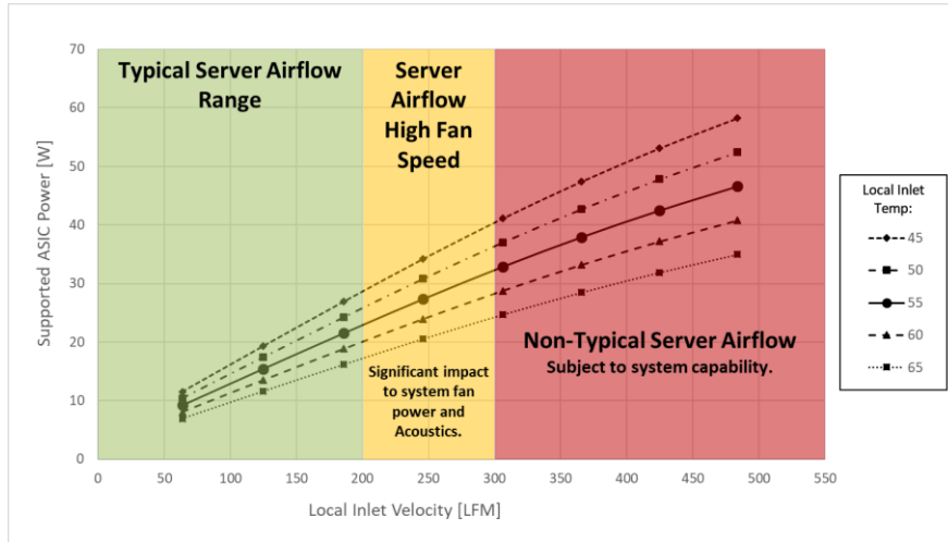
Figure 134: Server System Airflow Capability – LFF Card Hot Aisle Cooling
