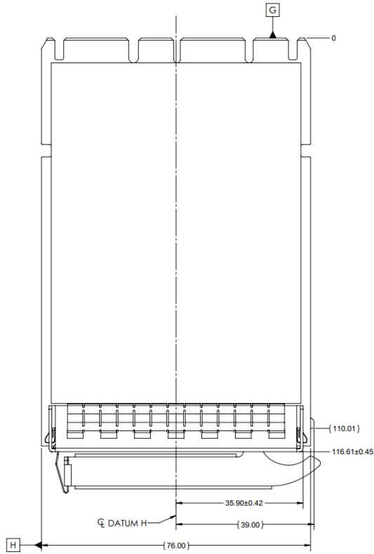
Figure 48: SFF OCP NIC 3.0 Card with Ejector CTF Dimensions (Front View)
