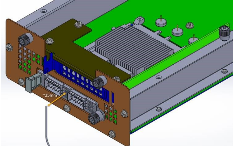
Figure 148: External Thermocouple Placement for Cold Aisle Inlet Temperature Measurement
