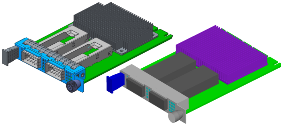
Figure 129: OCP NIC 3.0 SFF Reference Design and CFD Geometry
