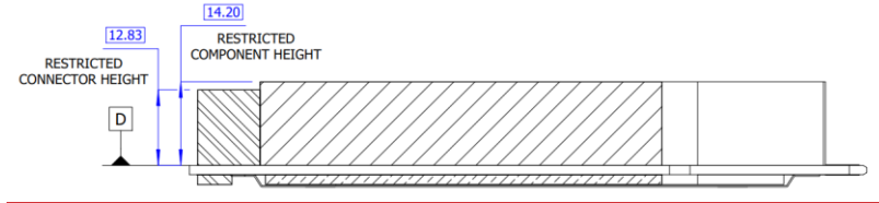
Figure 32: TSFF Keep Out Zone – Side View
