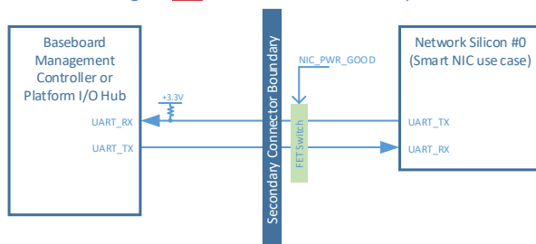
Figure 101: UART Connection Example
