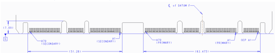
Figure 79: LFF Gold Finger Dimensions – x32 – Bottom Side (“A” Pins)
