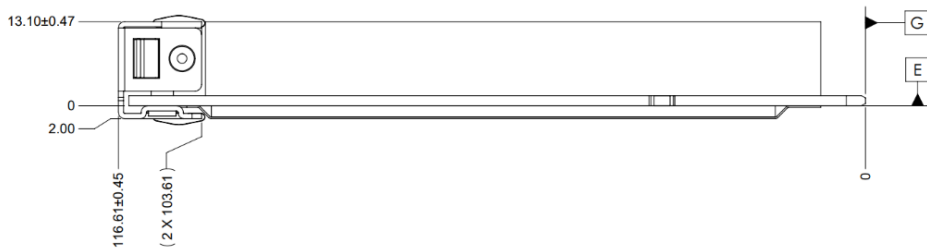
Figure 52: SFF OCP NIC 3.0 Card with Internal Lock CTF Dimensions (Side View)
