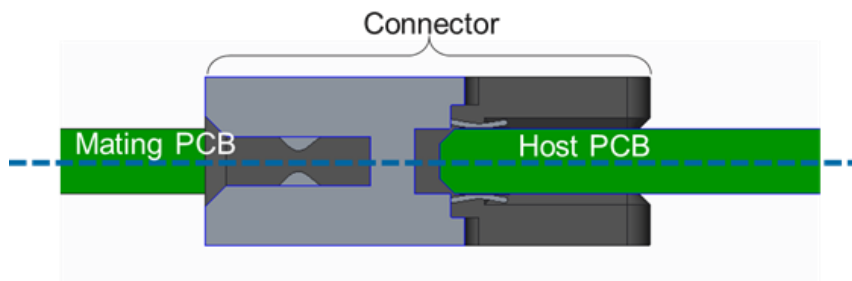
Figure 86: 0 mm Offset (Coplanar) for 0.062" Thick Baseboards
