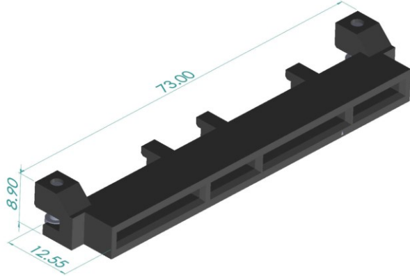
Figure 84: 140-pin Base Board Secondary Connector – Straddle Mount
