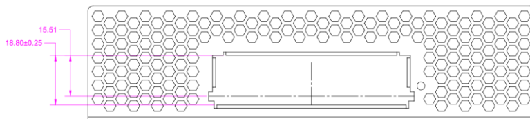
Figure 61: TSFF Baseboard Chassis CTF Dimensions (Rear View)
