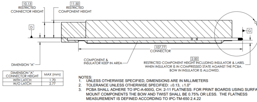
Figure 30: SFF Keep Out Zone – Side View
