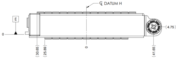
Figure 45: SFF OCP NIC 3.0 Card with Pull Tab CTF Dimensions (Front View)
