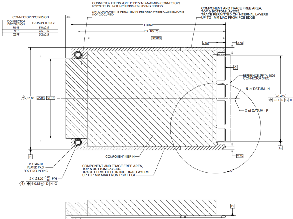
Figure 27: SFF Keep Out Zone – Top View
