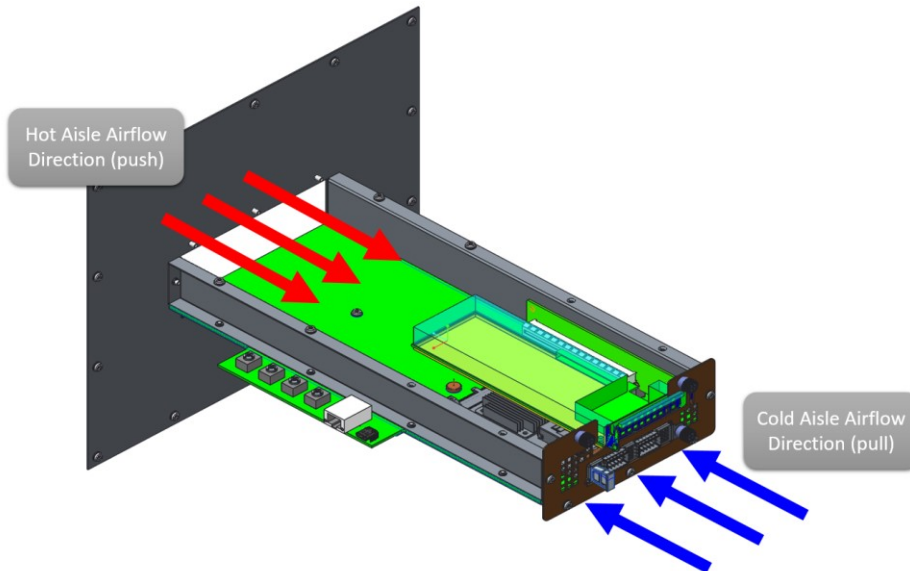
Figure 147: Thermal Test Fixture Airflow Direction
