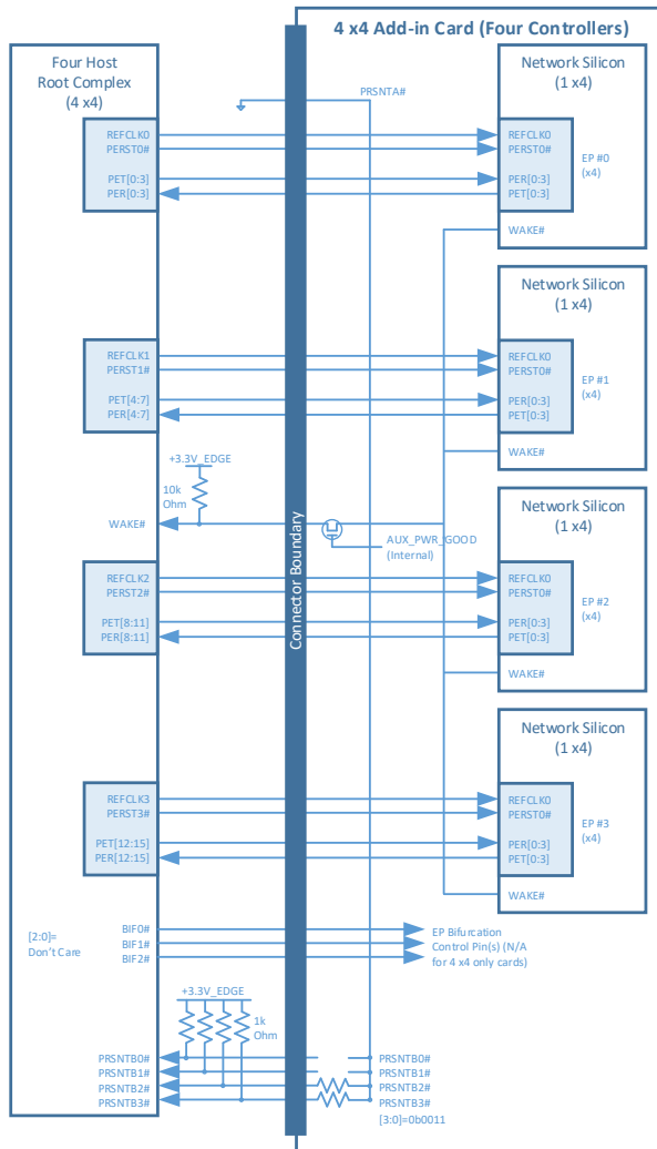
Figure 105: Quad Hosts (4 x4) and 4 x4 OCP NIC 3.0 Card (Quad Controllers)
