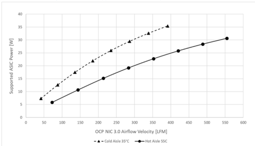
Figure 137: ASIC Supportable Power Comparison – SFF Card
