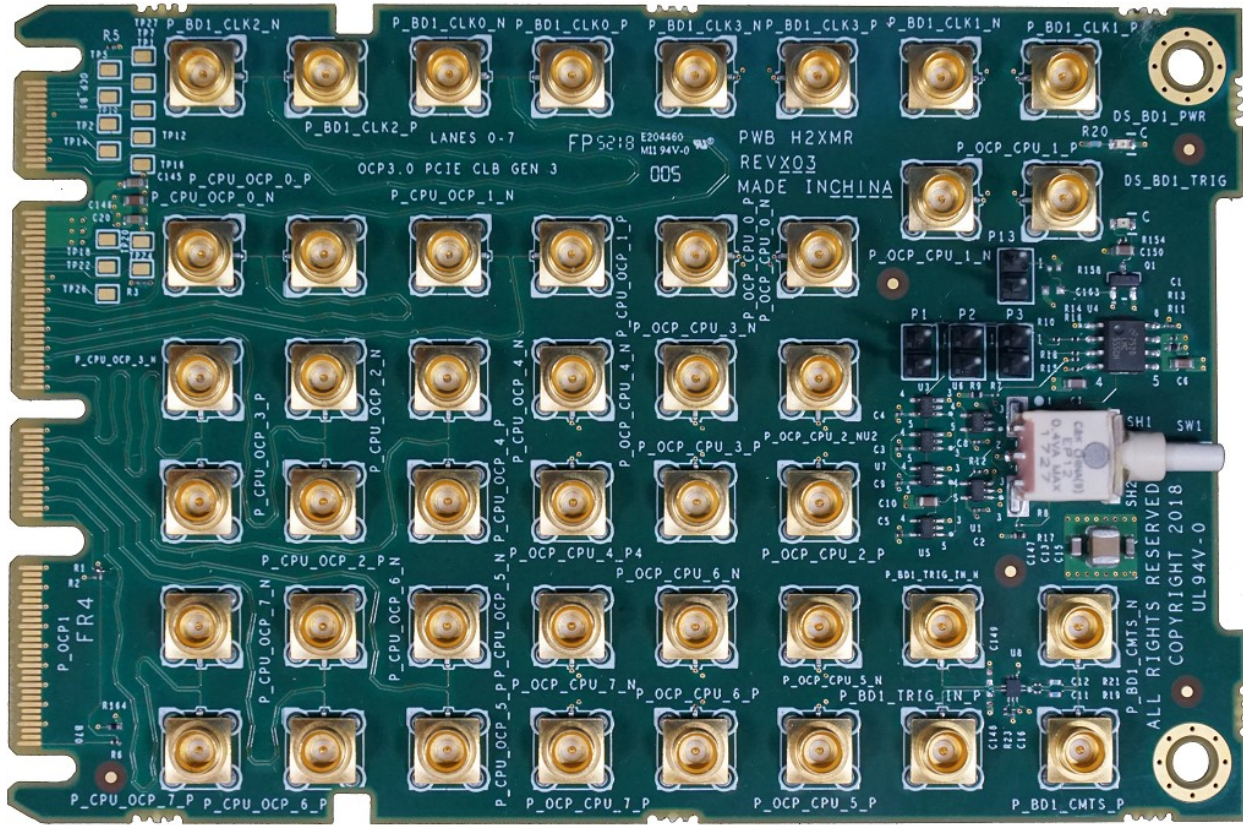
Figure 116: PCIe Load Board Test Fixture for OCP NIC 3.0 SFF
