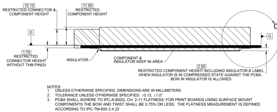
Figure 32: LFF Keep Out Zone – Side View
