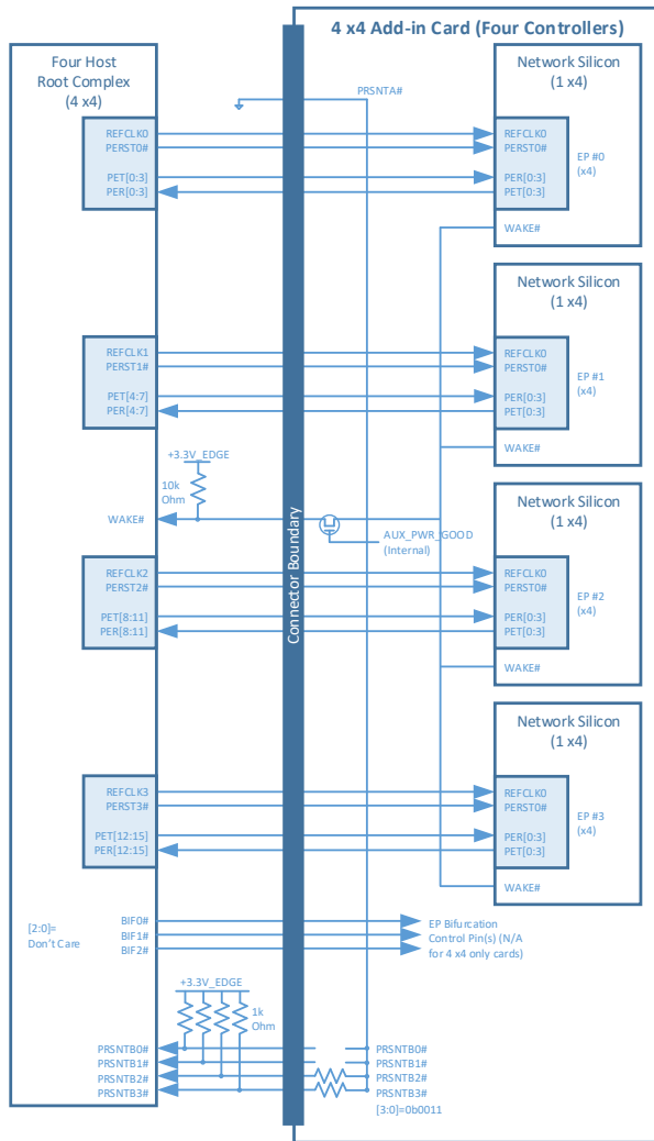
Figure 9796: Quad Hosts (4 x4) and 4 x4 OCP NIC 3.0 Card (Quad Controllers)
