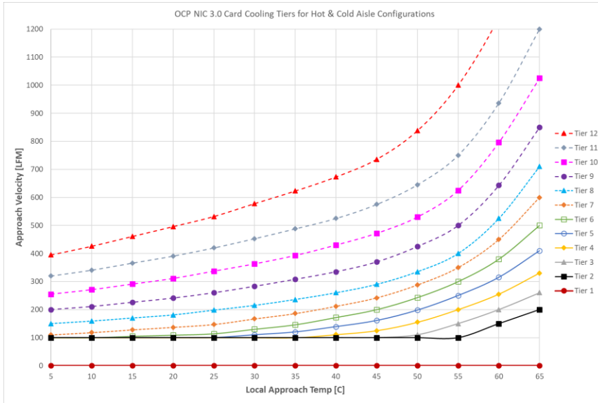
Figure 144142: Typical Operating Range for Hot Aisle Configurations
