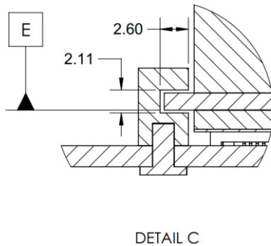
Figure 53: SFF Baseboard Chassis CTF Dimensions (Rail Guide Detail) – Detail C
