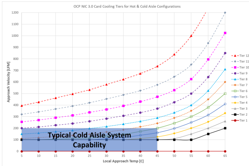
Figure 145143: Typical Operating Range for Cold Aisle Configurations
