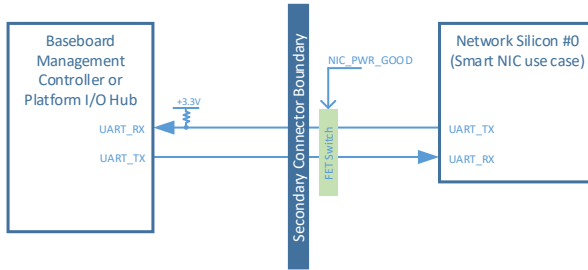
Figure 9392 : UART Connection Example
