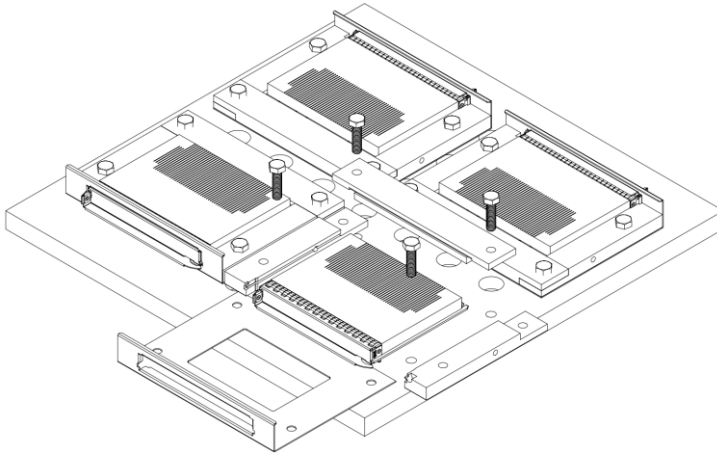
Figure 147145 : LFF Shock and Vibe Fixture
