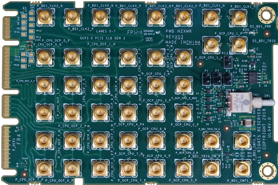
Figure 116445: PCIe Load Board Test Fixture for OCP NIC 3.0 SFF
