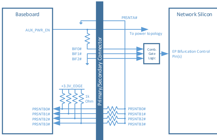
Figure 83: PCIe Present and Bifurcation Control Pins (Static BIF[2:0-2]#)
