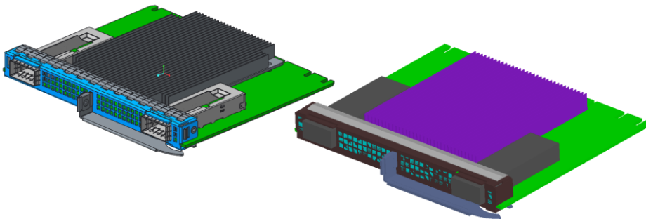
Figure 125124: OCP NIC 3.0 LFF Reference Design and CFD Geometry
