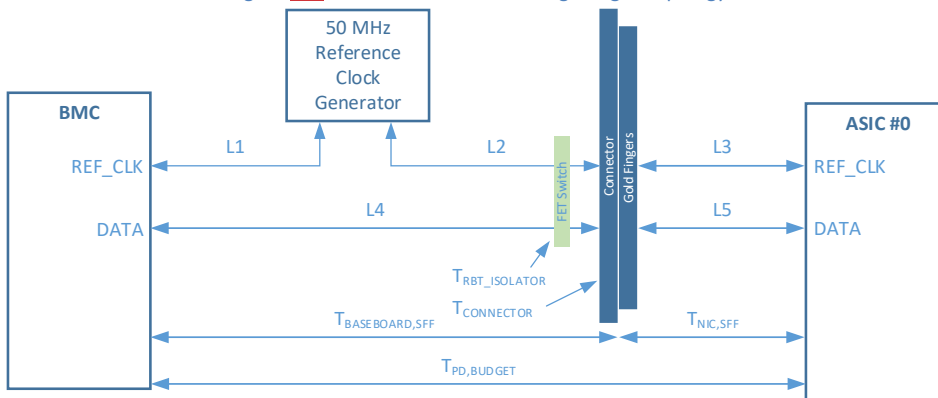
Figure 113442: NC-SI over RBT Timing Budget Topology
