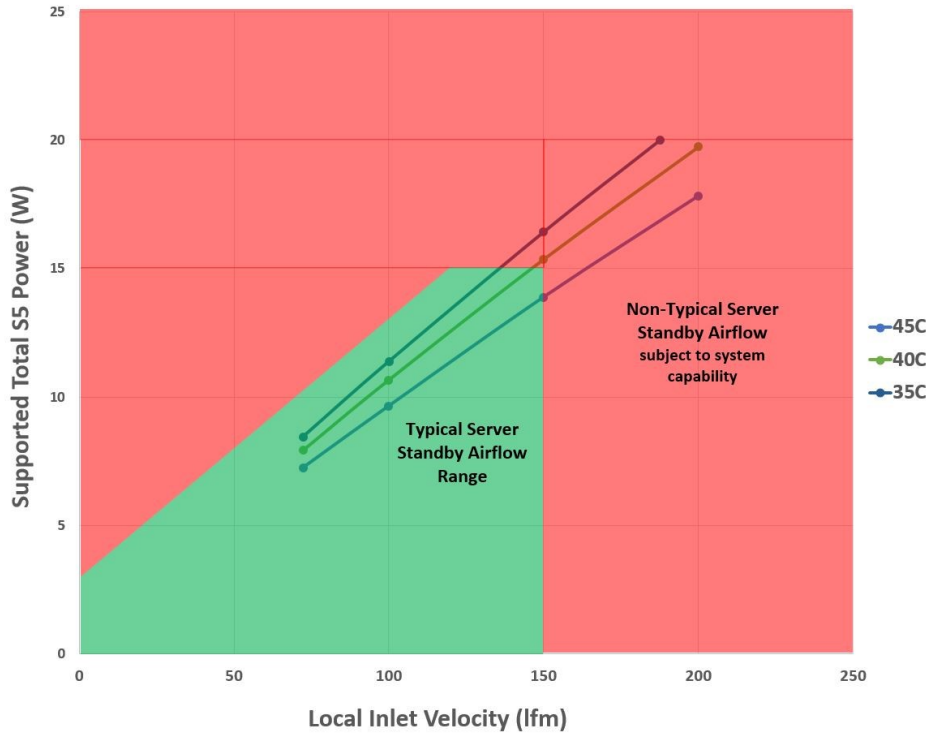
Figure 123122 : Server System Airflow Capability – SFF Card Hot Aisle Cooling in standby (S5) Aux Power mode
