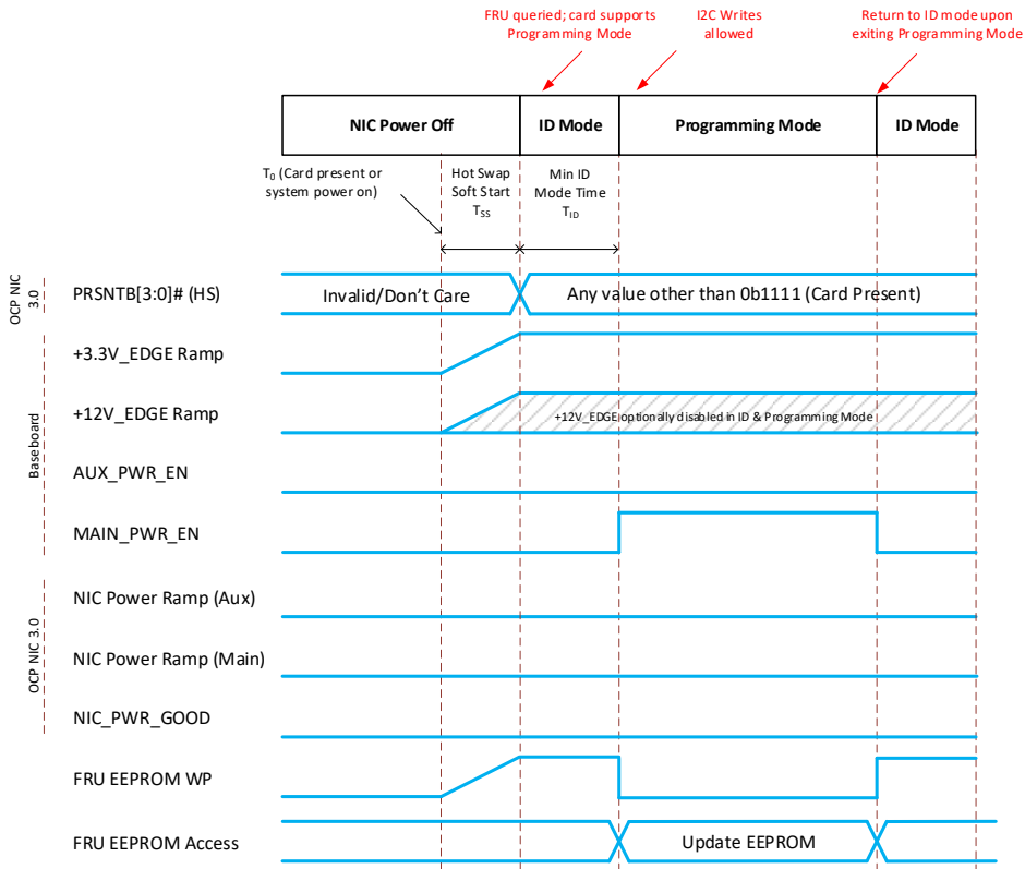
Figure 109108: Programming Mode Sequencing
