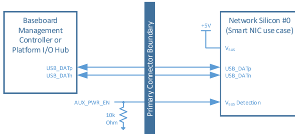
Figure 9199: USB 2.0 Connection Example – Basic Connectivity
