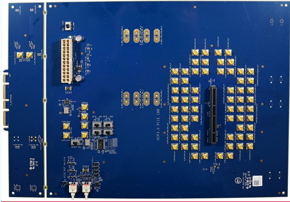
Figure 117416: PCIe Base Board Test Fixture for OCP NIC 3.0 SFF
