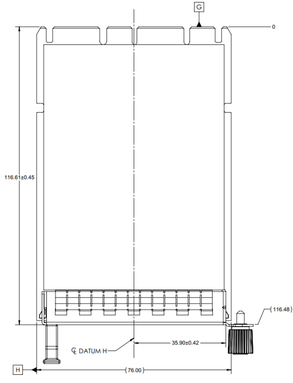
Figure 41: SFF OCP NIC 3.0 Card with Pull Tab CTF Dimensions (Front View)
