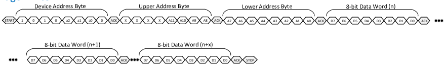
Figure 111440: FRU EEPROM Reads with Double Byte Addressing
