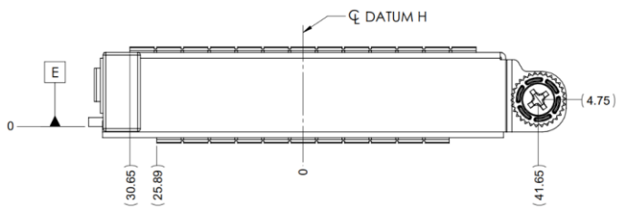
Figure 42: SFF OCP NIC 3.0 Card with Pull Tab CTF Dimensions (Side View)
