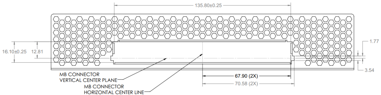
Figure 57: LFF Baseboard Chassis CTF Dimensions (Rear View)
