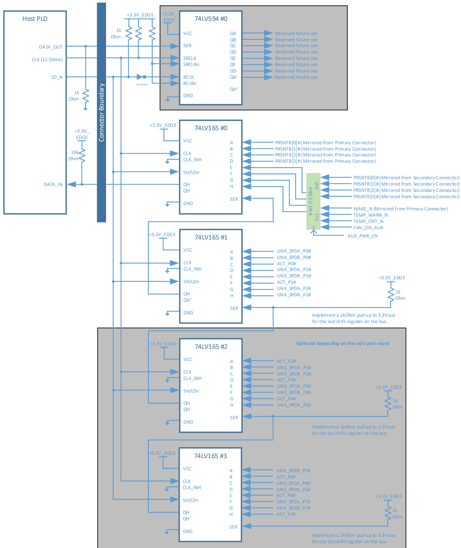
Figure 8988: Scan Chain Connection Example
