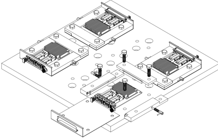
Figure 146145 : LFF Shock and Vibe Fixture
