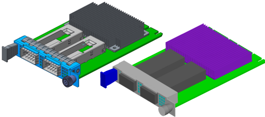
Figure 121420: OCP NIC 3.0 SFF Reference Design and CFD Geometry
