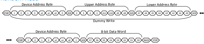
Figure 111440: FRU EEPROM Reads with Double Byte Addressing
