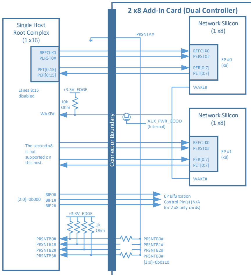
Figure 9897: Single Host with no Bifurcation (1 x16) and 2 x8 OCP NIC 3.0 Card (Dual Controllers)
