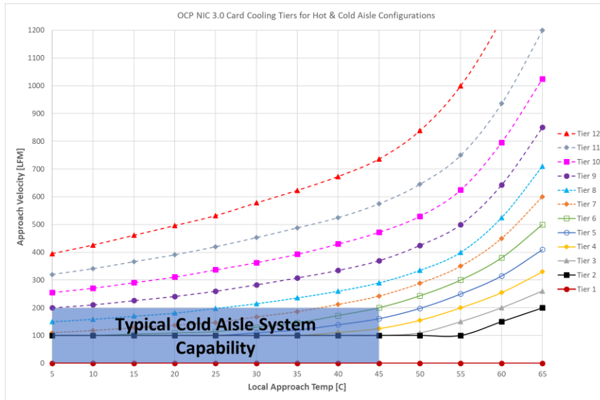
Figure 144143: Typical Operating Range for Cold Aisle Configurations
