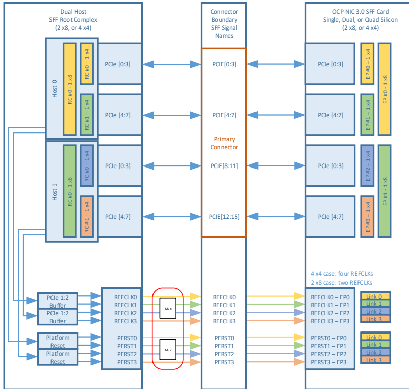
Figure 10099: SFF PCIe REFCLK Mapping – Dual Host – 2 and 4 links
