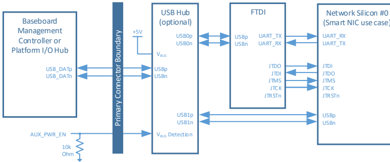
Figure 9294: USB 2.0 Connection Example – USB-Serial / USB-JTAG Connectivity
