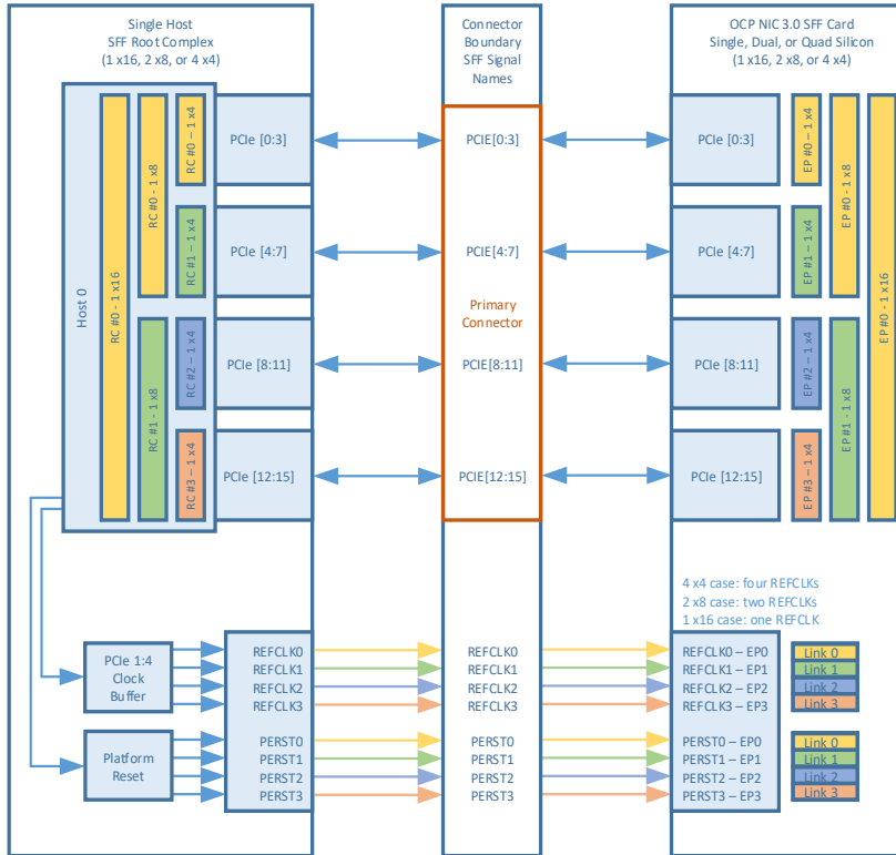
Figure 9998: SFF PCIe REFCLK Mapping – Single Host – 1, 2 and 4 links
