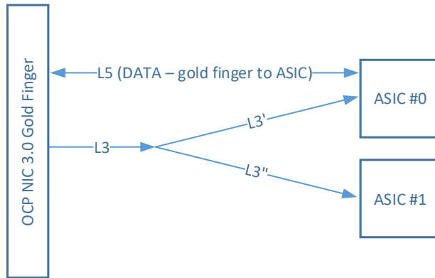
Figure 114113: NC-SI over RBT Propagation Delay Matching for Two Target ASICs – No Clock Buffer
