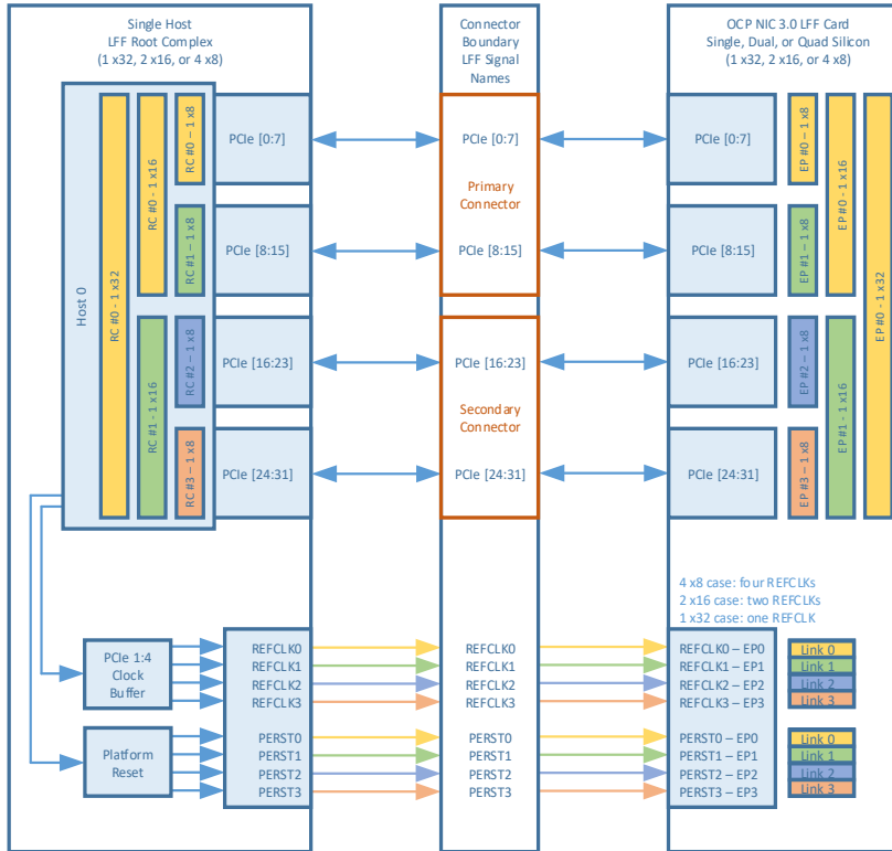
Figure 102401: LFF PCIe REFCLK Mapping – Single Host – 1, 2 and 4 links
