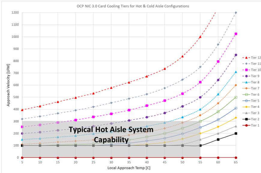
Figure 143142: Typical Operating Range for Hot Aisle Configurations
