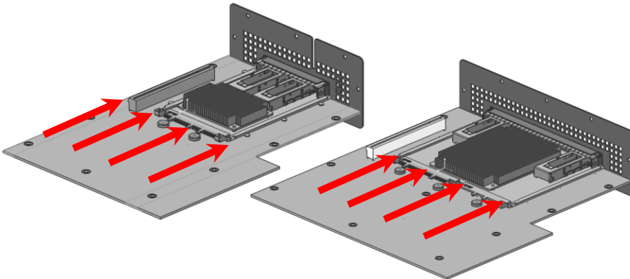
Figure 118117: Airflow Direction for Hot Aisle Cooling (SFF and LFF)
