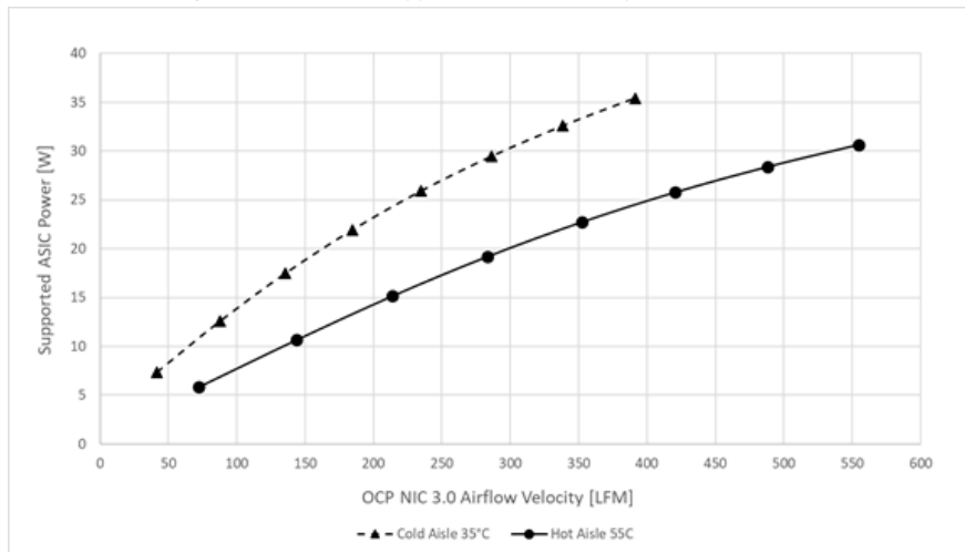
Figure 129128: ASIC Supportable Power Comparison – SFF Card
