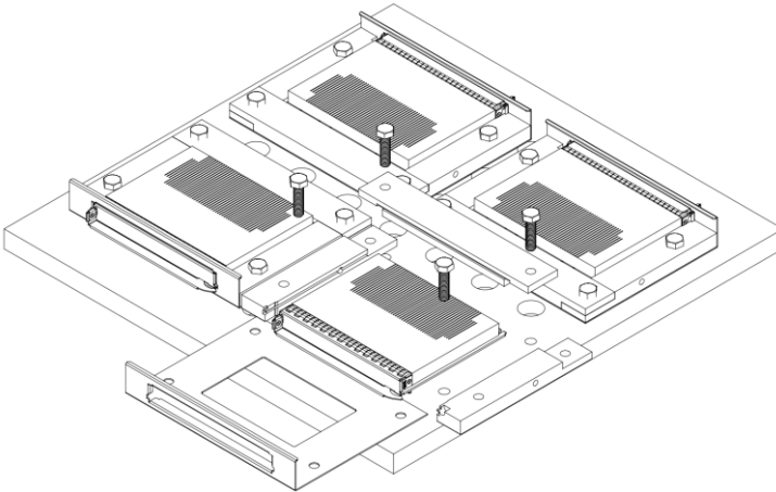
Figure 146145 : LFF Shock and Vibe Fixture
