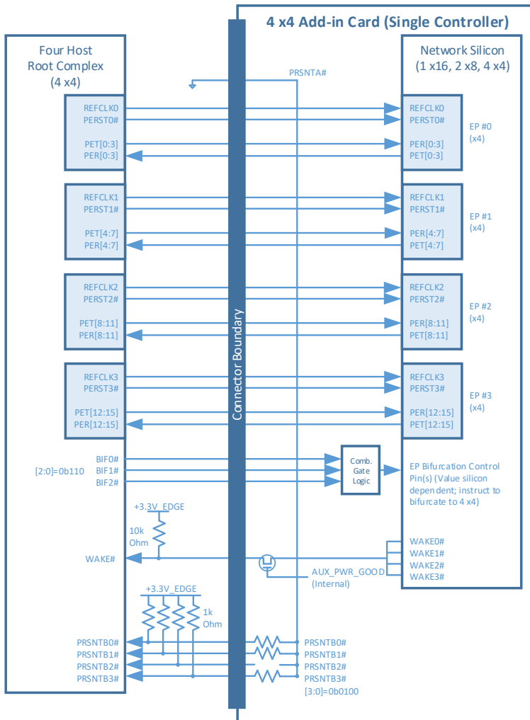
Figure 9695: Quad Hosts (4 x4) and 4 x4 OCP NIC 3.0 Card (Single Controller)
