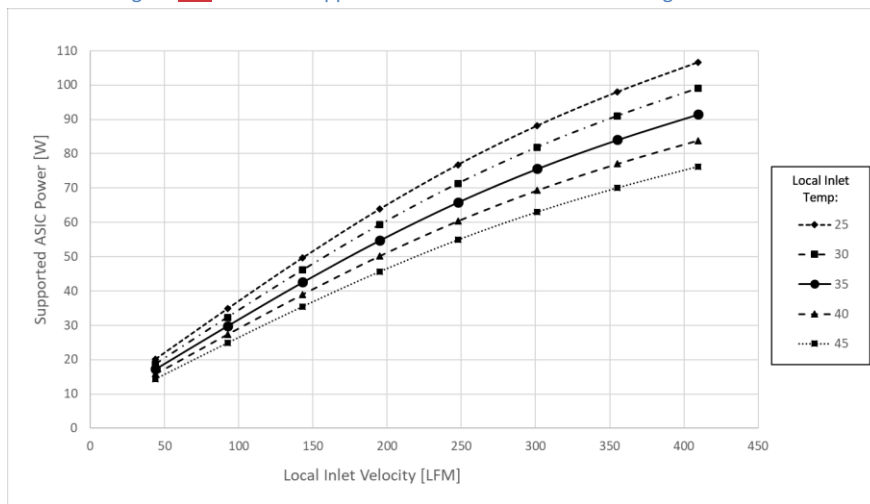
Figure 130129: ASIC Supportable Power for Cold Aisle Cooling – LFF Card
