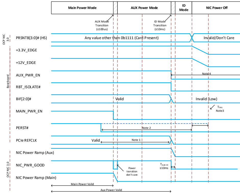
Figure 108107: Power-Down Sequencing – Normal Operation
