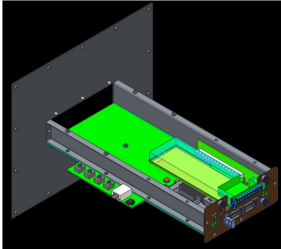
Figure 134133 : SFF Thermal Test Fixture Preliminary Design – Cover Removed
