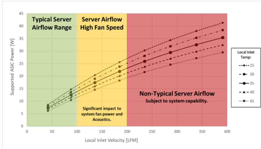
Figure 128127: Server System Airflow Capability – SFF Cold Aisle Cooling
