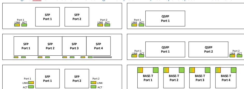
Figure 105-104: Port and LED Ordering – Example SFF Link/Activity and Speed LED Placement
