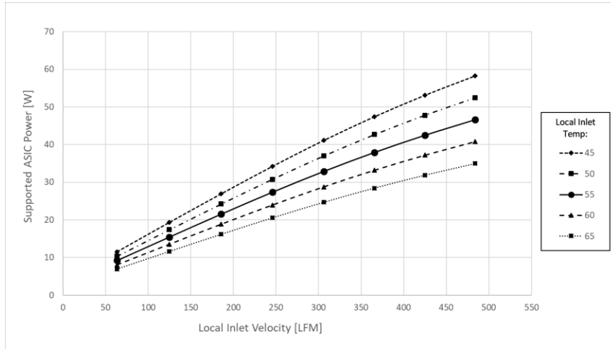
Figure 124123: ASIC Supportable Power for Hot Aisle Cooling – LFF Card
