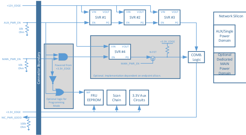
Figure 9089: Example Power Supply Topology
