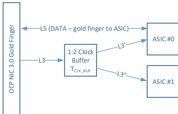
Figure 115114: NC-SI over RBT Propagation Delay Matching for Two Target ASICs – Clock Buffer
