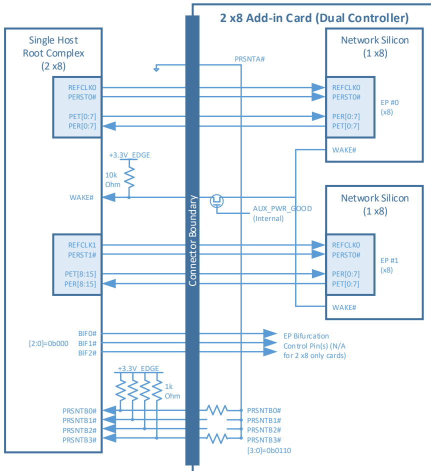
Figure 9594: Single Host (2 x8) and 2 x8 OCP NIC 3.0 Card (Dual Controllers)
