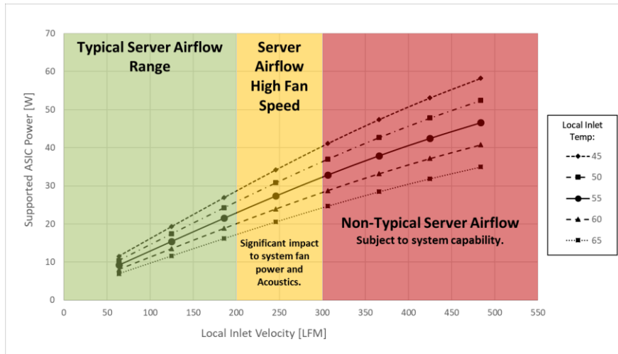
Figure 126125: Server System Airflow Capability – LFF Card Hot Aisle Cooling
