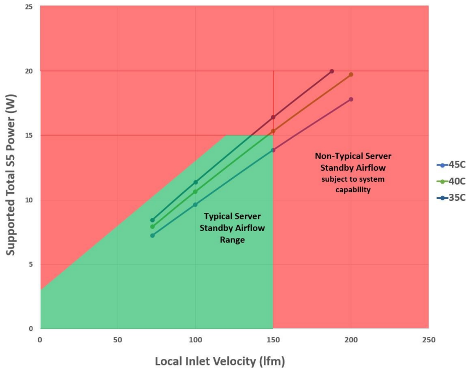
Figure 123422: Server System Airflow Capability – SFF Card Hot Aisle Cooling in standby (S5) mode
