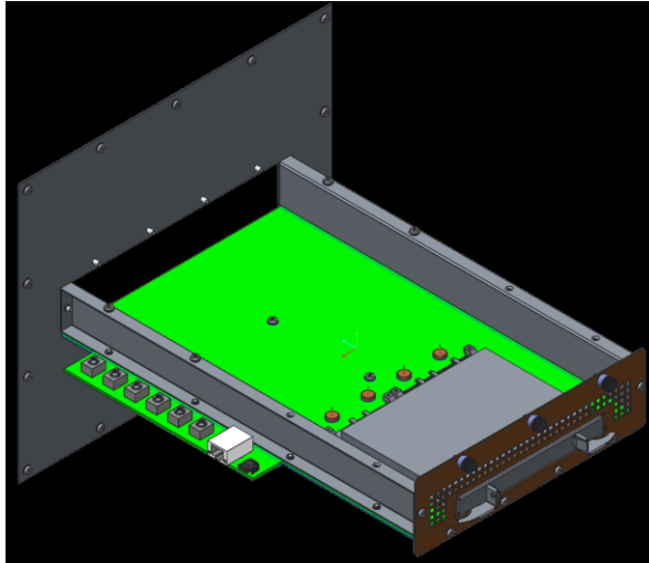
Figure 137 136 : LFF Card Thermal Test Fixture Design – Cover Removed
