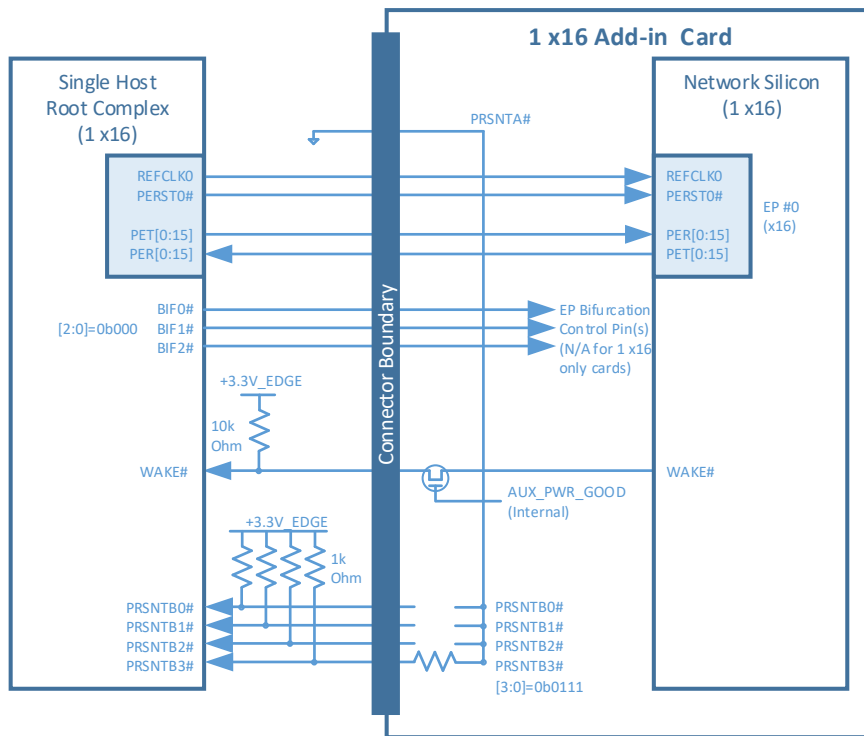
Figure 9493: Single Host (1 x16) and 1 x16 OCP NIC 3.0 Card (Single Controller)
