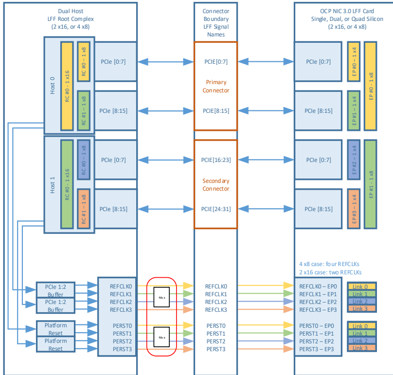
Figure 103402: LFF PCIe REFCLK Mapping – Dual Host – 2 and 4 links
