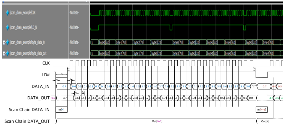
Figure 87: Example Scan Chain Timing Diagram Example 1
