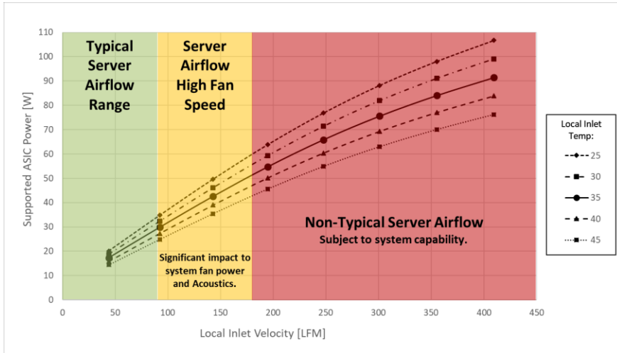
Figure 131430: Server System Airflow Capability – LFF Cold Aisle Cooling
