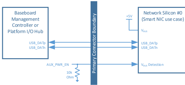
Figure 9199: USB 2.0 Connection Example – Basic Connectivity
