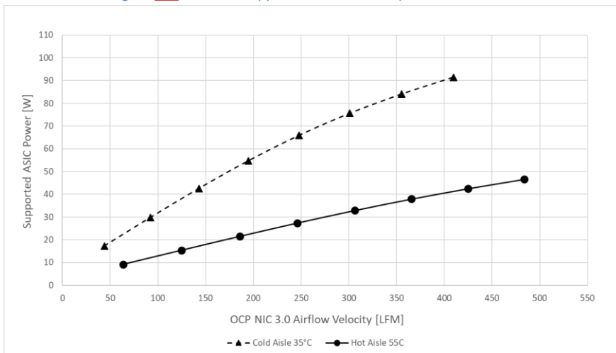
Figure 132131: ASIC Supportable Power Comparison – LFF Card
