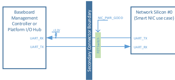
Figure 9392: UART Connection Example
