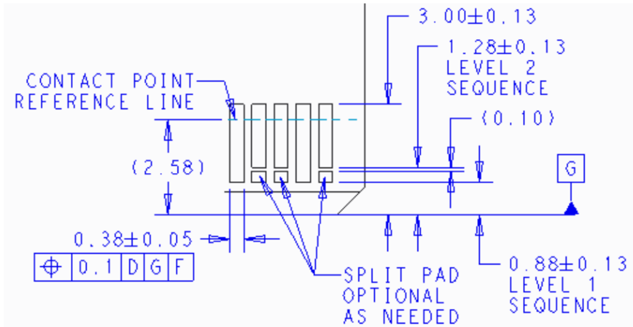
Figure 69: SFF Primary Conector Gold Finger - Detail D
