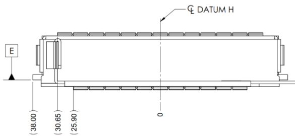
Figure 44: SFF OCP NIC 3.0 Card with Ejector CTF Dimensions (Front View)
