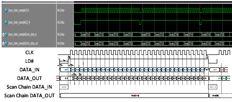
Figure 88: Scan Chain Timing Diagram Example 2
