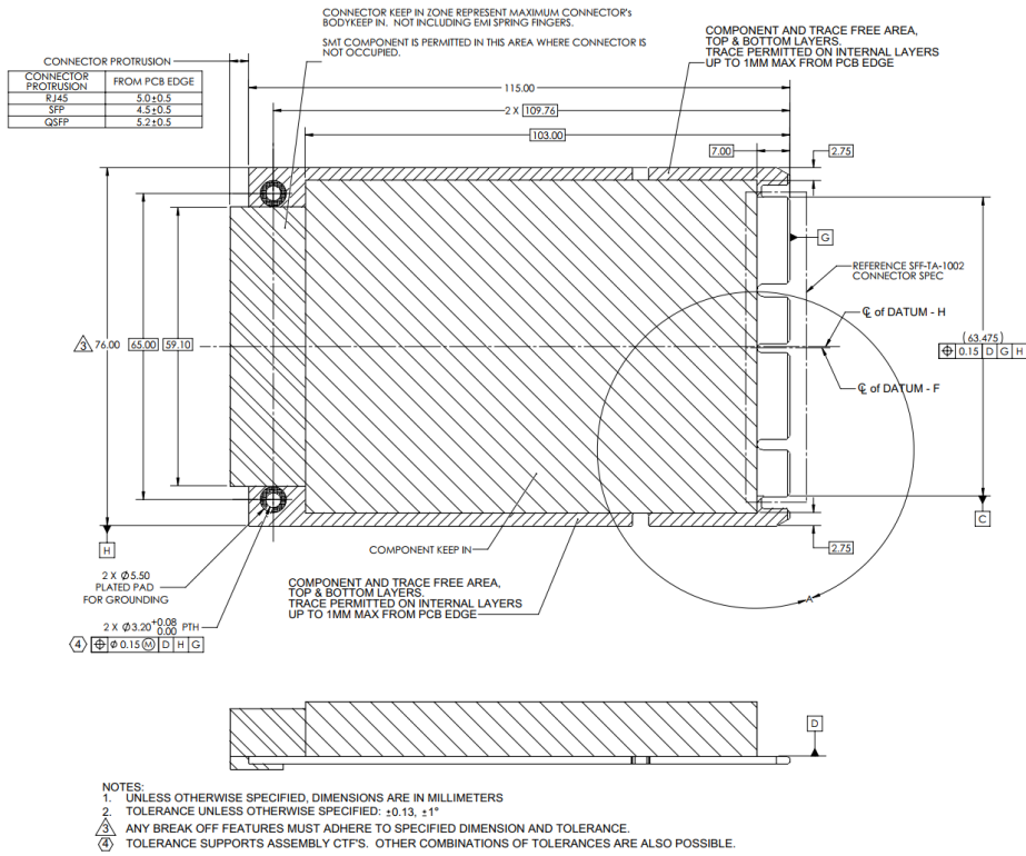
Figure 24: SFF Keep Out Zone – Top View
