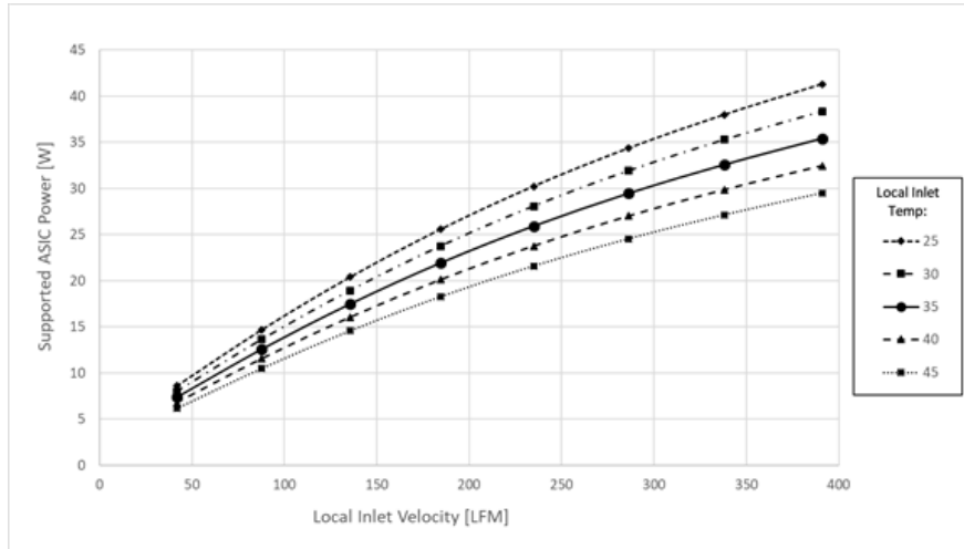
Figure 127 126: ASIC Supportable Power for Cold Aisle Cooling – SFF Card
