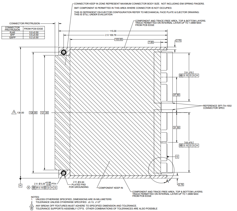
Figure 29: LFF Keep Out Zone – Top View
