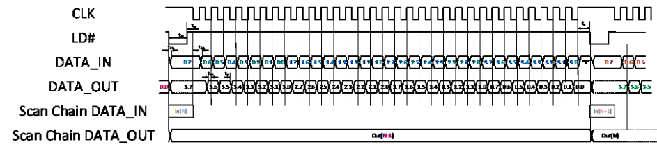
Figure 88: Scan Chain Timing Diagram Example 2
