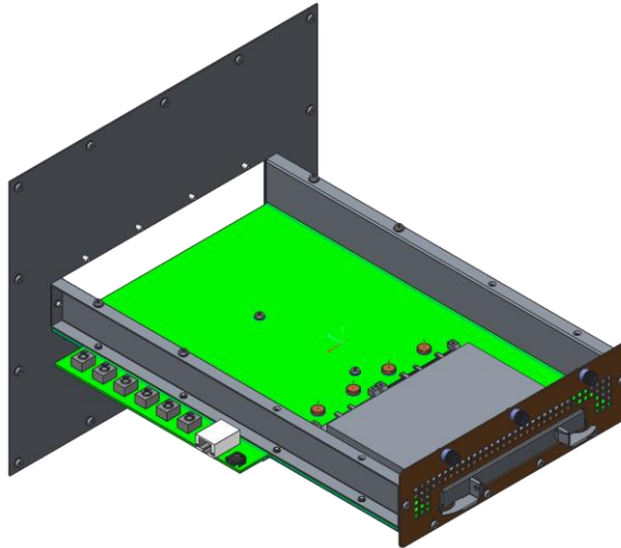
Figure 136: LFF Card Thermal Test Fixture Design – Cover Removed
