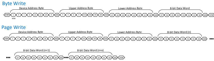
Figure 109: FRU EEPROM Writes with Double Byte Addressing
