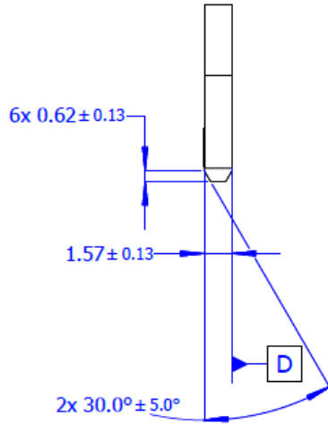
Figure 69: SFF Primary Connector Gold Finger - Detail D
