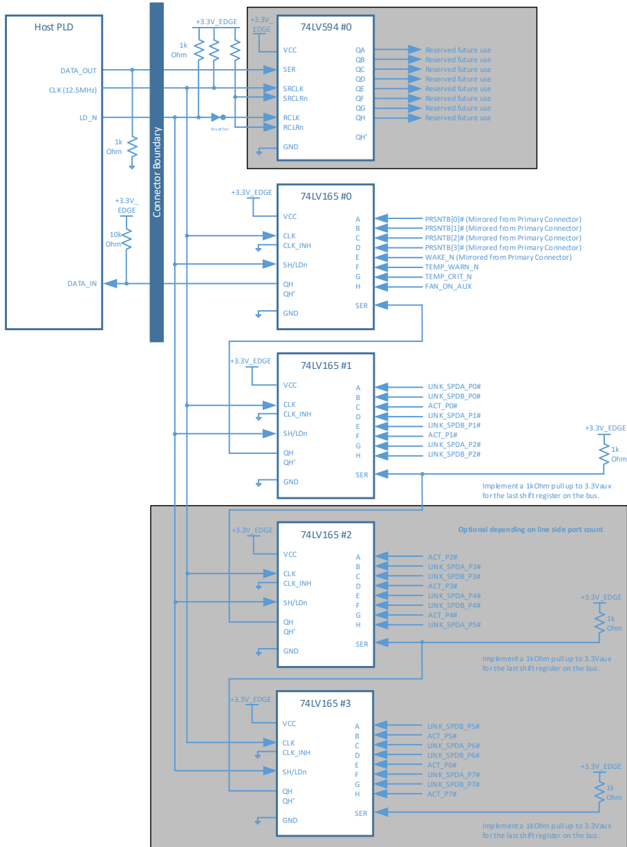
Figure 88: Scan Chain Connection Example
