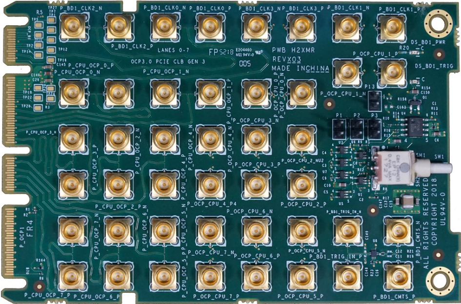
Figure 115414: PCIe Load Board Test Fixture for OCP NIC 3.0 SFF
