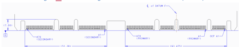
Figure 7170 : LFF Gold Finger Dimensions – x32 – Bottom Side (“A” Pins)
