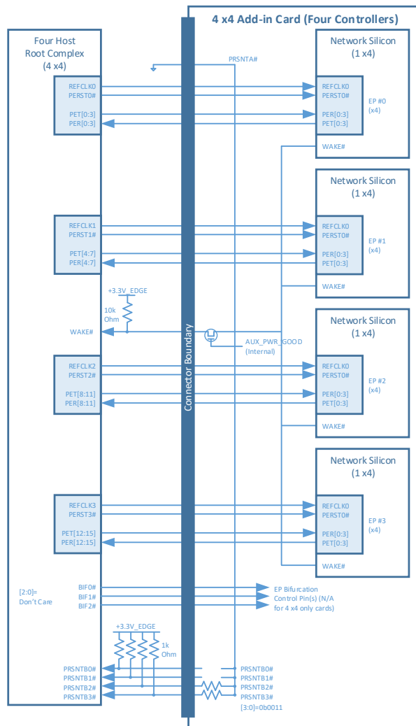
Figure 96 95: Quad Hosts (4 x4) and 4 x4 OCP NIC 3.0 Card (Quad Controllers)
