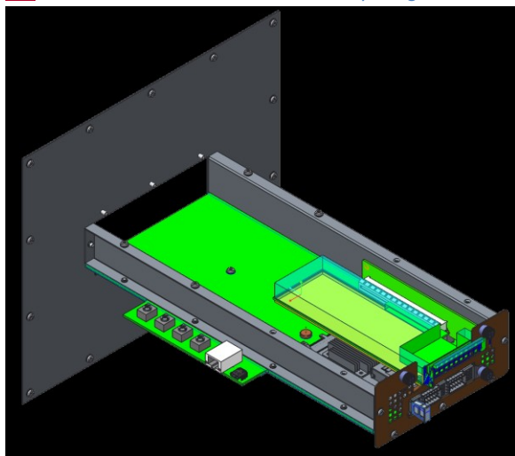
Figure 133 132: SFF Thermal Test Fixture Preliminary Design – Cover Removed
