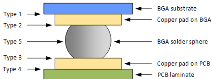
Figure 146 145 : Dye and Pull Type Locations
