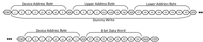
Figure 110109 : FRU EEPROM Reads with Double Byte Addressing
