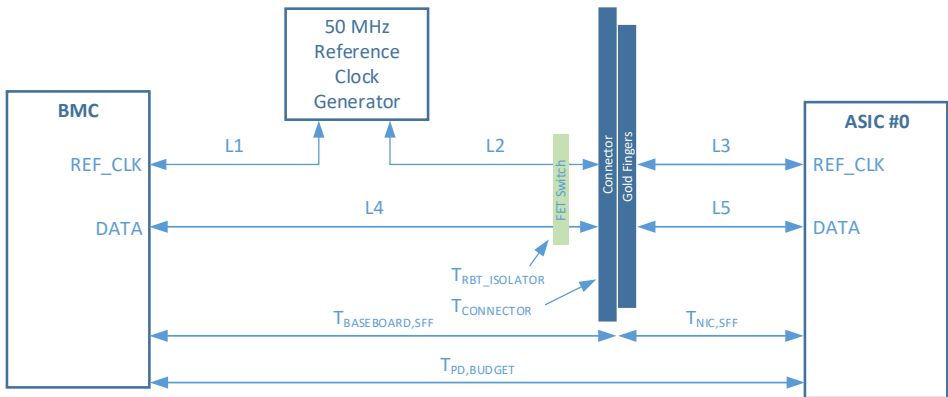
Figure 112.111 : NC-SI over RBT Timing Budget Topology
