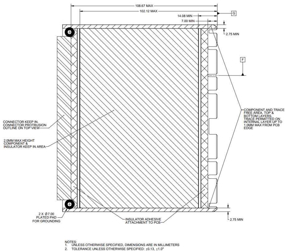
Figure 31: LFF Keep Out Zone – Bottom View
