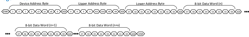
Figure 110109 : FRU EEPROM Reads with Double Byte Addressing
