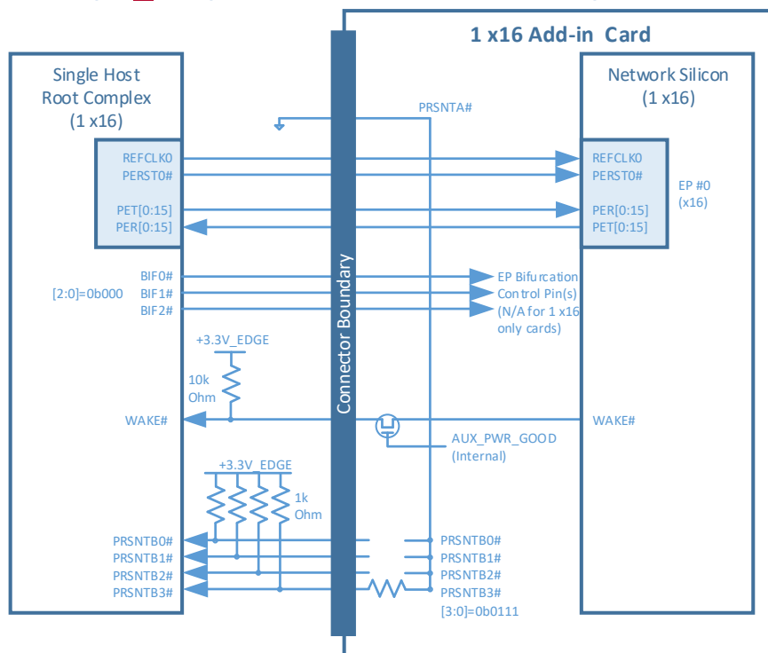
Figure 93 92 : Single Host (1 x16) and 1 x16 OCP NIC 3.0 Card (Single Controller)
