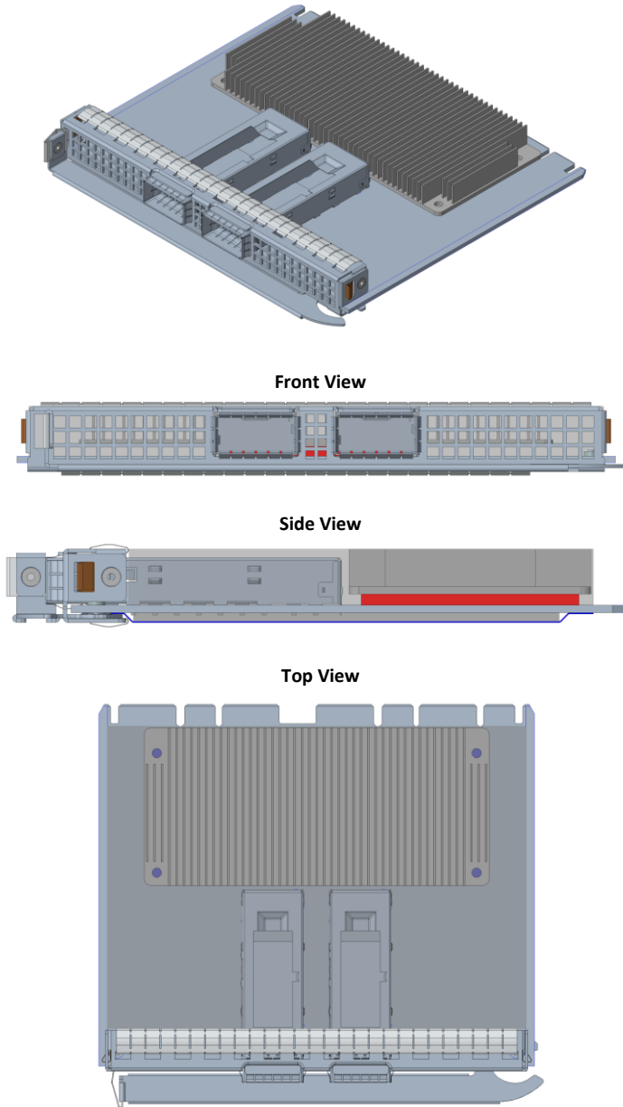
Figure 10: LFF NIC Configuration Views
