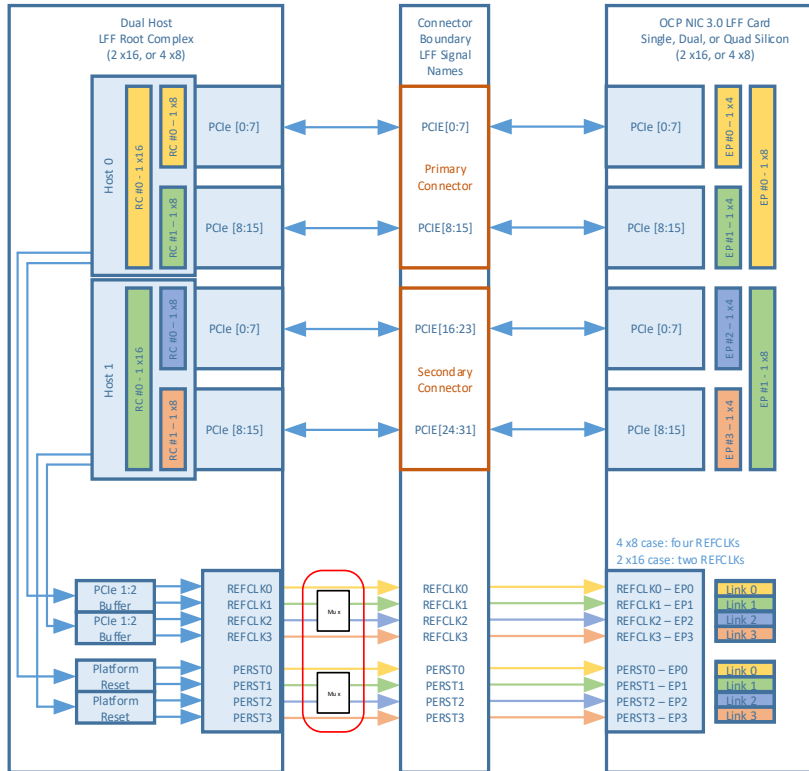
Figure 102401 102401: LFF PCIe REFCLK Mapping – Dual Host – 2 and 4 links
