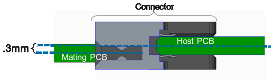
Figure 7978 : 0.3 mm Offset for 0.076" Thick Baseboards
