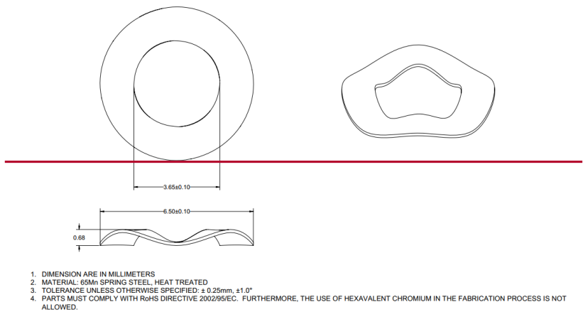
Figure 23: Wave Washer
