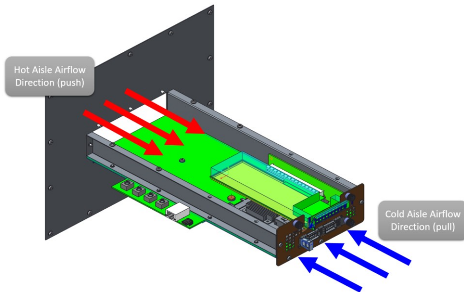
Figure 138 137 : Thermal Test Fixture Airflow Direction
