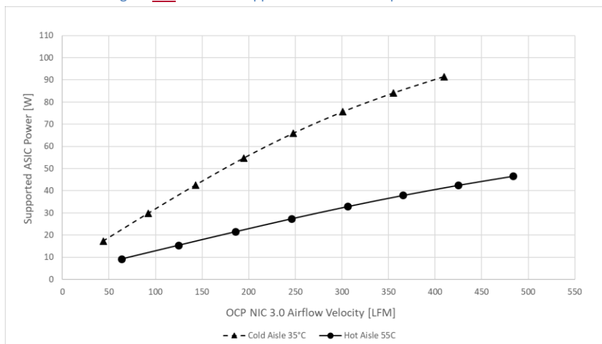
Figure 131130 130: ASIC Supportable Power Comparison – LFF Card
