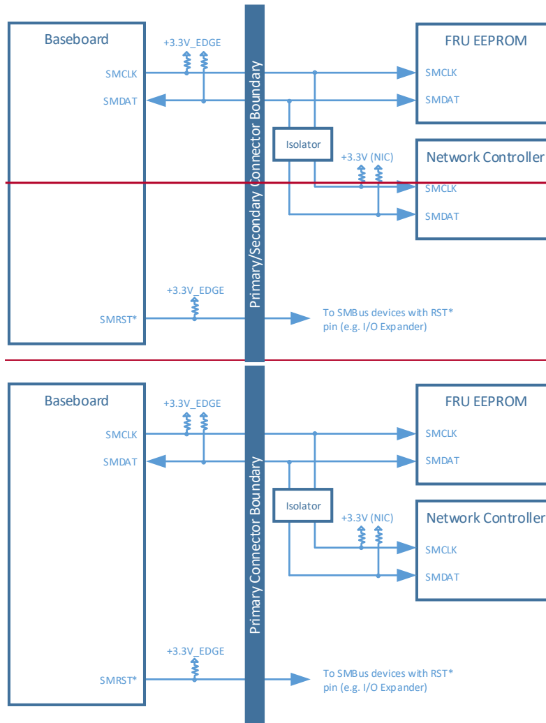
Figure 8483 : Example SMBus Connections
