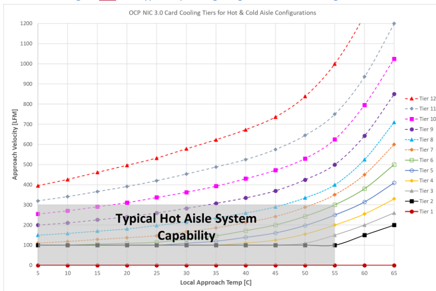
Figure 1424 141: Typical Operating Range for Hot Aisle Configurations
