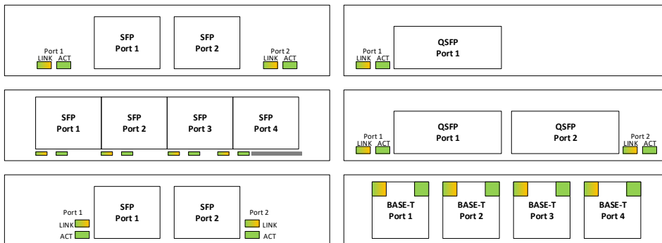
Figure 104 103: Port and LED Ordering – Example SFF Link/Activity and Speed LED Placement
