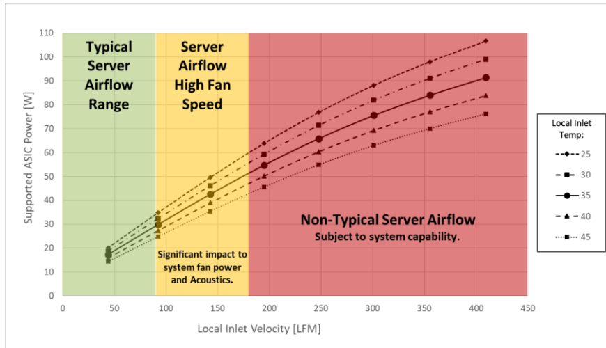
Figure 130129 130: Server System Airflow Capability – LFF Cold Aisle Cooling
