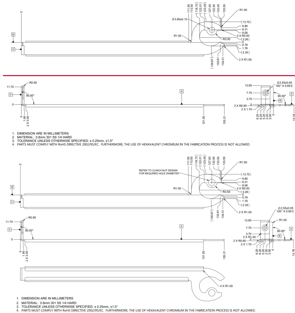
Figure 20: LFF I/O Faceplate – Ejector Lever (2D View)
