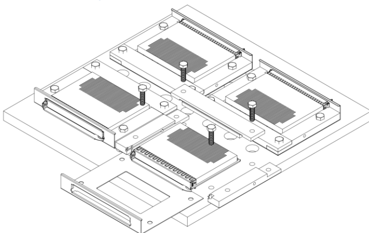
Figure 145144 : LFF Shock and Vibe Fixture
