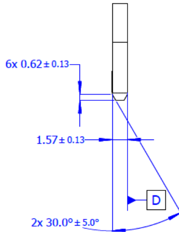
Figure 6968 : SFF Primary Connector Gold Finger - Detail D
