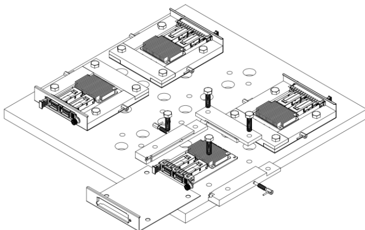
Figure 144143 : SFF Shock and Vibe Fixture
