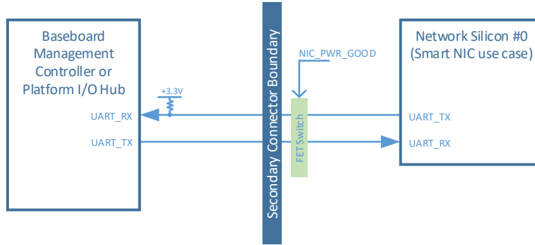
Figure 92: UART Connection Example
