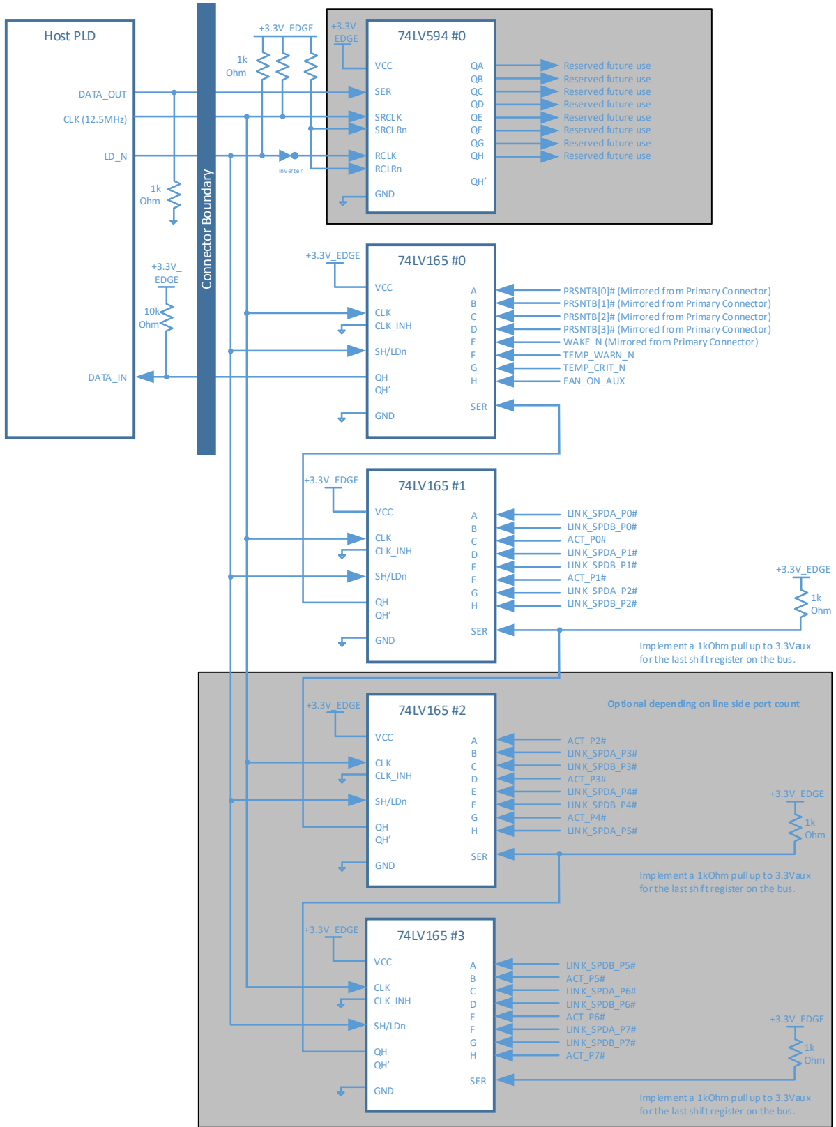
Figure 88: Scan Chain Connection Example
