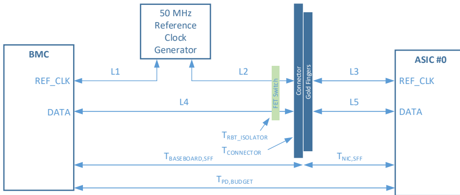
Figure 112141 : NC-SI over RBT Timing Budget Topology
