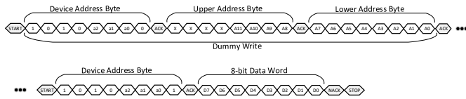
Figure 110409: FRU EEPROM Reads with Double Byte Addressing
