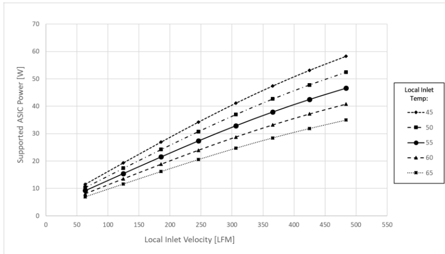
Figure 123Figure 122: ASIC Supportable Power for Hot Aisle Cooling – LFF Card
