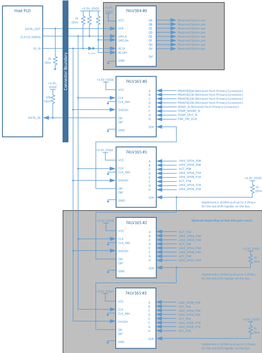
Figure 8887: Scan Chain Connection Example
