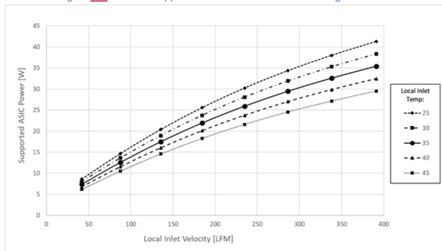
Figure 126 125: ASIC Supportable Power for Cold Aisle Cooling – SFF Card
