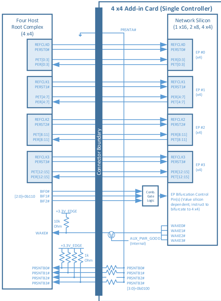
Figure 9594: Quad Hosts (4 x4) and 4 x4 OCP NIC 3.0 Card (Single Controller)
