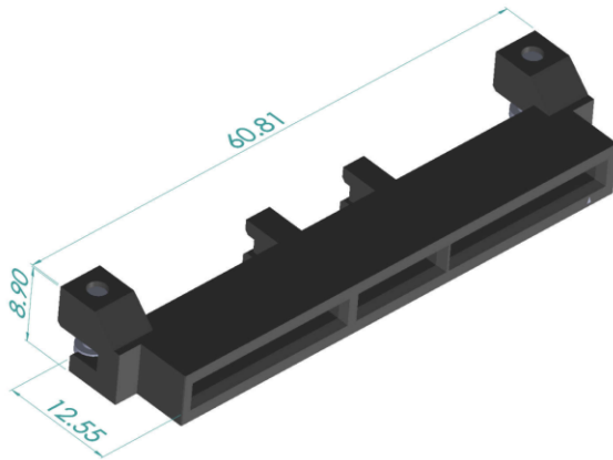
Figure 7675 : 140-pin Base Board Secondary Connector – Straddle Mount
