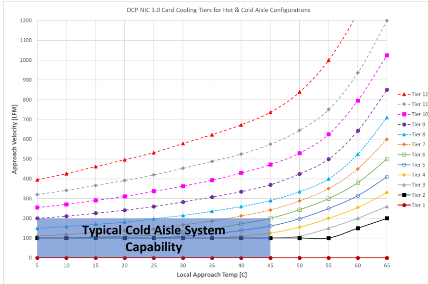
Figure 143142: Typical Operating Range for Cold Aisle Configurations
