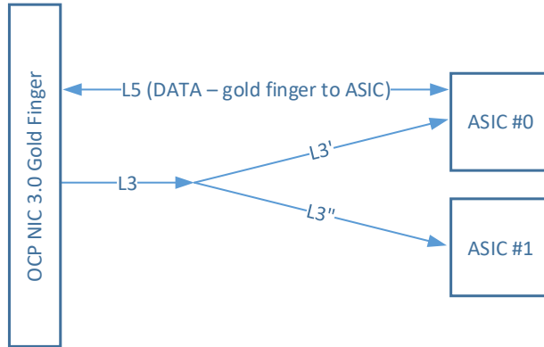
Figure 113112: NC-SI over RBT Propagation Delay Matching for Two Target ASICs – No Clock Buffer
