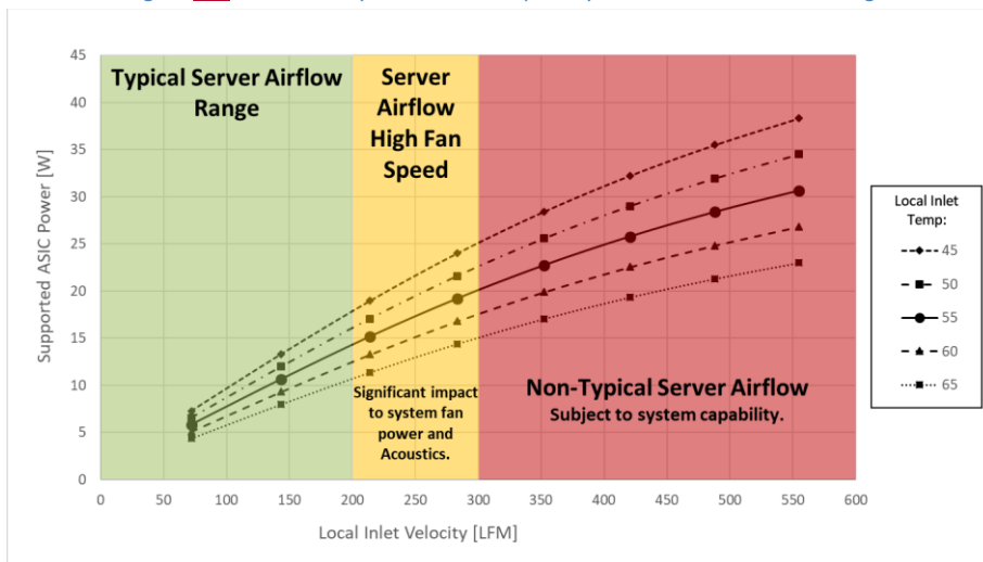
Figure 121120: Server System Airflow Capability – SFF Card Hot Aisle Cooling
