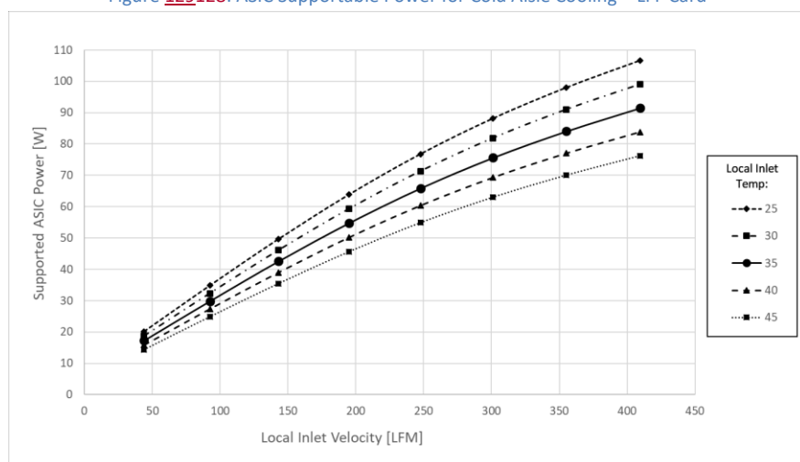
Figure 129 128 : ASIC Supportable Power for Cold Aisle Cooling – LFF Card
