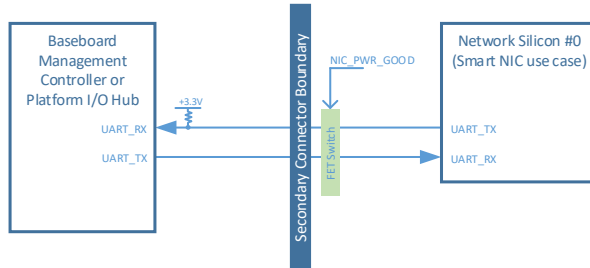
Figure 9291 : UART Connection Example
