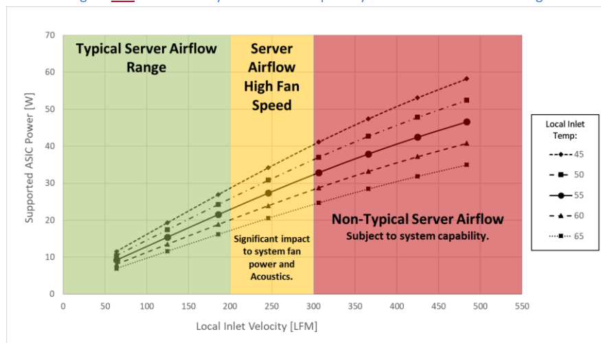
Figure 125124 : Server System Airflow Capability – LFF Card Hot Aisle Cooling
