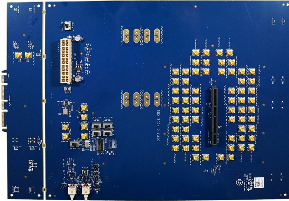
Figure 116445 : PCIe Base Board Test Fixture for OCP NIC 3.0 SFF
