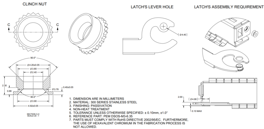
Figure 22: Clinch Nut Option A Ejector-Bushing
