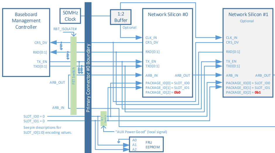
Figure 8584: NC-SI over RBT Connection Example – Single Primary Connector
