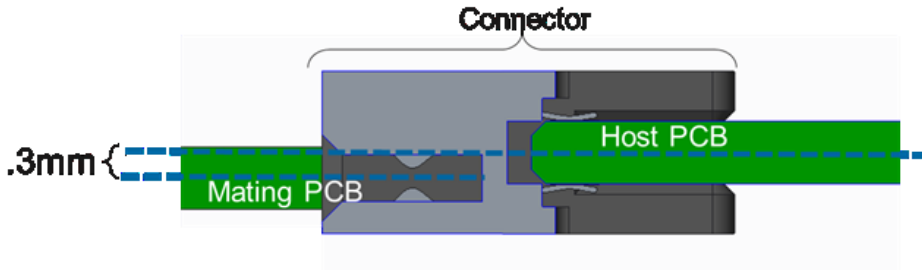
Figure 7978: 0.3 mm Offset for 0.076" Thick Baseboards
