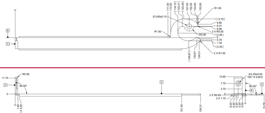
Figure 20: LFF I/O Faceplate – Ejector Lever (2D View)
