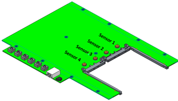
Figure 137136 : LFF Card Thermal Test Fixture PCB
