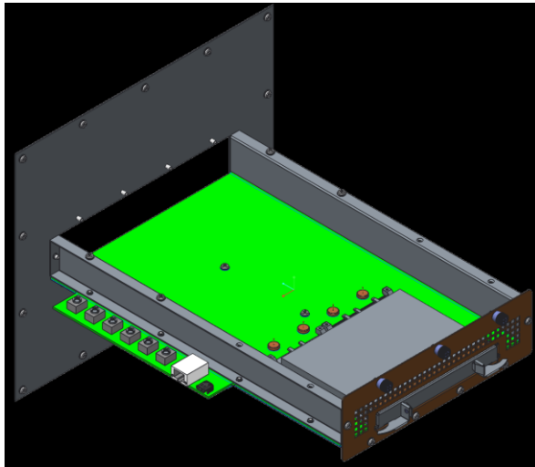
Figure 136 135 : LFF Card Thermal Test Fixture Design – Cover Removed
