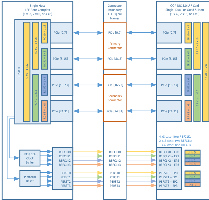
Figure 101400 : LFF PCIe REFCLK Mapping – Single Host – 1, 2 and 4 links
