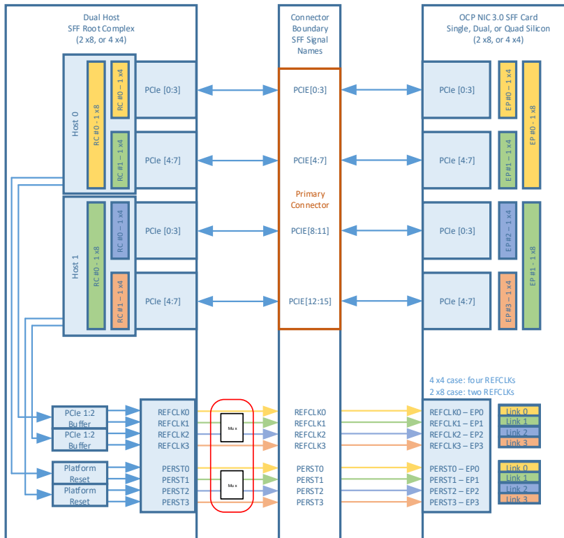
Figure 9998: SFF PCIe REFCLK Mapping – Dual Host – 2 and 4 links
