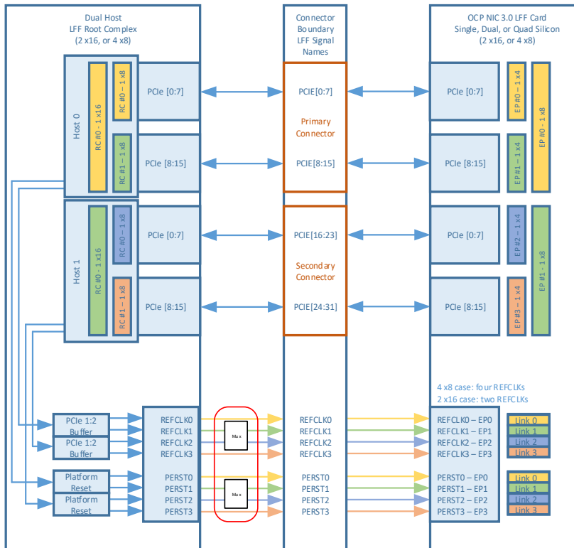
Figure 102401 : LFF PCIe REFCLK Mapping – Dual Host – 2 and 4 links
