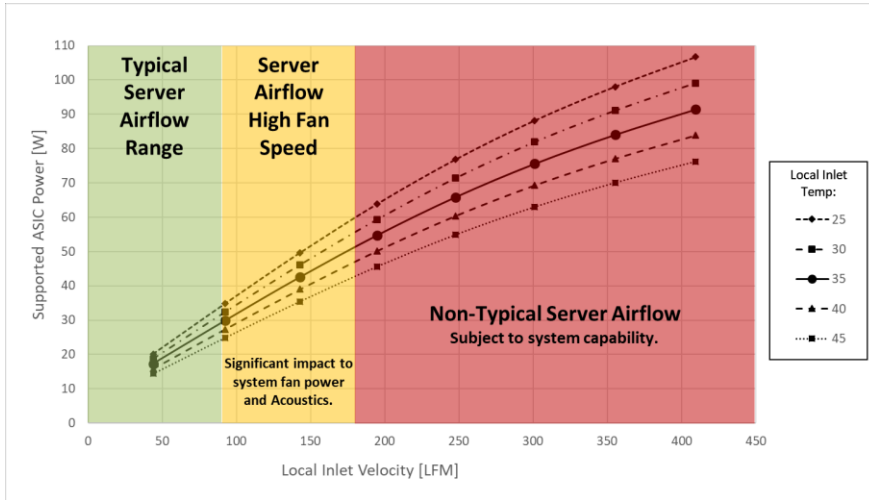
Figure 130129 : Server System Airflow Capability – LFF Cold Aisle Cooling
