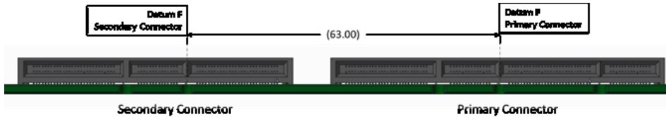
Figure 8079: Primary and Secondary Connector Locations for LFF Support with Right Angle Connectors
