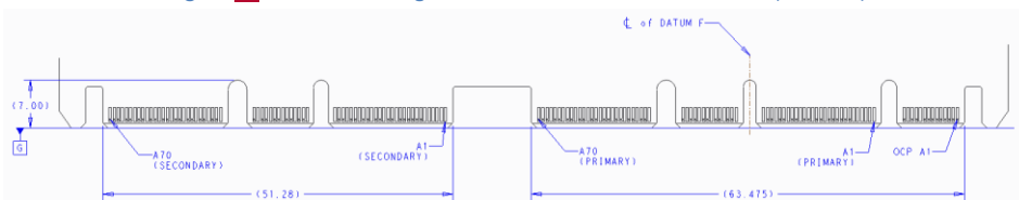
Figure 7170: LFF Gold Finger Dimensions – x32 – Bottom Side (“A” Pins)
