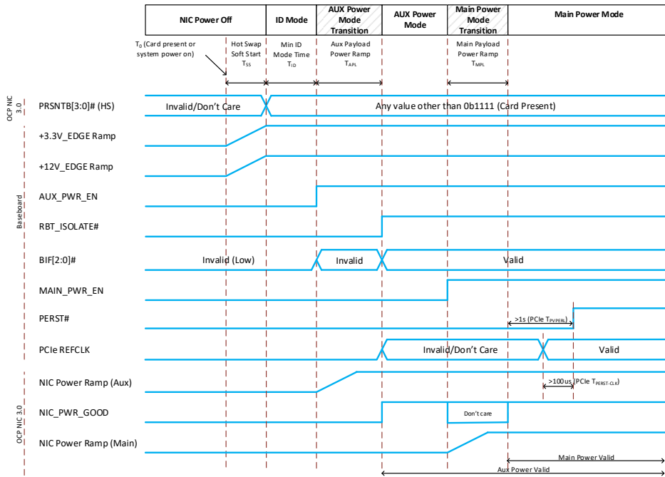
Figure 106405: Power-Up Sequencing – Normal Operation
