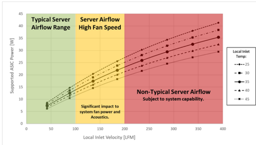
Figure 127126 : Server System Airflow Capability – SFF Cold Aisle Cooling
