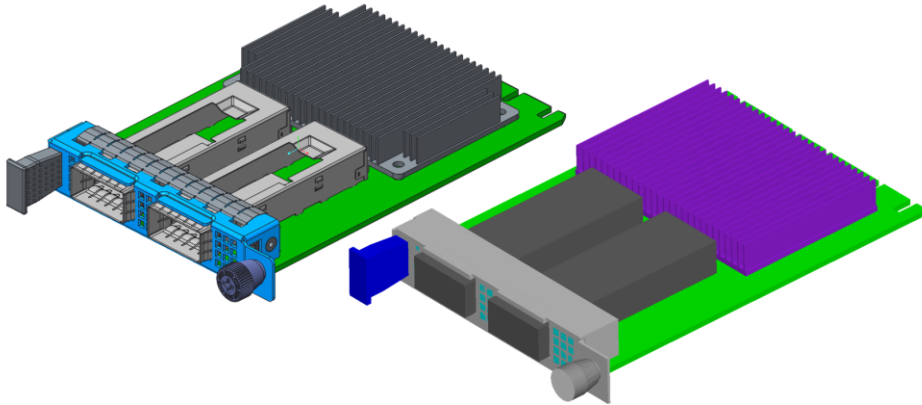
Figure 120149: OCP NIC 3.0 SFF Reference Design and CFD Geometry
