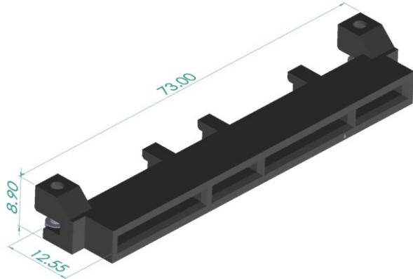
Figure 7675 : 140-pin Base Board Secondary Connector – Straddle Mount
