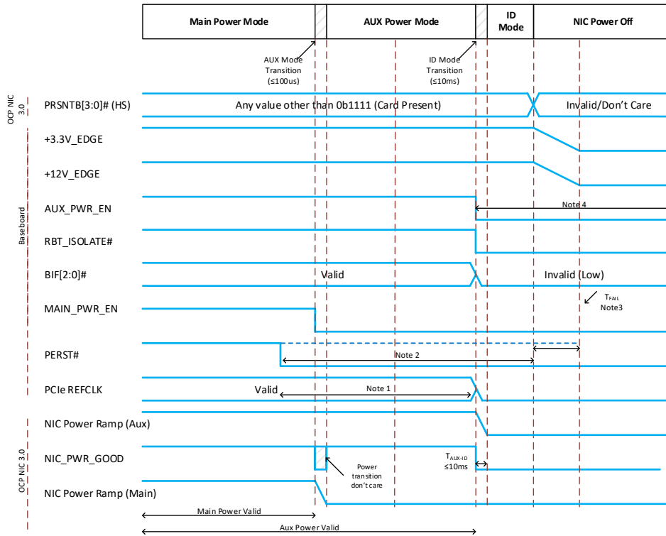
Figure 107106: Power-Down Sequencing – Normal Operation
