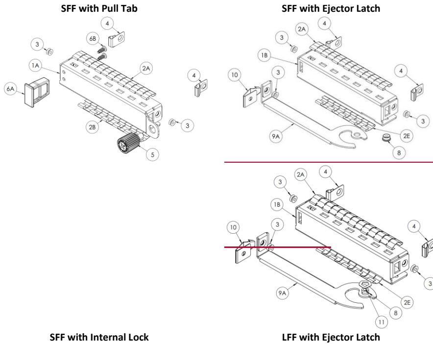
Figure 14: Faceplate Assembly Exploded Views (SFF and LFF)
