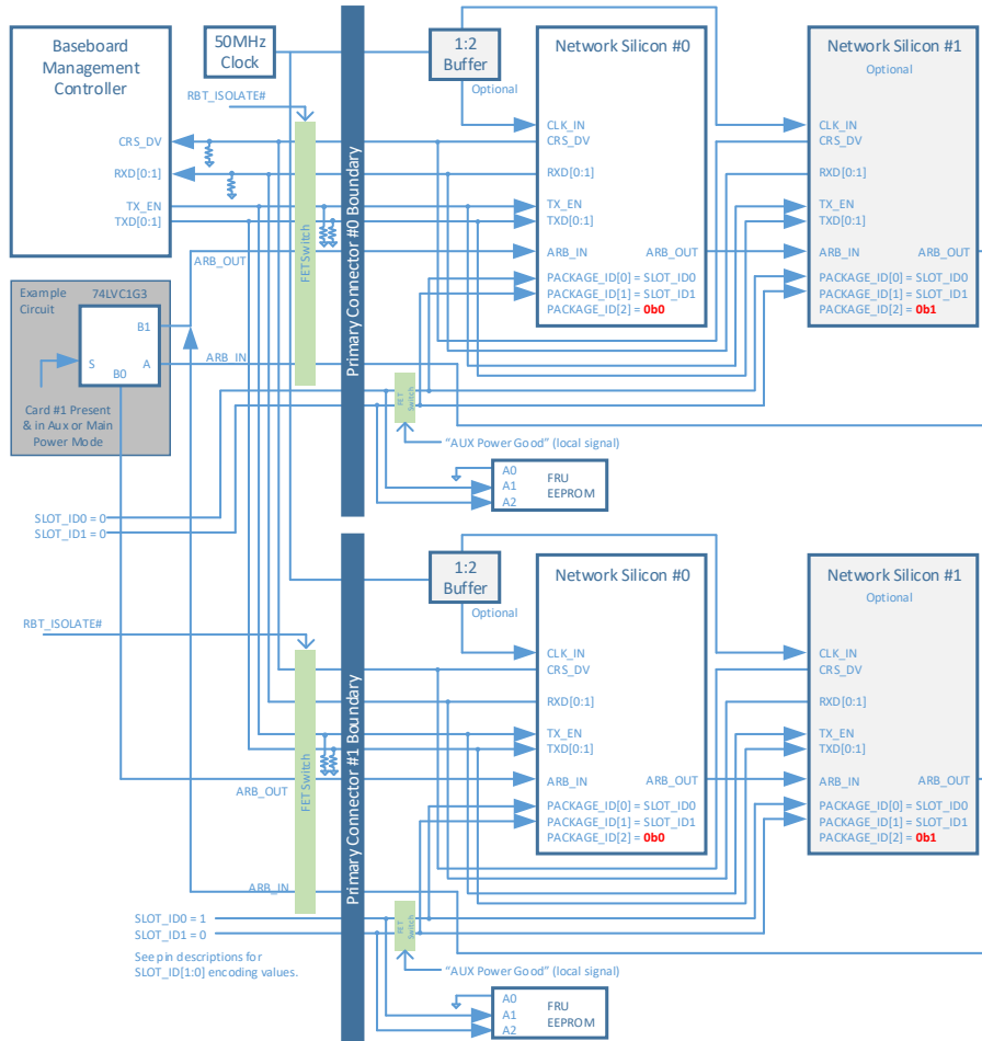
Figure 8685: NC-SI over RBT Connection Example – Dual Primary Connectors
