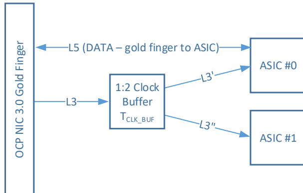
Figure 114113: NC-SI over RBT Propagation Delay Matching for Two Target ASICs – Clock Buffer
