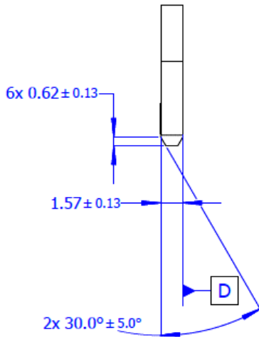
Figure 6867: SFF Primary Connector Card Profile Dimensions
