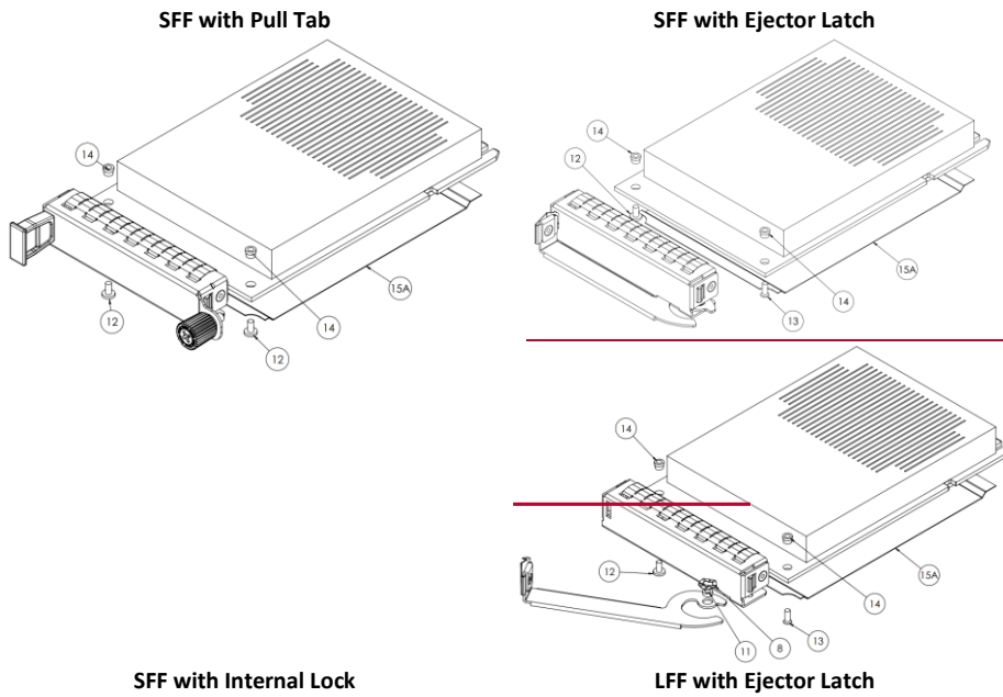
Figure 13: PBA Exploded Views (SFF and LFF)
