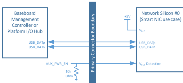
Figure 9089 : USB 2.0 Connection Example – Basic Connectivity
