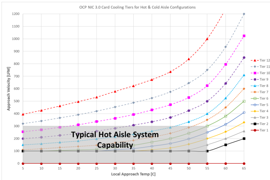
Figure 142441 : Typical Operating Range for Hot Aisle Configurations
