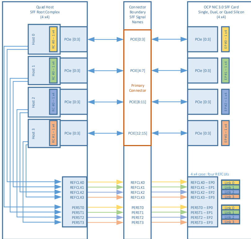
Figure 10099: SFF PCIe REFCLK Mapping – Quad Host – 4 Links
