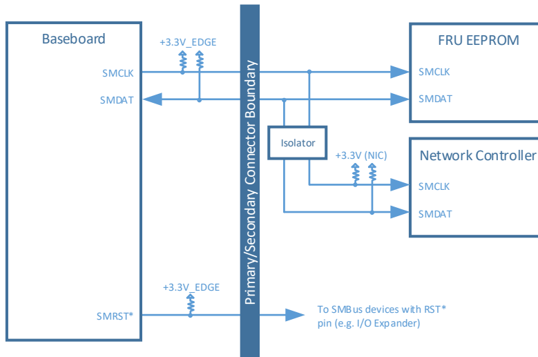
Figure 8483 : Example SMBus Connections
