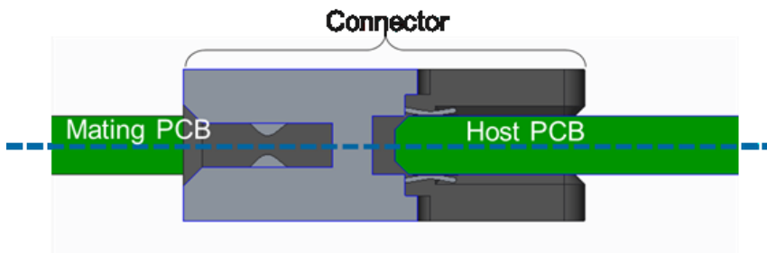
Figure 78 77 : 0 mm Offset (Coplanar) for 0.062" Thick Baseboards
