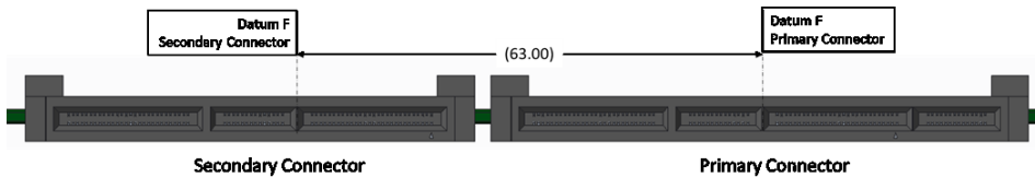
Figure 8180: Primary and Secondary Connector Locations for LFF Support with Straddle Mount Connectors
