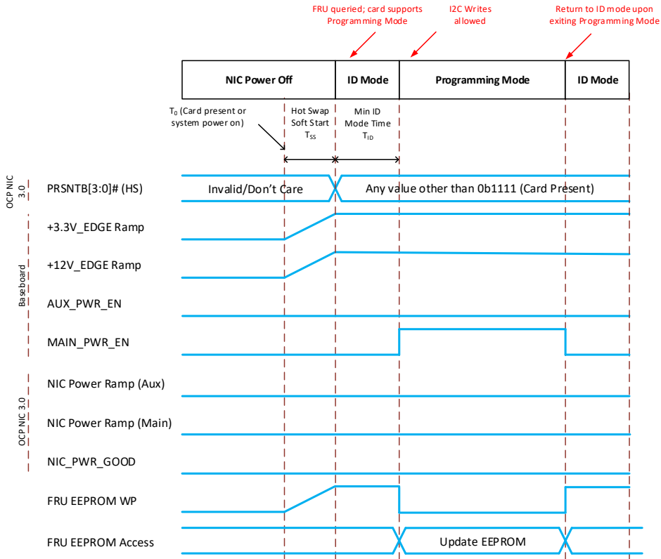
Figure 108107: Programming Mode Sequencing
