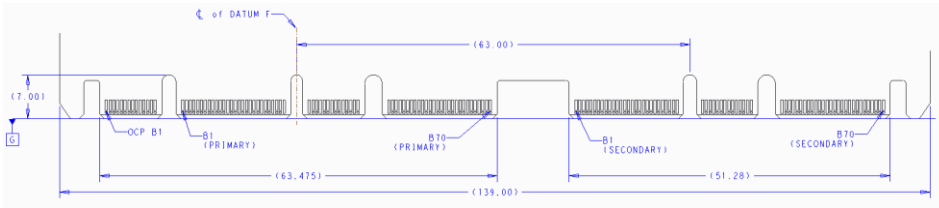
Figure 7069: LFF Gold Finger Dimensions – x32 – Top Side (“B” Pins)
