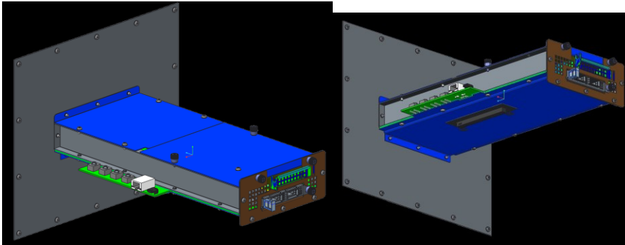
Figure 132 131 : SFF Thermal Test Fixture Preliminary Design
