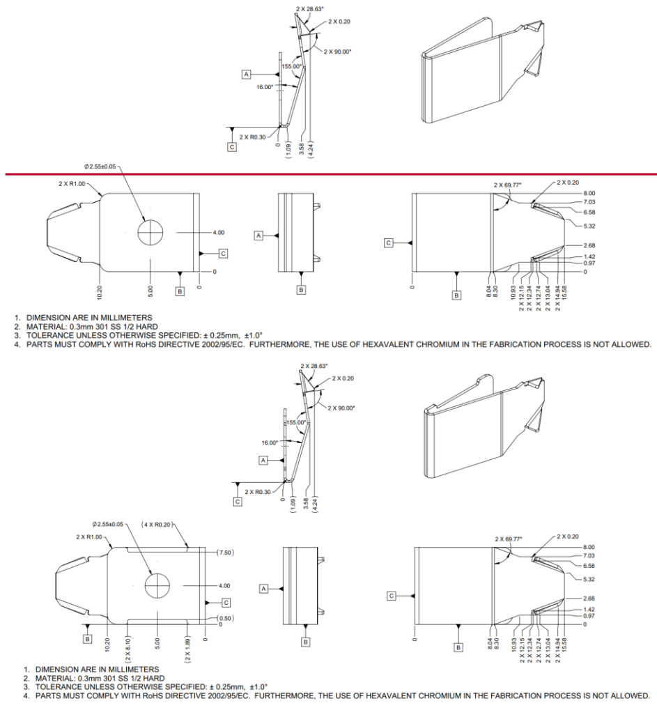
Figure 21: Ejector Lock
