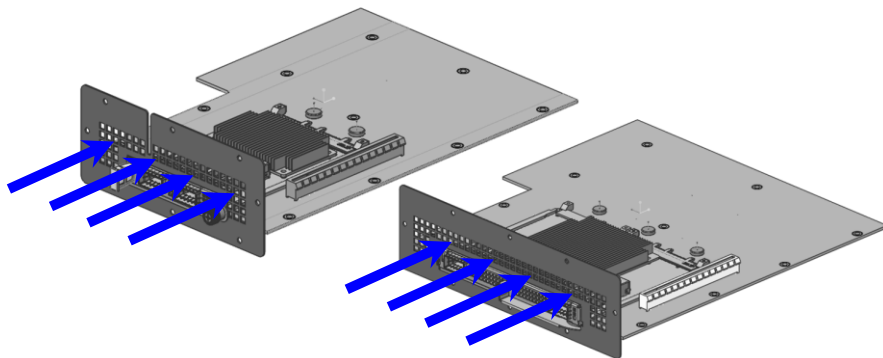
Figure 118 117 : Airflow Direction for Cold Aisle Cooling (SFF and LFF)
