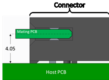
Figure 7473: OCP NIC 3.0 Card and Host Offset for Right Angle Connectors
