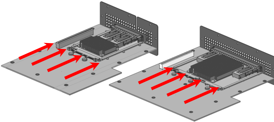
Figure 117 116: Airflow Direction for Hot Aisle Cooling (SFF and LFF)
