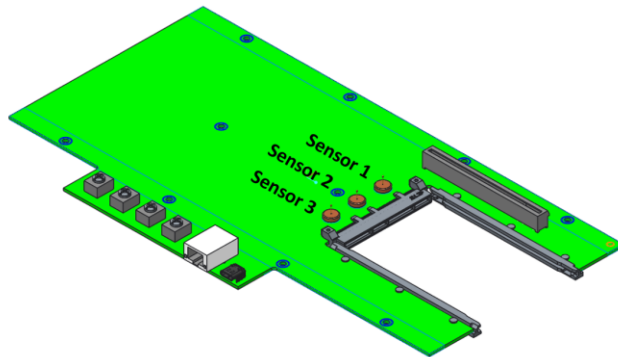
Figure 134133 : SFF Card Thermal Test Fixture PCB
