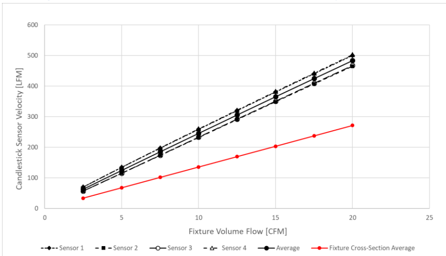
Figure 140139 : LFF Fixture, Hot Aisle Flow – Candlestick Air Velocity vs. Volume Flow
