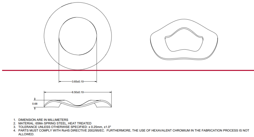
Figure 23: Wave Washer
