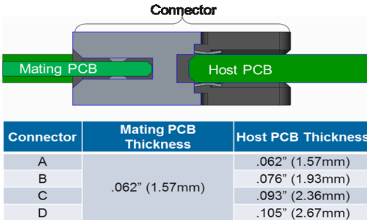
Figure 77 76 : OCP NIC 3.0 Card and Baseboard PCB Thickness Options for Straddle Mount Connectors
