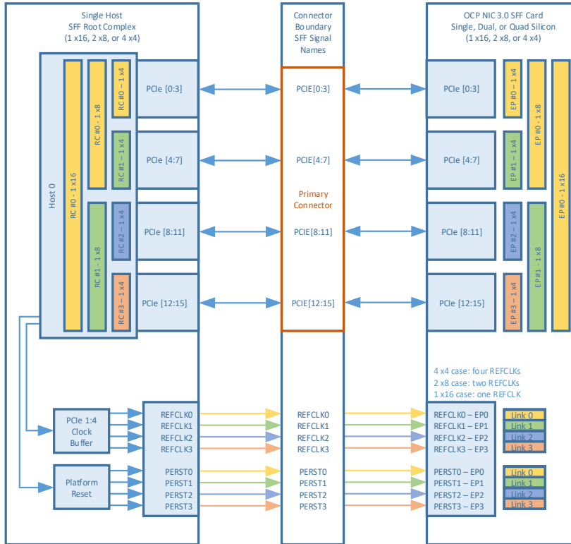
Figure 989 7: SFF PCIe REFCLK Mapping – Single Host – 1, 2 and 4 links
