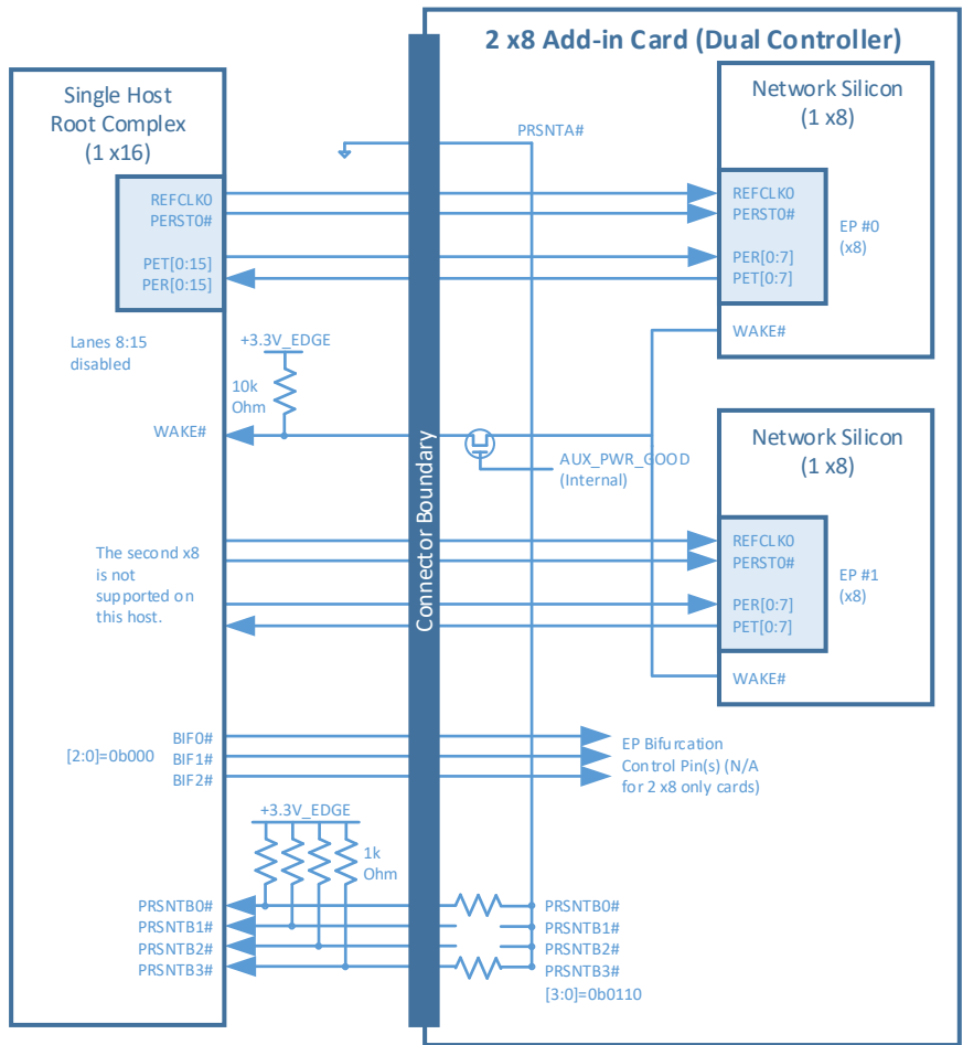
Figure 9796: Single Host with no Bifurcation (1 x16) and 2 x8 OCP NIC 3.0 Card (Dual Controllers)
