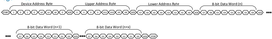
Figure 110409: FRU EEPROM Reads with Double Byte Addressing
