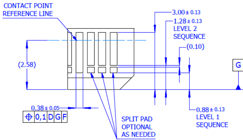
Figure 6968: SFF Primary Connector Gold Finger - Detail D
