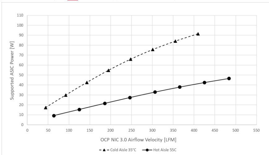
Figure 131130 : ASIC Supportable Power Comparison – LFF Card
