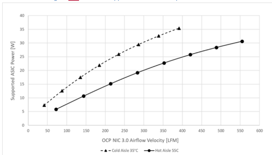
Figure 128127 : ASIC Supportable Power Comparison – SFF Card
