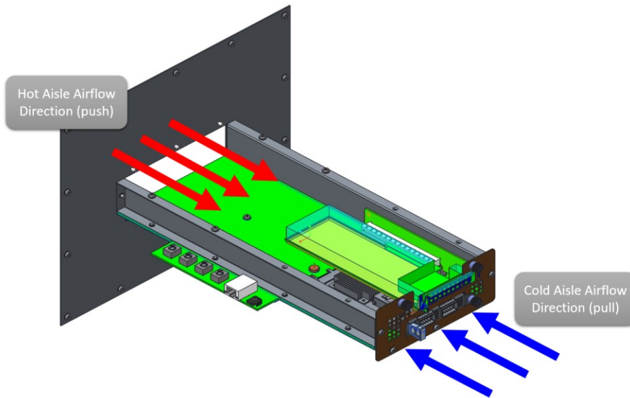
Figure 138 137 : Thermal Test Fixture Airflow Direction
