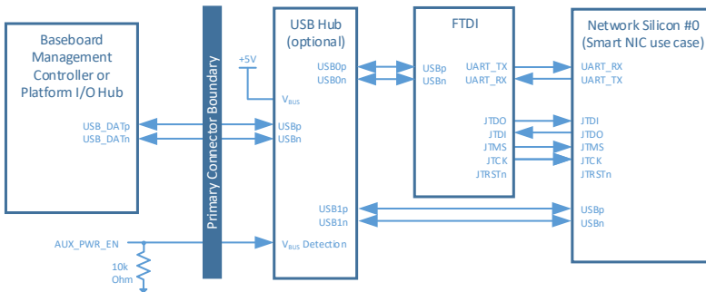
Figure 9190 : USB 2.0 Connection Example – USB-Serial / USB-JTAG Connectivity
