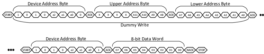
Figure 109: FRU EEPROM Reads with Double Byte Addressing
