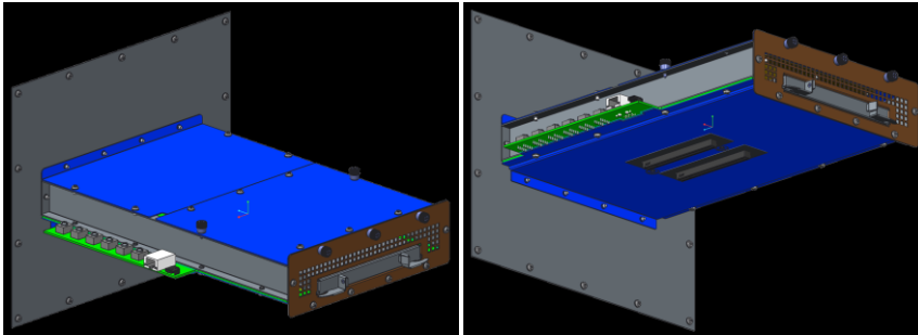
Figure 134 133 131 : LFF Card Thermal Test Fixture Design
