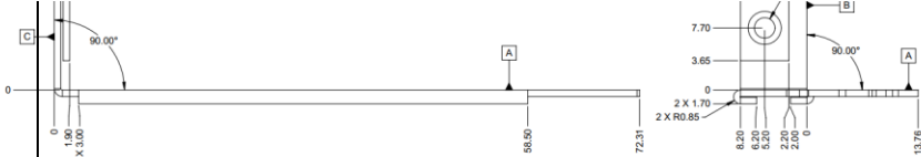
Figure 19: SFF I/O Faceplate – Ejector Lever (2D View)
