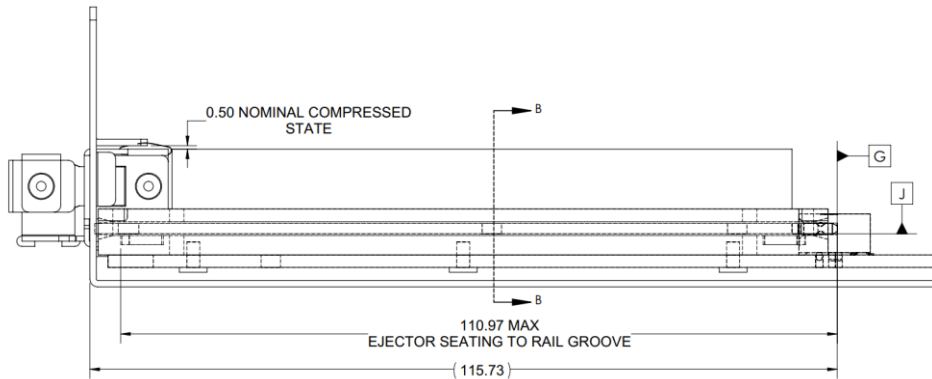
Figure 52: SFF Baseboard Chassis CTF Dimensions (Rear Rail Guide View)
