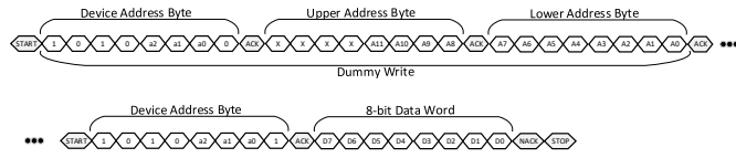
Figure 109109108: FRU EEPROM Reads with Double Byte Addressing
