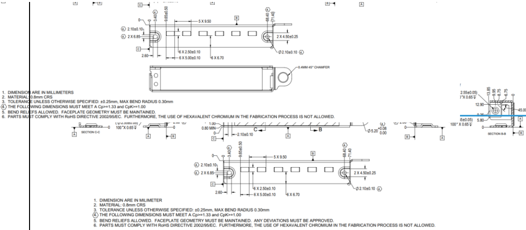
Figure 15: SFF Generic I/O Faceplate with Pulltab Version (2D View)
