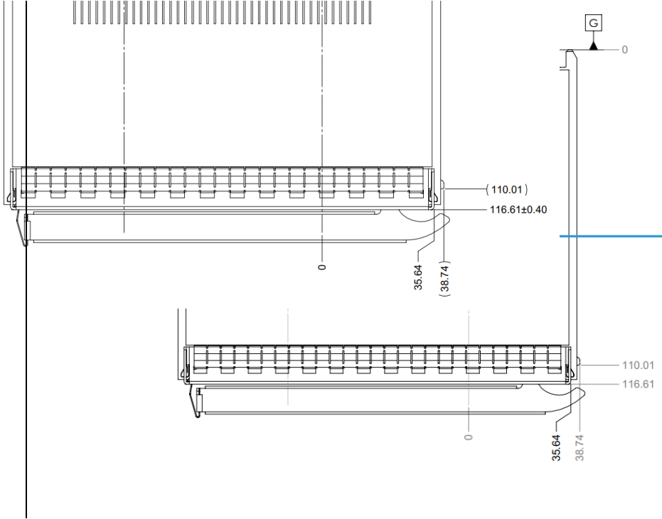
Figure 55: LFF OCP NIC 3.0 Card with Ejector CTF Dimensions (Front View)
