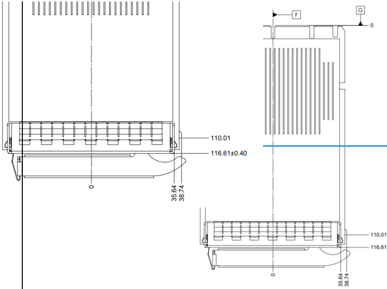
Figure 43: SFF OCP NIC 3.0 Card with Ejector CTF Dimensions (Top View)
