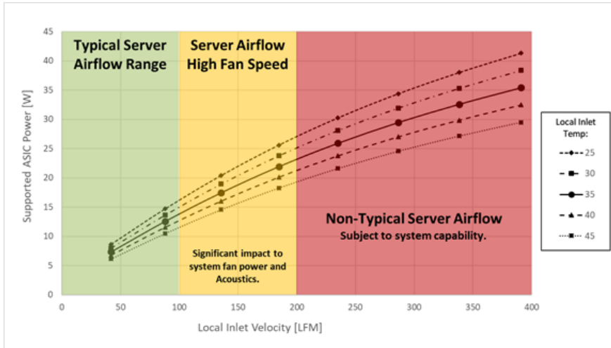
Figure 126125123 123: Server System Airflow Capability – SFF Cold Aisle Cooling
