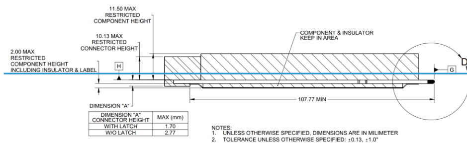
Figure 27: SFF Keep Out Zone – Side View
