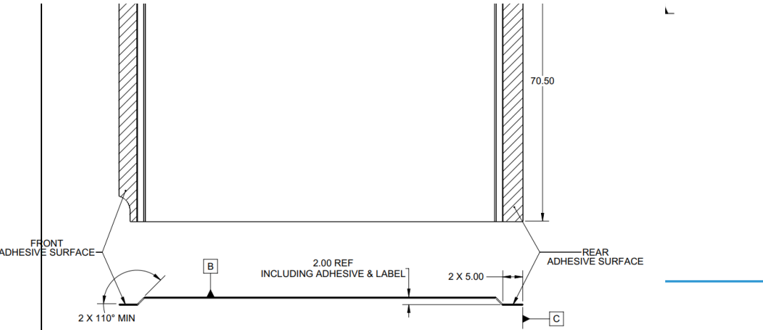
Figure 35: SFF Bottom Side Insulator (Top and Side View)
