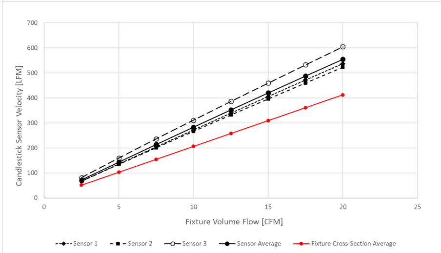
Figure 139138136 : LFF Fixture, Hot Aisle Flow — Candlestick Air Velocity vs. Volume Flow
