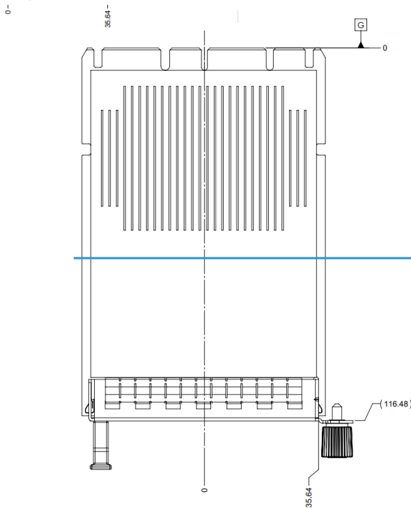
Figure 40: SFF OCP NIC 3.0 Card with Pull Tab CTF Dimensions (Top View)
