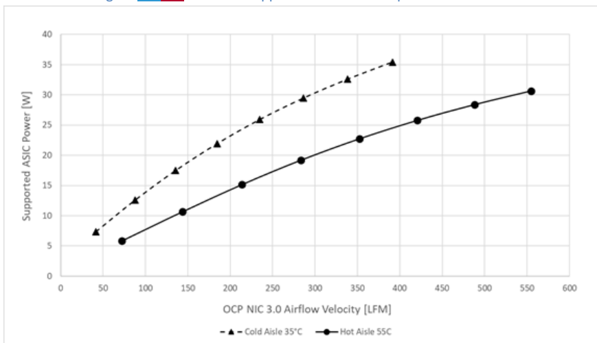
Figure 127126124 124: ASIC Supportable Power Comparison – SFF Card
