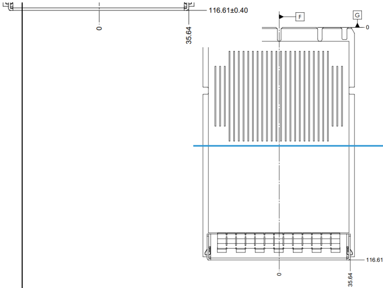
Figure 46: SFF OCP NIC 3.0 Card with Internal Lock CTF Dimensions (Top View)
