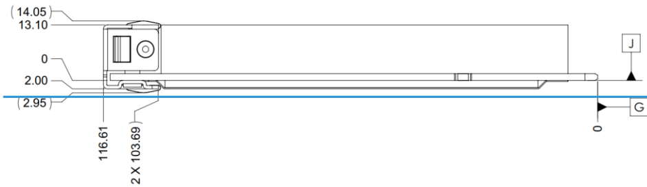
Figure 48: SFF OCP NIC 3.0 Card with Internal Lock CTF Dimensions (Side View)
