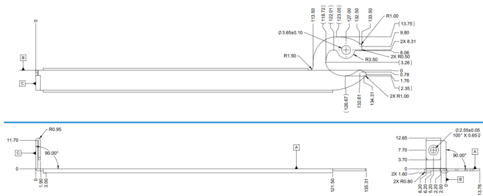
Figure 20: LFF I/O Faceplate – Ejector Lever (2D View)
