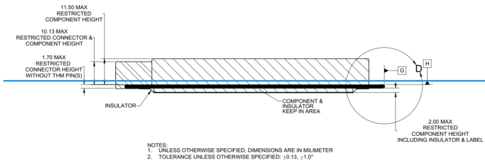
Figure 32: LFF Keep Out Zone – Side View
