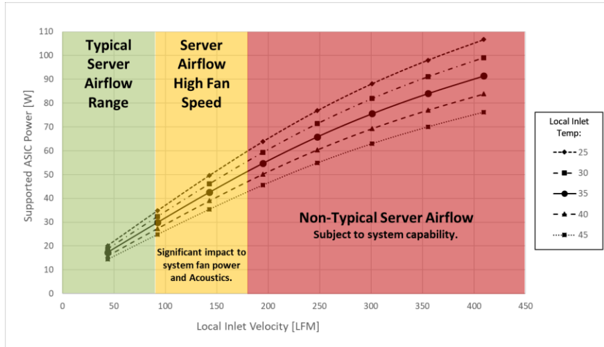
Figure 129129126 126: Server System Airflow Capability – LFF Cold Aisle Cooling
