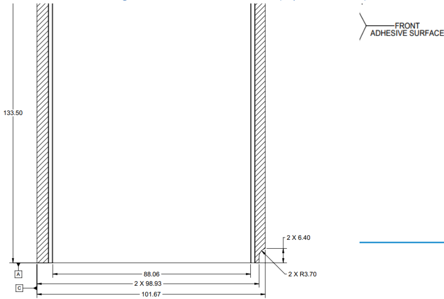
Figure 38: LFF Bottom Side Insulator (Top and Side View)
