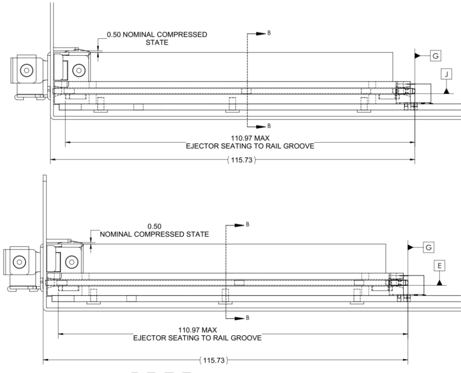
Figure 59: LFF Baseboard Chassis CTF Dimensions (Rail Guide View)
