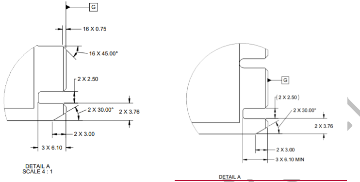
Figure 30: LFF Keep Out Zone – Top View – Detail A
