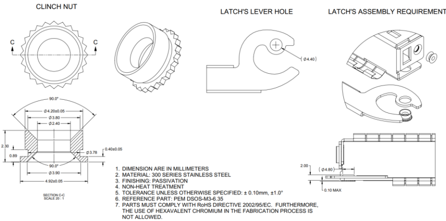
Figure 23: Clinch Nut Option B
