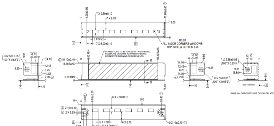
Figure 17: SFF Generic I/O Faceplate – Internal Lock Version (2D View)
