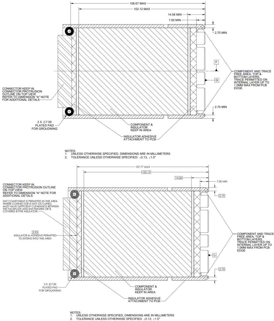
Figure 27: SFF Keep Out Zone – Side View
