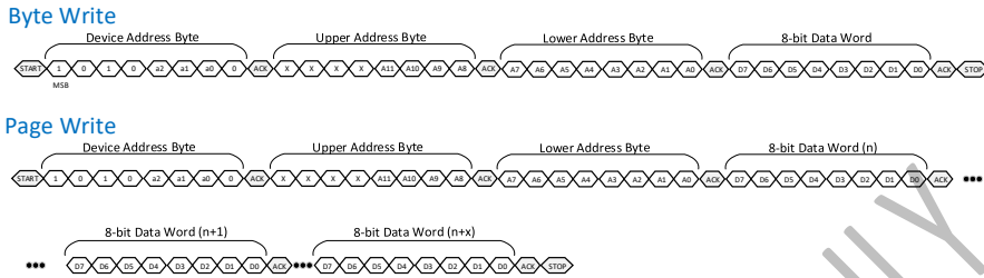
Figure 109: FRU EEPROM Writes with Double Byte Addressing
