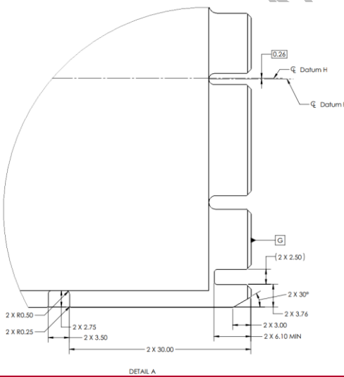
Figure 26: SFF Keep Out Zone – Bottom View
