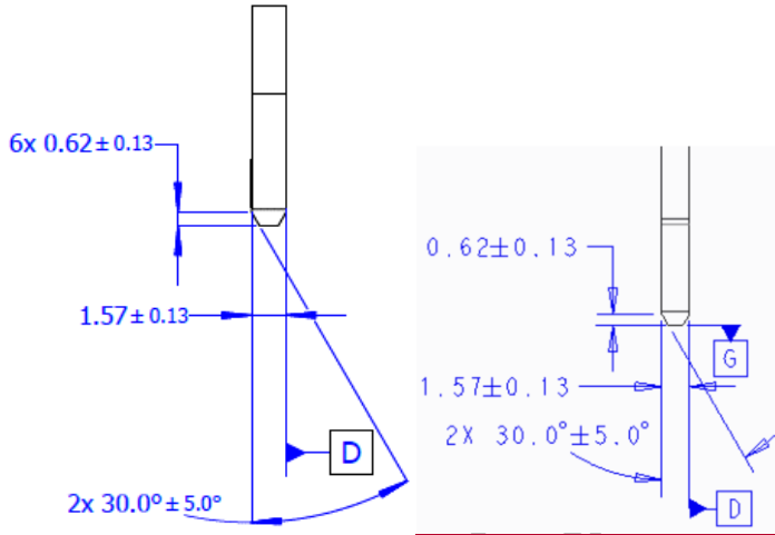
Figure 69: SFF Primary Connector Gold Finger - Detail D
