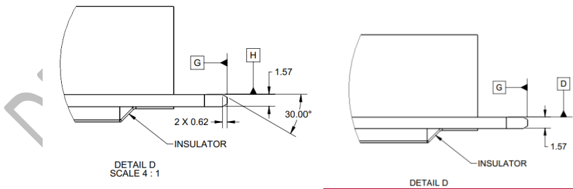
Figure 33: LFF Keep Out Zone – Side View – Detail D
