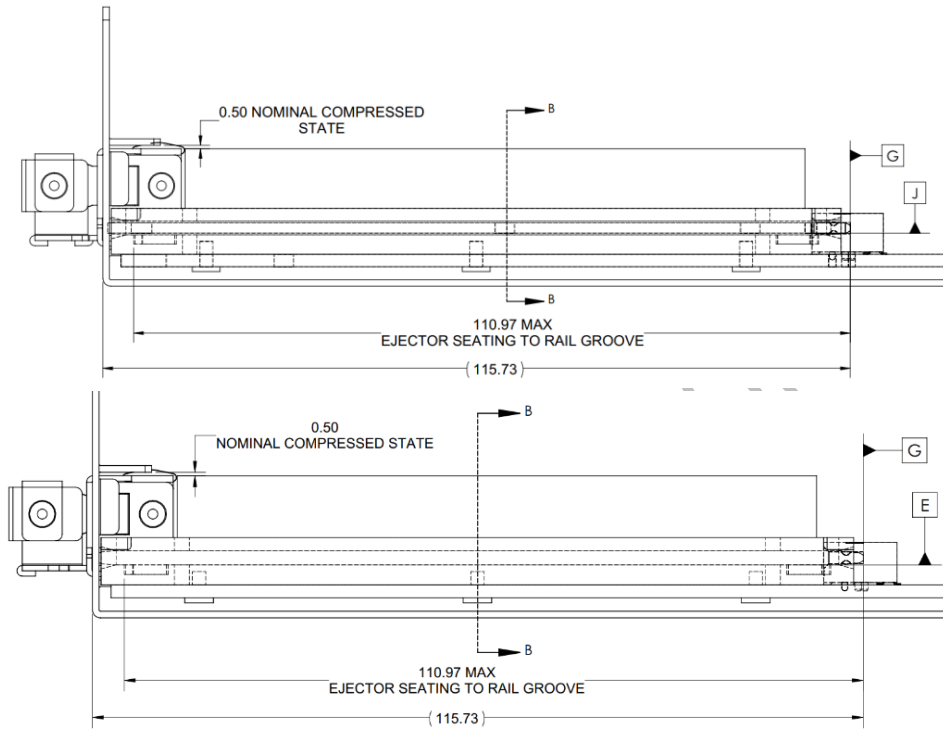
Figure 52: SFP Baseboard Chassis CTF Dimensions (Rear Rail Guide View)
