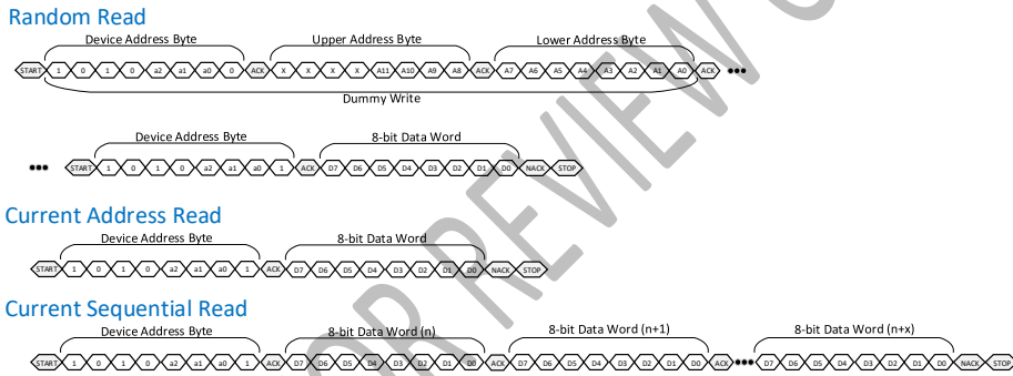
Figure 110: FRU EEPROM Reads with Double Byte Addressing
