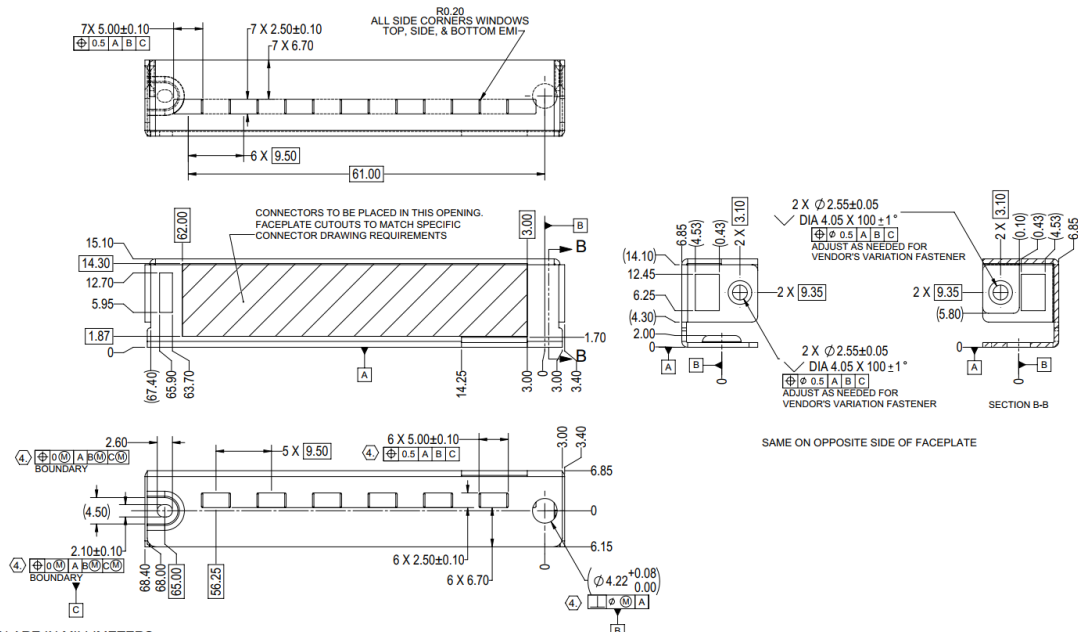
Figure 16: SFF Generic I/O Faceplate – Ejector Version (2D View)
