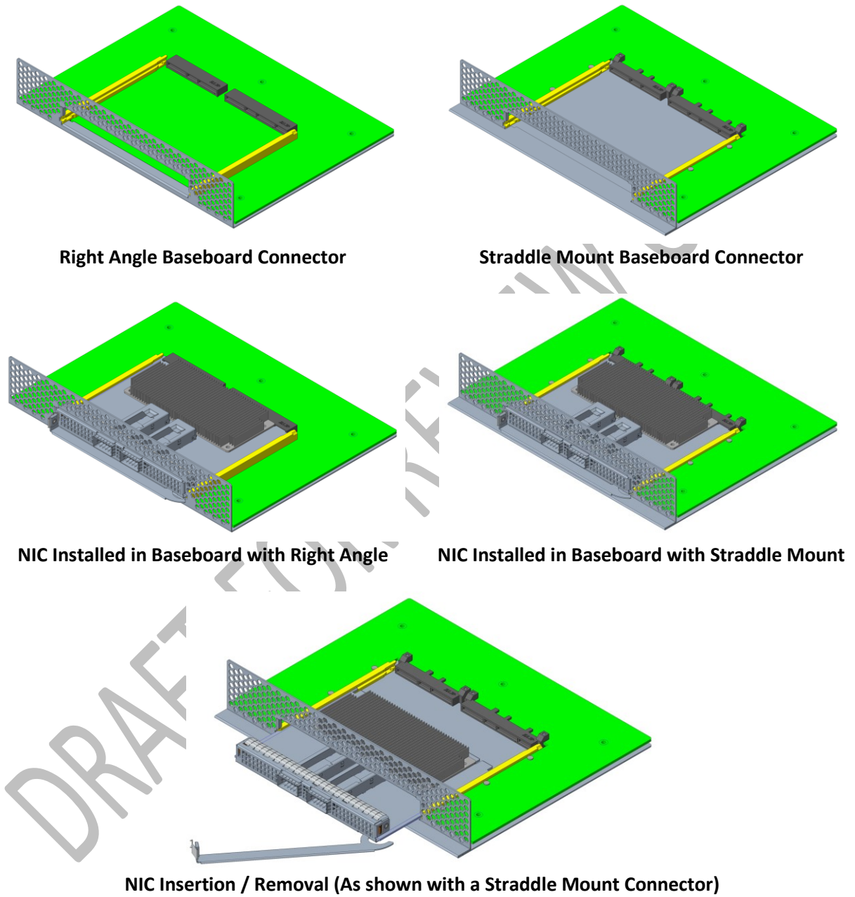
Figure 12: LFF NIC Chassis Mounted 3D Views
