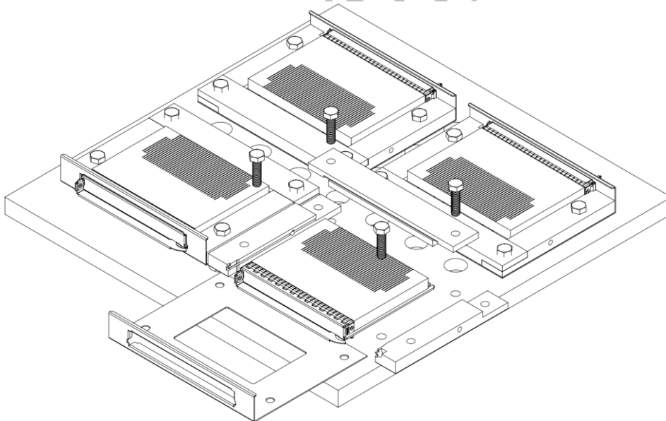
Figure 145: LFF Shock and Vibe Fixture
