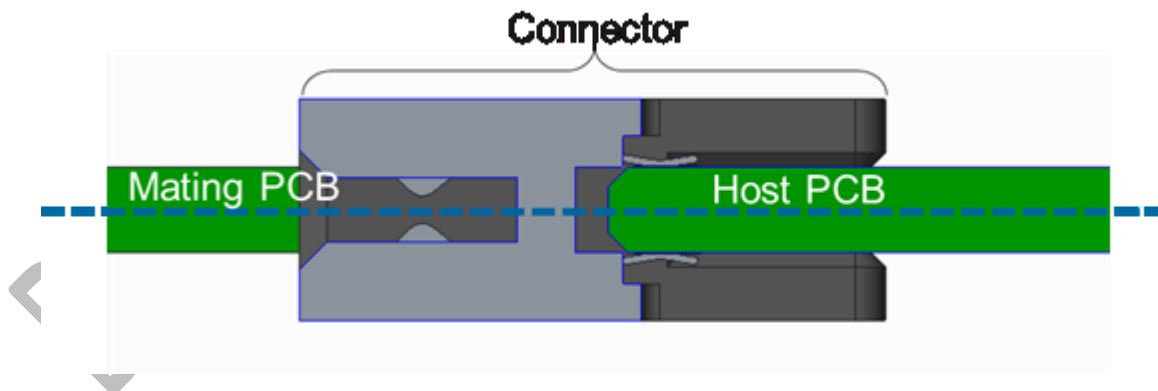
Figure 78: 0 mm Offset (Coplanar) for 0.062" Thick Baseboards
