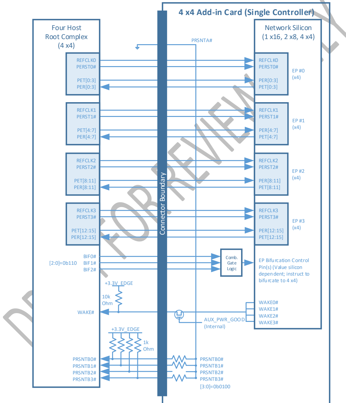
Figure 95: Quad Hosts (4 x4) and 4 x4 OCP NIC 3.0 Card (Single Controller)
