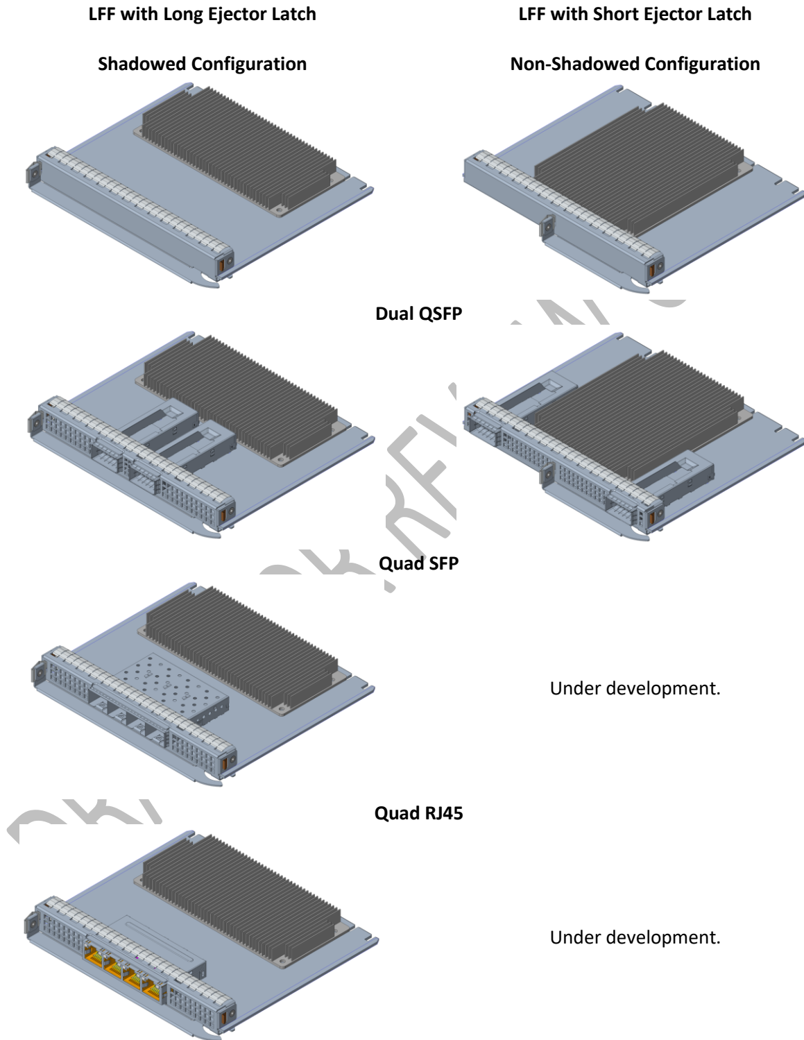
Figure 11: LFF NIC Line Side 3D Views
