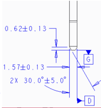
Figure 69: SFF Primary Connector Gold Finger - Detail D
