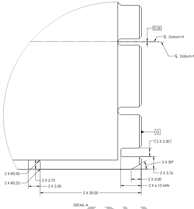
Figure 25: SFF Keep Out Zone – Top View – Detail A
