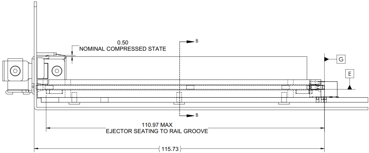
Figure 59: LFF Baseboard Chassis CTF Dimensions (Rail Guide View)
