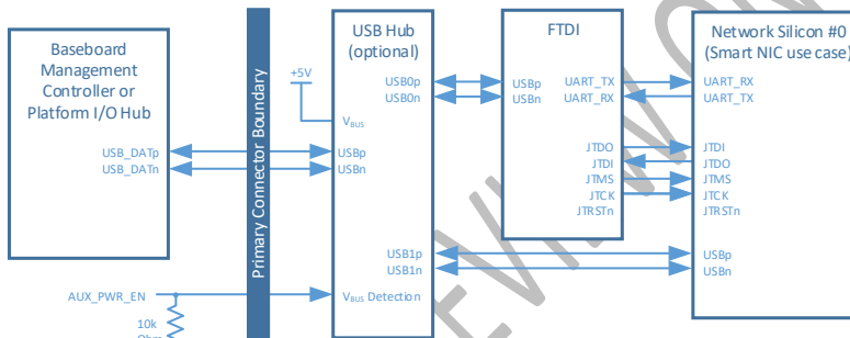
Figure 91: USB 2.0 Connection Example – USB-Serial / USB-JTAG Connectivity
