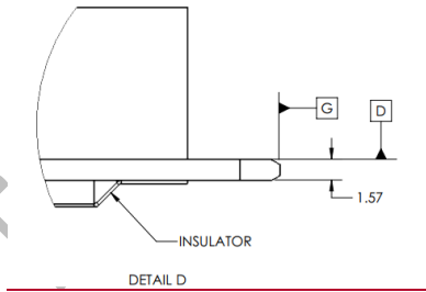
Figure 28: SFF Keep Out Zone – Side View – Detail D
