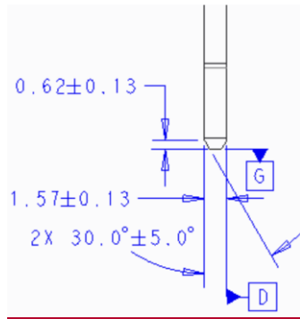
Figure 68: SFF Primary Connector Card Profile Dimensions
