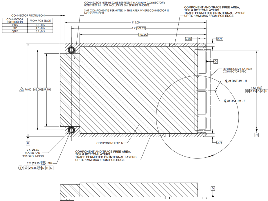
Figure 24: SFF Keep Out Zone – Top View
