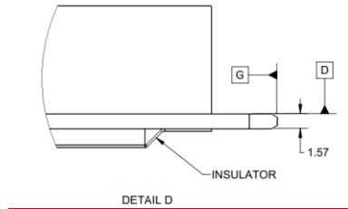
Figure 33: LFF Keep Out Zone – Side View – Detail D
