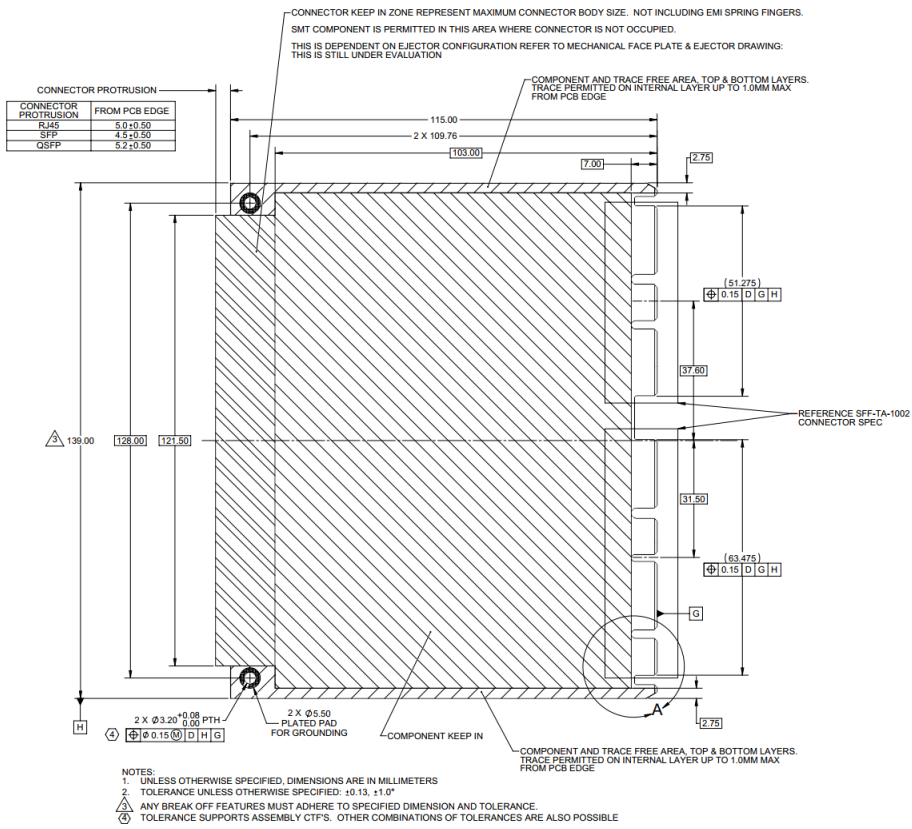
Figure 29: LFF Keep Out Zone – Top View
