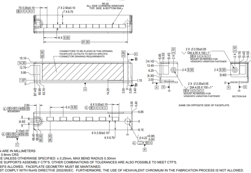
Figure 16: SFF Generic I/O Faceplate – Ejector Version (2D View)
