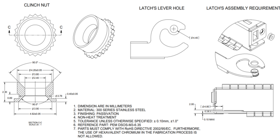
Figure 22: Clinch Nut Option A
