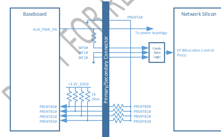
Figure 83: PCIe Present and Bifurcation Control Pins (Static BIF[0:2]#)
