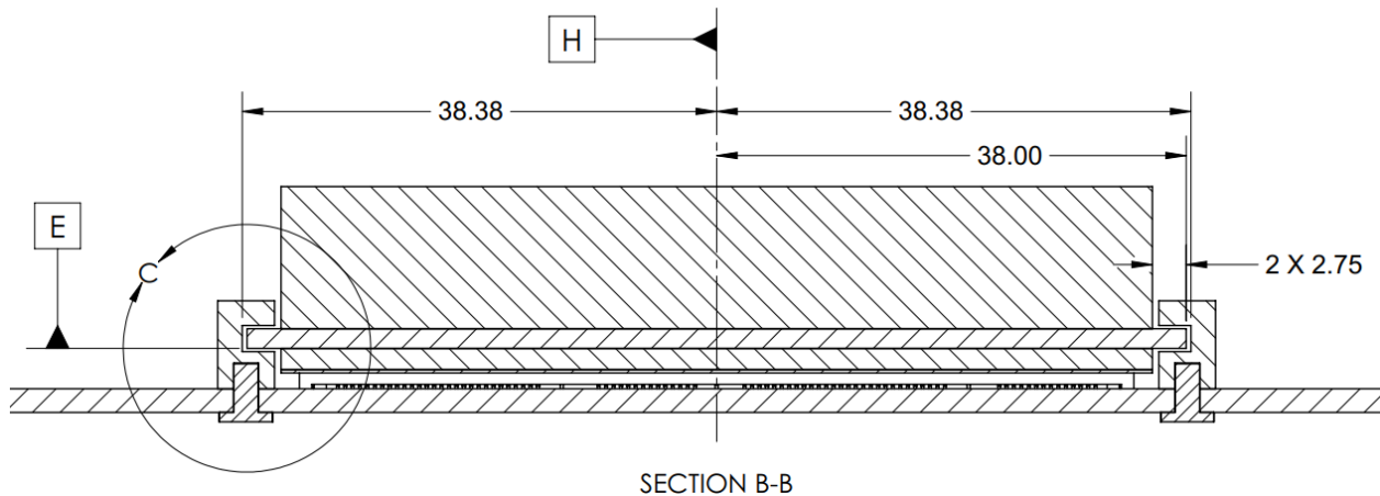
Figure 52: SFF Baseboard Chassis CTF Dimensions (Rear Rail Guide View)
