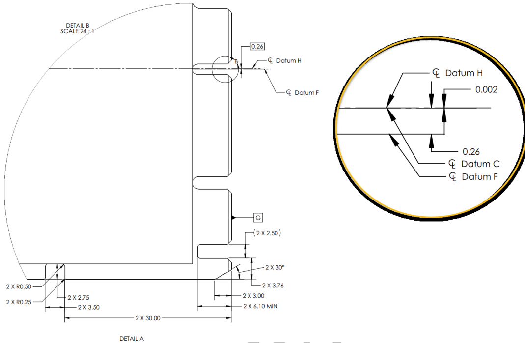
Figure 25: SFF Keep Out Zone – Top View – Detail A
