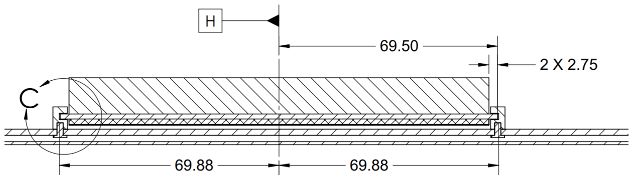
Figure 59: LFF Baseboard Chassis CTF Dimensions (Rail Guide View)
