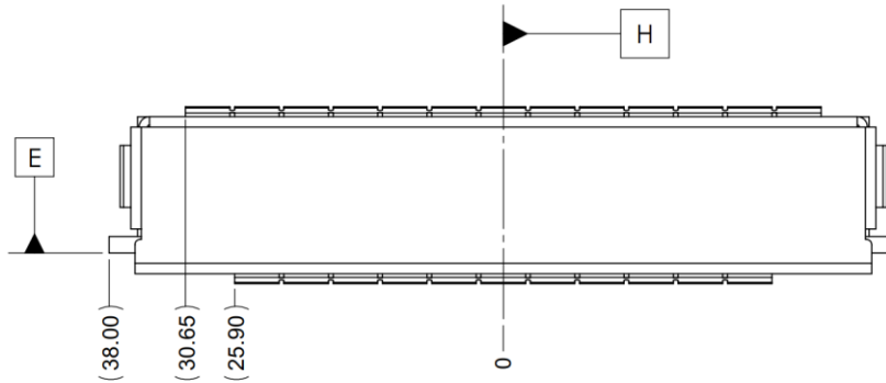
Figure 48: SFF OCP NIC 3.0 Card with Internal Lock CTF Dimensions (Side View)
