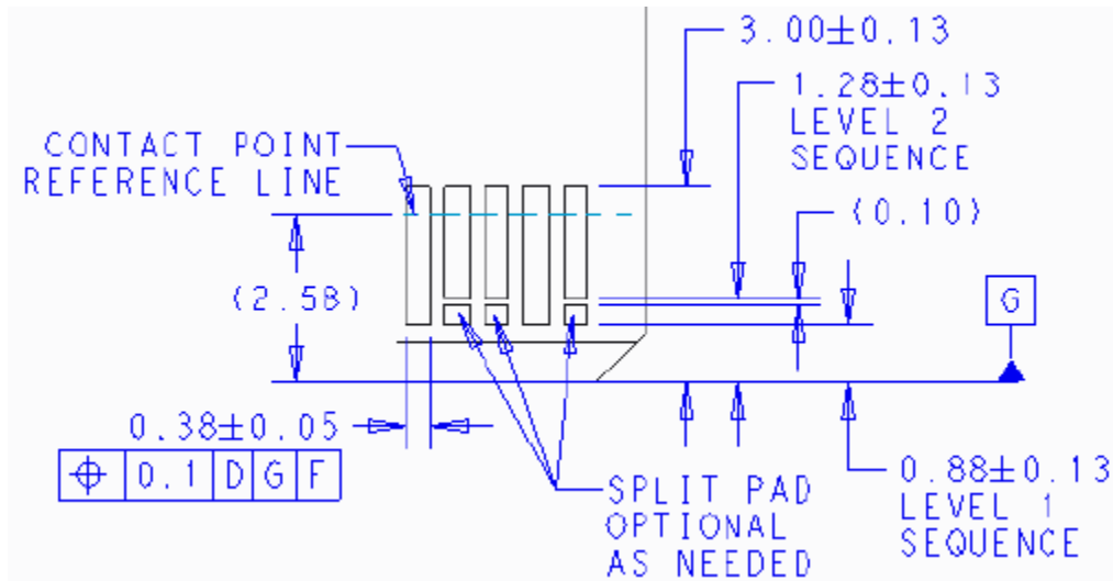
Figure 68: SFF Primary Connector Gold Finger - Detail D
