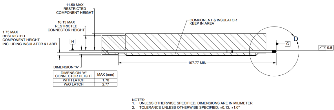
Figure 27: SFF Keep Out Zone – Side View
