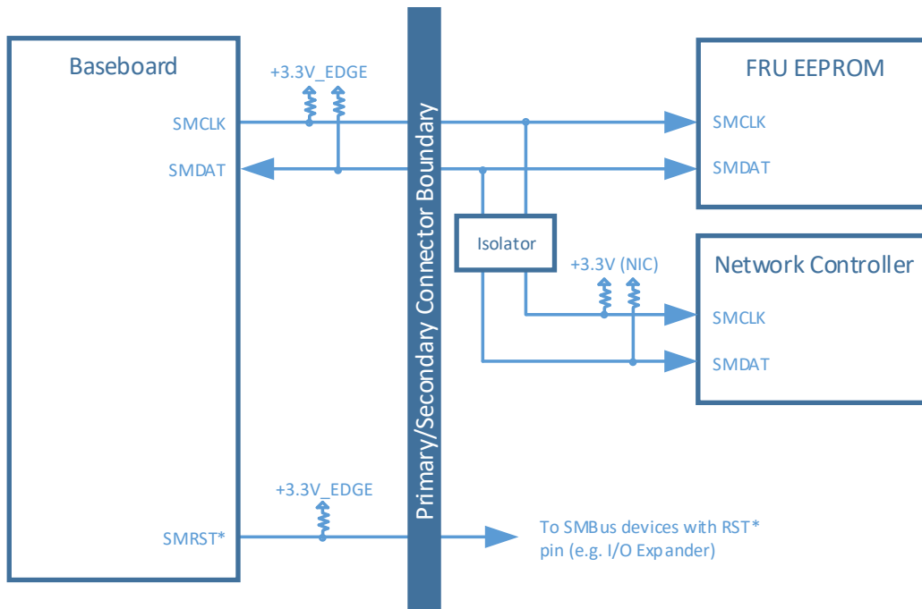
Figure 80: Example SMBus Connections
