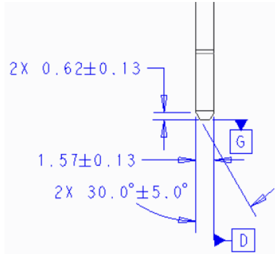
Figure 64: SFF Primary Connector Card Profile Dimensions
