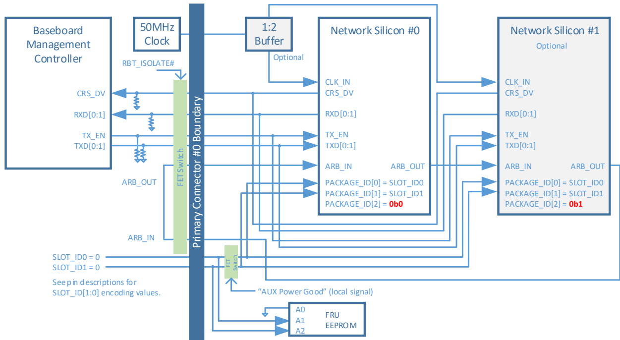
Figure 81: NC-SI over RBT Connection Example – Single Primary Connector
