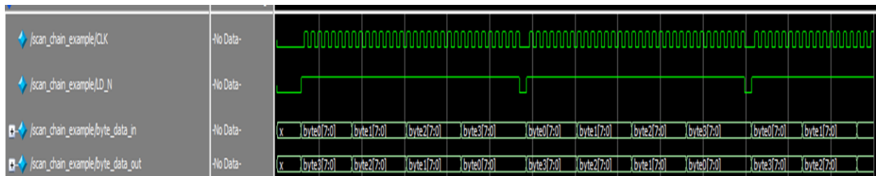
Figure 83: Example Scan Chain Timing Diagram
