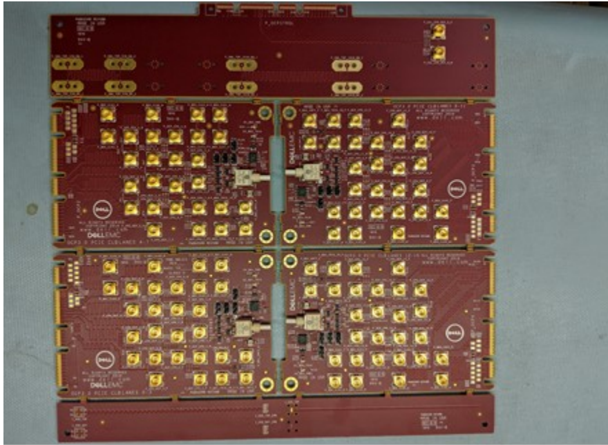
Figure 105: PCIe Load Board Test Fixture for OCP NIC 3.0 SFF
