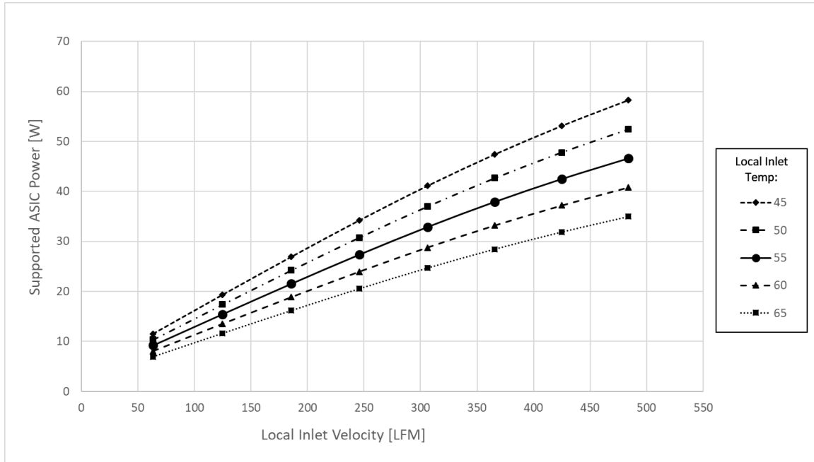
Figure 112: ASIC Supportable Power for Hot Aisle Cooling – LFF Card
