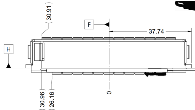
Figure 45: SFF OCP NIC 3.0 Card with Ejector CTF Dimensions (Side View)
