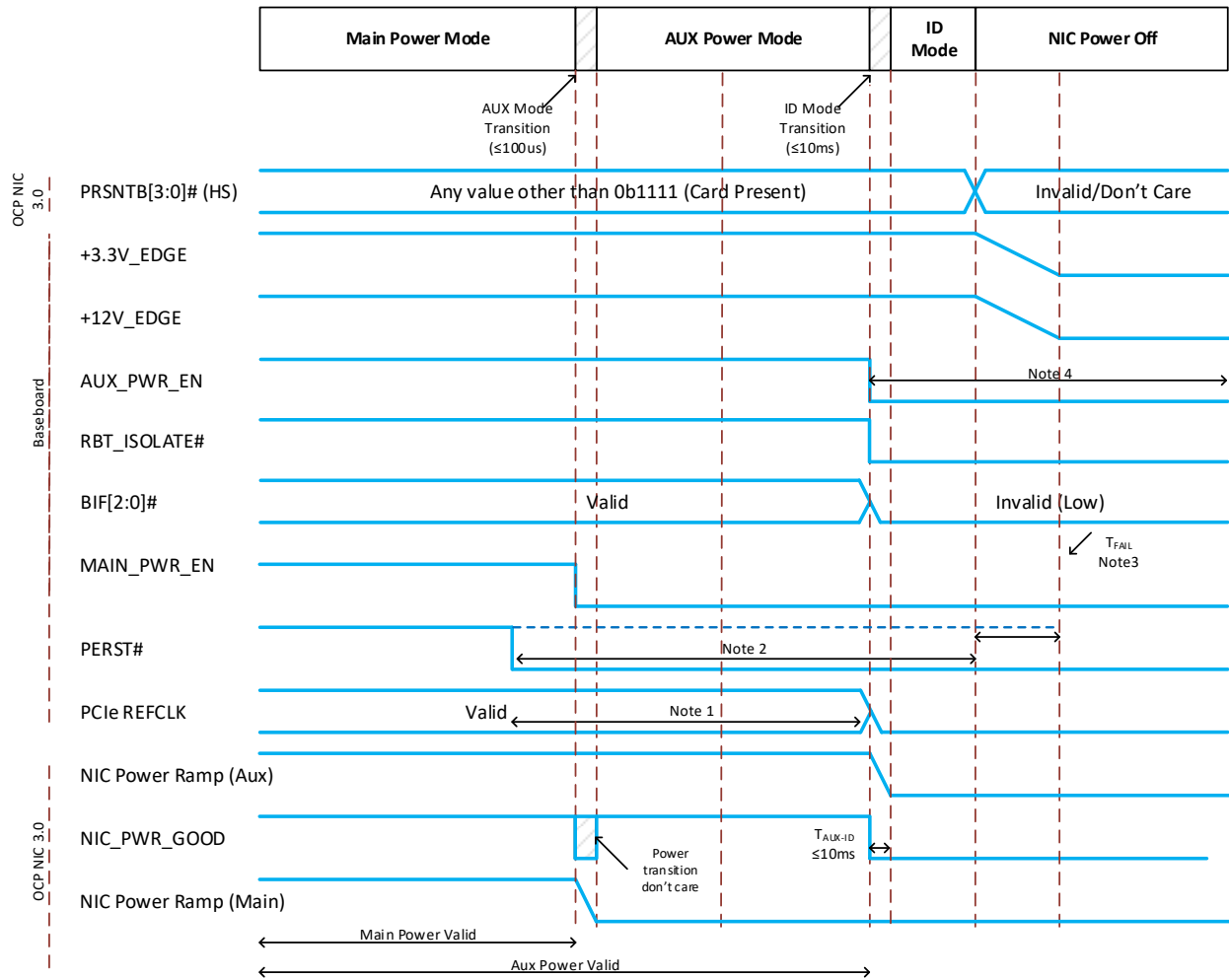
Figure 103: Power-Down Sequencing
