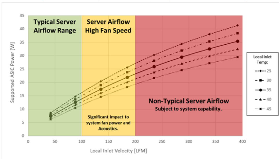
Figure 116: Server System Airflow Capability – SFF Cold Aisle Cooling
