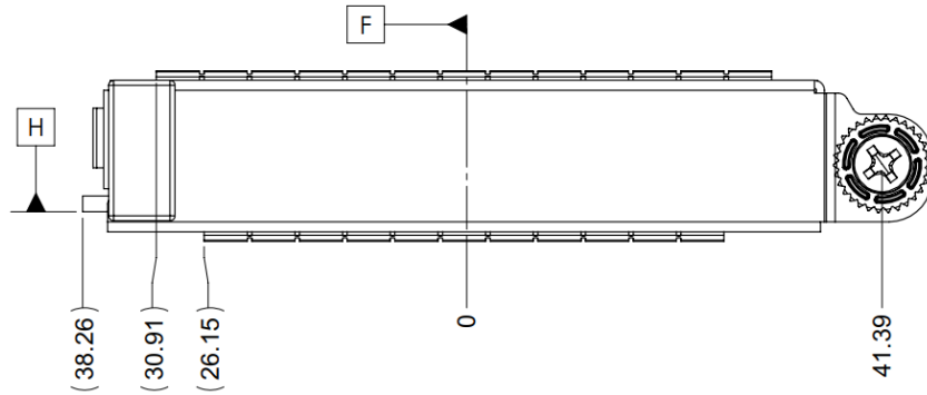
Figure 41: SFF OCP NIC 3.0 Card with Pull Tab CTF Dimensions (Front View)
