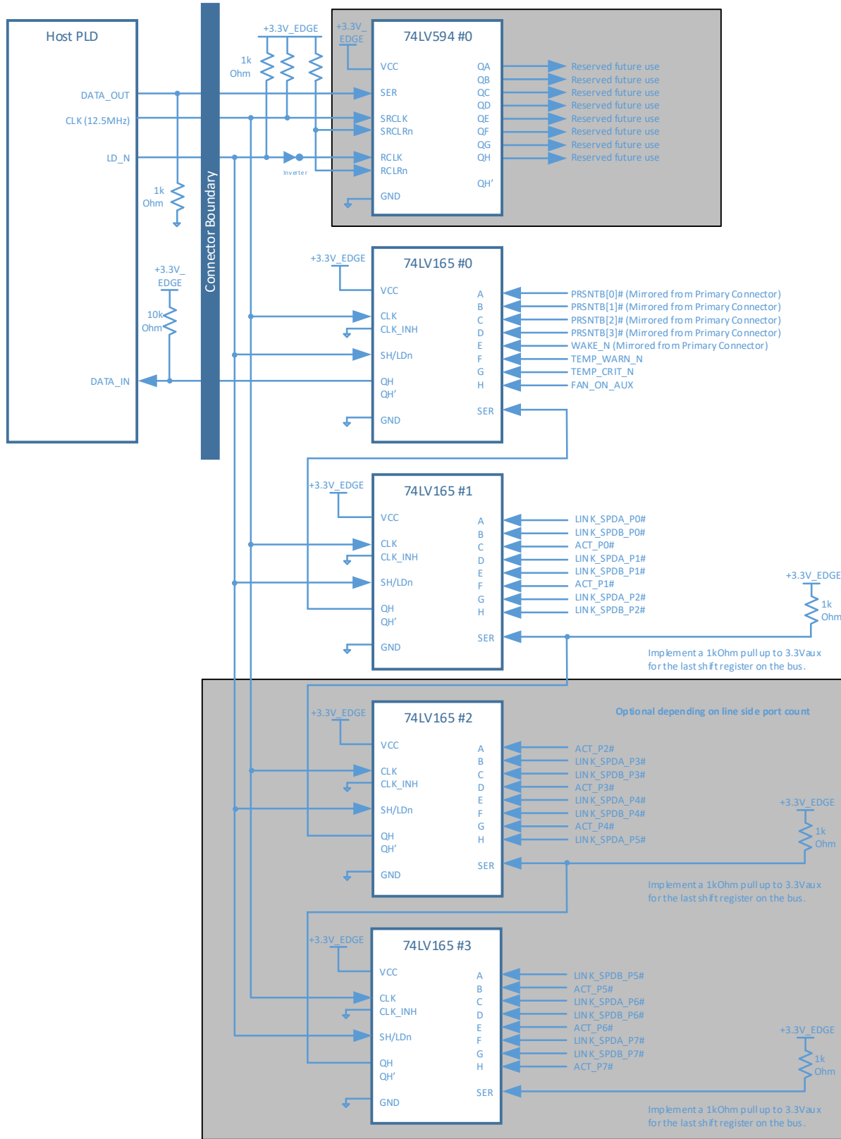
Figure 84: Scan Chain Connection Example
