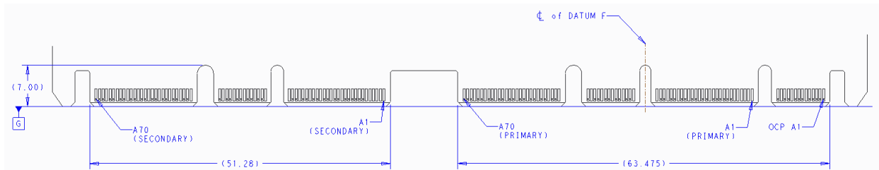
Figure 67: LFF Gold Finger Dimensions – x32 – Bottom Side (“A” Pins)
