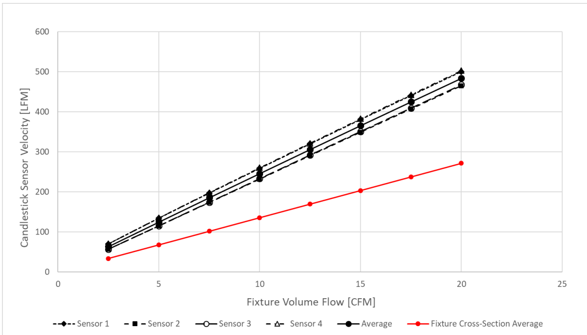
Figure 129: LFF Fixture, Hot Aisle Flow - Candlestick Air Velocity vs. Volume Flow
