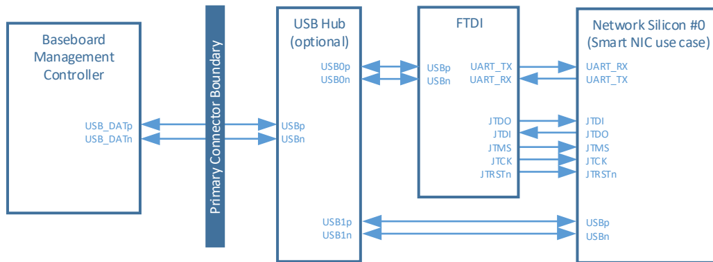
Figure 87: USB 2.0 Connection Example – USB-Serial / USB-JTAG Connectivity
