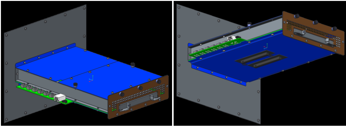
Figure 124: LFF Card Thermal Test Fixture Design
