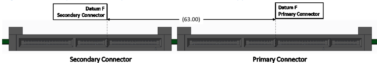
Figure 77: Primary and Secondary Connector Locations for LFF Support with Straddle Mount Connectors
