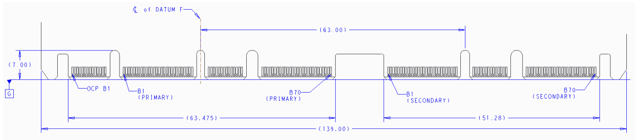
Figure 66: LFF Gold Finger Dimensions – x32 – Top Side (“B” Pins)
