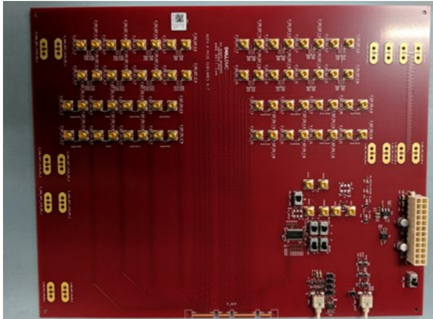
Figure 106: PCIe Base Board Test Fixture for OCP NIC 3.0 SFF
