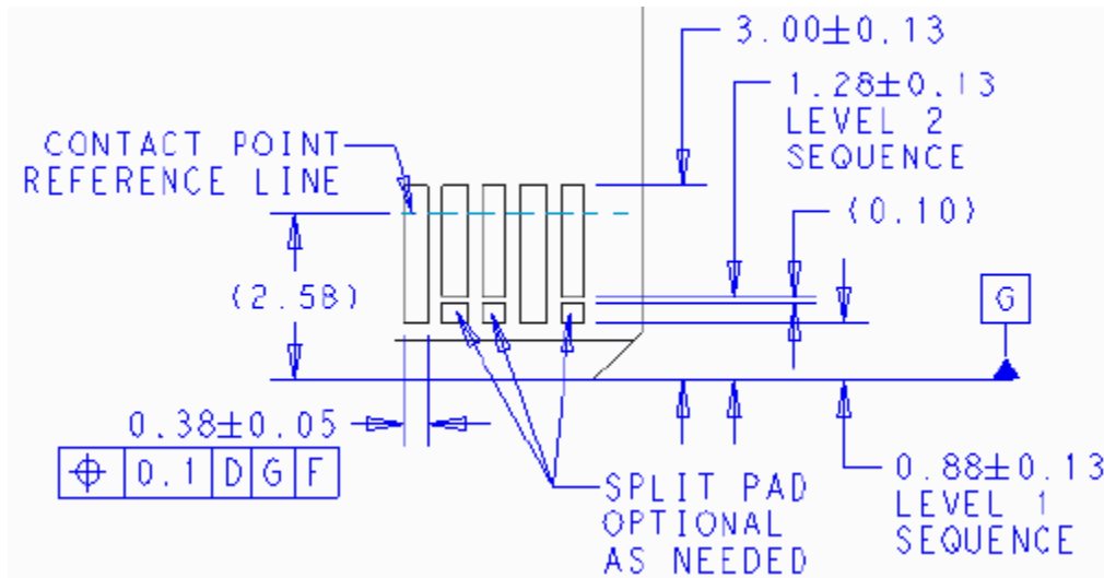
Figure 65: SFF Primary Conector Gold Finger - Detail D
