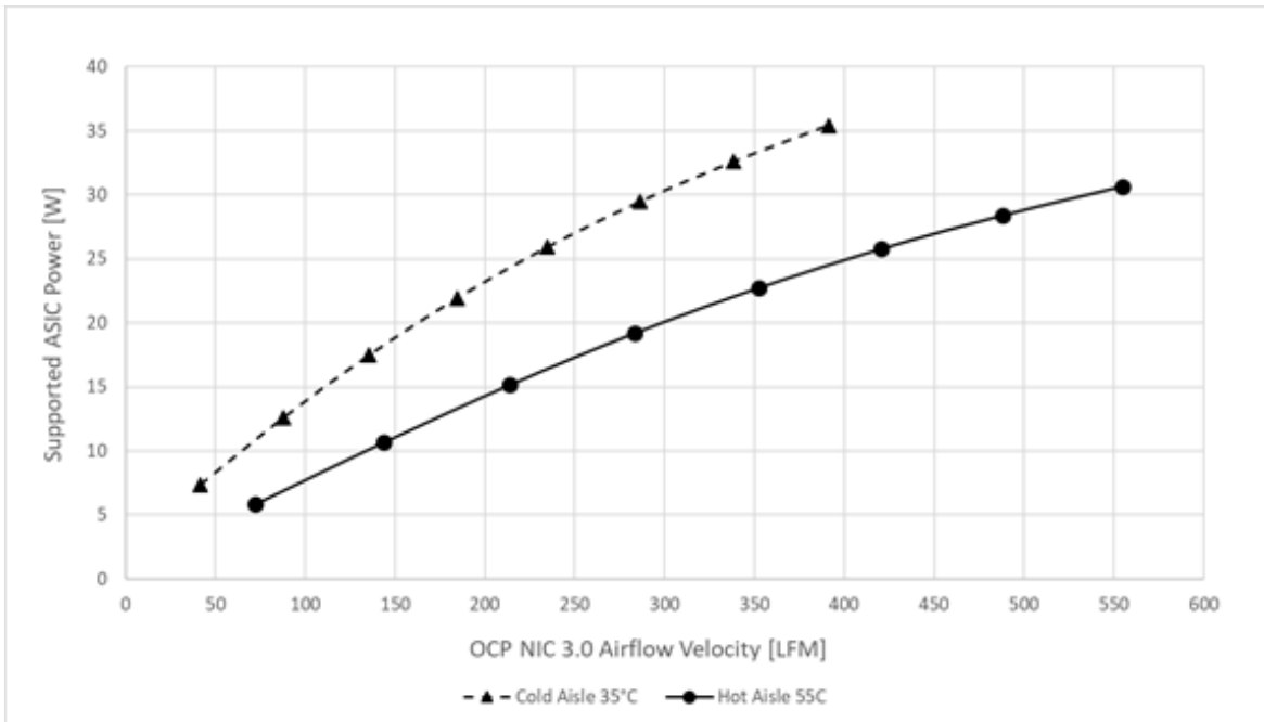
Figure 117: ASIC Supportable Power Comparison – SFF Card
