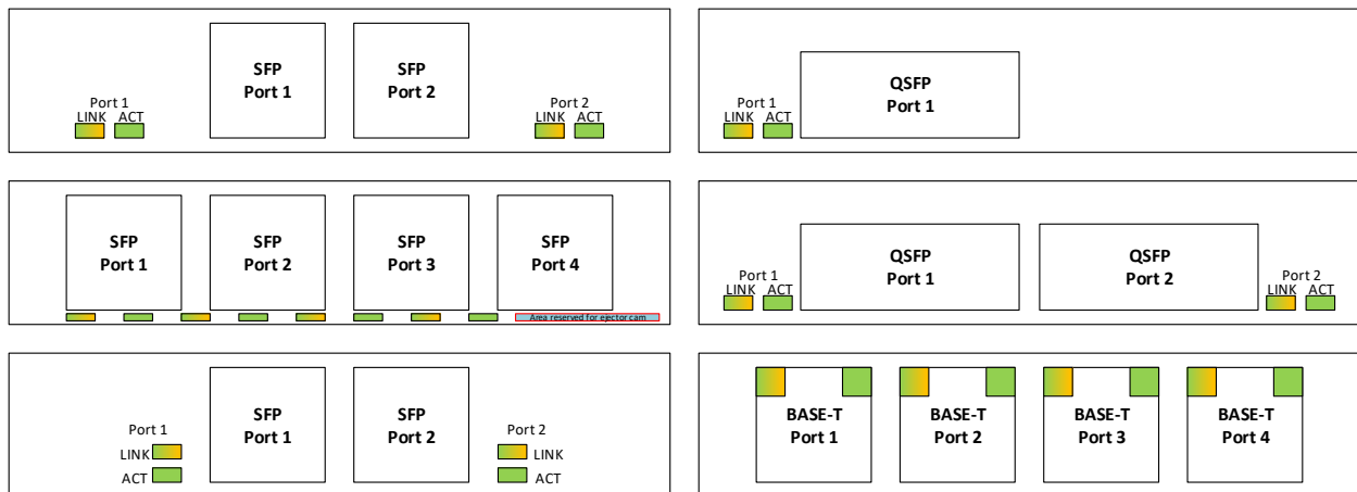
Figure 100: Port and LED Ordering – Example SFF Link/Activity and Speed LED Placement
