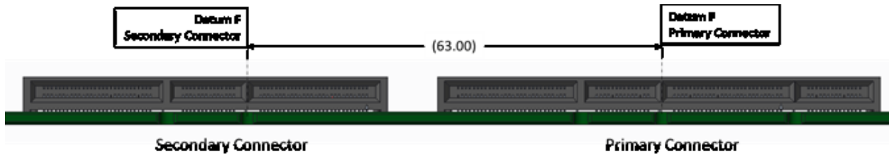
Figure 76: Primary and Secondary Connector Locations for LFF Support with Right Angle Connectors
