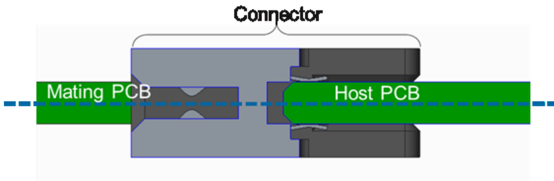
Figure 74: 0 mm Offset (Coplanar) for 0.062" Thick Baseboards
