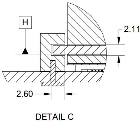
Figure 57: LFF Baseboard Chassis CTF Dimensions (Rail Guide – Detail C)
