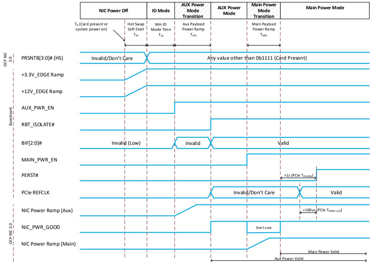
Figure 102: Power-Up Sequencing
