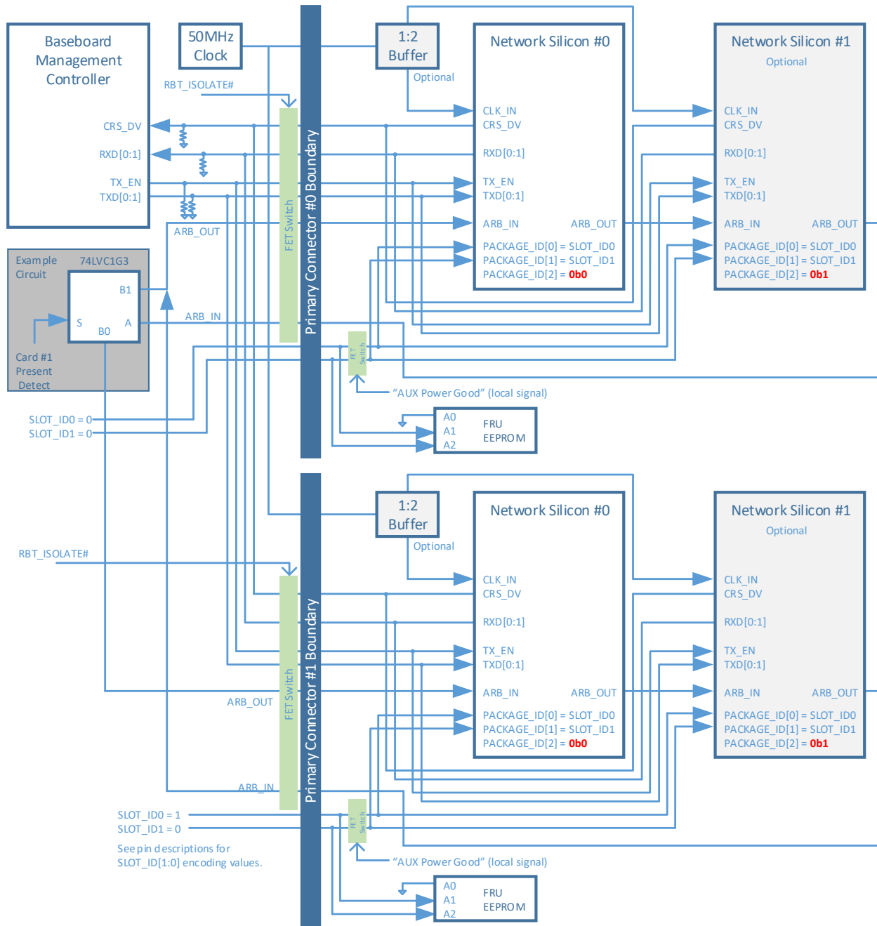
Figure 82: NC-SI over RBT Connection Example – Dual Primary Connectors
