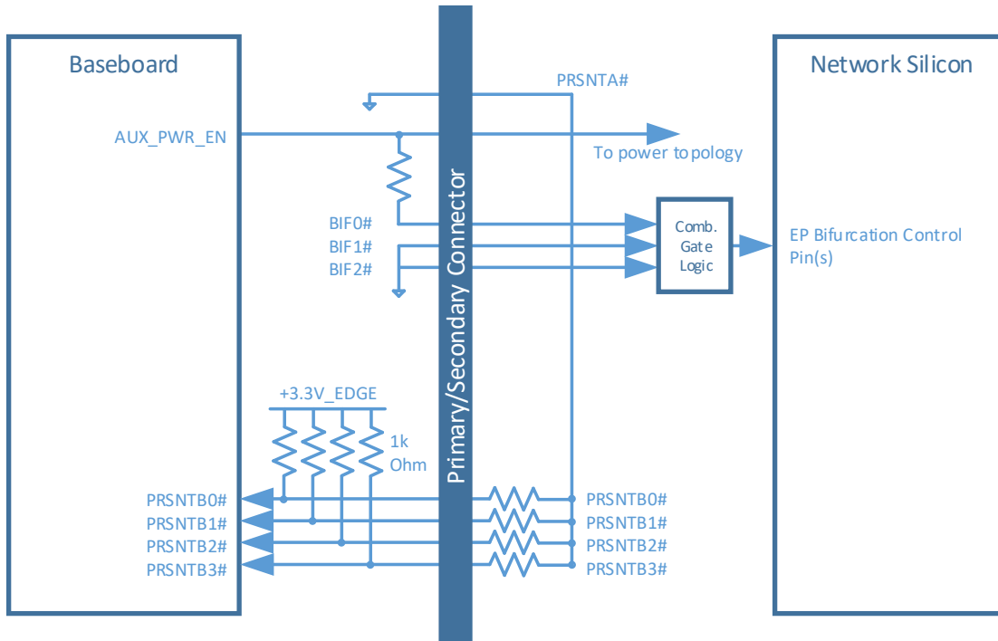
Figure 79: PCIe Present and Bifurcation Control Pins (Static BIF[0:2]#)
