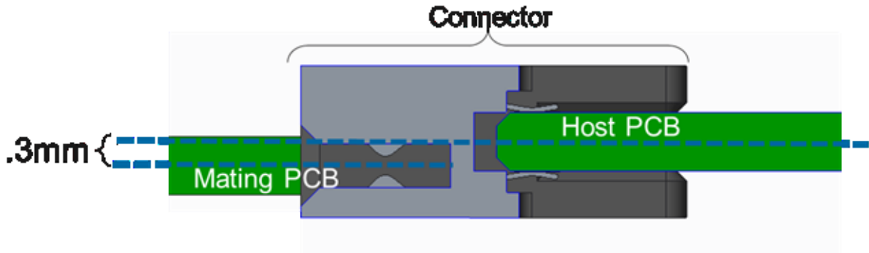
Figure 75: 0.3 mm Offset for 0.076" Thick Baseboards
