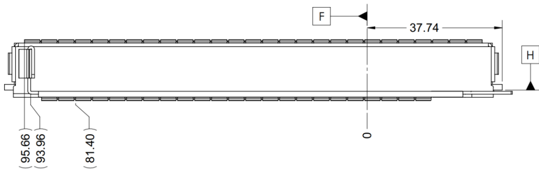
Figure 52: LFF OCP NIC 3.0 Card with Ejector CTF Dimensions (Front View)
