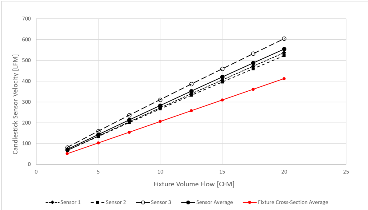
Figure 128: SFF Fixture, Hot Aisle Flow - Candlestick Air Velocity vs. Volume Flow
