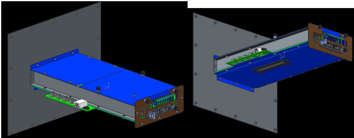
Figure 121: SFF Thermal Test Fixture Preliminary Design
