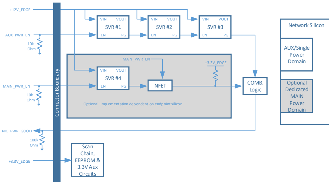
Figure 85: Example Power Supply Topology
