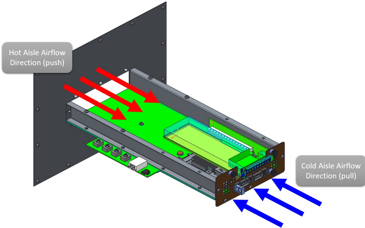
Figure 127: Thermal Test Fixture Airflow Direction
