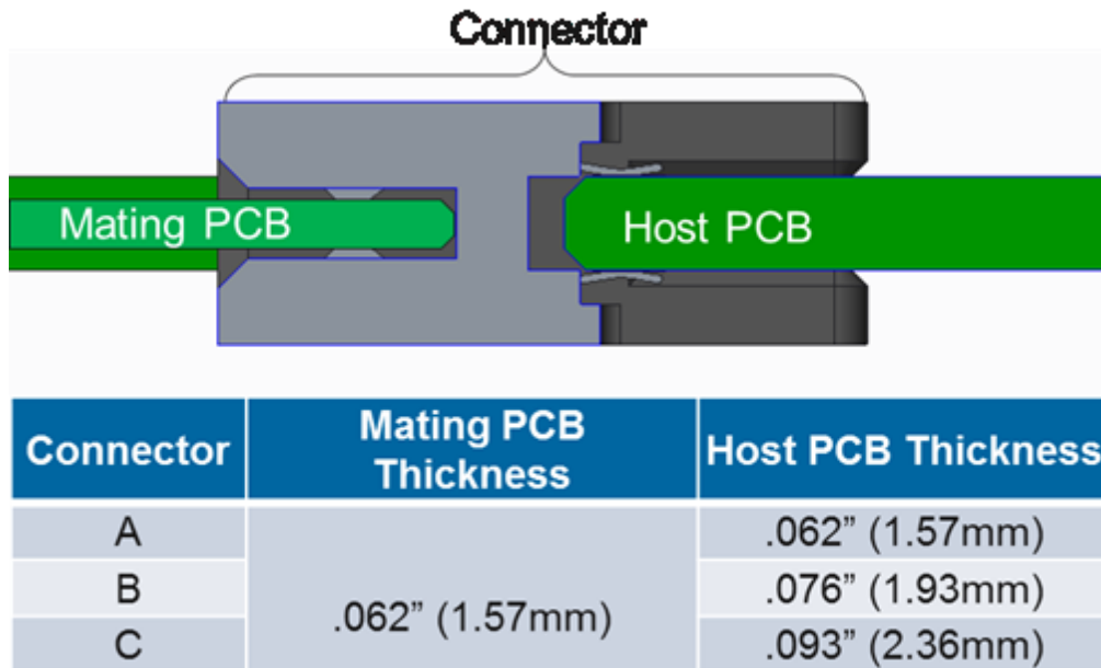
Figure 73: OCP NIC 3.0 Card and Baseboard PCB Thickness Options for Straddle Mount Connectors
