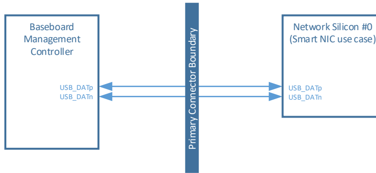
Figure 86: USB 2.0 Connection Example – Basic Connectivity
