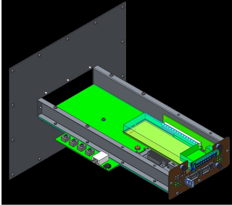
Figure 122: SFF Thermal Test Fixture Preliminary Design – Cover Removed
