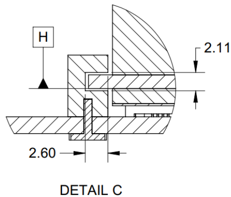
Figure 50: SFF Baseboard Chassis CTF Dimensions (Rail Guide Detail) – Detail C
