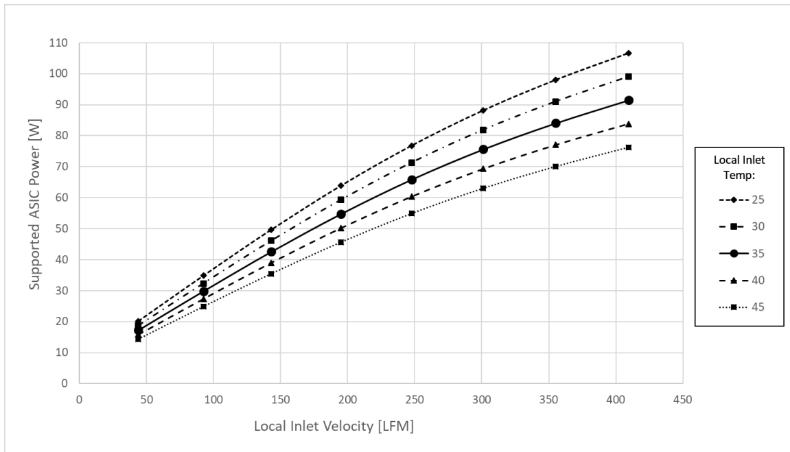
Figure 118: ASIC Supportable Power for Cold Aisle Cooling – LFF Card
