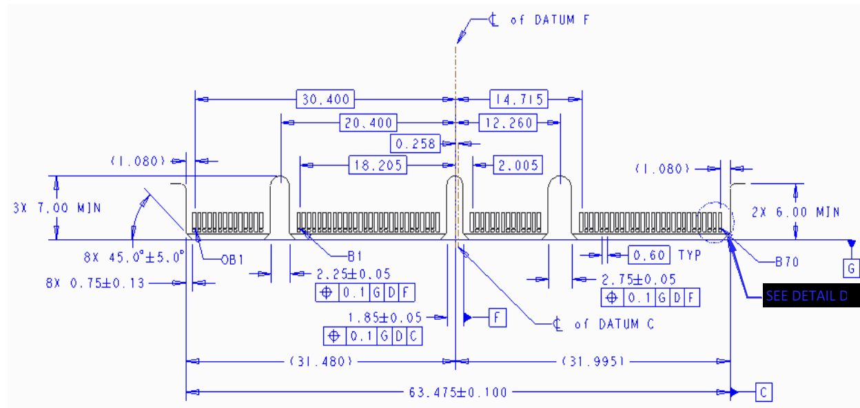
Figure 63: SFF Primary Connector Gold Finger Dimensions – x16 – Top Side (“B” Pins)
