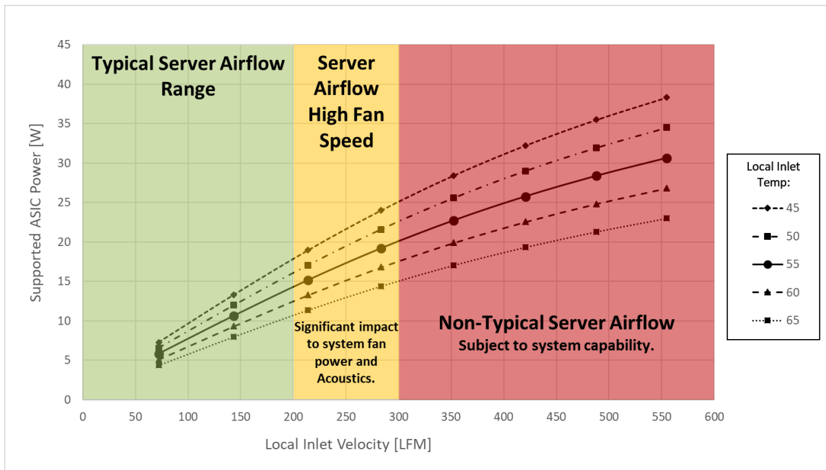
Figure 111: Server System Airflow Capability – SFF Card Hot Aisle Cooling
