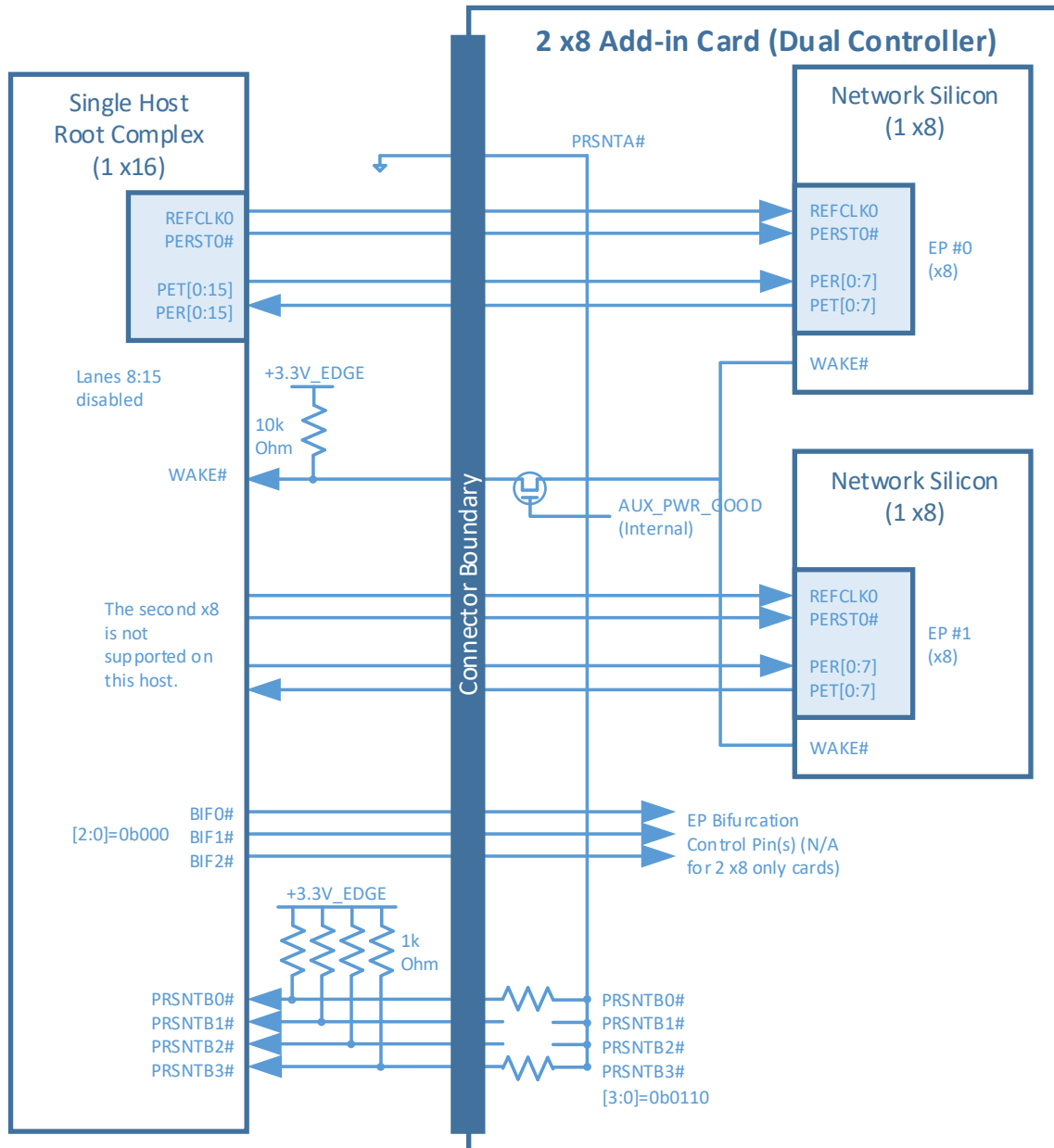
Figure 93: Single Host with no Bifurcation (1 x16) and 2 x8 OCP NIC 3.0 Card (Dual Controllers)
