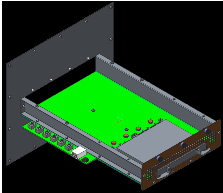
Figure 125: LFF Card Thermal Test Fixture Design – Cover Removed
