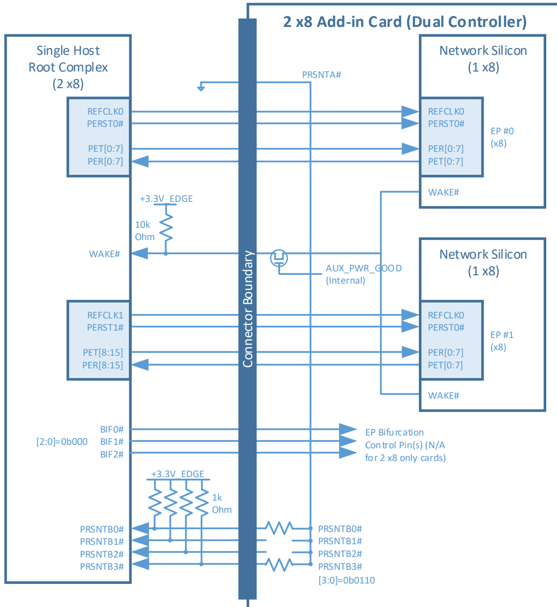
Figure 90: Single Host (2 x8) and 2 x8 OCP NIC 3.0 Card (Dual Controllers)
