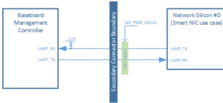
Figure 88: UART Connection Example
