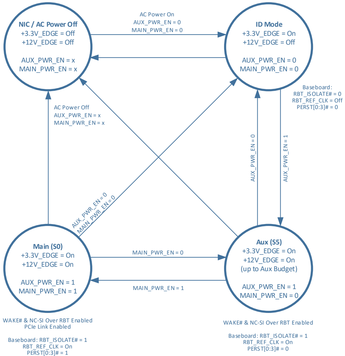
Figure 101: Baseboard Power States
