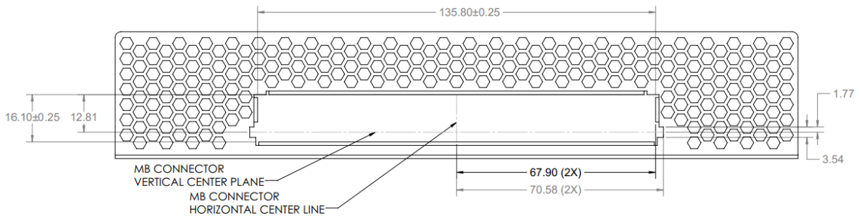
Figure 54: LFF Baseboard Chassis CTF Dimensions (Rear View)
