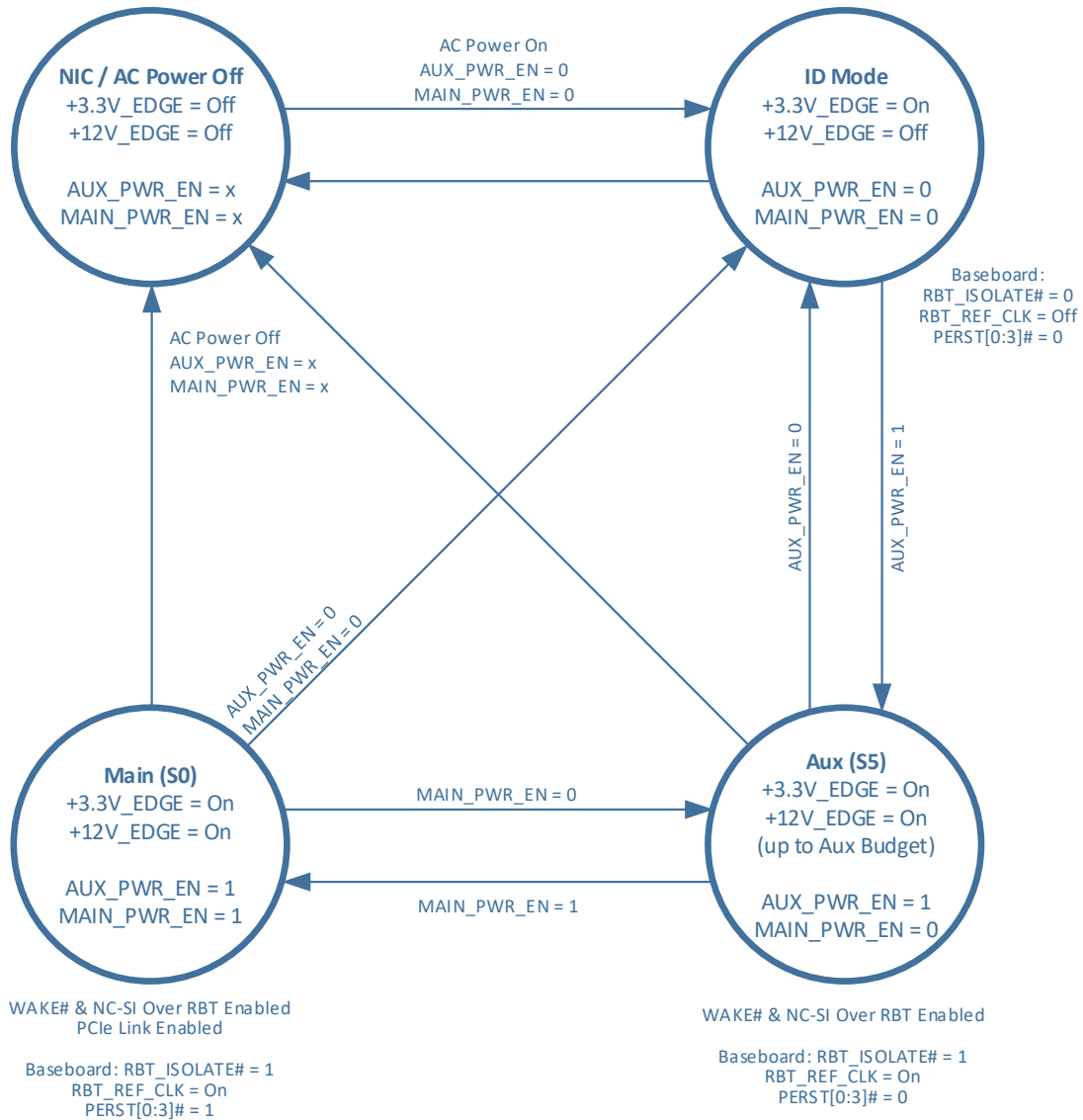
Figure 101: Baseboard Power States
