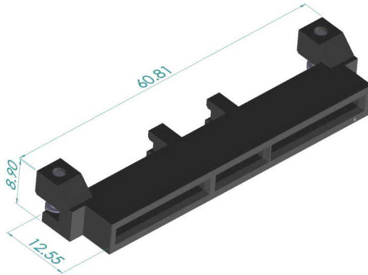
Figure 72: 140-pin Base Board Secondary Connector – Straddle Mount
