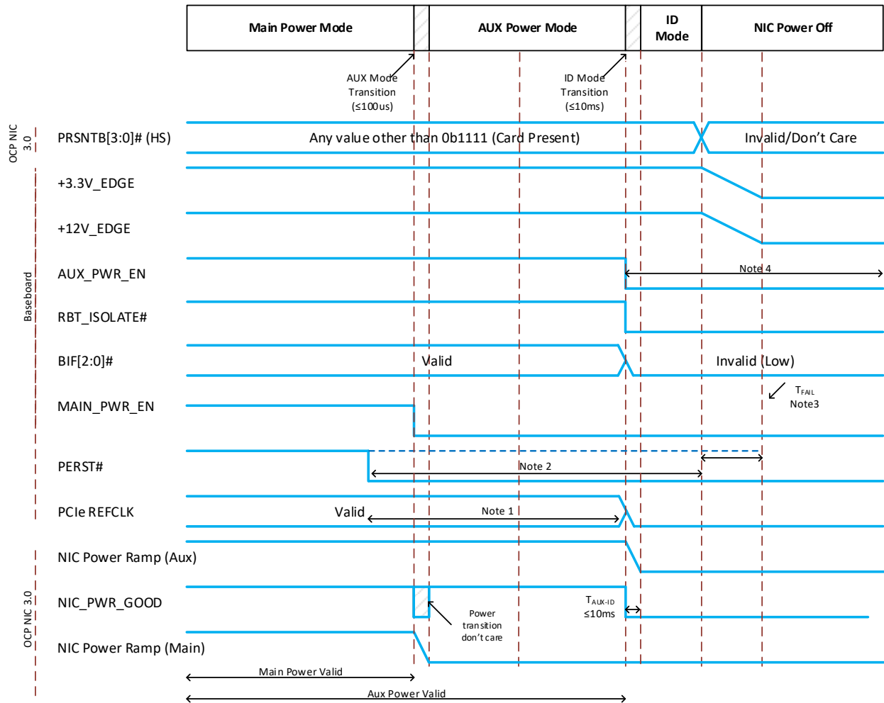
Figure 103: Power-Down Sequencing
