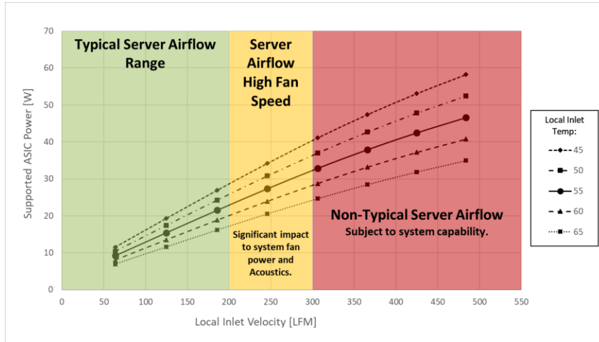
Figure 114105 : Server System Airflow Capability – LFF Card Hot Aisle Cooling
