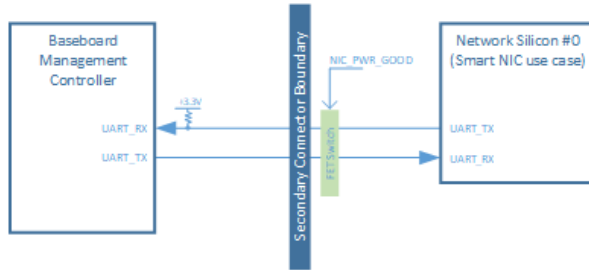
Figure 8884 : UART Connection Example
