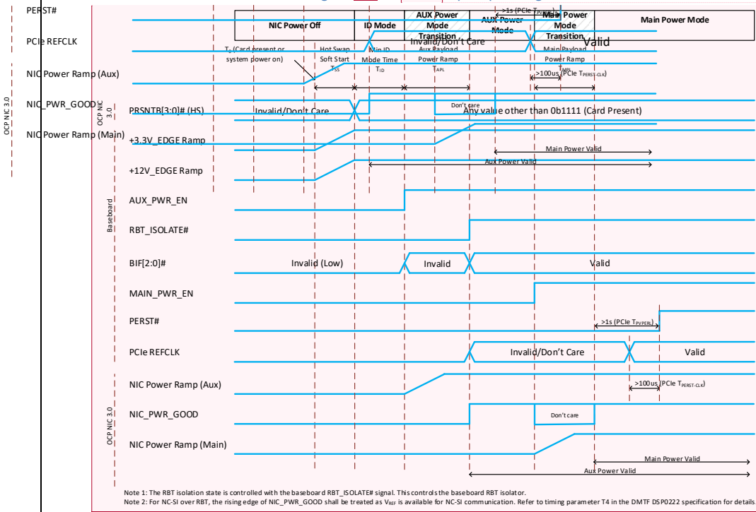
Figure 10294: Power-Up Sequencing
