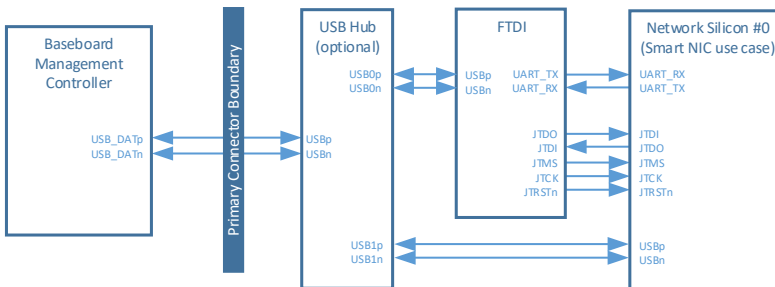
Figure 8783 : USB 2.0 Connection Example – USB-Serial / USB-JTAG Connectivity
