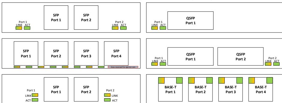
Figure 10092 : Port and LED Ordering – Example SFF Link/Activity and Speed LED Placement
