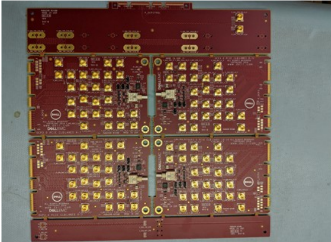
Figure 10596 : PCIe Load Board Test Fixture for OCP NIC 3.0 SFF
