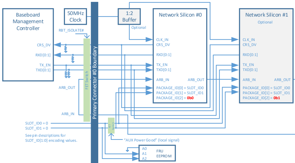
Figure 8177: NC-SI Over-over RBT Connection Example – Single Primary Connector
