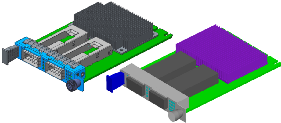
Figure 110491 : OCP NIC 3.0 SFF Reference Design and CFD Geometry
