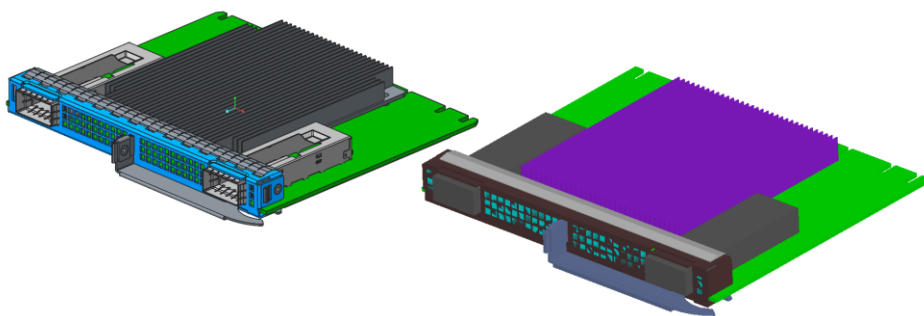
Figure 113 104 : OCP NIC 3.0 LFF Reference Design and CFD Geometry
