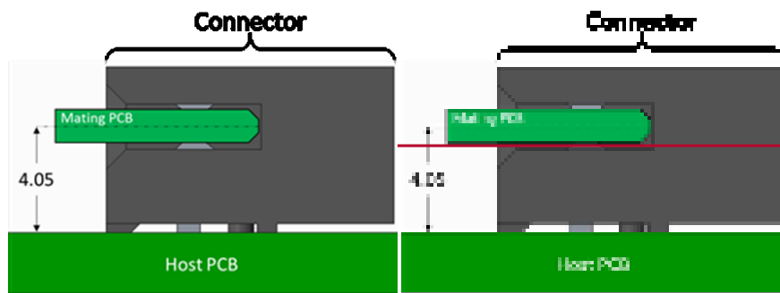
Figure 7066 : OCP NIC 3.0 Card and Host Offset for Right Angle Connectors
