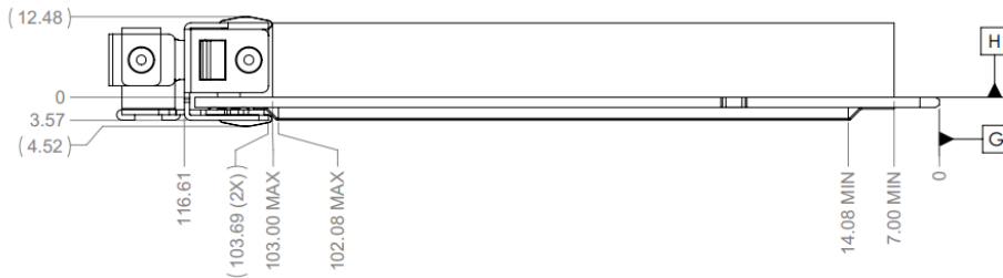
Figure 4543 : SFF OCP NIC 3.0 Card with Ejector CTF Dimensions (Side View)
