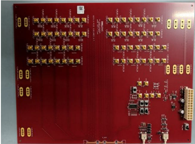
Figure 10697 : PCIe Base Board Test Fixture for OCP NIC 3.0 SFF
