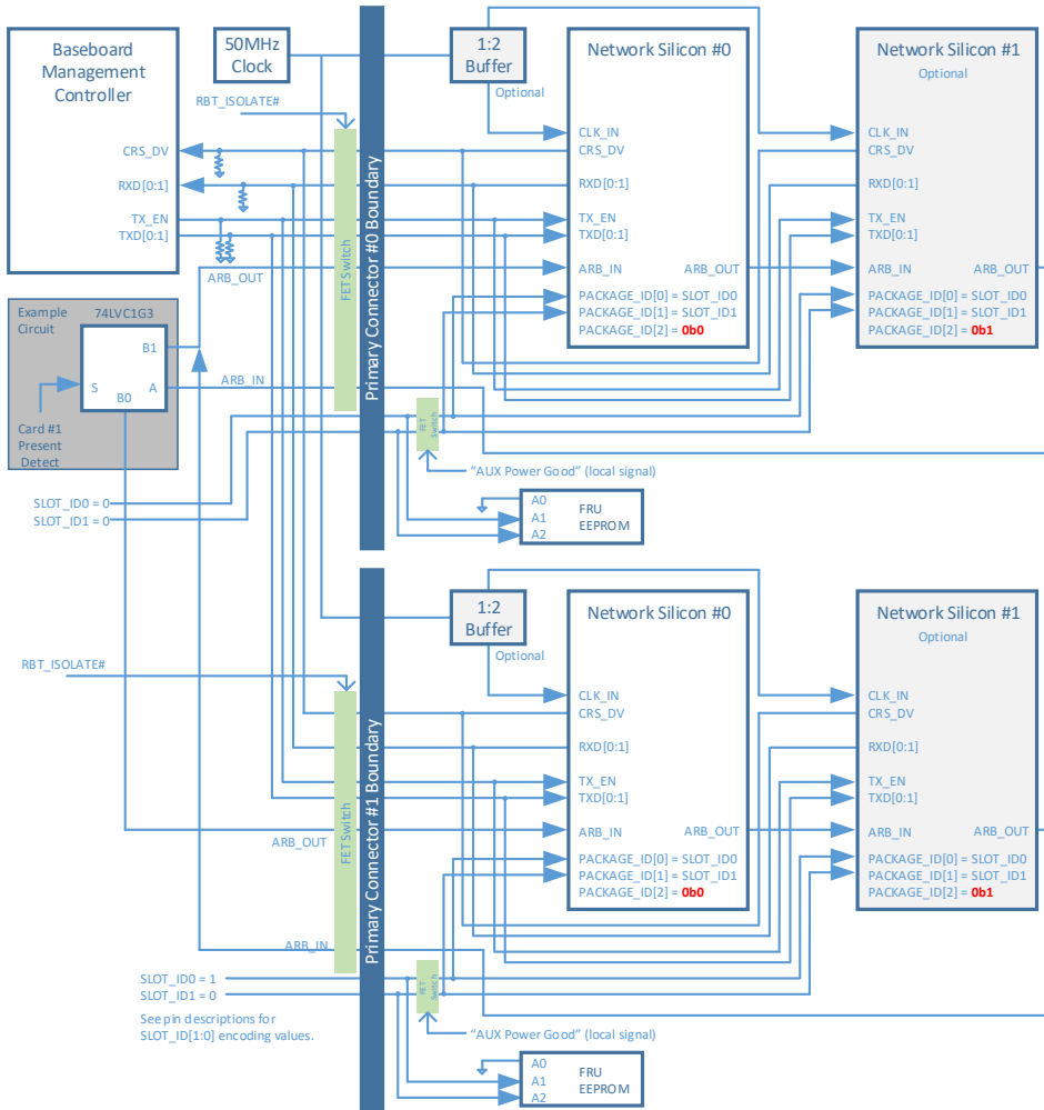
Figure 8278: NC-SI Over-over RBT Connection Example – Dual Primary Connectors
