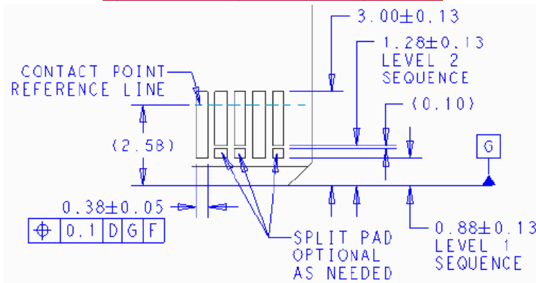
Figure 65: SFF Primary Connector Gold Finger - Detail D
