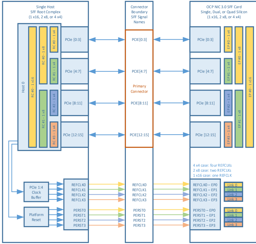
Figure 94: SFF PCIe REFCLK Mapping – Single Host – 1, 2 and 4 links
