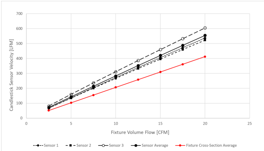
Figure 128119 : SFF Fixture, Hot Aisle Flow - Candlestick Air Velocity vs. Volume Flow
