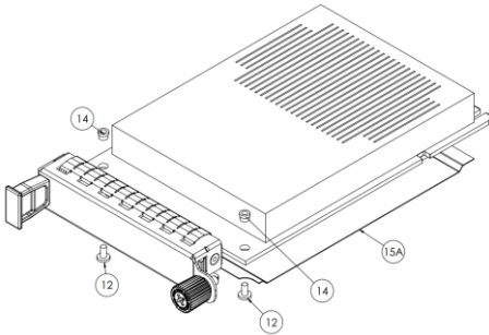
Small Form Factor (SFF) with Pull Tab
