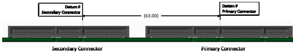
Figure 7672 : Primary and Secondary Connector Locations for LFF Support with Right Angle Connectors
