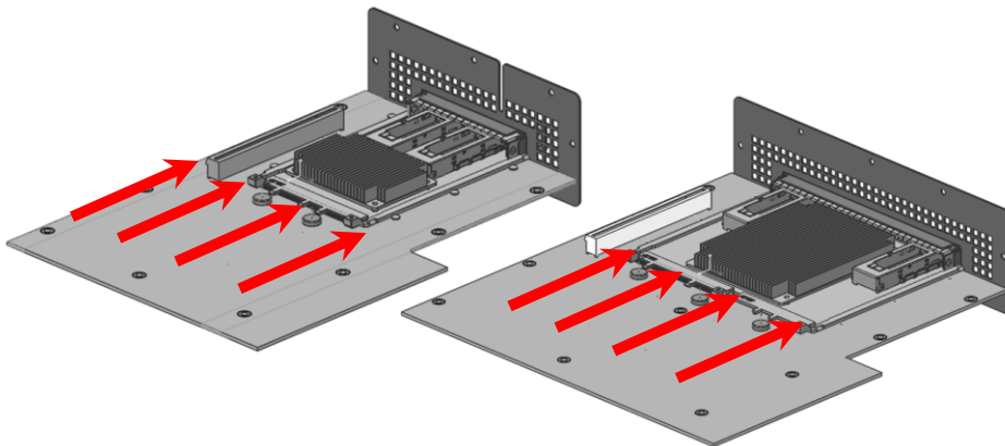
Figure 10798 : Airflow Direction for Hot Aisle Cooling (SFF and LFF)
