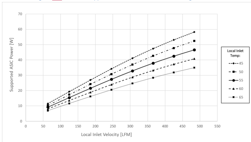
Figure 112 103 : ASIC Supportable Power for Hot Aisle Cooling – LFF Card
