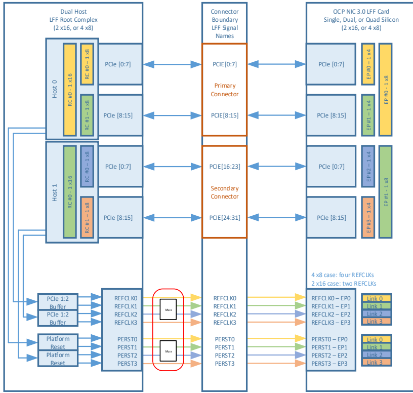
Figure 98: LFF PCIe REFCLK Mapping – Dual Host – 2 and 4 links
