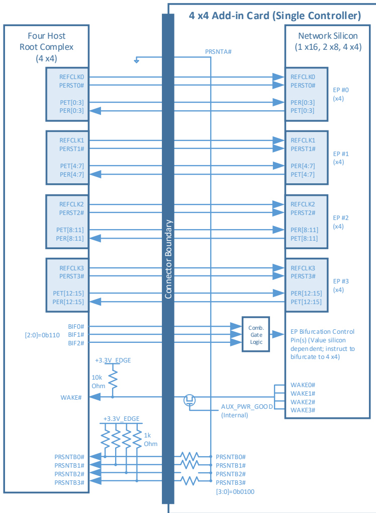
Figure 9187: Quad Hosts (4 x4) and 4 x4 OCP NIC 3.0 Card (Single Controller)
