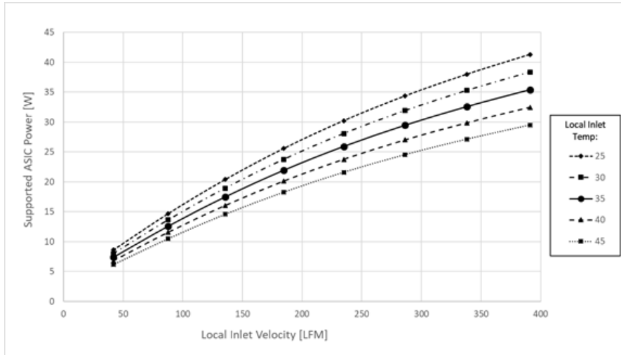
Figure 115106: ASIC Supportable Power for Cold Aisle Cooling – SFF Card
