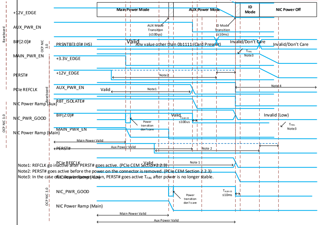
Figure 10395: Power-Down Sequencing
