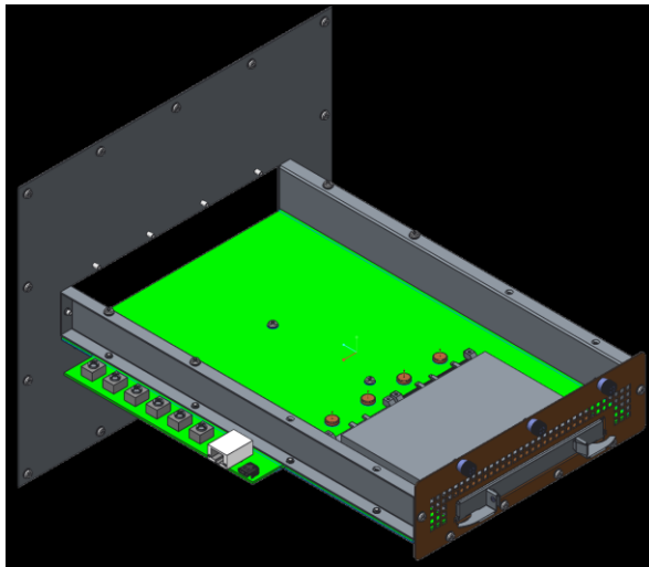
Figure 126 117 : LFF Card Thermal Test Fixture PCB
