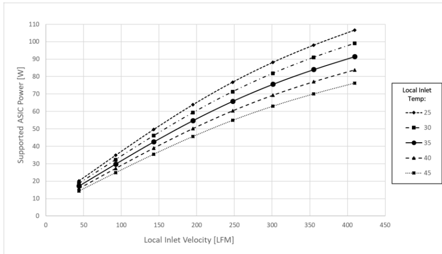
Figure 118 109 : ASIC Supportable Power for Cold Aisle Cooling – LFF Card
