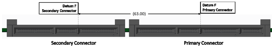
Figure 7773 : Primary and Secondary Connector Locations for LFF Support with Straddle Mount
