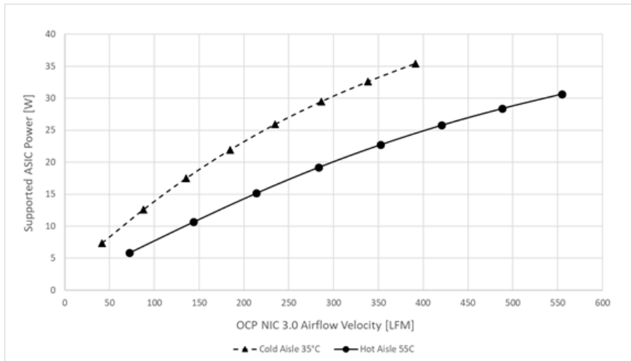
Figure 117 108 : ASIC Supportable Power Comparison – SFF Card
