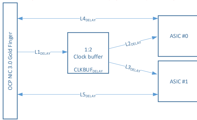
Figure 104: NC-SI over RBT Propagation Delay Matching
