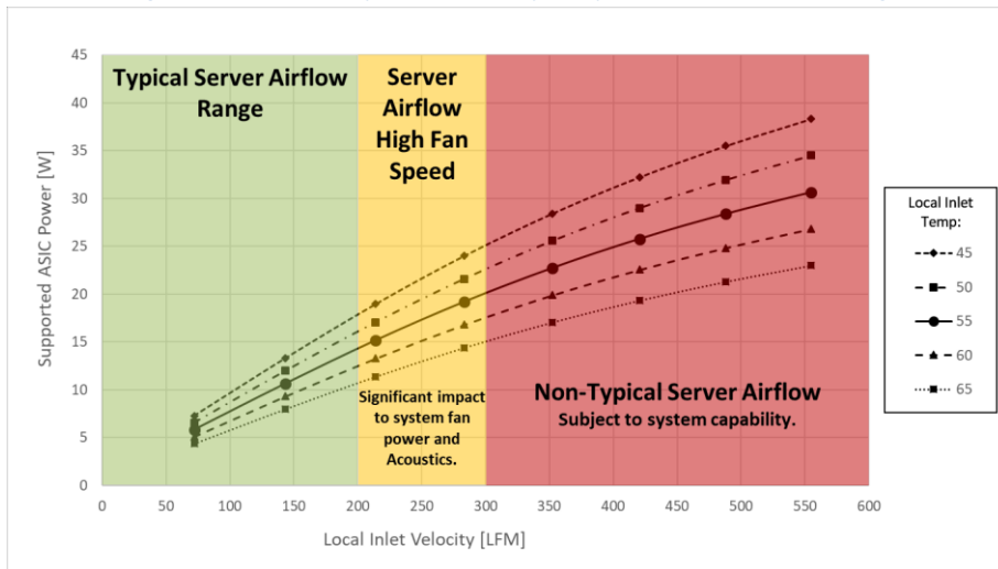
Figure 111 102: Server System Airflow Capability – SFF Card Hot Aisle Cooling
