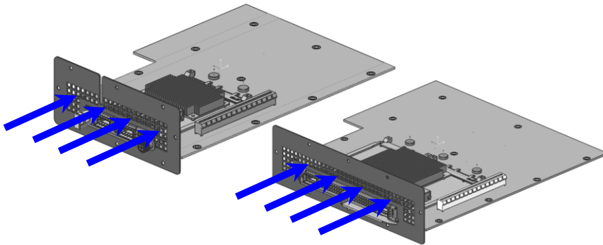
Figure 10899 : Airflow Direction for Cold Aisle Cooling (SFF and LFF)
