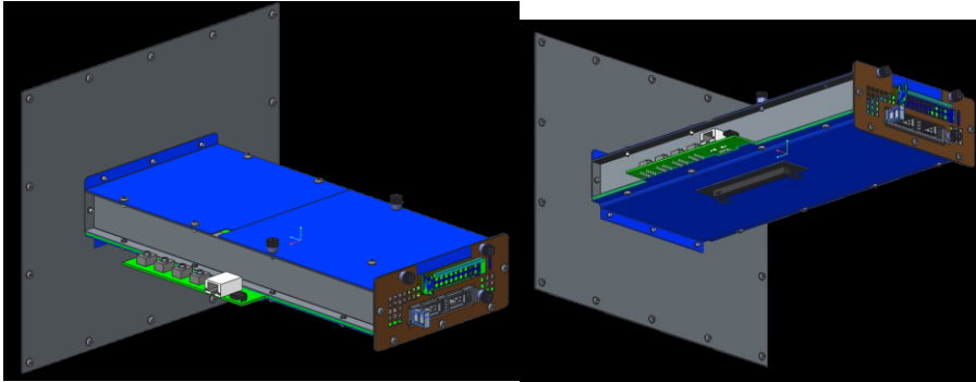
Figure 121 112 : SFF Thermal Test Fixture Preliminary Design
