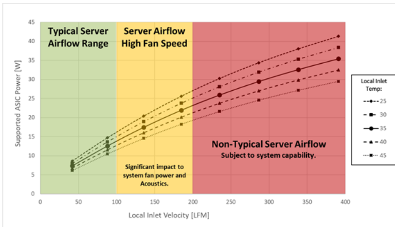
Figure 116107: Server System Airflow Capability – SFF Cold Aisle Cooling
