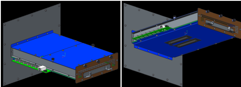
Figure 124 115 : LFF Card Thermal Test Fixture Design
