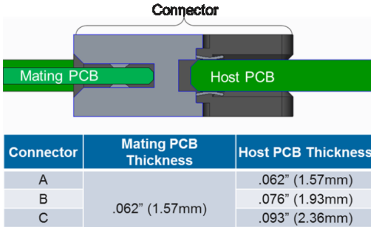
Figure 73 69: OCP NIC 3.0 Card and Baseboard PCB Thickness Options for Straddle Mount Connectors
