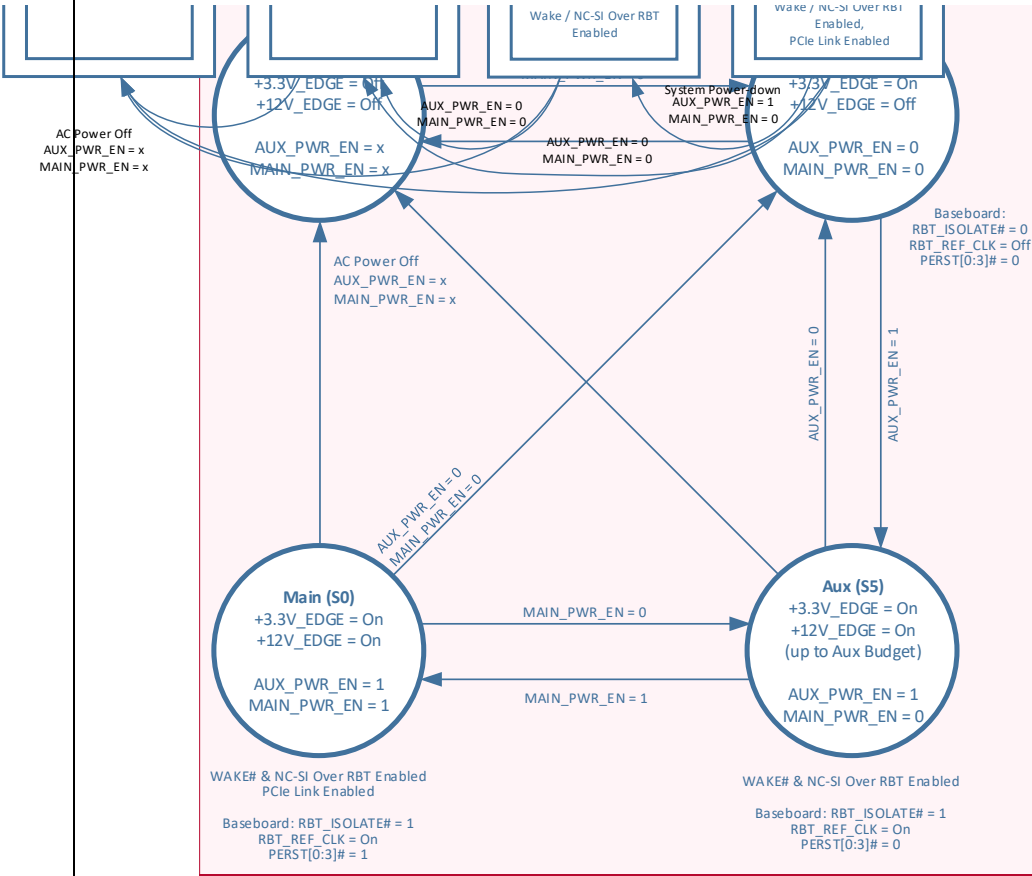
Figure 10193: Baseboard Power States
