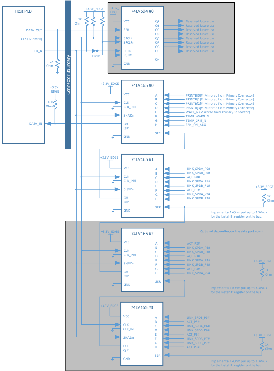
Figure 8480: Scan Chain Connection Example
