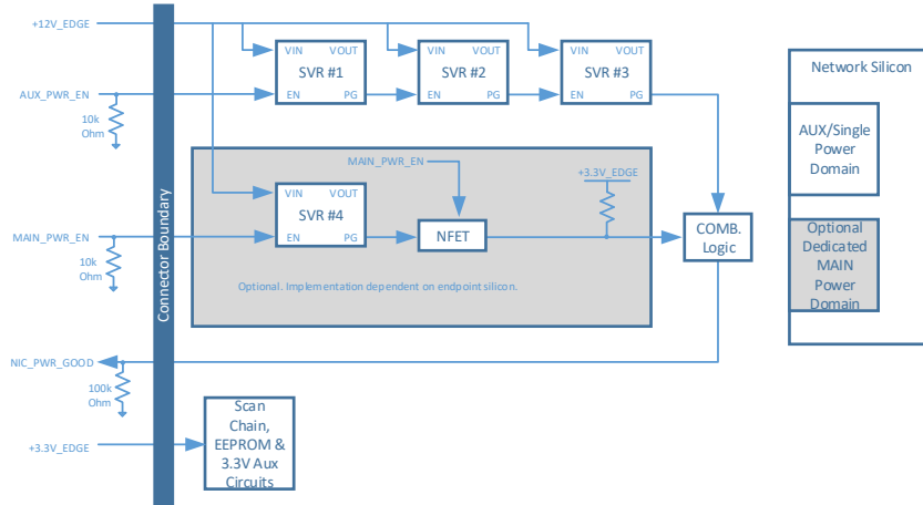
Figure 8584 : Example Power Supply Topology
