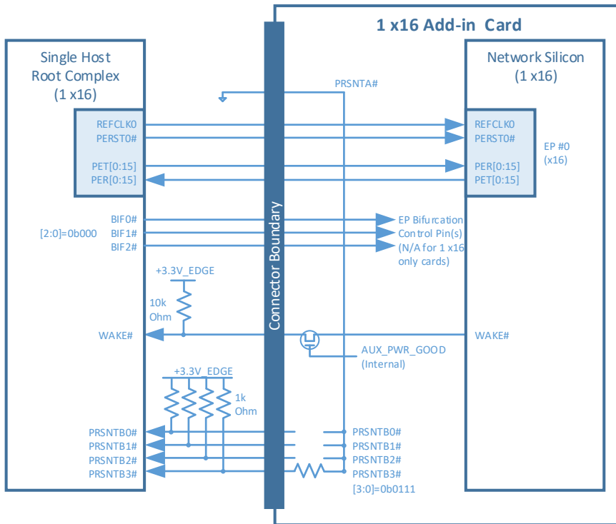
Figure 89 85: Single Host (1 x16) and 1 x16 OCP NIC 3.0 Card (Single Controller)
