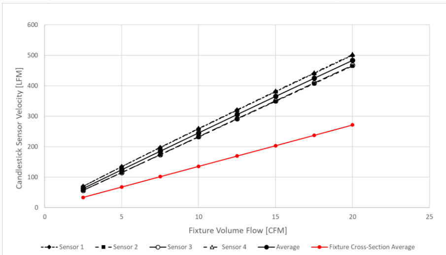
Figure 129120 : LFF Fixture, Hot Aisle Flow - Candlestick Air Velocity vs. Volume Flow
