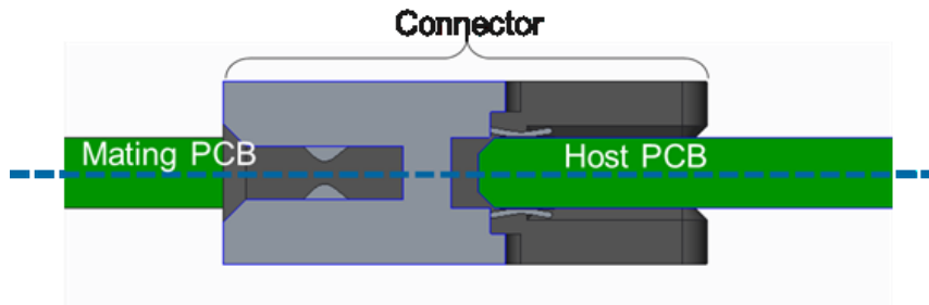
Figure 74 70: 0.3mm Offset (Coplanar) for 0.062" Thick Baseboards
