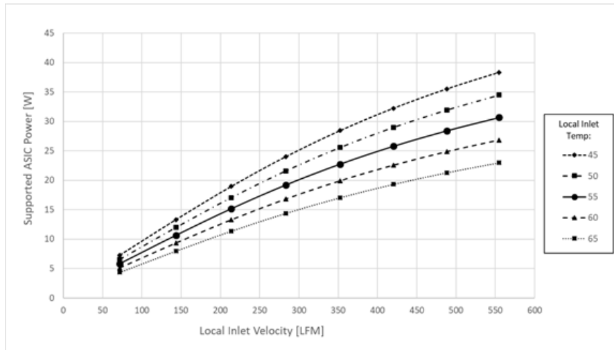
Figure 109100: ASIC Supportable Power for Hot Aisle Cooling – SFF
