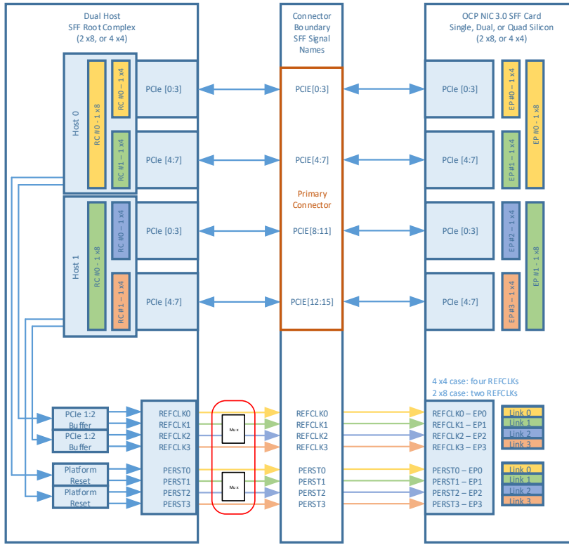
Figure 95: SFF PCIe REFCLK Mapping – Dual Host – 2 and 4 links
