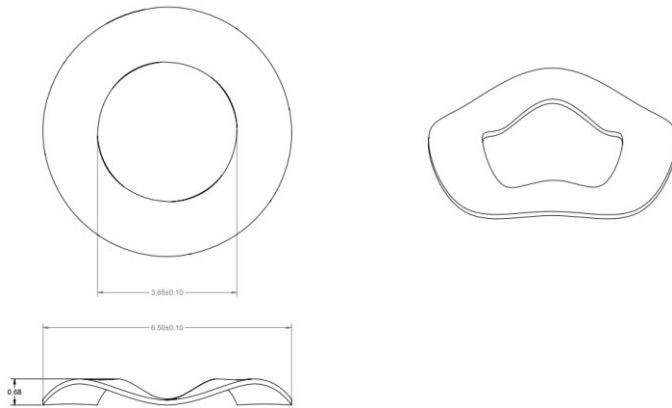
Figure 23: Wave Washer
