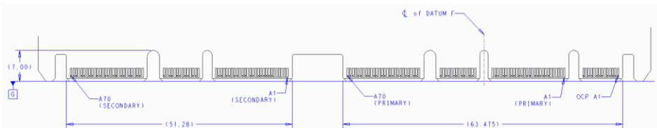
Figure 6763: LFF Gold Finger Dimensions – x32 – Bottom Side (“A” Pins)
