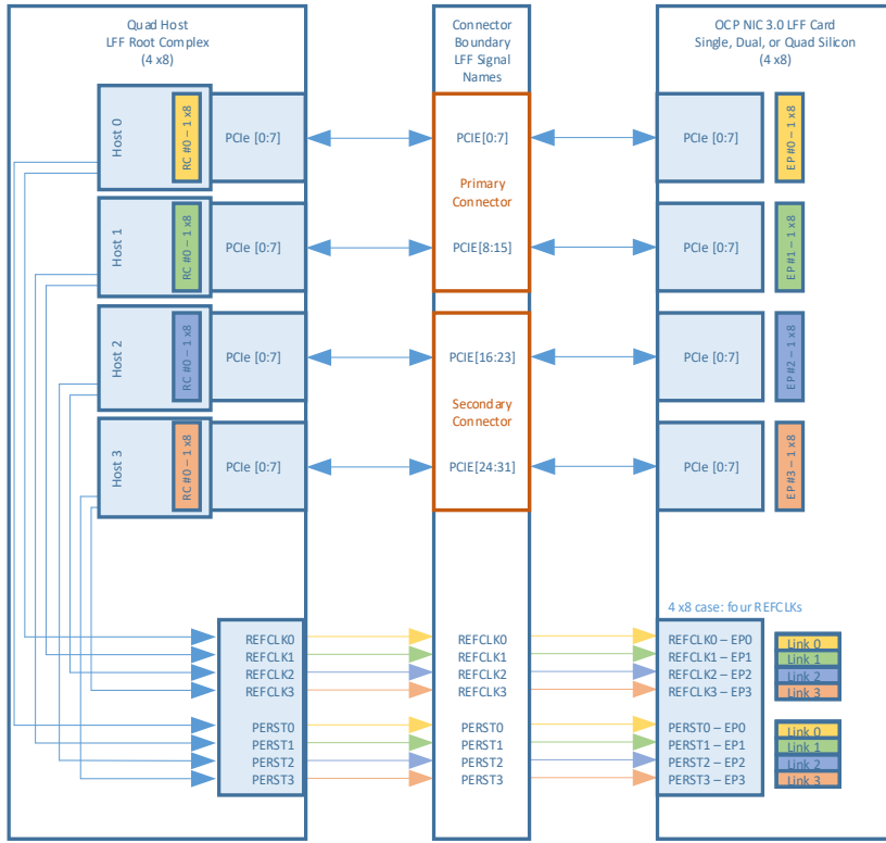
Figure 99: LFF PCIe REFCLK Mapping – Quad Host – 4 Links
