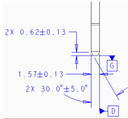
Figure 65: SFF Primary Connector Gold Finger - Detail D
