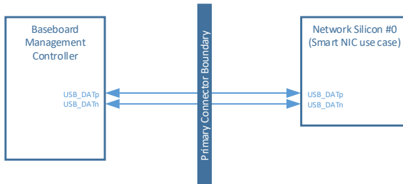
Figure 8682 : USB 2.0 Connection Example – Basic Connectivity
