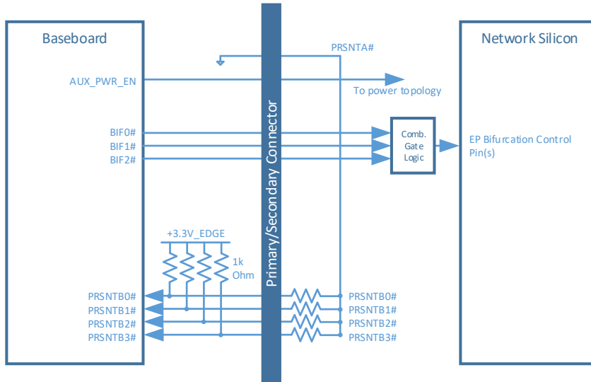
Figure 7874: PCIe Present and Bifurcation Control Pins (Baseboard Controlled BIF[0:2]#)
