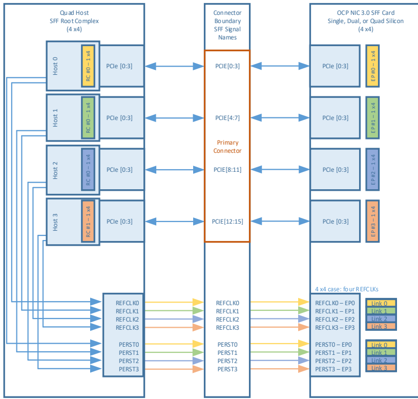
Figure 96: SFF PCIe REFCLK Mapping – Quad Host – 4 Links
