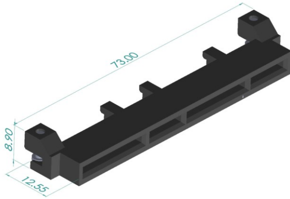
Figure 7268 : 140-pin Base Board Secondary Connector – Straddle Mount
