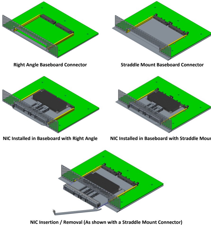
Figure 12: LFF NIC Chassis Mounted 3D Views
