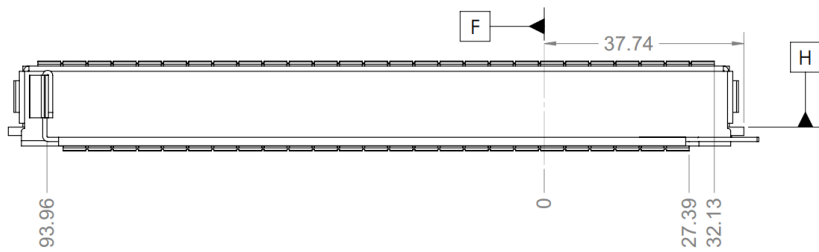
Figure 5250 : LFF OCP NIC 3.0 Card with Ejector CTF Dimensions (Front View)
