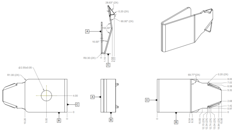
Figure 21: Ejector Lock
