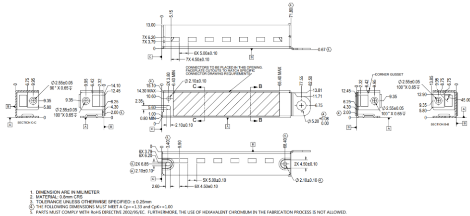
Figure 16: SFF Generic I/O Faceplate – Ejector Version (2D View)
