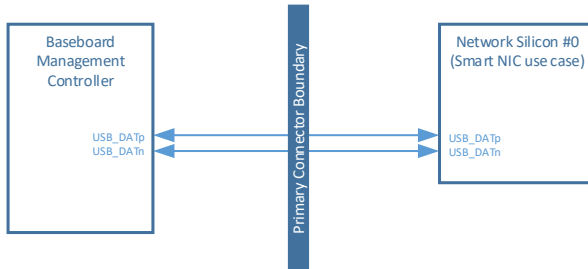
Figure 8482: USB 2.0 Connection Example – Basic Connectivity
