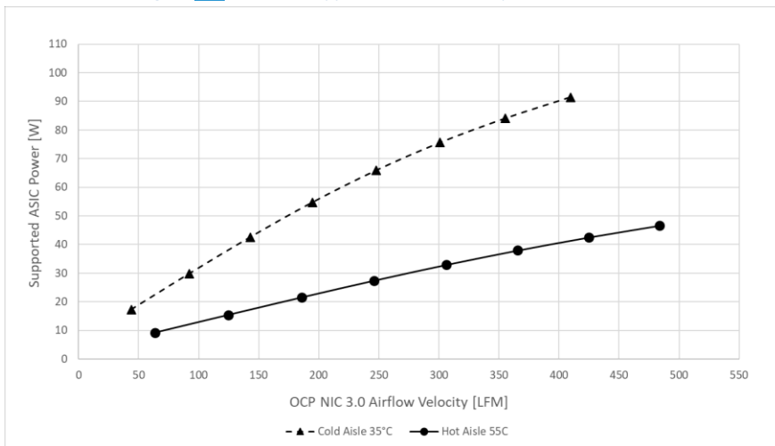
Figure 117141: ASIC Supportable Power Comparison – LFF Card
