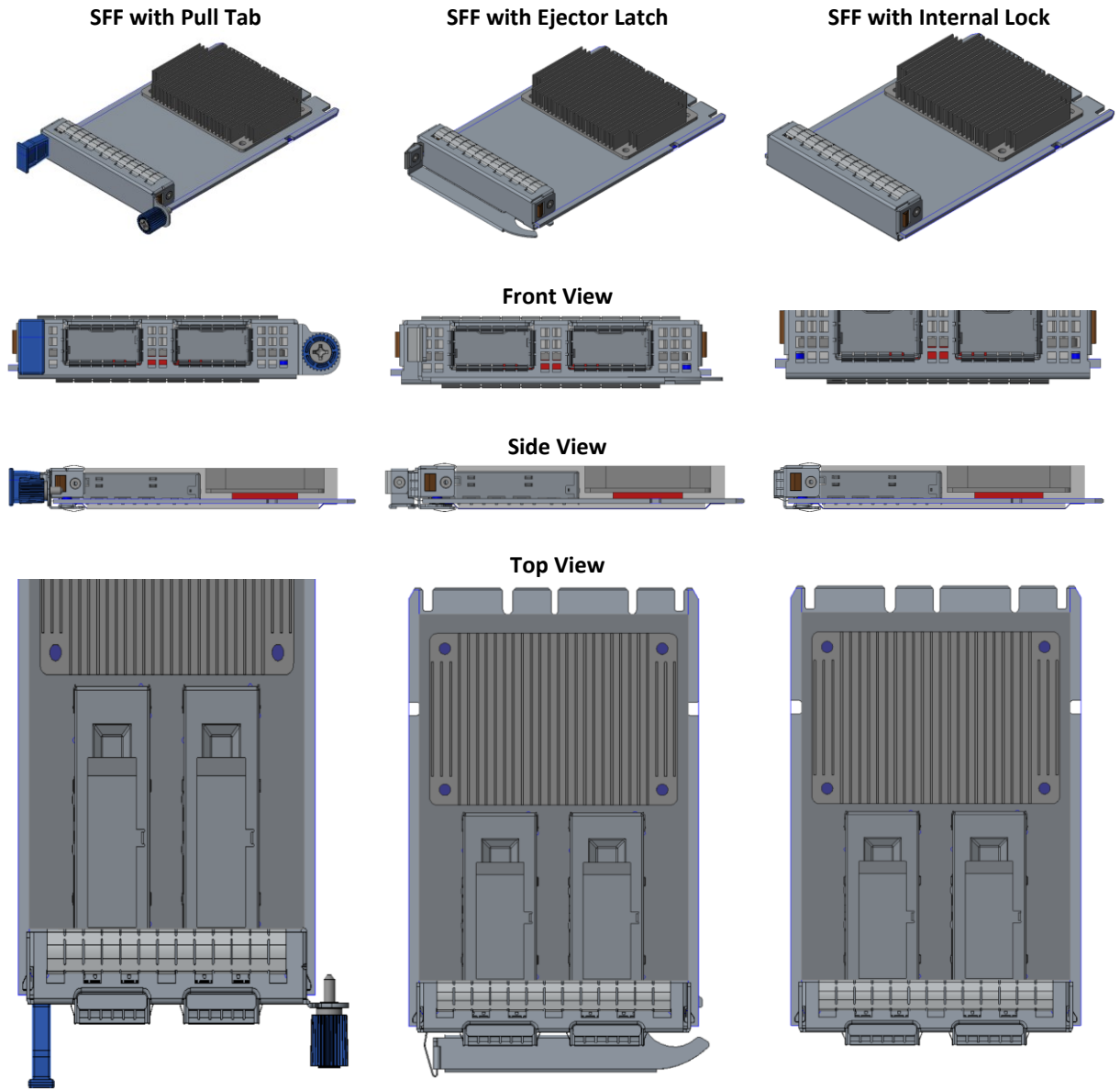
Figure 7: SFF NIC Configuration Views
