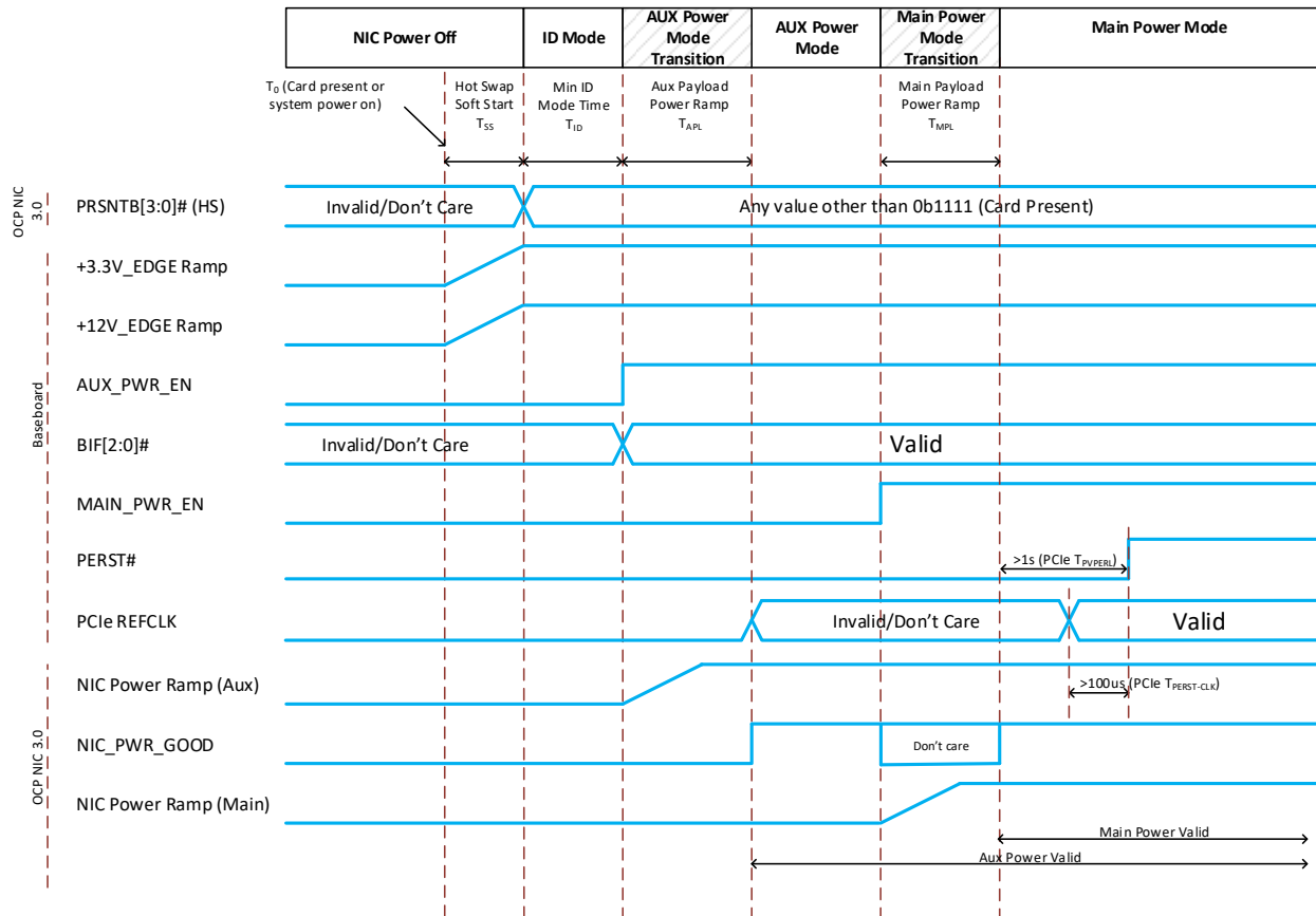
Figure 94: Power-Up Sequencing
