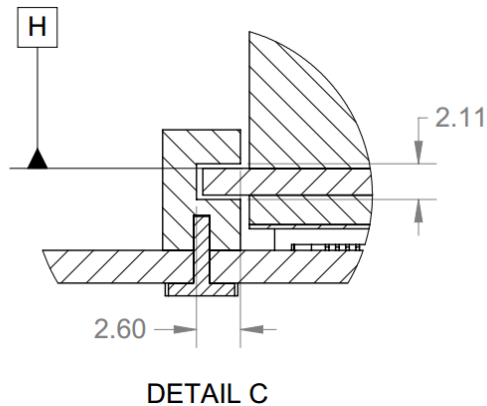
Figure 55: LFF Baseboard Chassis CTF Dimensions (Rail Guide – Detail C)
