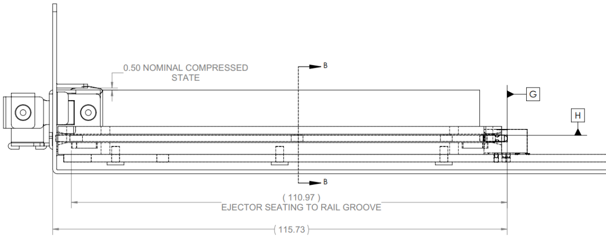
Figure 53: LFF Baseboard Chassis CTF Dimensions (Side View)
