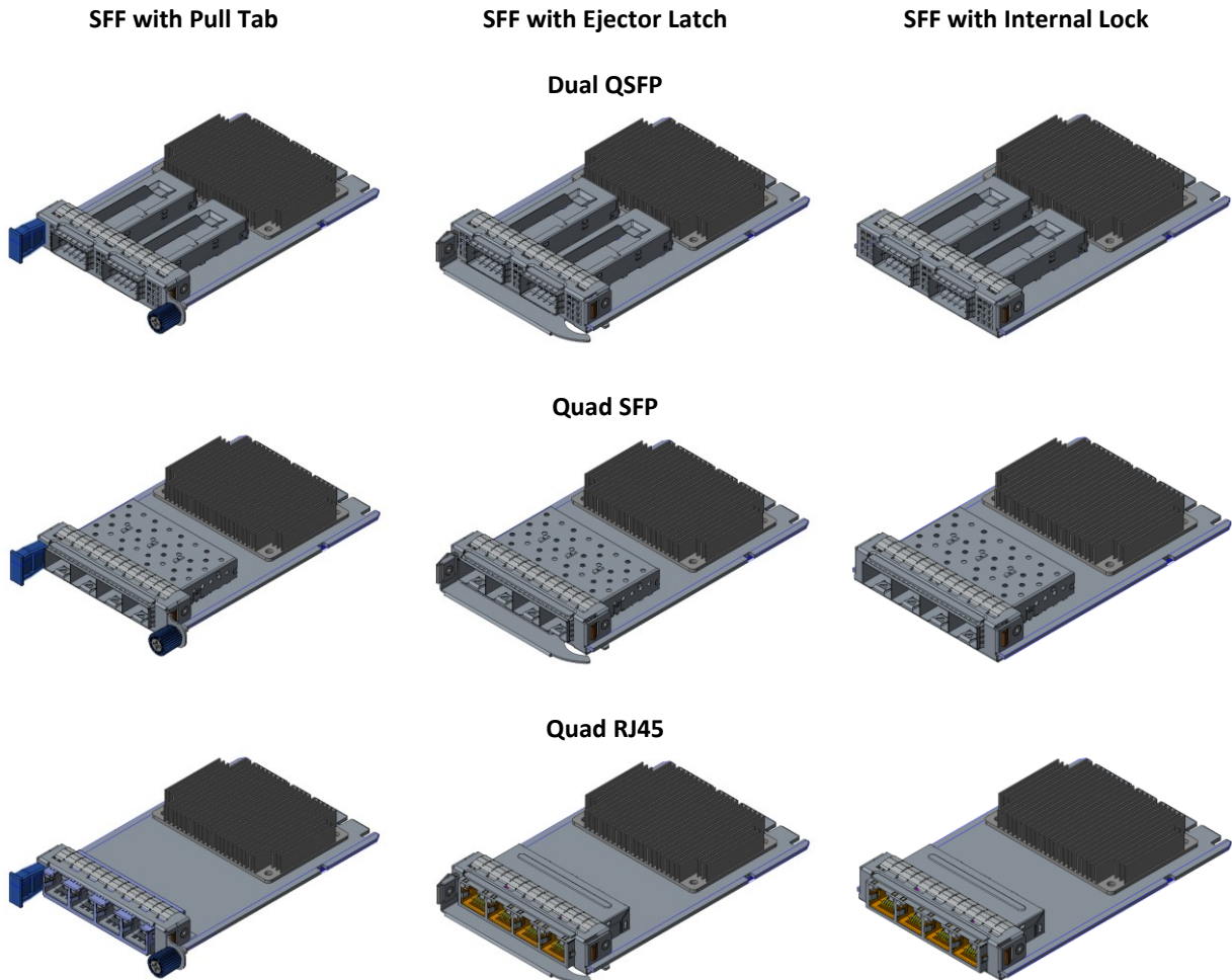
Figure 8: SFF NIC Line Side 3D Views
