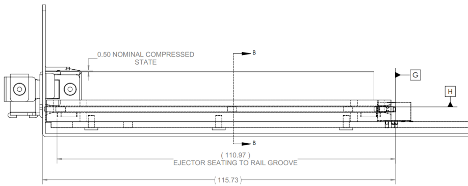
Figure 54: LFF Baseboard Chassis CTF Dimensions (Rail Guide View)
