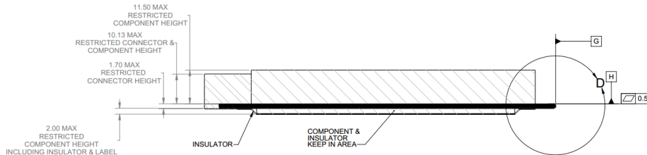
Figure 32: LFF Keep Out Zone – Side View
