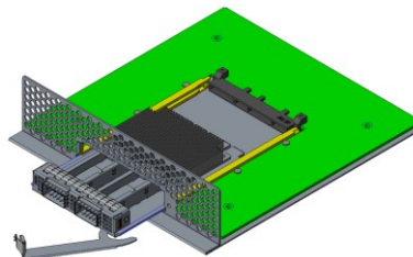
Straddle Mount Baseboard Connector
