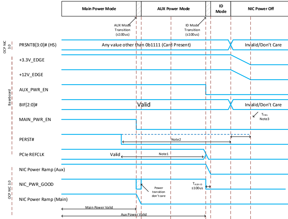
Figure 95: Power-Down Sequencing
