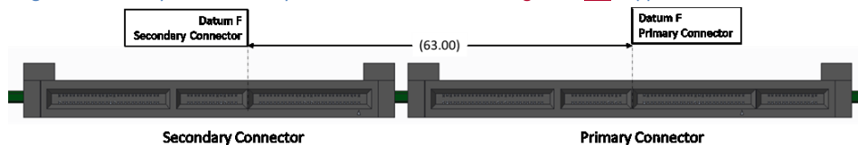
Figure 73: Primary and Secondary Connector Locations for Large-Card LF Support with Straddle Mount
