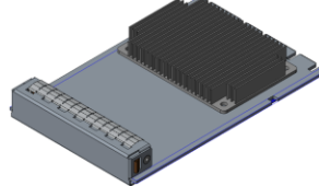
Small Form Factor (SFF) with Internal Lock
