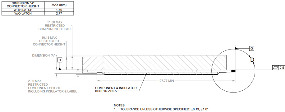
Figure 27: Small Form Factor SFF Keep Out Zone – Side View
