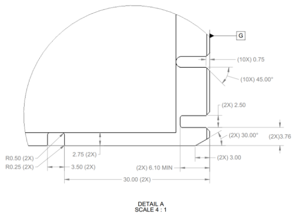
Figure 25: Small Form Factor (SFF) Keep Out Zone – Top View – Detail A
