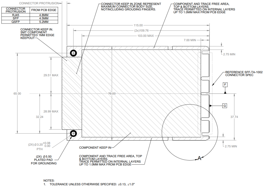
Figure 24: Small Form Factor (SFF) Keep Out Zone – Top View
