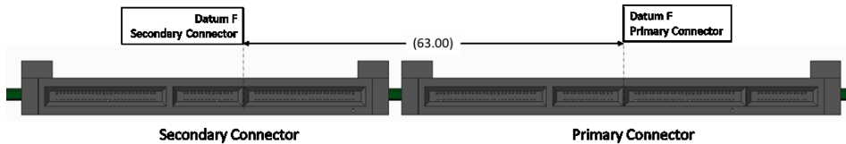
Figure 73: Primary and Secondary Connector Locations for Large-Card FF Support with Straddle Mount Connectors
