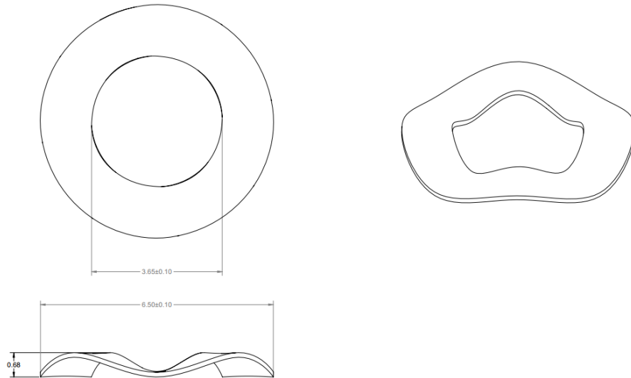
Figure 23: Wave Washer
