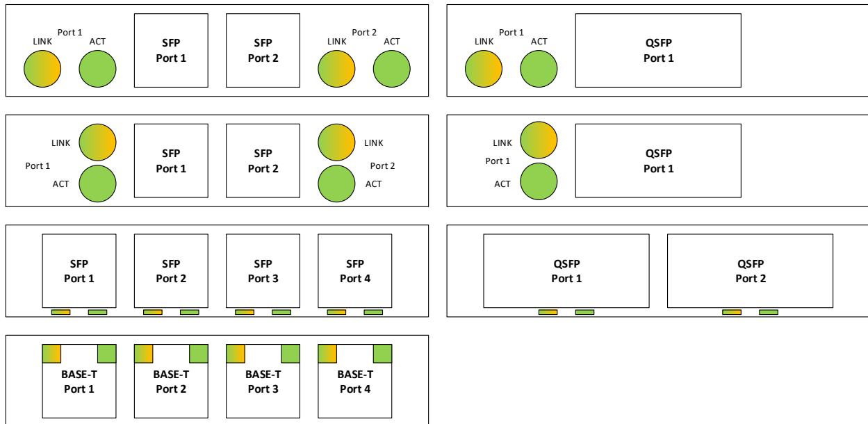
Figure 92: Port and LED Ordering – Example SFF Link/Activity and Speed LED Placement
