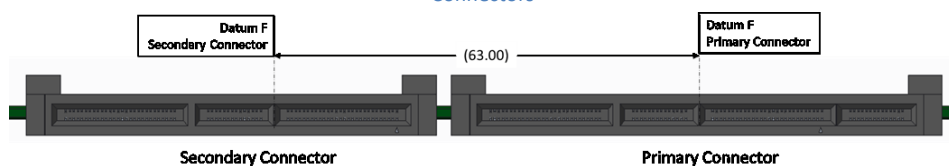
Figure 73: Primary and Secondary Connector Locations for Large-Card LF Support with Straddle Mount Connectors
