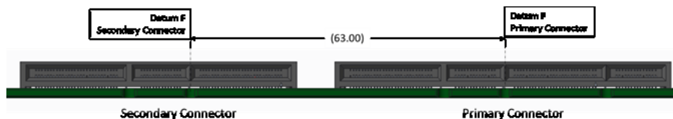
Figure 72: Primary and Secondary Connector Locations for Large-Card LF Support with Right Angle Connectors
