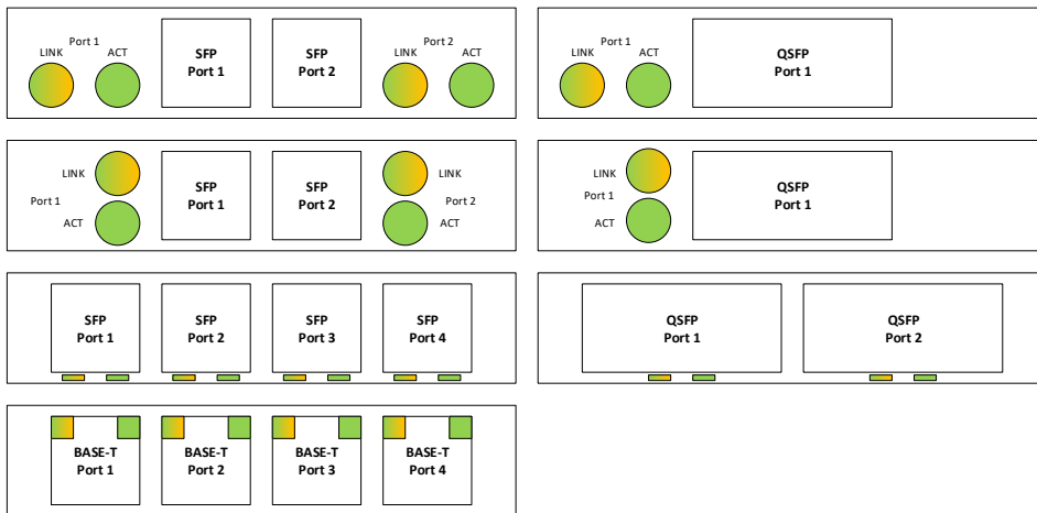
Figure 92: Port and LED Ordering – Example Small Card SFP Link/Activity and Speed LED Placement
