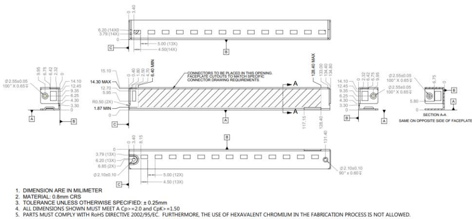
Figure 18: Large Card Generic I/O Faceplate – Dual Ejector Version (2D View)
