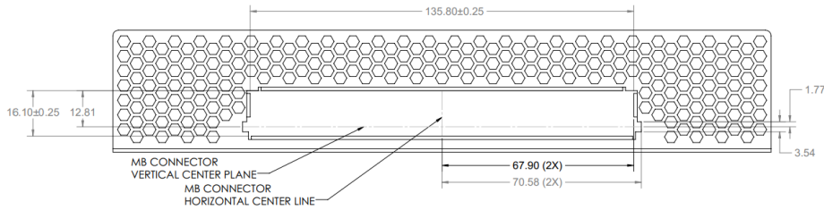
Figure 52: Large Form Factor Baseboard Chassis CTF Dimensions (Rear View)
