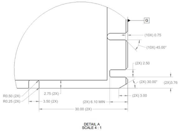
Figure 25: Small Form Factor Keep Out Zone – Top View – Detail A
