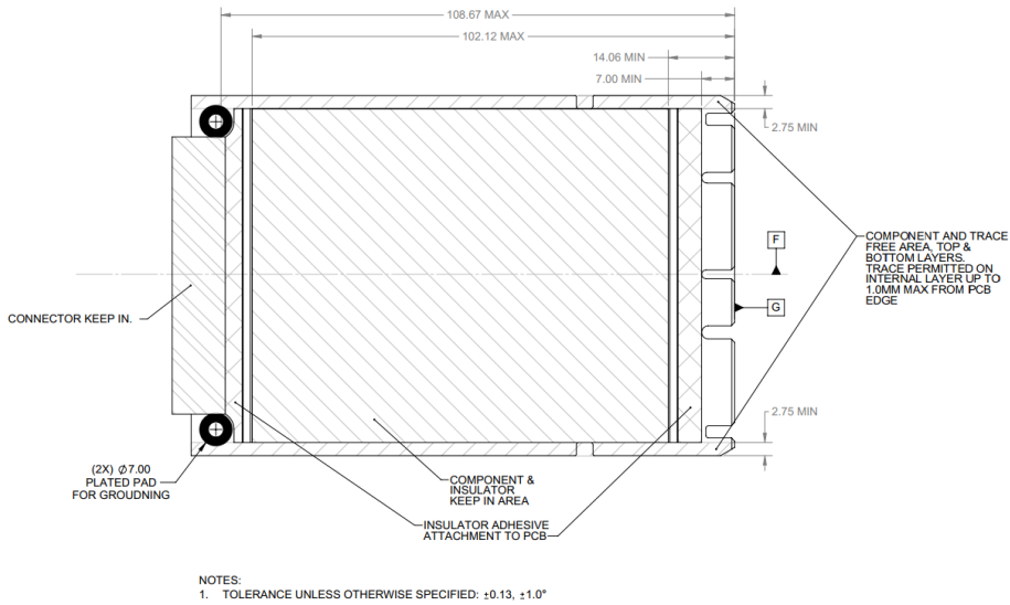
Figure 26: Small Form Factor Keep Out Zone – Bottom View
