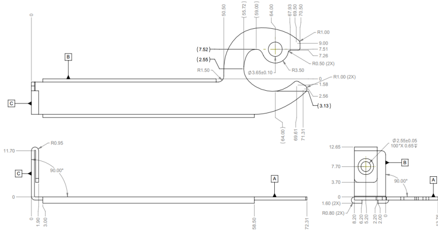
Figure 19: Small Card I/O Faceplate – Ejector Lever (2D View)
