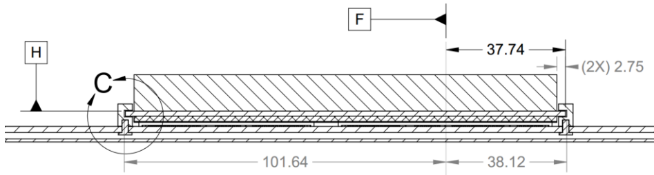
Figure 54: Large Form Factor Baseboard Chassis CTF Dimensions (Rail Guide View)
