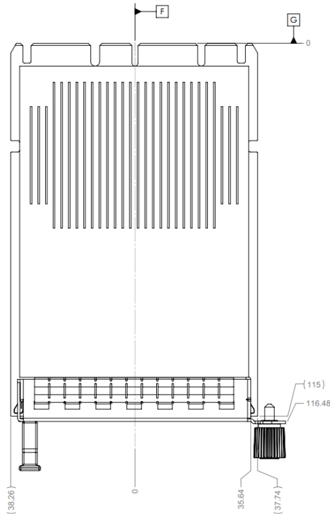
Figure 38: Small Form Factor OCP NIC 3.0 Card with Pull Tab CTF Dimensions (Top View)
