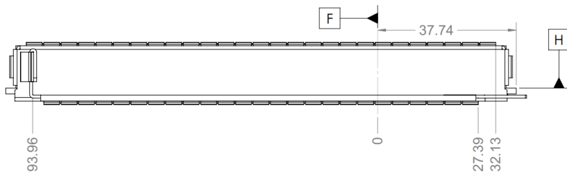
Figure 50: Large Form Factor OCP NIC 3.0 Card with Ejector CTF Dimensions (Front View)
