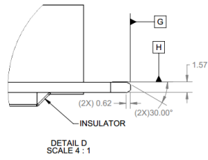
Figure 28: Small Form Factor Keep Out Zone – Side View – Detail D
