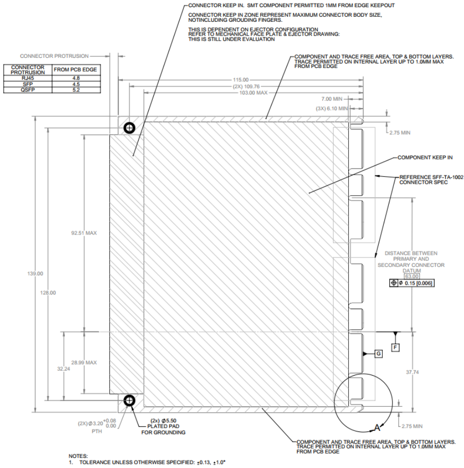
Figure 29: Large Form Factor Keep Out Zone – Top View
