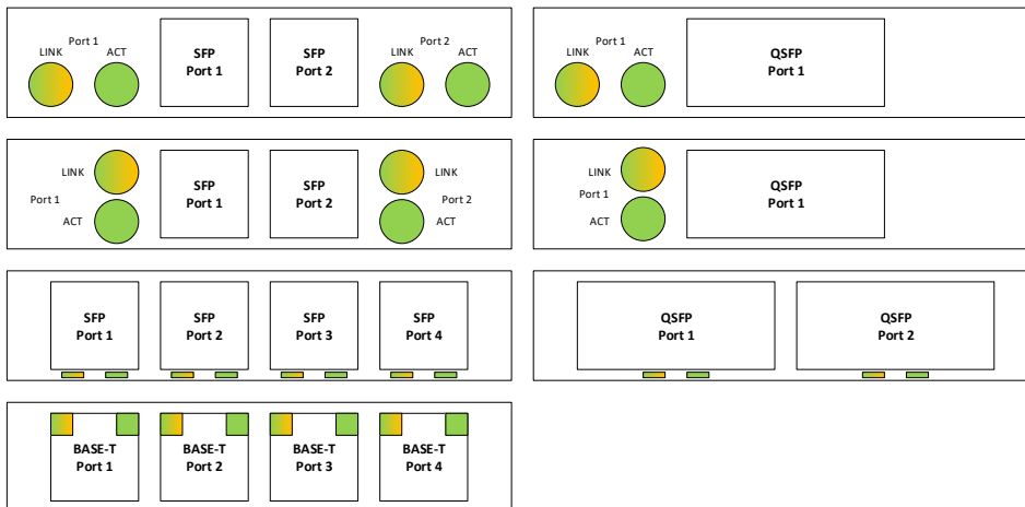
Figure 92: Port and LED Ordering – Example Small Card Link/Activity and Speed LED Placement
