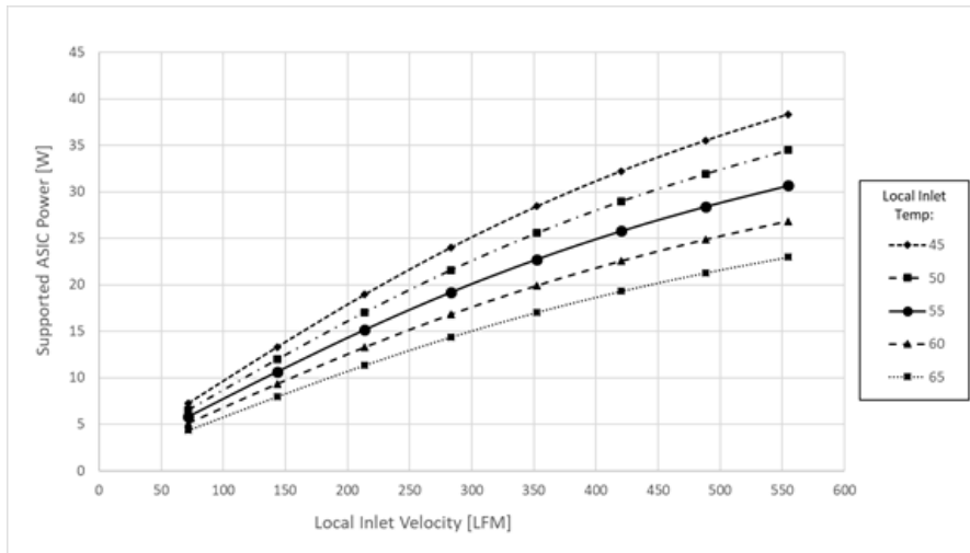
Figure 100: ASIC Supportable Power for Hot Aisle Cooling – Small Card Form Factor
