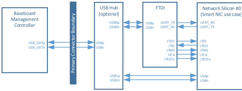
Figure 83: USB 2.0 Connection Example – USB-Serial / USB-JTAG Connectivity
