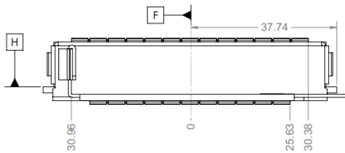
Figure 43: Small Form Factor OCP NIC 3.0 Card with Ejector CTF Dimensions (Side View)
