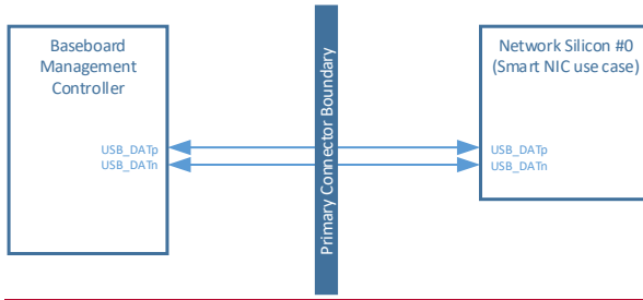
Figure 82: USB 2.0 Connection Example – Basic Connectivity
