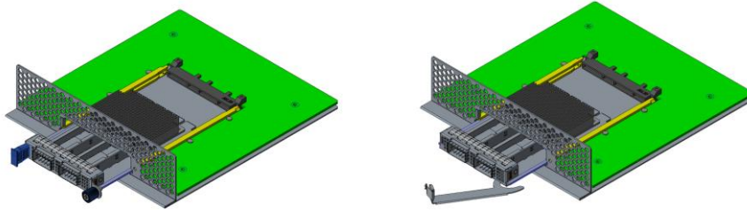
NIC Insertion / Removal (Shown with a Straddle Mount Connector)
