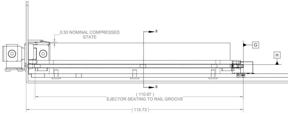
Figure 47: Small Form Factor Baseboard Chassis CTF Dimensions (Rear Rail Guide View)
