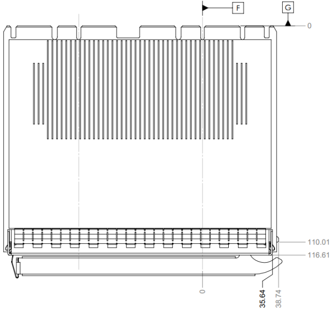
Figure 50: Large Form Factor OCP NIC 3.0 Card with Ejector CTF Dimensions (Front View)
