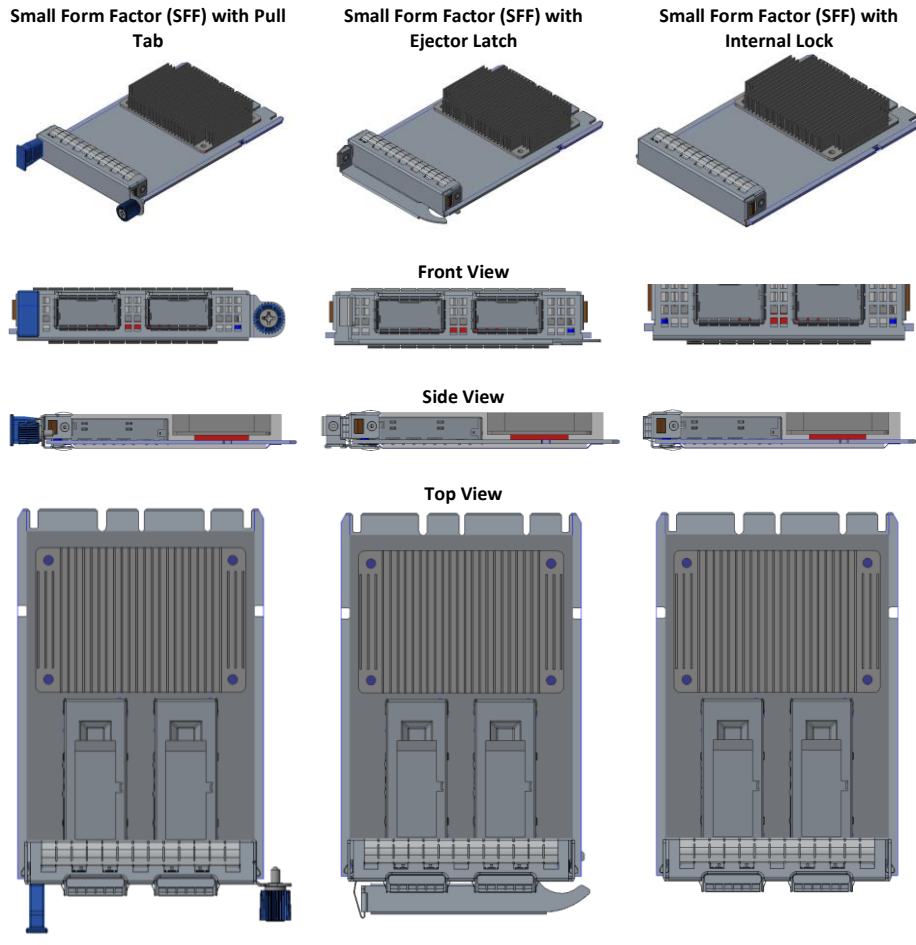
Figure 7: Small Form Factor NIC Configuration Views
