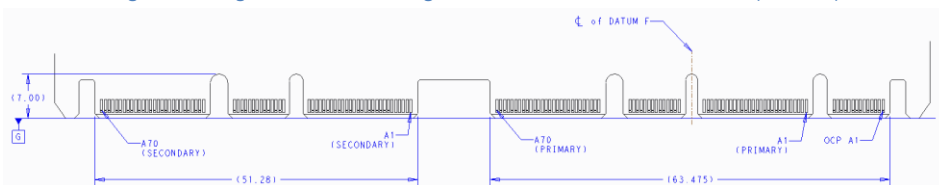
Figure 63: Large Size Card Gold Finger Dimensions – x32 – Bottom Side (“A” Pins)
