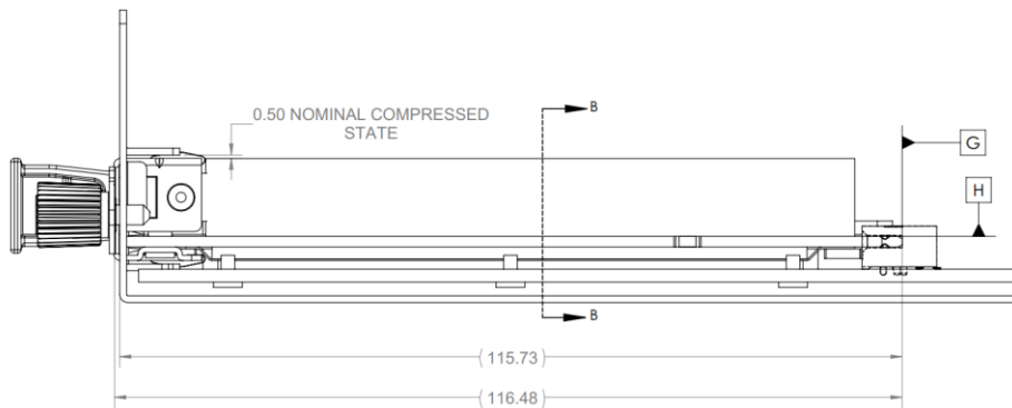
Figure 45: Small Form Factor Baseboard Chassis to Card Thumb Screw CTF Dimensions (Side View)
