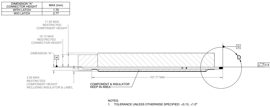
Figure 27: Small Form Factor Keep Out Zone – Side View
