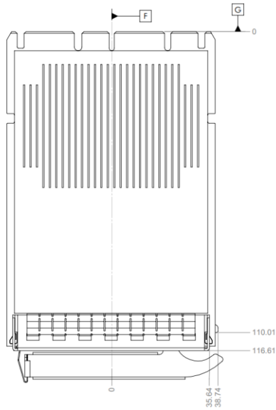
Figure 42: Small Form Factor OCP NIC 3.0 Card with Ejector CTF Dimensions (Front View)
