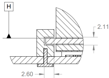
Figure 55: Large Form Factor Baseboard Chassis CTF Dimensions (Rail Guide – Detail C)
