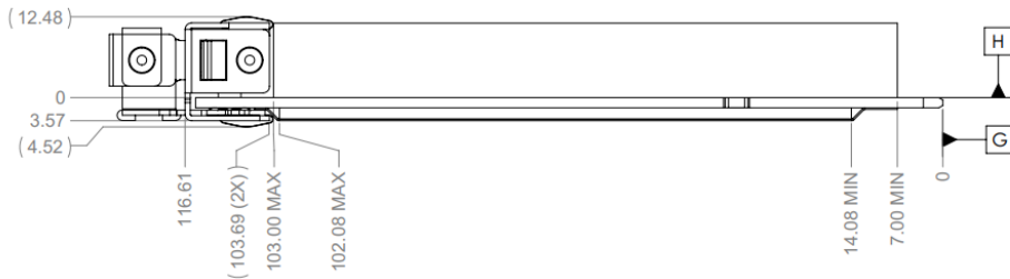
Figure 43: Small Form Factor OCP NIC 3.0 Card with Ejector CTF Dimensions (Side View)
