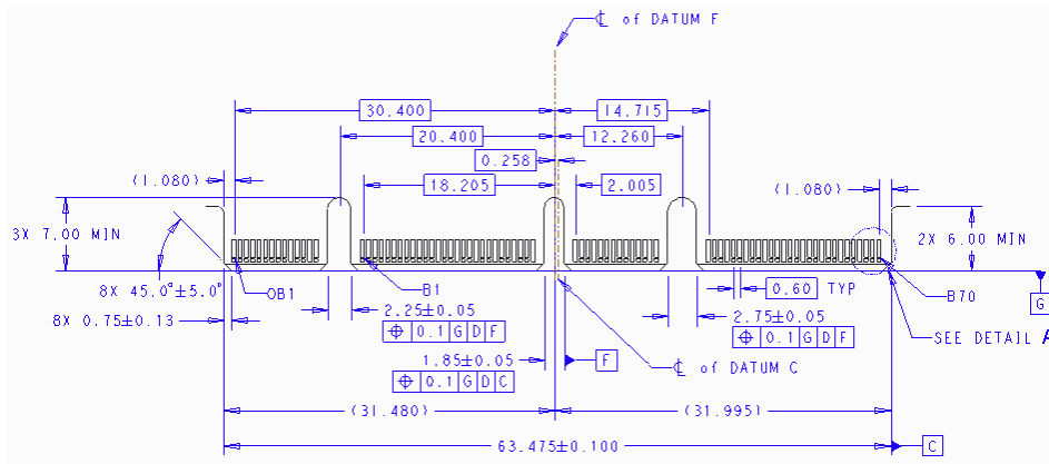
Figure 61: Small Size Primary Connector Gold Finger Dimensions – x16 – Top Side (“B” Pins)
