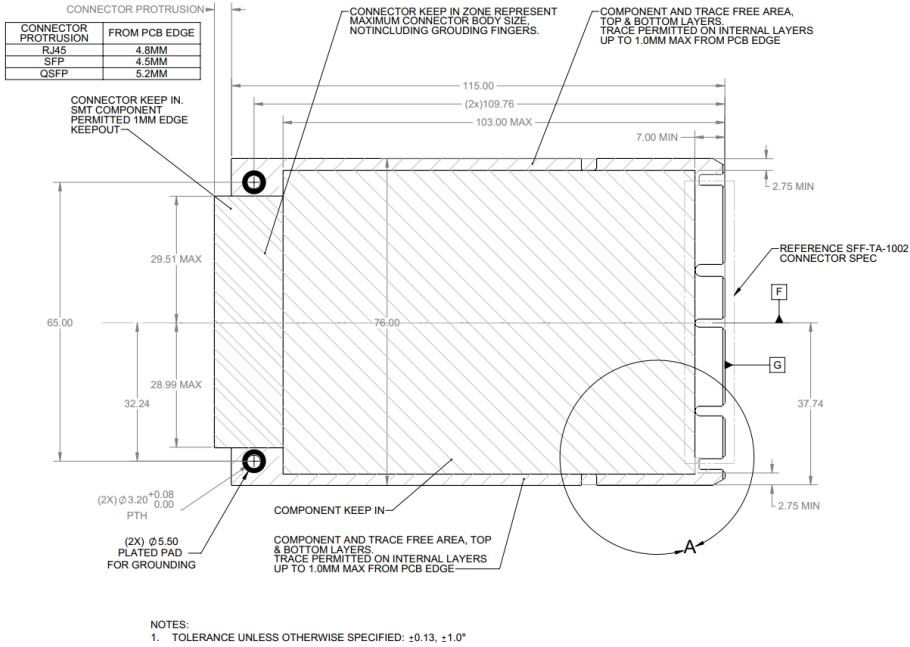
Figure 24: Small Form Factor Keep Out Zone – Top View
