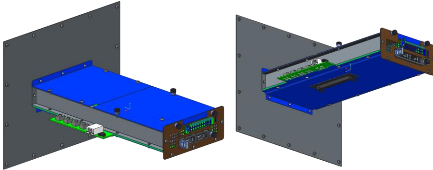
Figure 112: Small Card Thermal Test Fixture Preliminary Design
