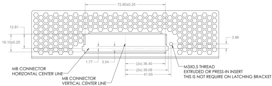
Figure 44: Small Form Factor Baseboard Chassis CTF Dimensions (Rear View)
