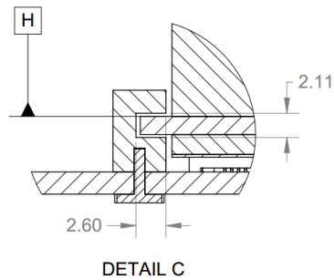
Figure 48: Small Form Factor Baseboard Chassis CTF Dimensions (Rail Guide Detail) – Detail C
