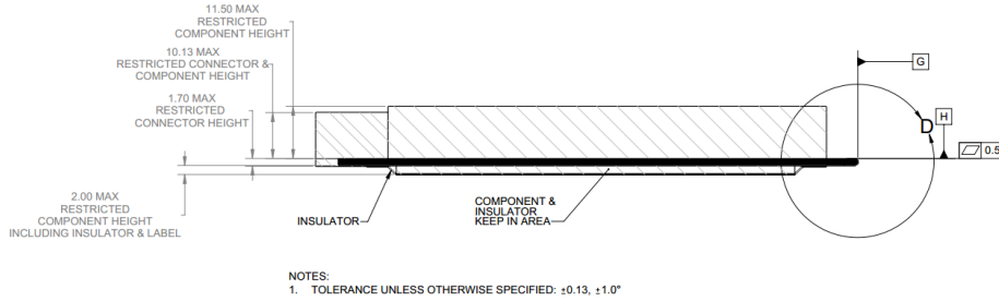
Figure 33: Large Form Factor Keep Out Zone – Side View – Detail D
