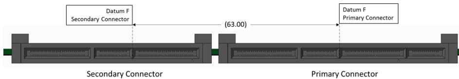
Figure 73: Primary and Secondary Connector Locations for Large Card Support with Straddle Mount Connectors
