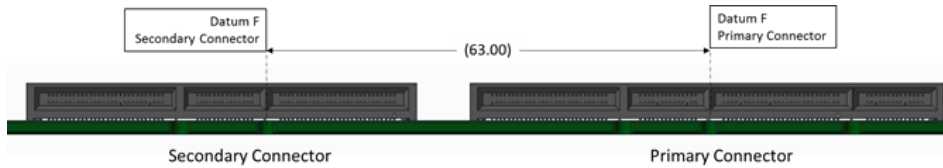
Figure 72: Primary and Secondary Connector Locations for Large Card Support with Right Angle Connectors
