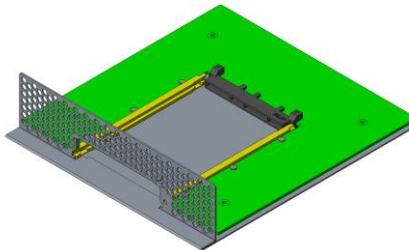
Figure 9: Small Form Factor NIC Chassis Mounted 3D Views
