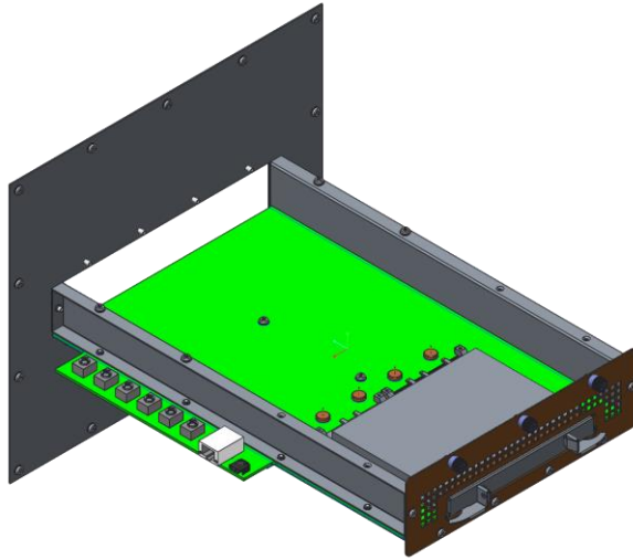
Figure 116: LFF Card Thermal Test Fixture Design – Cover Removed
