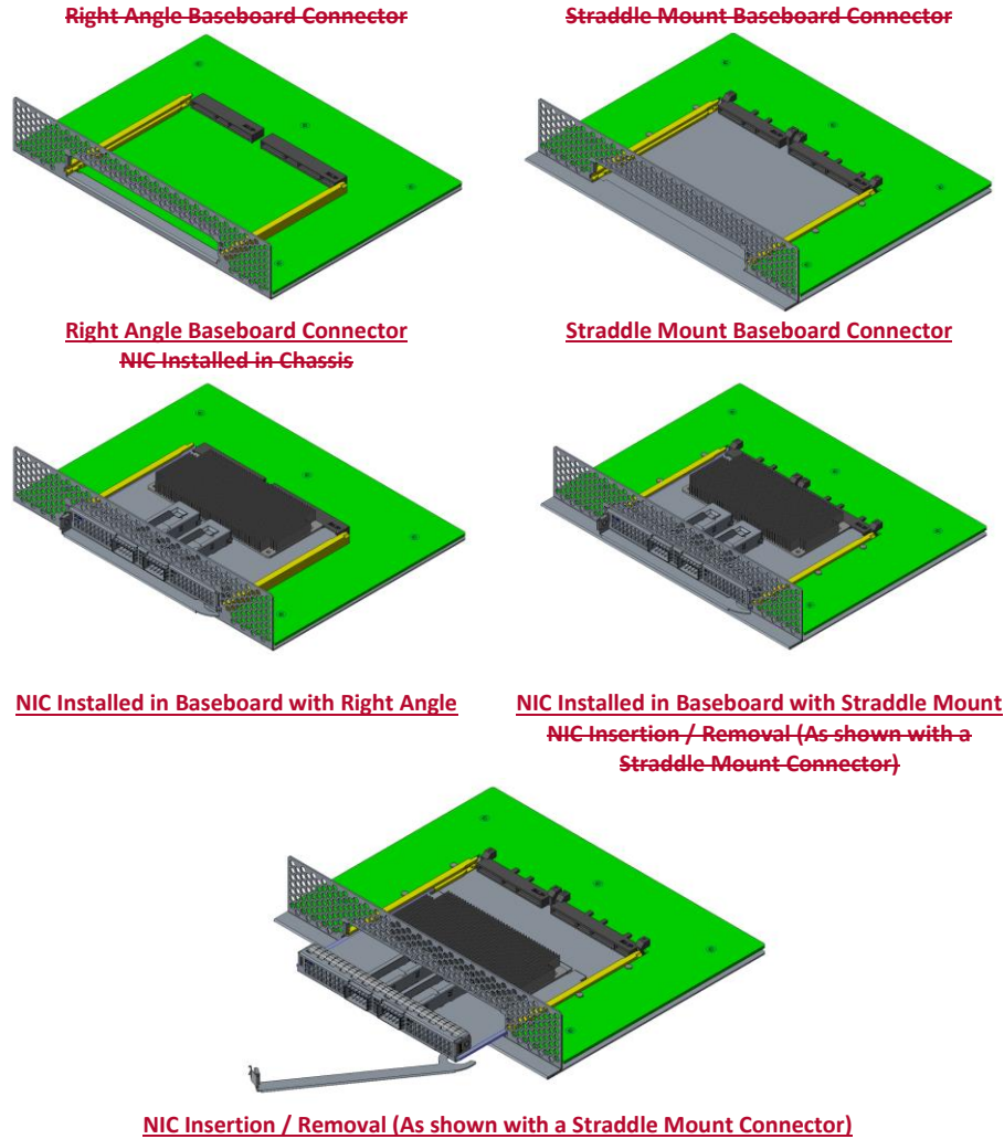
Figure 12: Large Form Factor NIC Chassis Mounted 3D Views
