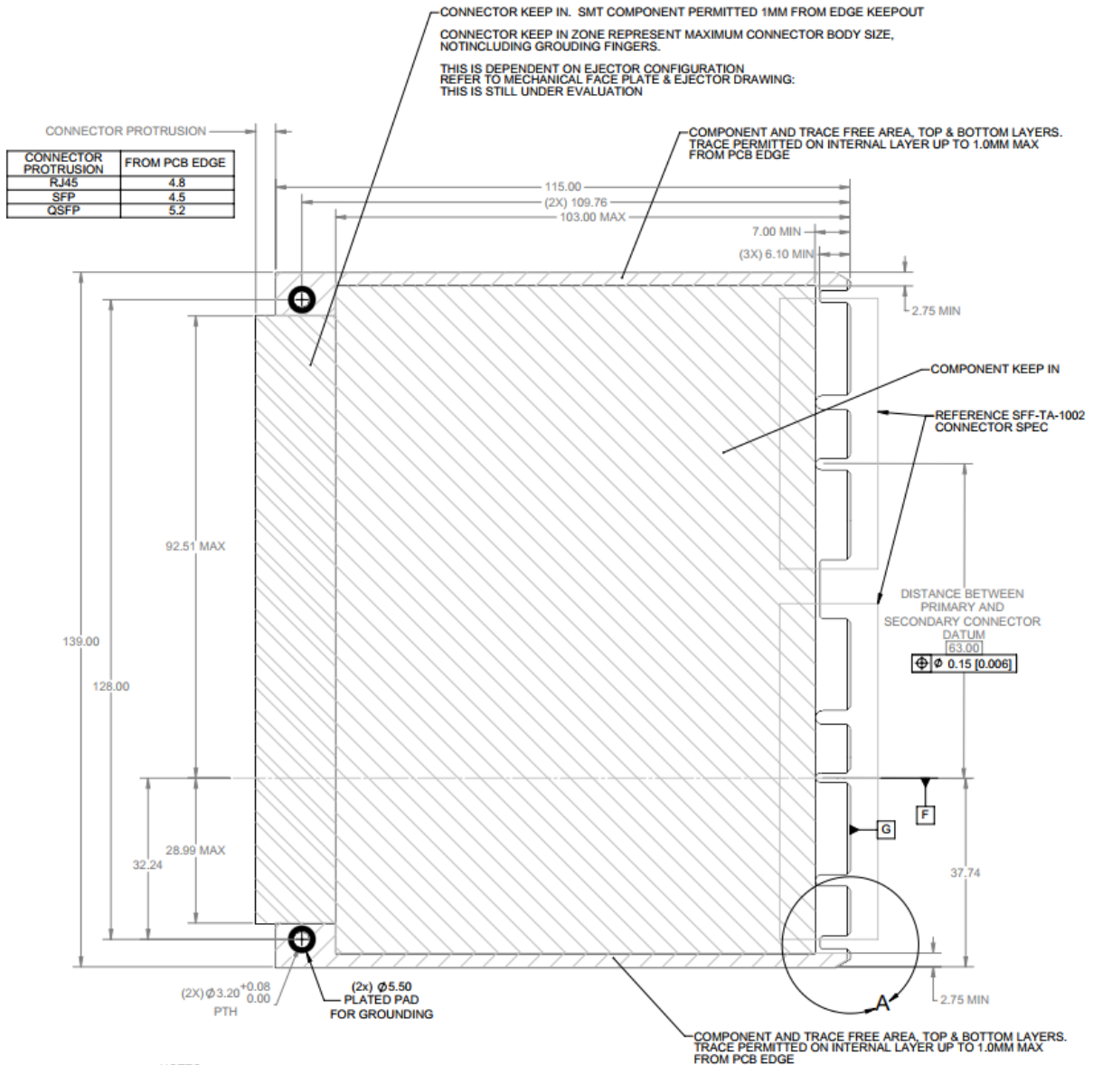
Figure 29: Large Form Factor Keep Out Zone – Top View
