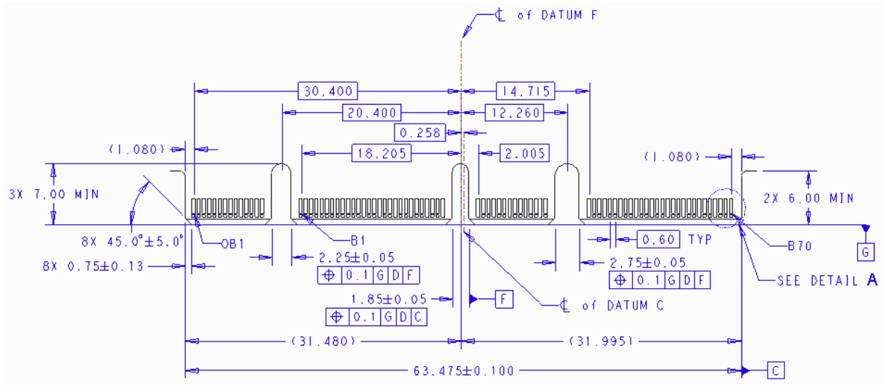
Figure 61: Small Size Primary Connector Gold Finger Dimensions – x16 – Top Side (“B” Pins)
