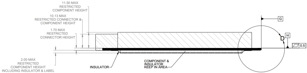
Figure 32: Large Form Factor Keep Out Zone – Side View
