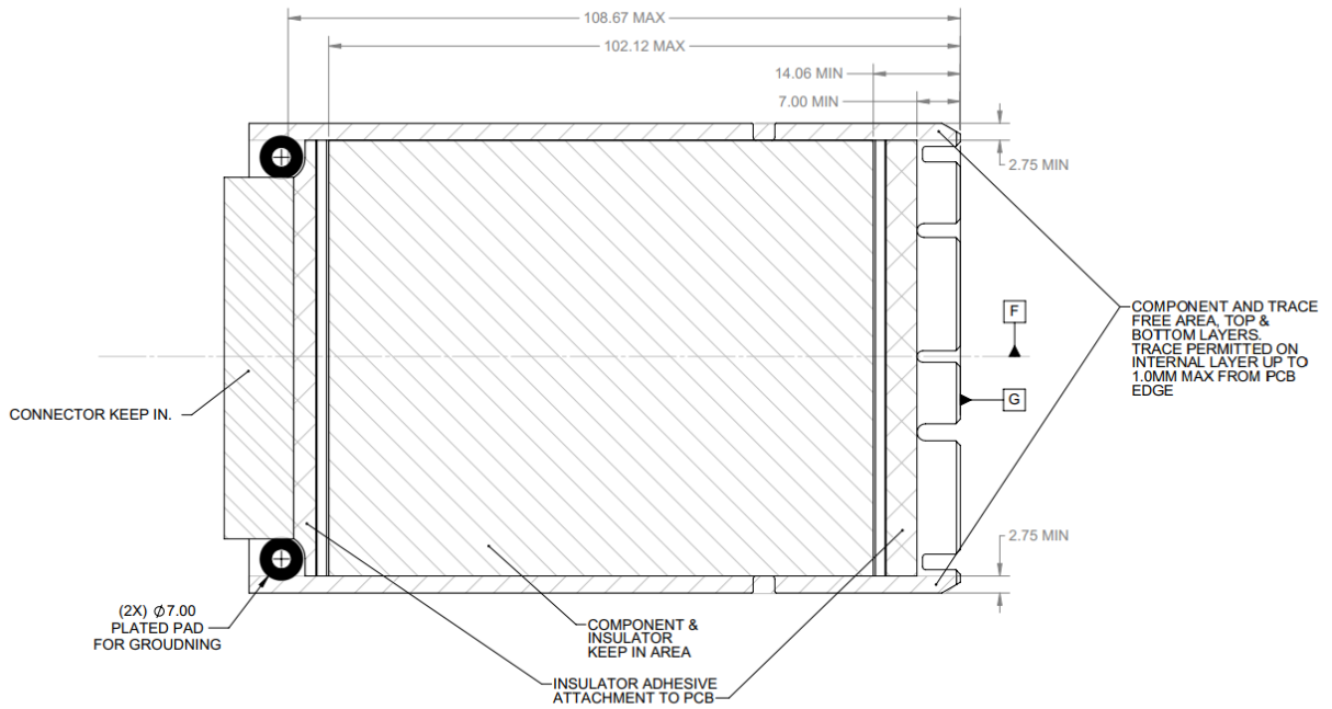
Figure 26: Small Form Factor Keep Out Zone – Bottom View
