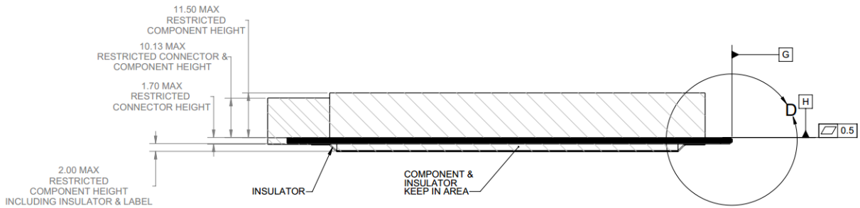
Figure 32: Large Form Factor Keep Out Zone – Side View
