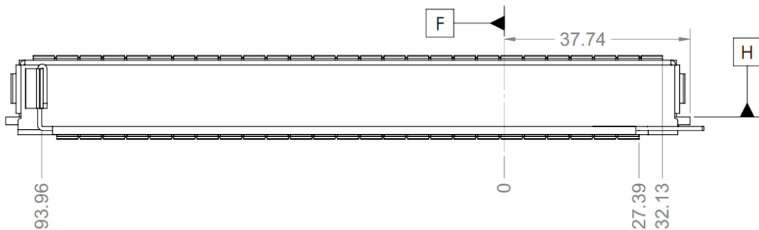
Figure 50: Large Form Factor OCP NIC 3.0 Card with Ejector CTF Dimensions (Front View)
