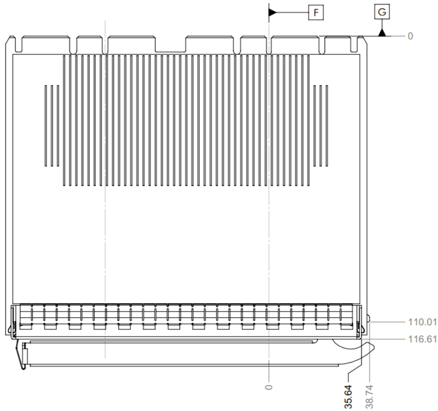
Figure 49: Large Form Factor OCP NIC 3.0 Card with Ejector CTF Dimensions (Top View)
