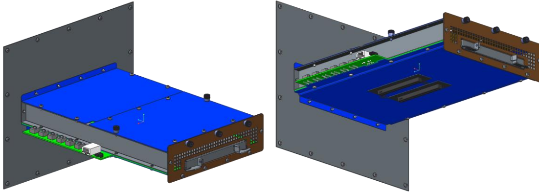
Figure 115: LFF Card Thermal Test Fixture Design
