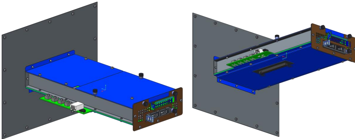
Figure 112: Small Card Thermal Test Fixture Preliminary Design
