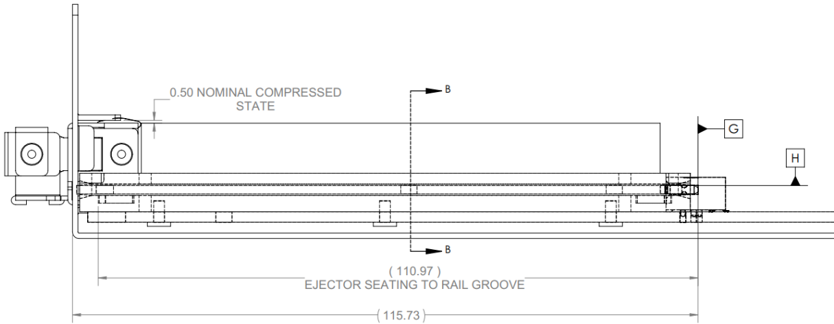
Figure 46: Small Form Factor Baseboard Chassis to Ejector lever Card CTF Dimensions (Side View)
