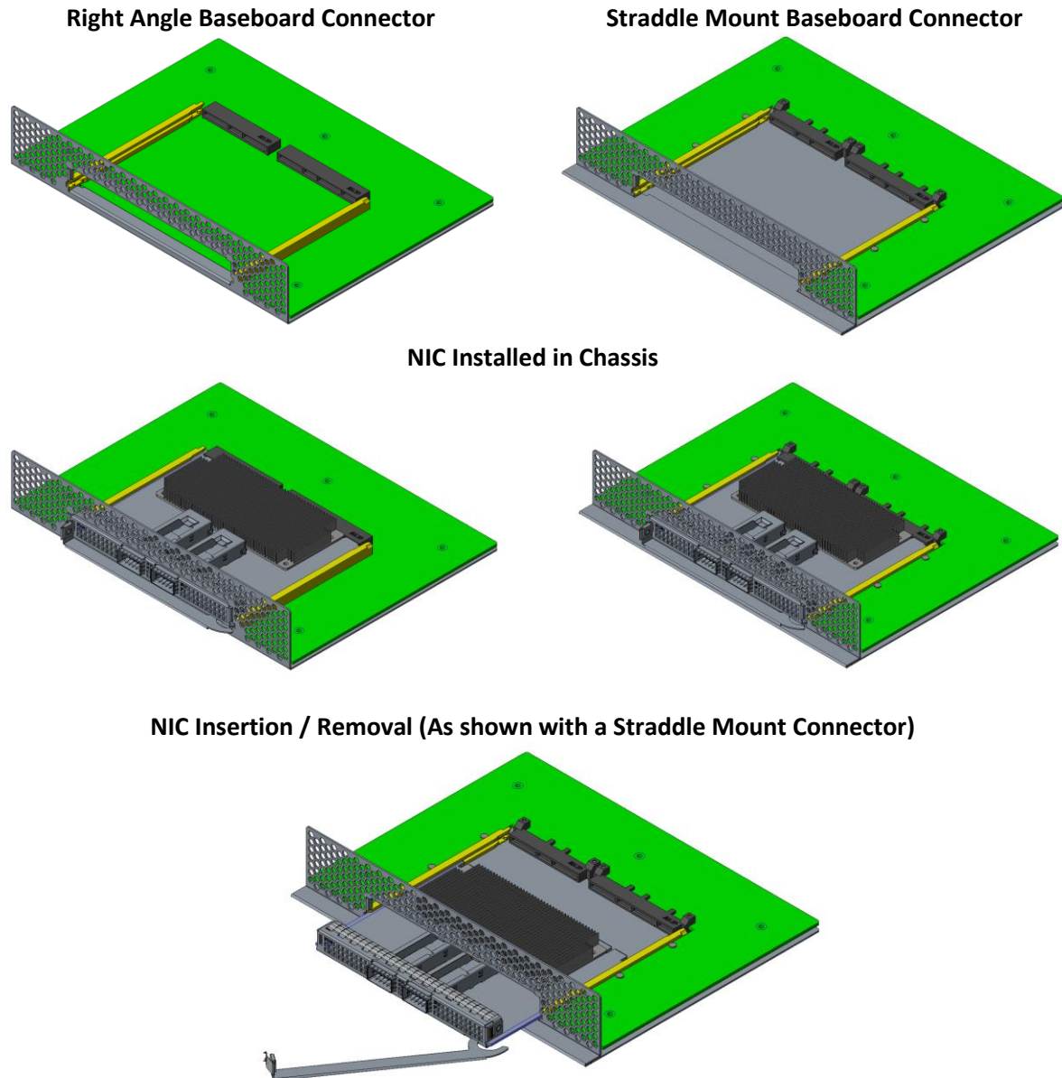
Figure 12: Large Form Factor NIC Chassis Mounted 3D Views
