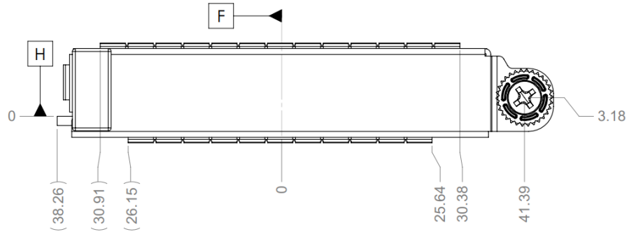
Figure 39: Small Form Factor OCP NIC 3.0 Card with Pull Tab CTF Dimensions (Front View)
