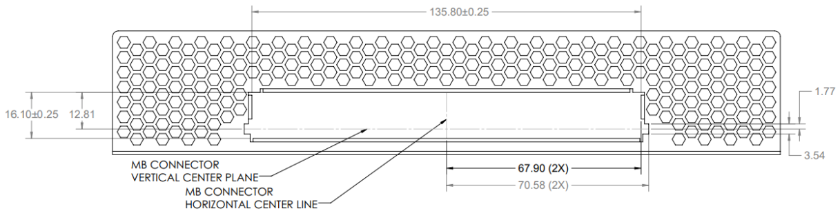
Figure 52: Large Form Factor Baseboard Chassis CTF Dimensions (Rear View)
