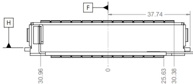
Figure 43: Small Form Factor OCP NIC 3.0 Card with Ejector CTF Dimensions (Side View)
