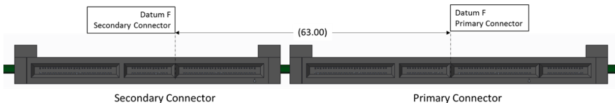
Figure 73: Primary and Secondary Connector Locations for Large Card Support with Straddle Mount Connectors
