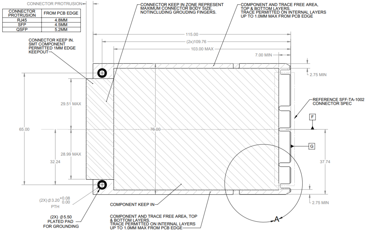
Figure 24: Small Form Factor Keep Out Zone – Top View
