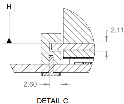
Figure 55: Large Form Factor Baseboard Chassis CTF Dimensions (Rail Guide – Detail C)
