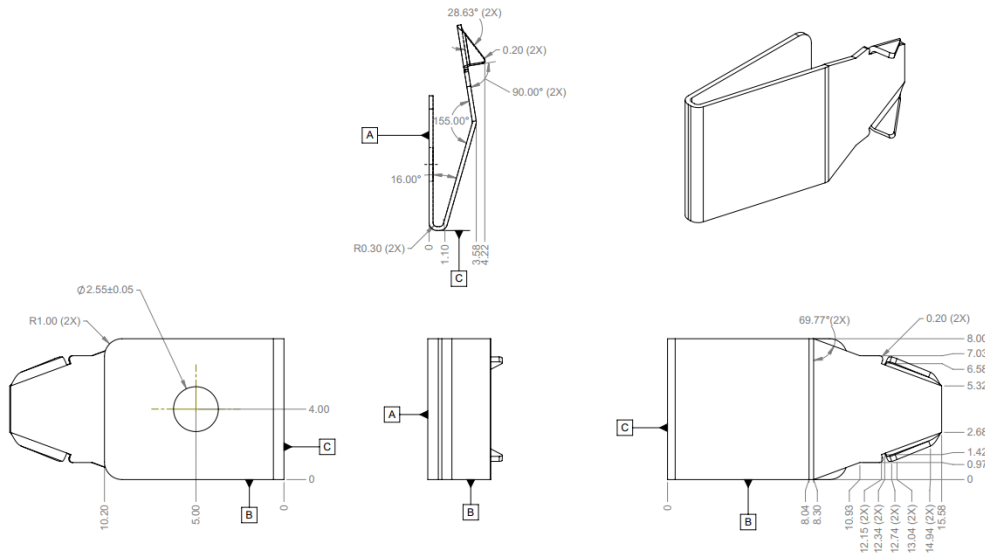
Figure 21: Ejector Lock
