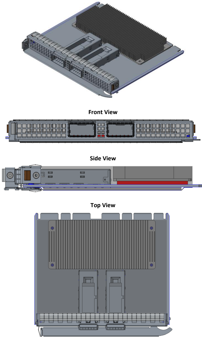
Figure 10: Large Form Factor NIC Configuration Views Large Form Factor (LFF) with Ejector Latch
