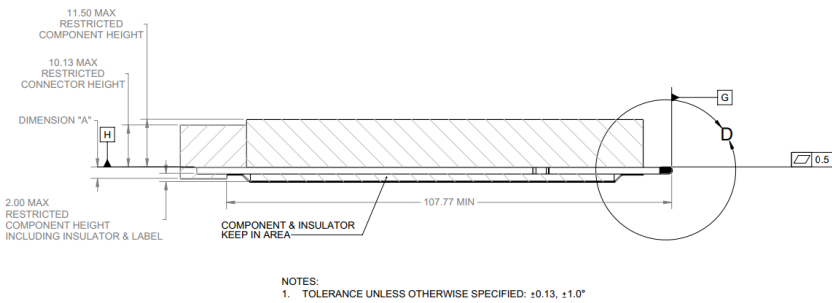
Figure 27: Small Form Factor Keep Out Zone – Side View
