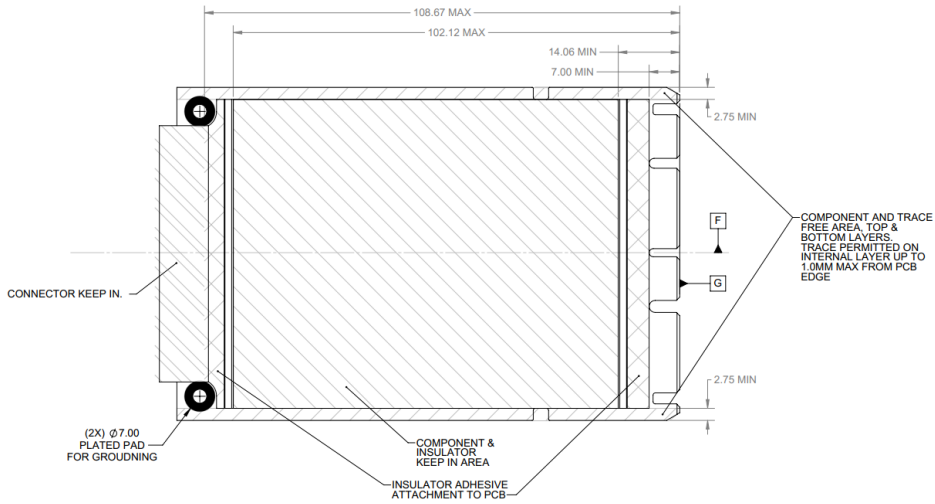
Figure 24: Small Form Factor Keep Out Zone – Bottom View
