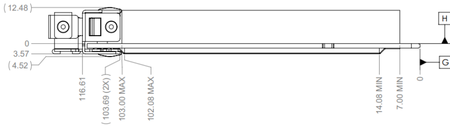
Figure 41: Small Form Factor OCP NIC 3.0 Card with Ejector CTF Dimensions (Side View)
