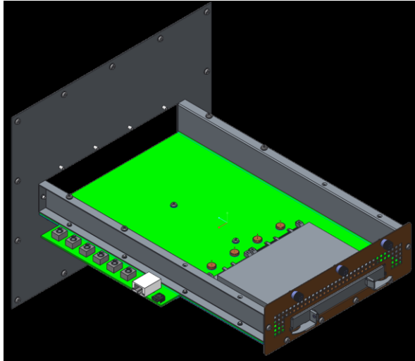
Figure 110: LFF Card Thermal Test Fixture PCB
