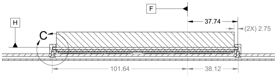
Figure 52: Large Form Factor Baseboard Chassis CTF Dimensions (Rail Guide View)
