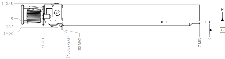
Figure 38: Small Form Factor OCP NIC 3.0 Card with Pull Tab CTF Dimensions (Side View)
