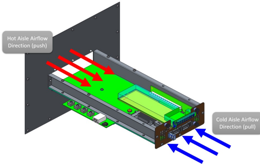
Figure 111: Thermal Test Fixture Airflow Direction
