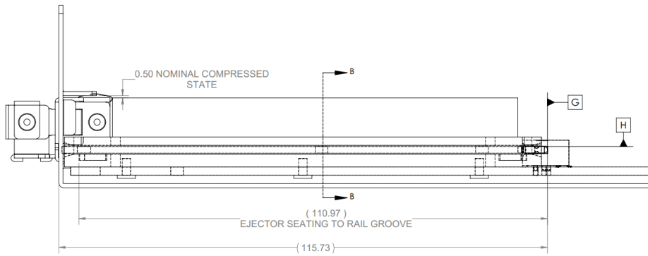
Figure 52: Large Form Factor Baseboard Chassis CTF Dimensions (Rail Guide View)
