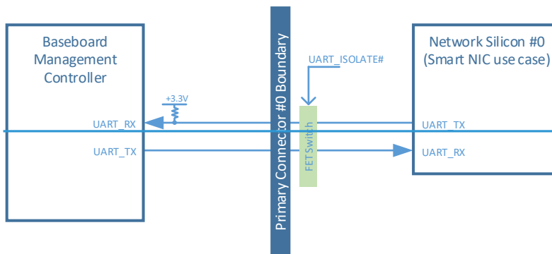
Figure 80: UART Connection Example
