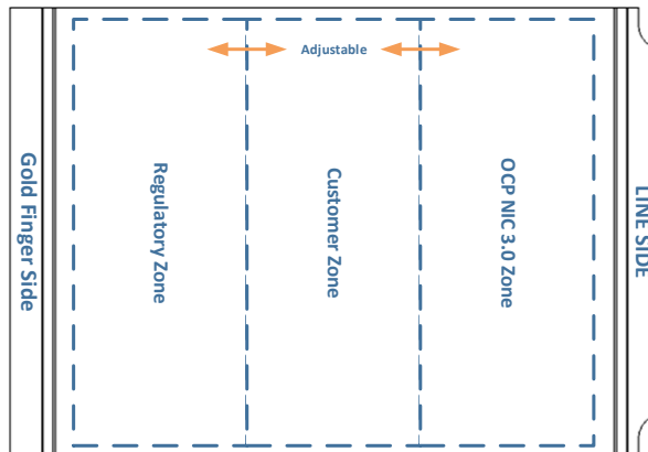
Figure 54: Small Card Label Area Example
