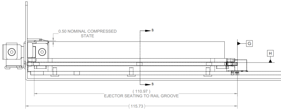
Figure 45: Small Form Factor Baseboard Chassis CTF Dimensions (Rear Rail Guide View)
