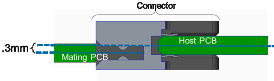
Figure 69: 0.3mm Offset for 0.076" Thick Baseboards
