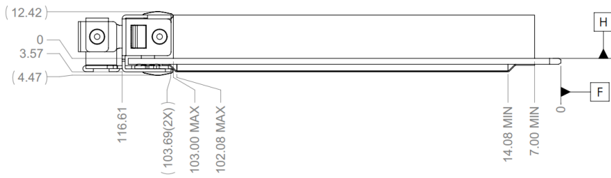
Figure 49: Large Form Factor OCP NIC 3.0 Card with Ejector CTF Dimensions (Side View)
