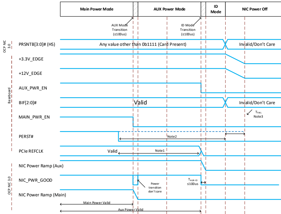
Figure 90: Power-Down Sequencing
