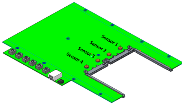
Figure 110: LFF Card Thermal Test Fixture PCB
