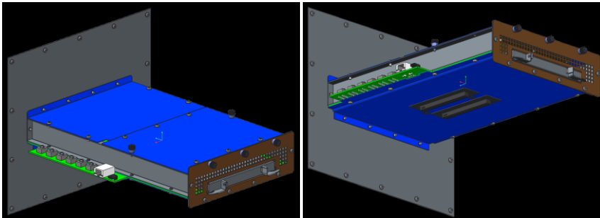
Figure 108: LFF Card Thermal Test Fixture Design
