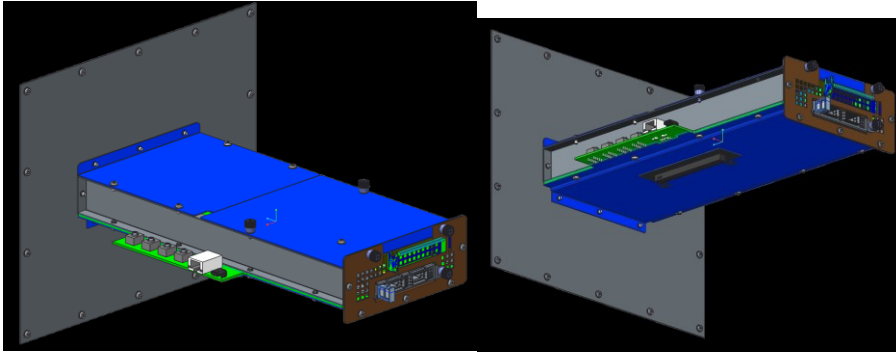
Figure 106: SFF Card Thermal Test Fixture Preliminary Design – Cover Removed
