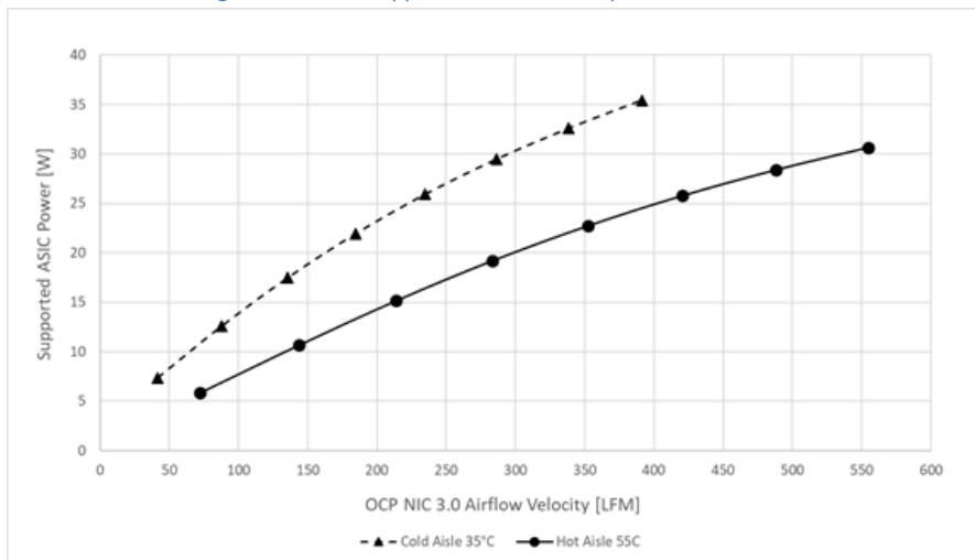
Figure 101: ASIC Supportable Power Comparison – SFF Card
