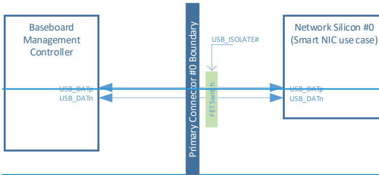
Figure 80: USB 2.0 Connection Example
