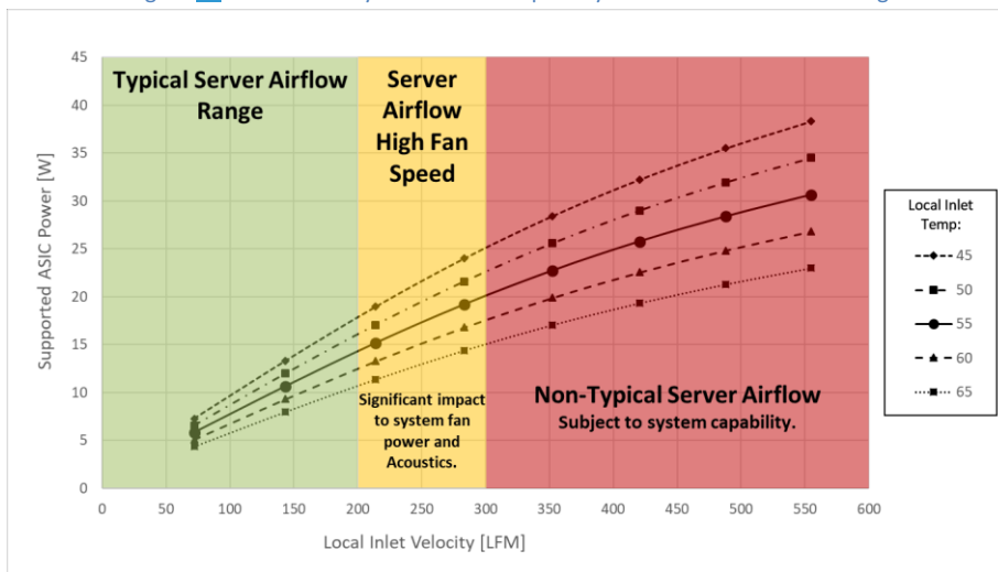
Figure 959597: Server System Airflow Capability – SFF Card Hot Aisle Cooling
