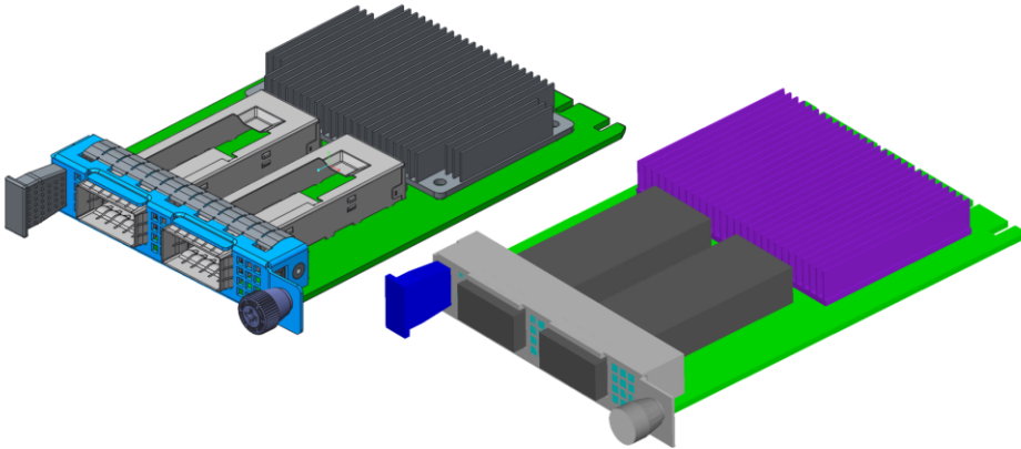
Figure 94: OCP NIC 3.0 SFF Reference Design and CFD Geometry
