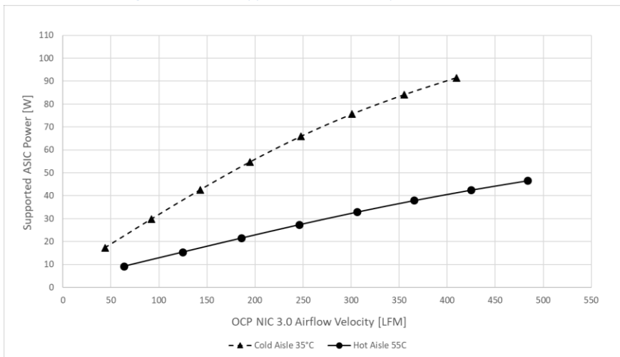
Figure 104: ASIC Supportable Power Comparison – LFF Card
