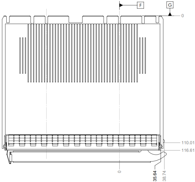
Figure 48: Large Form Factor OCP NIC 3.0 Card with Ejector CTF Dimensions (Front View)
