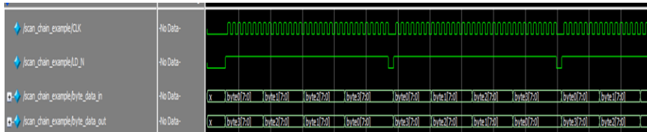
Figure 77: Example Scan Chain Timing Diagram
