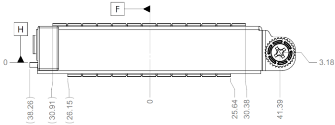
Figure 38: Small Form Factor OCP NIC 3.0 Card with Pull Tab CTF Dimensions (Side View)
