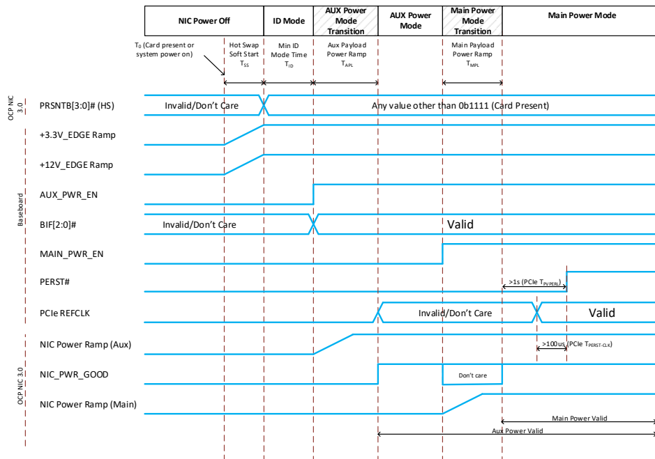
Figure 89: Power-Up Sequencing
