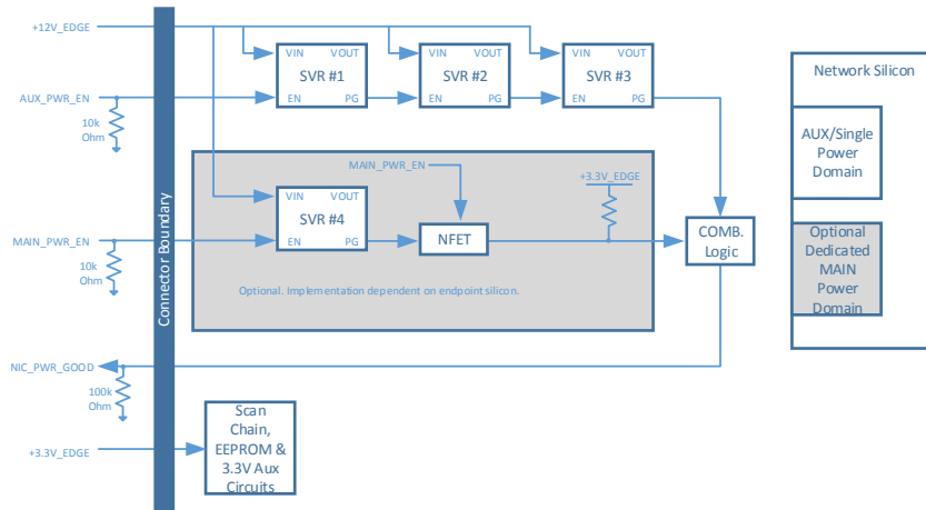
Figure 82: Example Power Supply Topology
