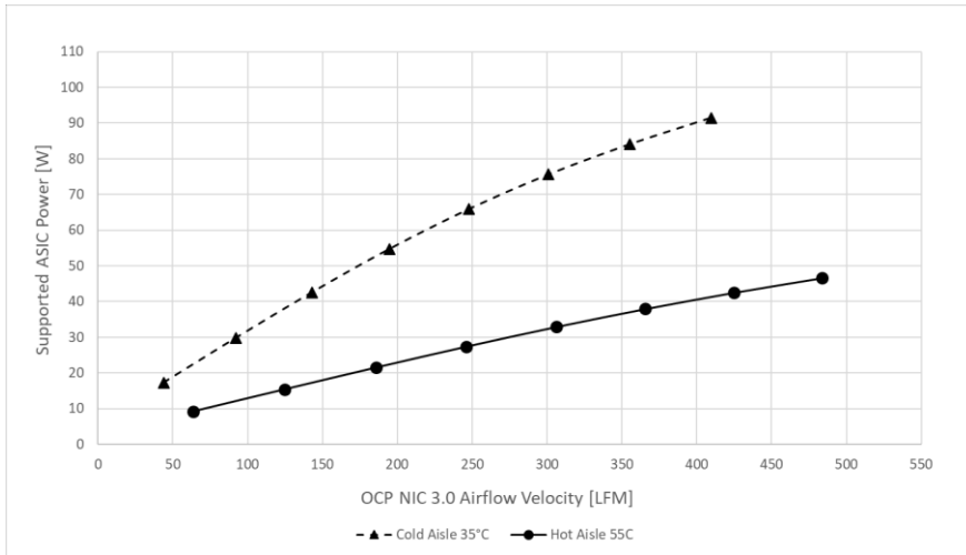
Figure 107 106 : ASIC Supportable Power Comparison – LFF Card
