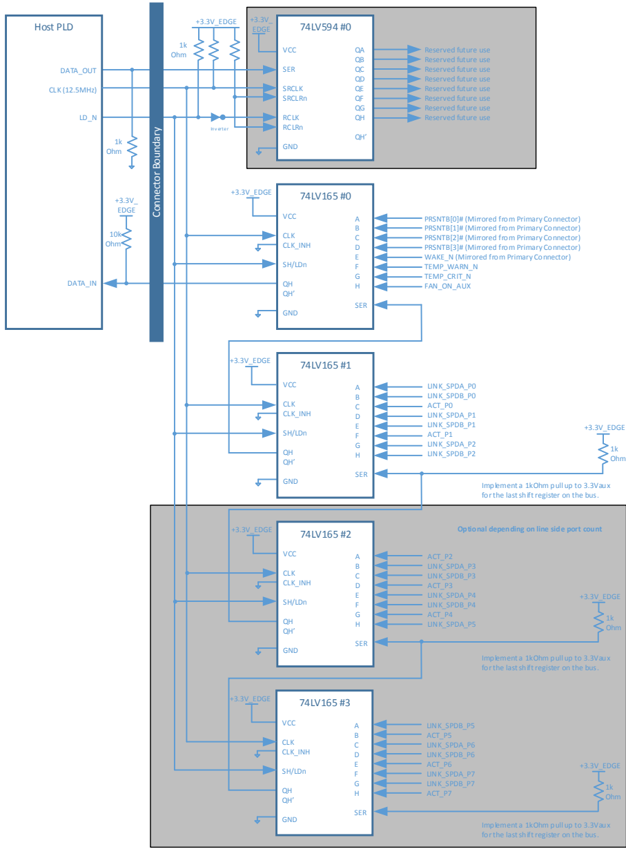
Figure 79: Scan Chain Connection Example
