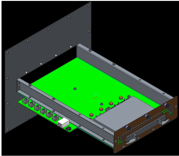
Figure 113442: LFF Card Thermal Test Fixture PCB
