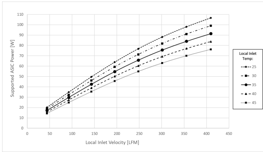
Figure 105 104 : ASIC Supportable Power for Cold Aisle Cooling – LFF Card
