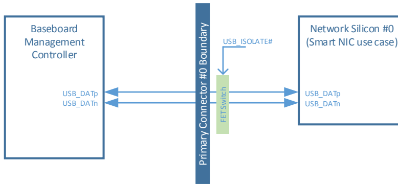
Figure 8079: USB 2.0 Connection Example
