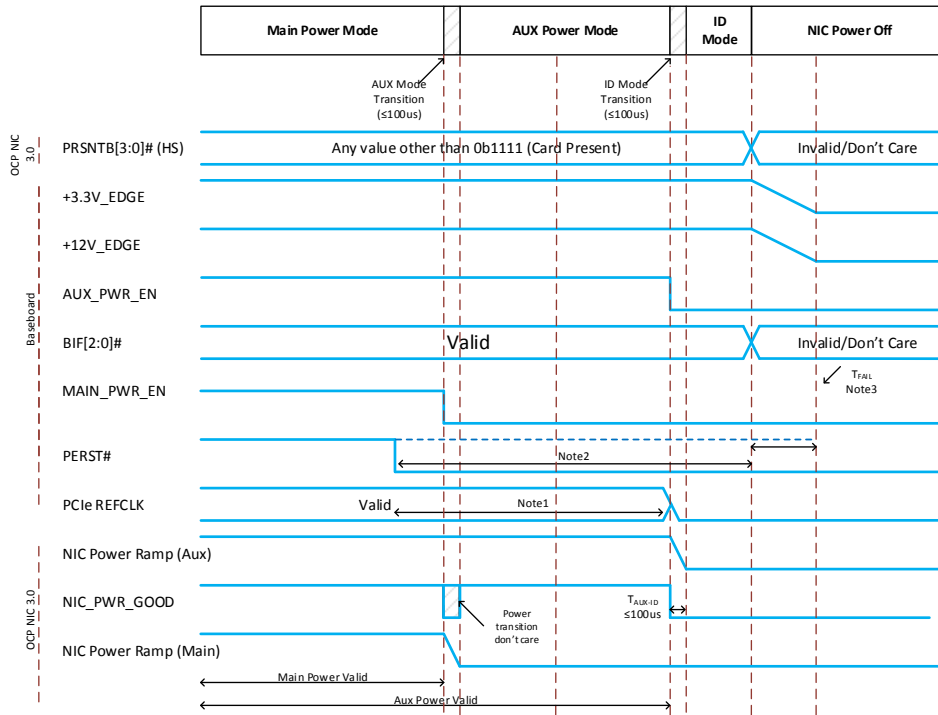
Figure 93: Power-Down Sequencing
