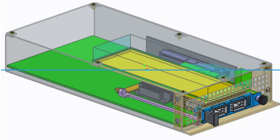
Figure 109108102 : Small-SFF Card Thermal Test Fixture Preliminary Design – Transparent View Cover
