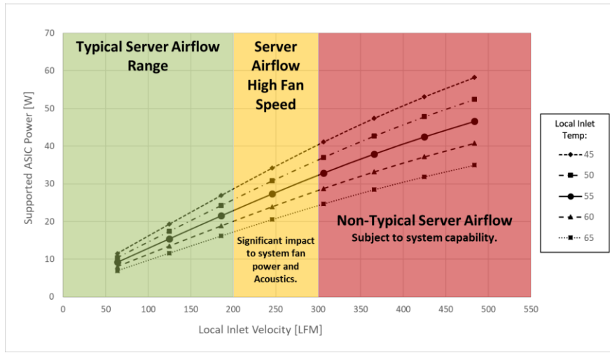
Figure 101490: Server System Airflow Capability – LFF Card Hot Aisle Cooling
