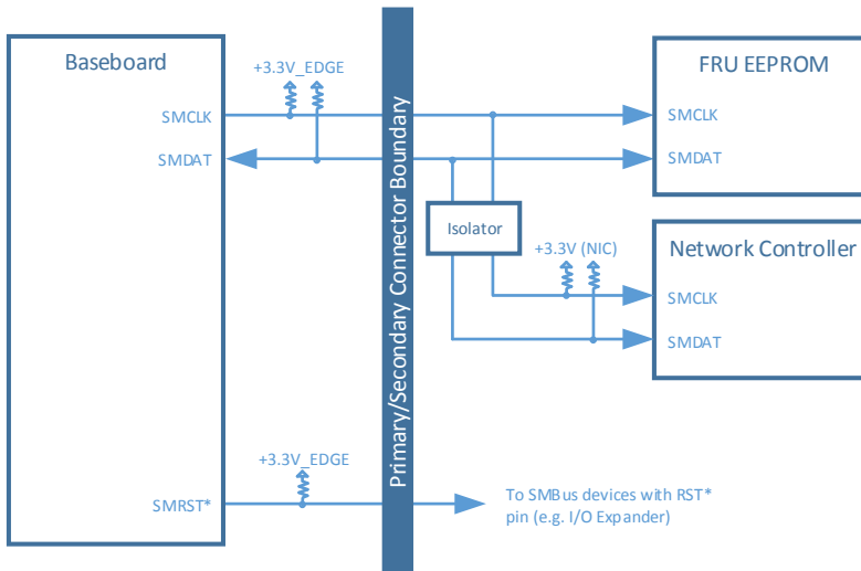
Figure 75: Example SMBus Connections
