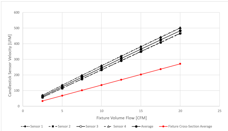
Figure 116415: LFF Fixture, Hot Aisle Flow - Candlestick Air Velocity vs. Volume Flow
