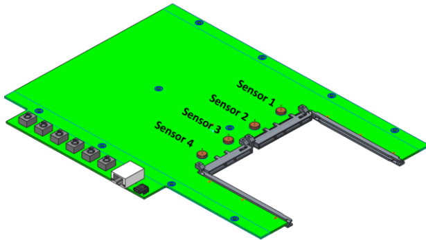
Figure 113442: LFF Card Thermal Test Fixture PCB
