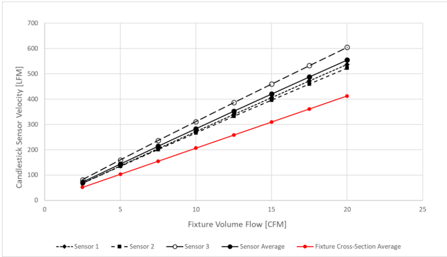
Figure 115414: SFF Fixture, Hot Aisle Flow - Candlestick Air Velocity vs. Volume Flow
