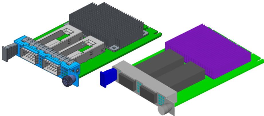
Figure 97: OCP NIC 3.0 SFF Reference Design and CFD Geometry-CAD & CFD
