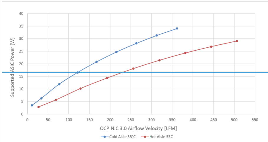
Figure 104 103 100 : ASIC Supportable Power Comparison – Small-SFF Card-Form Factor
