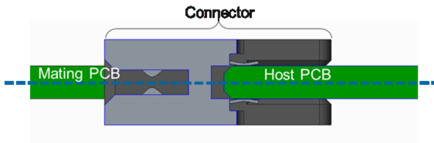
Figure 69: 0mm Offset (Coplanar) for 0.062" Thick Baseboards
