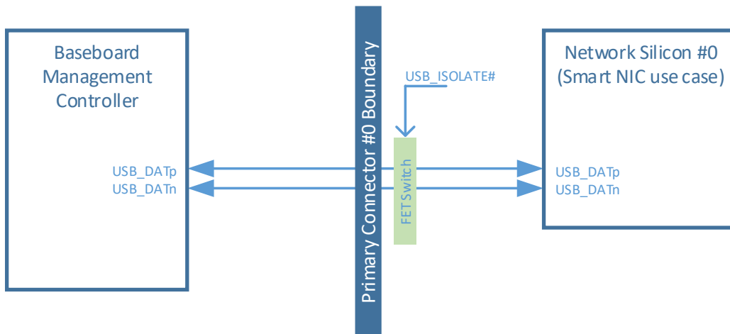
Figure 79: USB 2.0 Connection Example
