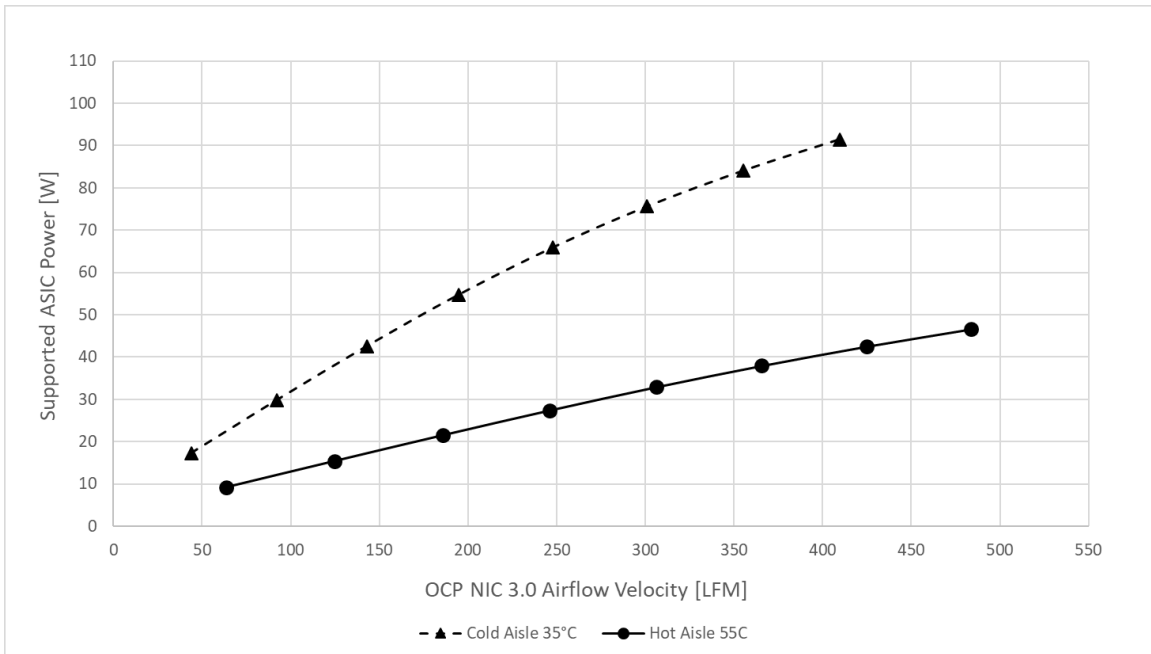
Figure 106: ASIC Supportable Power Comparison – LFF Card
