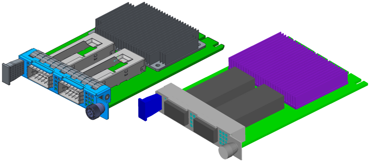
Figure 96: OCP NIC 3.0 SFF Reference Design and CFD Geometry
