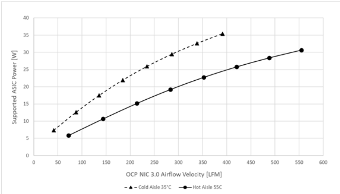
Figure 103: ASIC Supportable Power Comparison – SFF Card
