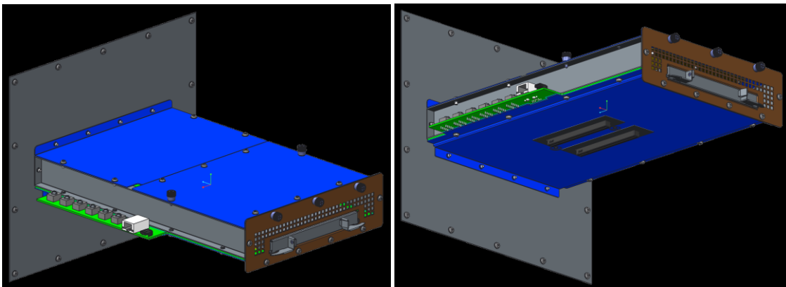
Figure 110: LFF Card Thermal Test Fixture Design
