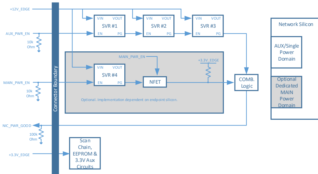
Figure 81: Example Power Supply Topology
