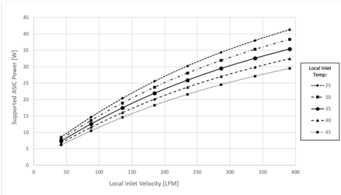
Figure 101: ASIC Supportable Power for Cold Aisle Cooling – SFF Card
