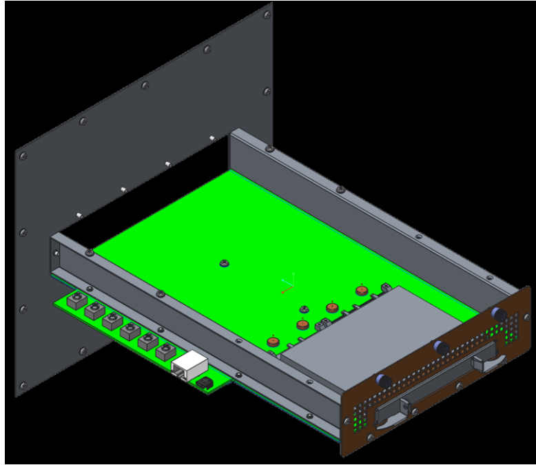
Figure 111: LFF Card Thermal Test Fixture Design – Cover Removed
