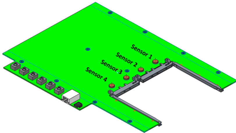
Figure 112: LFF Card Thermal Test Fixture PCB
