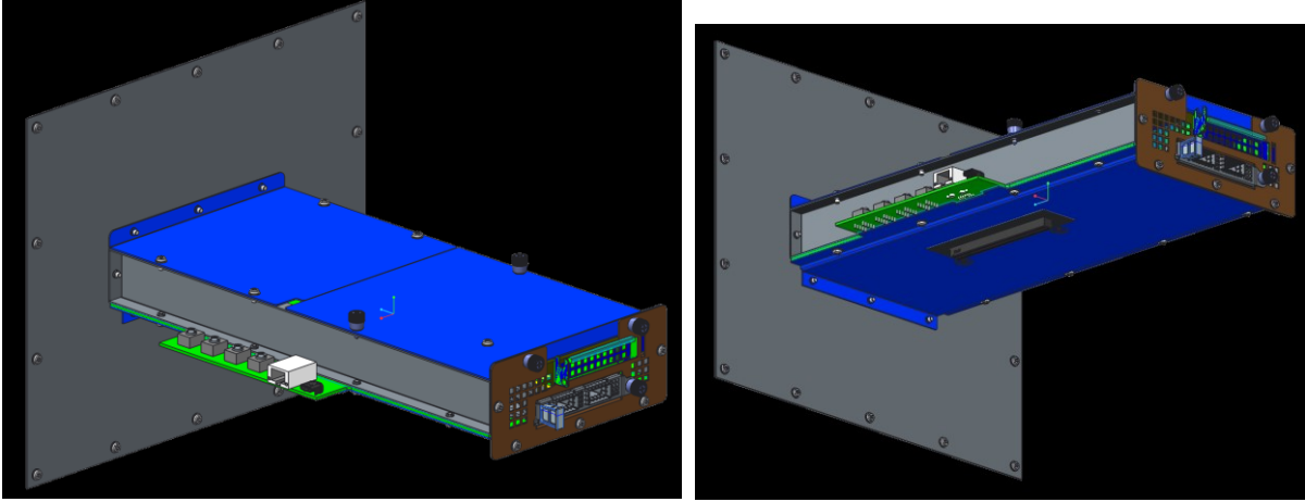
Figure 107: Small Card Thermal Test Fixture Preliminary Design
