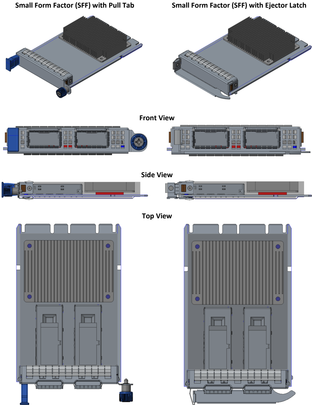
Figure 7: Small Form Factor NIC Configuration Views
