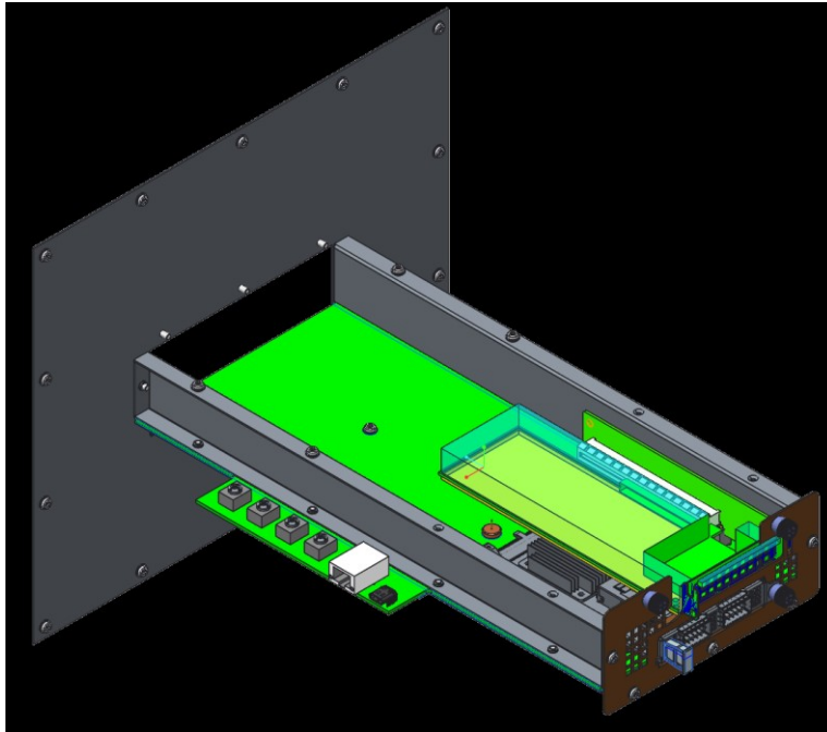
Figure 108: SFF Card Thermal Test Fixture Preliminary Design – Cover Removed
