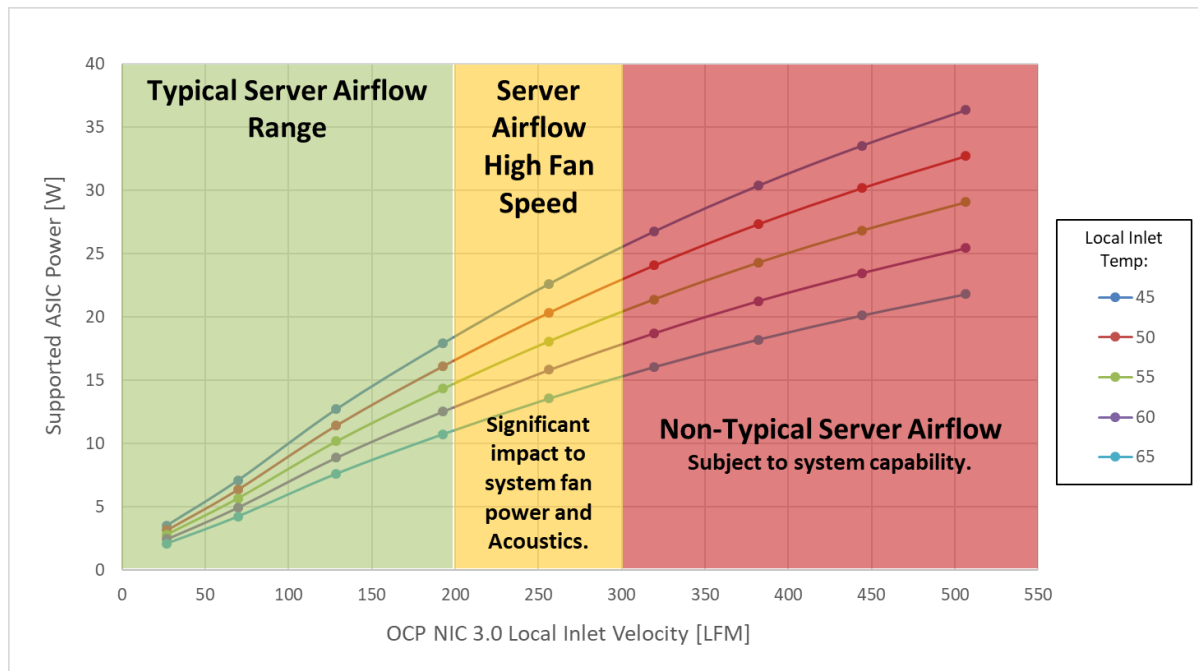
Figure 97: Server System Airflow Capability – Hot Aisle Cooling
