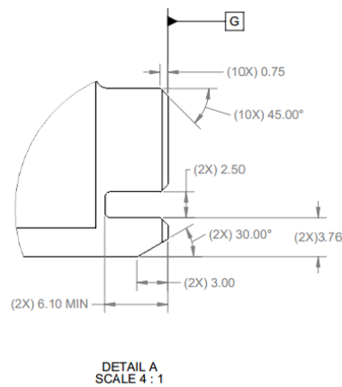
Figure 41: Small Form Factor Keep Out Zone – Top View – Detail A
