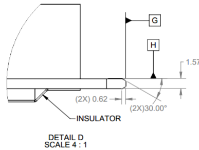
Figure 44: Small Form Factor Keep Out Zone – Side View – Detail D
