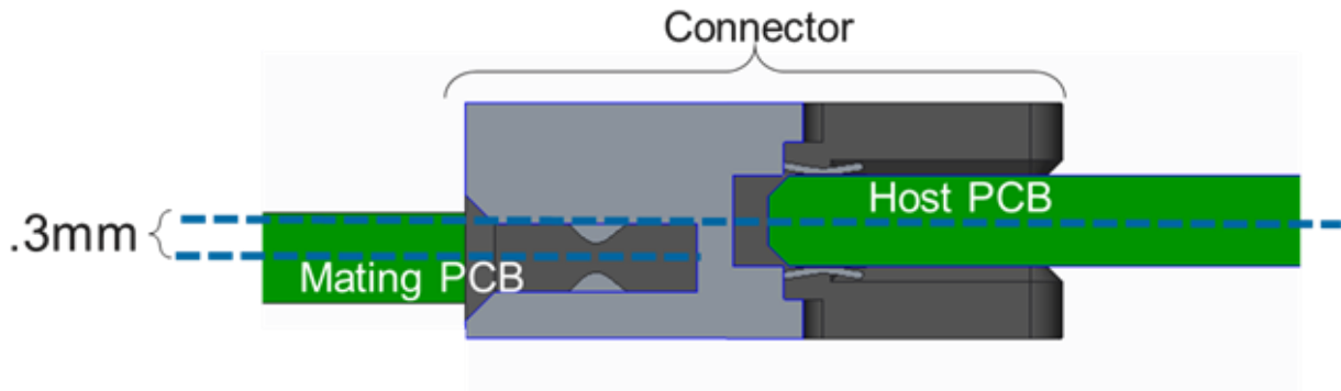
Figure 72: 0.3mm Offset for 0.076" Thick Baseboards
