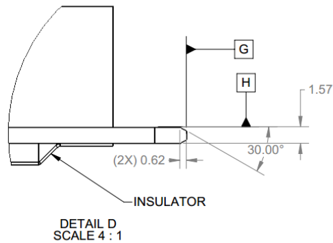
Figure 49: Large Form Factor Keep Out Zone – Side View – Detail D
