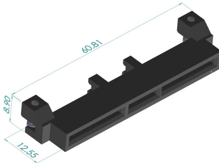
Figure 69: 140-pin Base Board Secondary Connector – Straddle Mount
