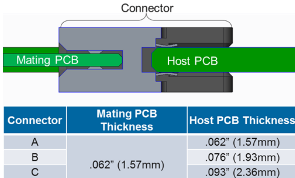
Figure 70: OCP NIC 3.0 Card and Baseboard PCB Thickness Options for Straddle Mount Connectors
