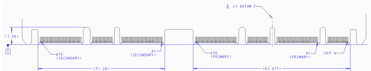
Figure 64: Large Size Card Gold Finger Dimensions – x32 – Bottom Side (“A” Pins)
