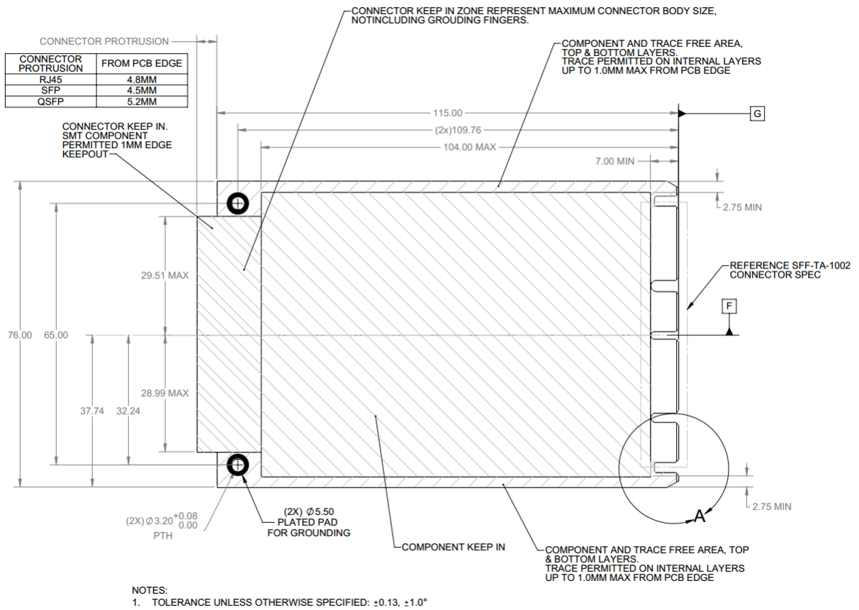
Figure 41: Small Form Factor Keep Out Zone – Top View – Detail A
