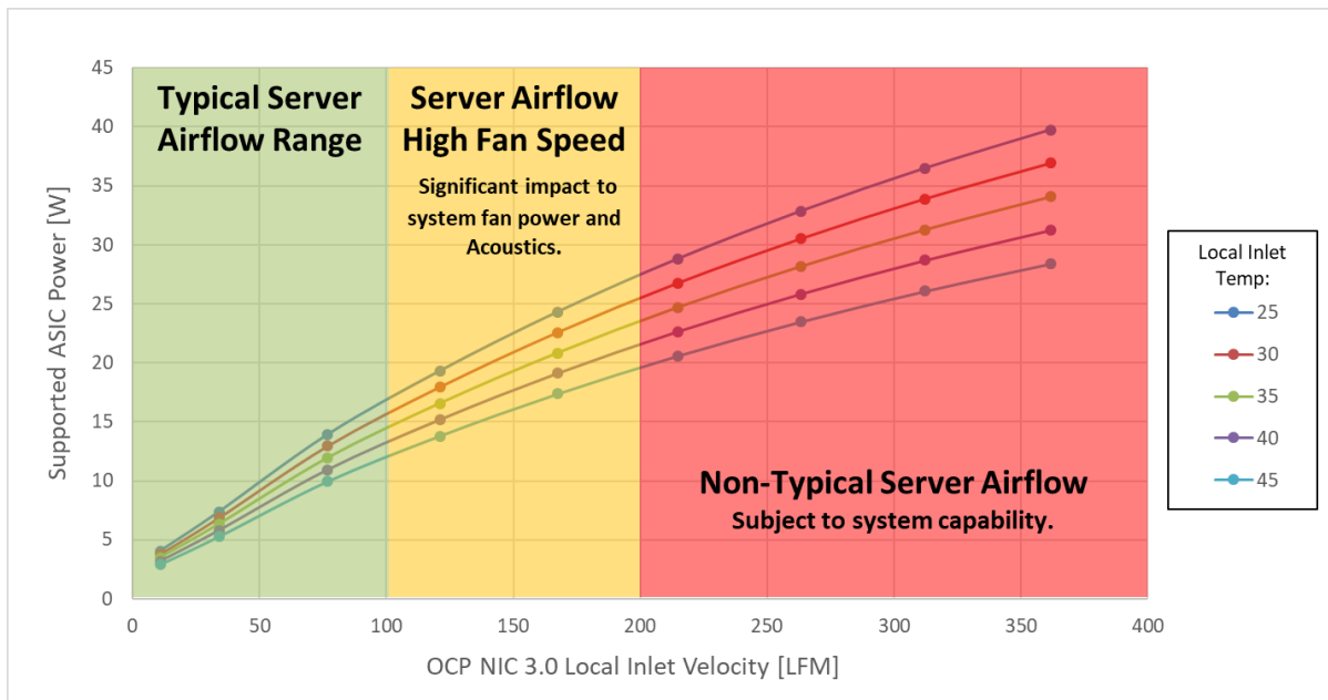
Figure 100: Server System Airflow Capability – Cold Aisle Cooling
