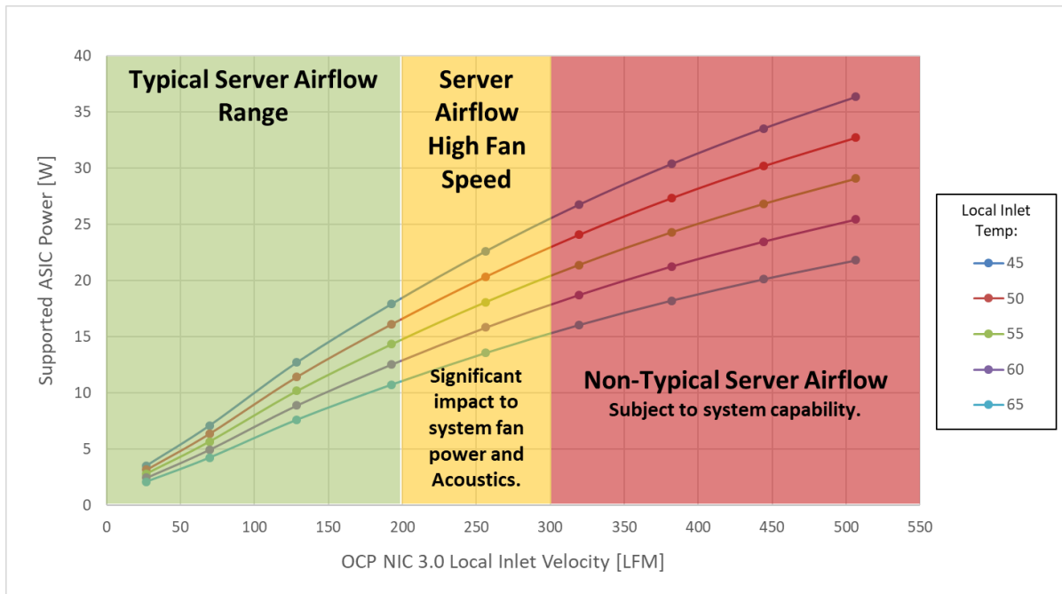
Figure 98: Server System Airflow Capability – Hot Aisle Cooling
