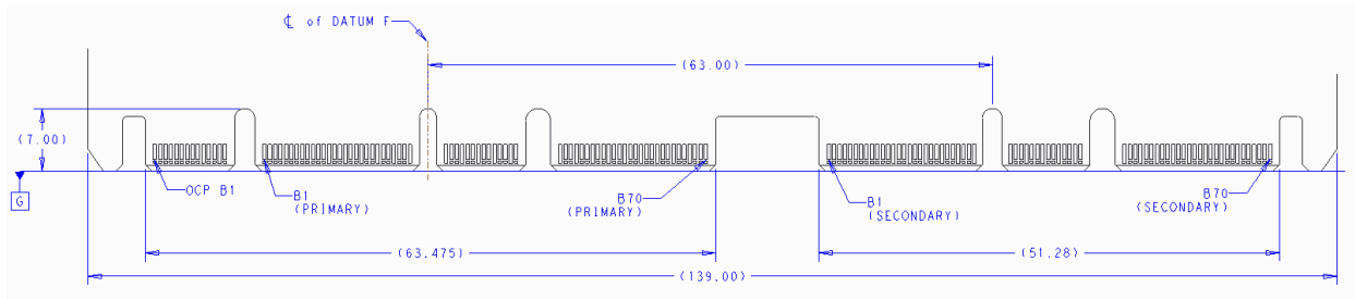
Figure 63: Large Size Card Gold Finger Dimensions – x32 – Top Side (“B” Pins)
