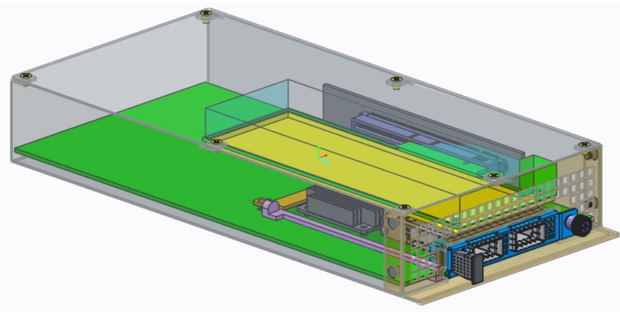
Figure 103: Small Card Thermal Test Fixture Preliminary Design – Transparent View
