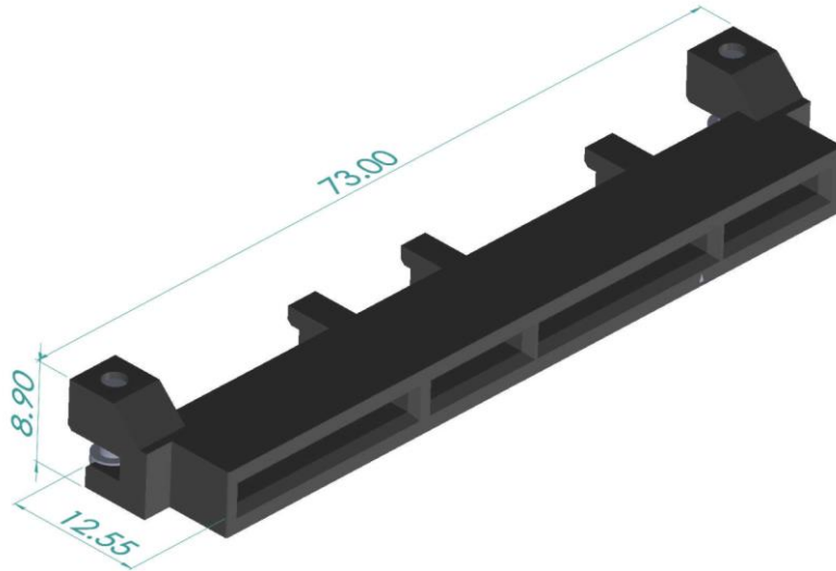
Figure 68: 168-pin Base Board Primary Connector – Straddle Mount
