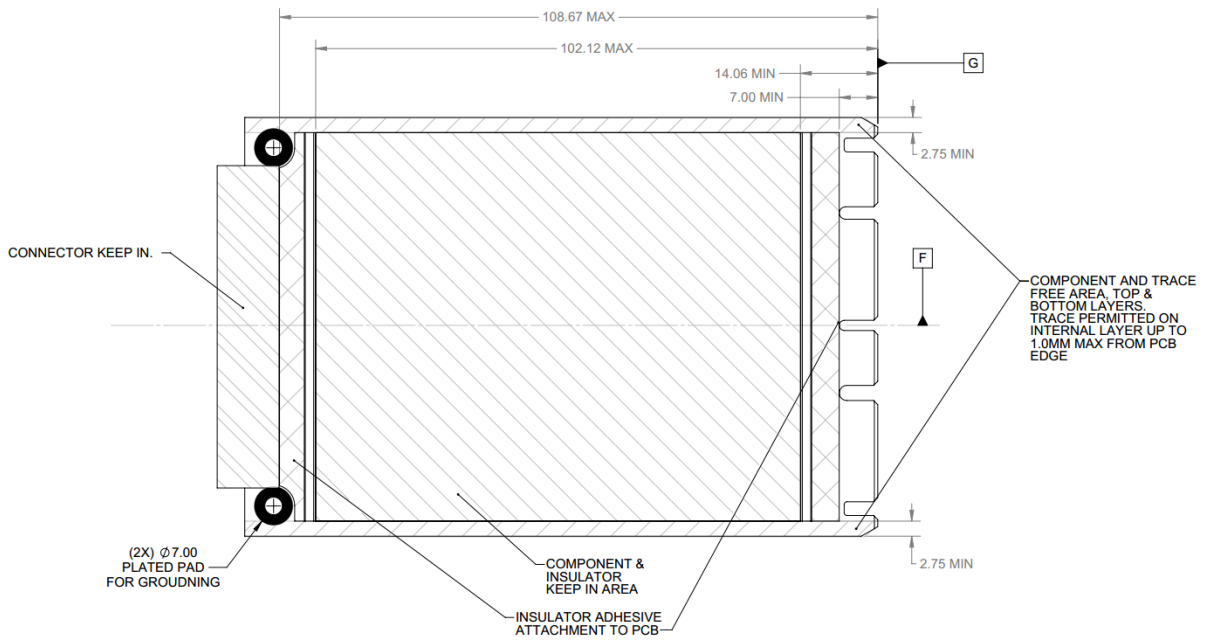
Figure 42: Small Form Factor Keep Out Zone – Bottom View
