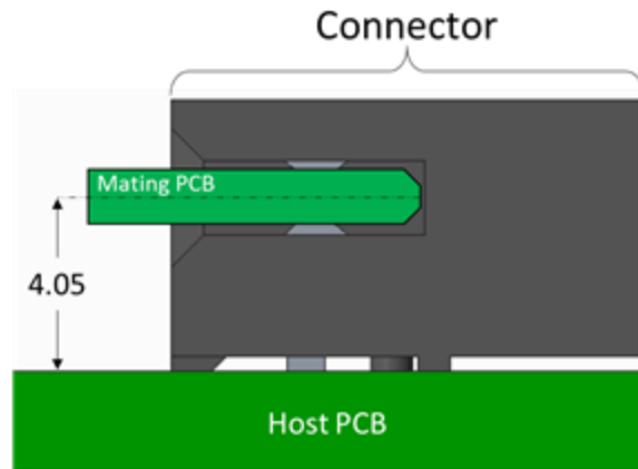
Figure 67: OCP NIC 3.0 Card and Host Offset for Right Angle Connectors
