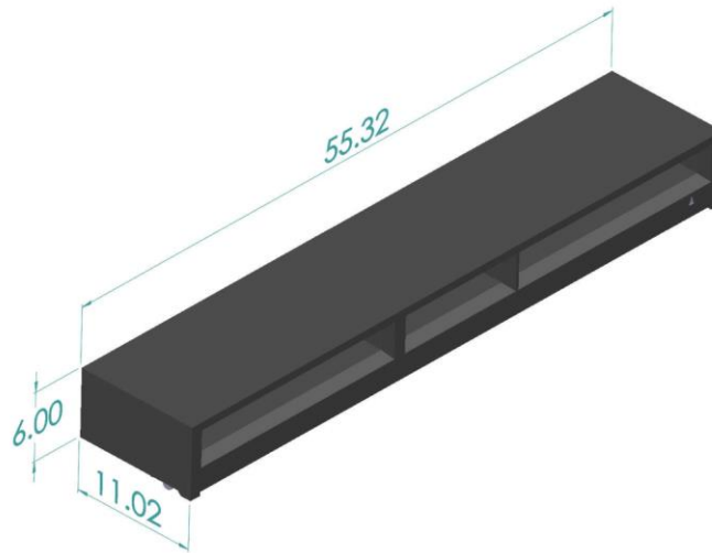
Figure 66: 140-pin Base Board Secondary Connector – Right Angle
