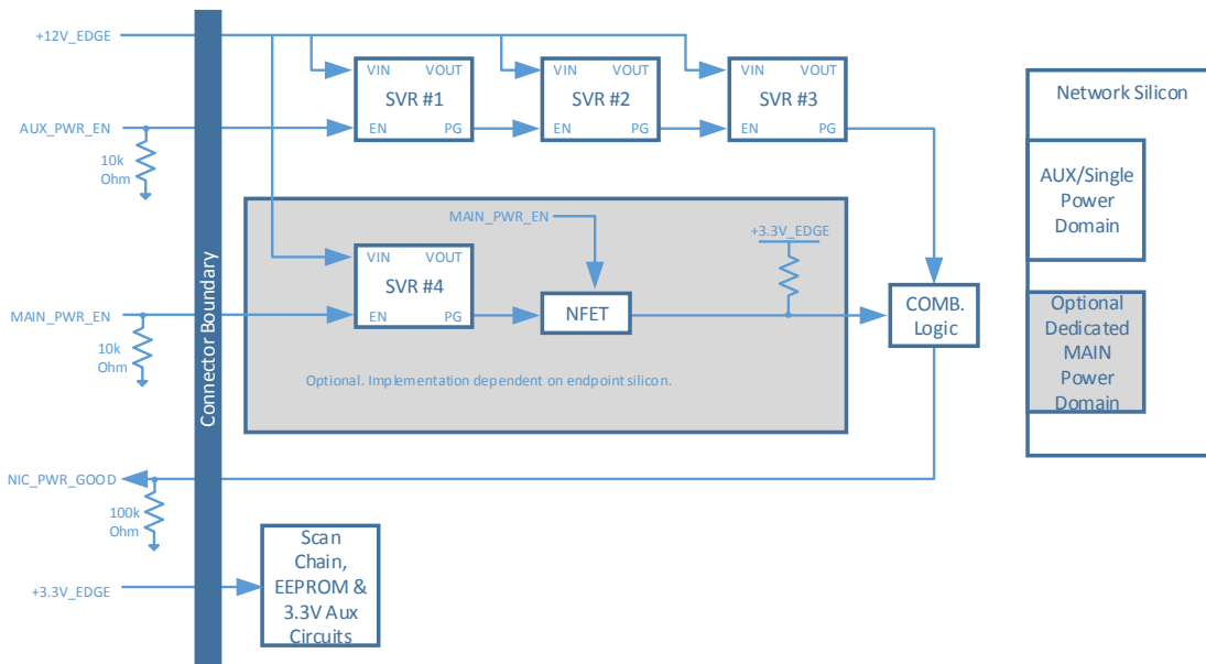
Figure 82: Example Power Supply Topology
