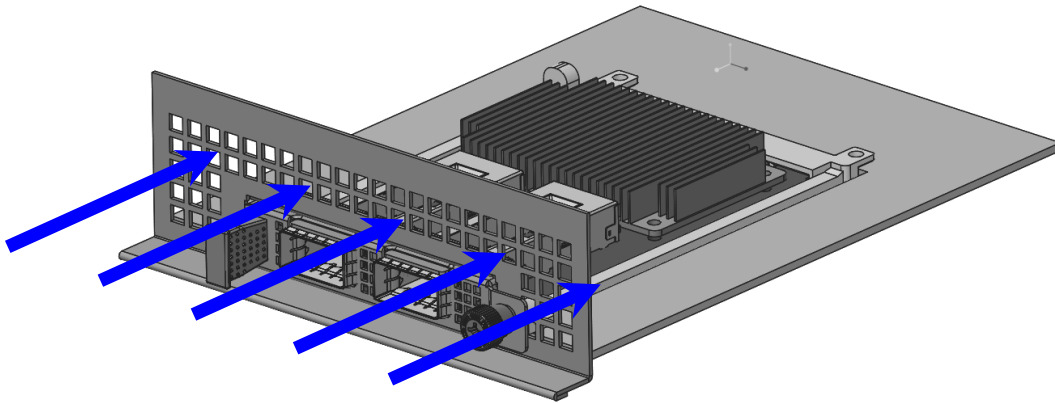
Figure 95: Airflow Direction for Cold Aisle Cooling
