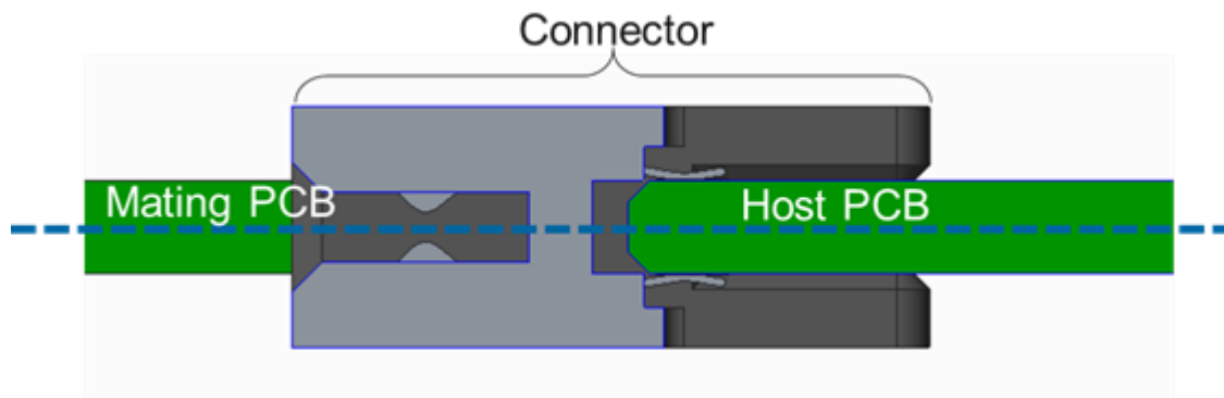
Figure 71: 0mm Offset (Coplanar) for 0.062" Thick Baseboards
