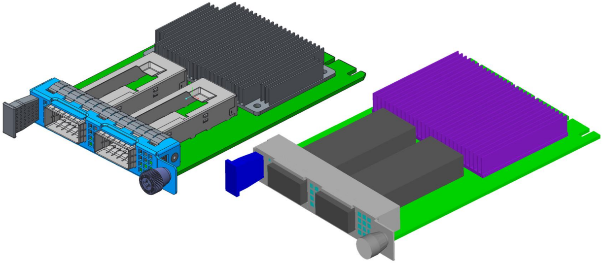
Figure 97: OCP NIC 3.0 Reference Geometry CAD &amp; CFD
