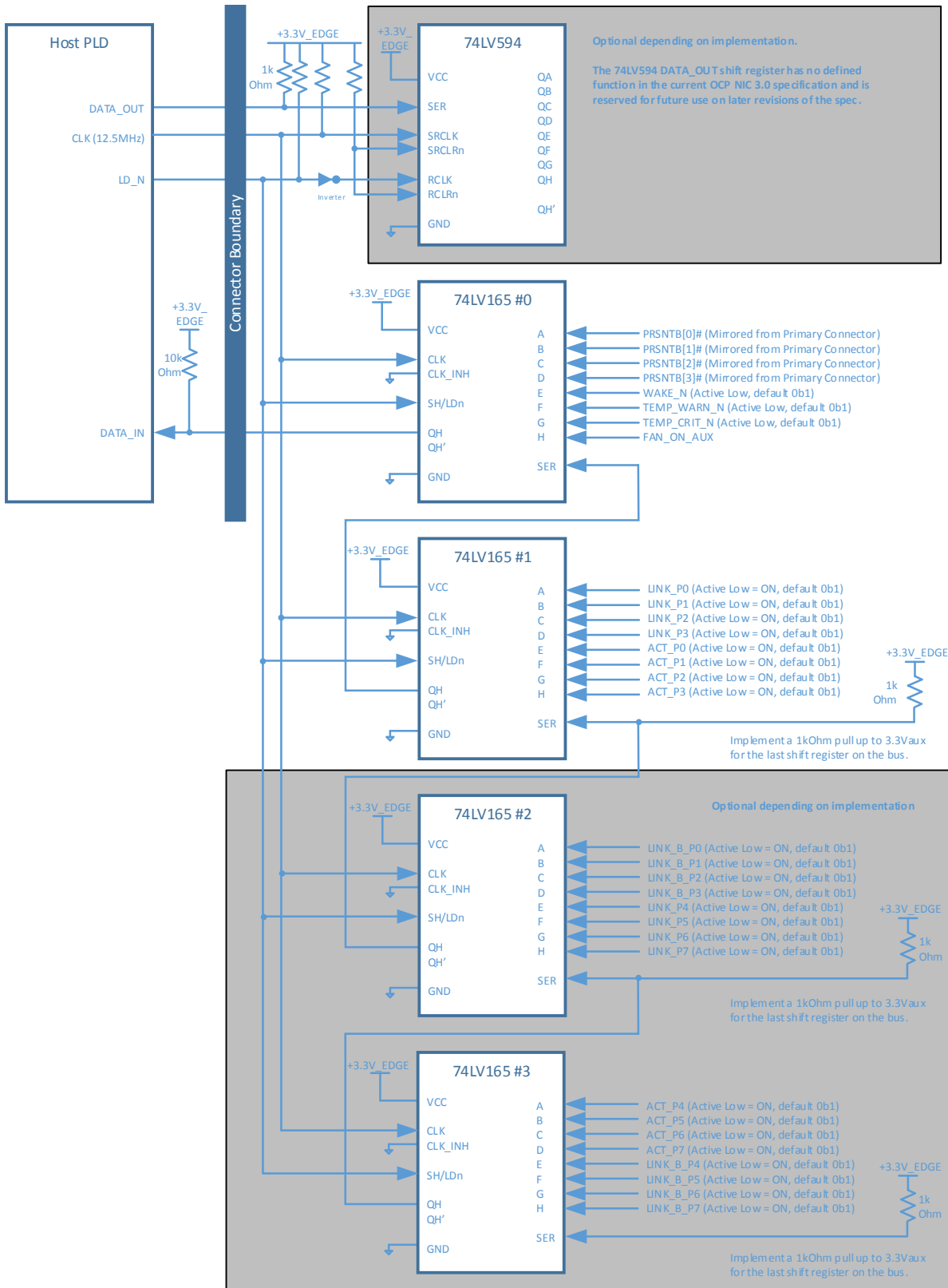
Figure 81: Scan Bus Connection Example
