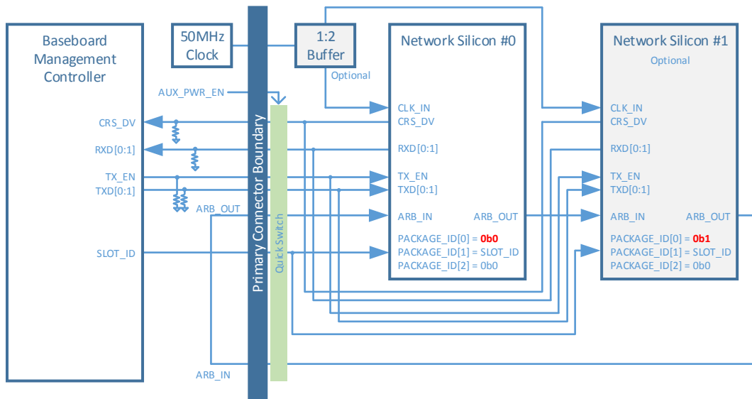
Figure 78: NC-SI Over RBT Connection Example – Single Primary Connector
