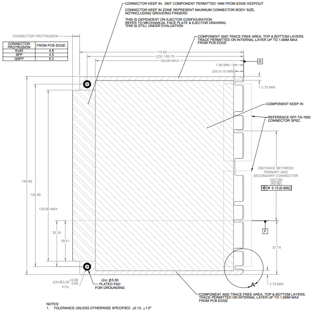
Figure 45: Large Form Factor Keep Out Zone – Top View
