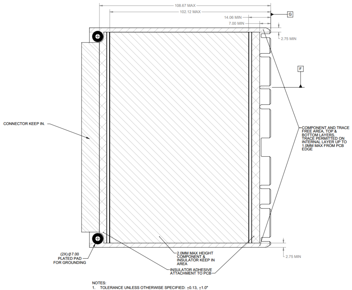
Figure 47: Large Form Factor Keep Out Zone – Bottom View
