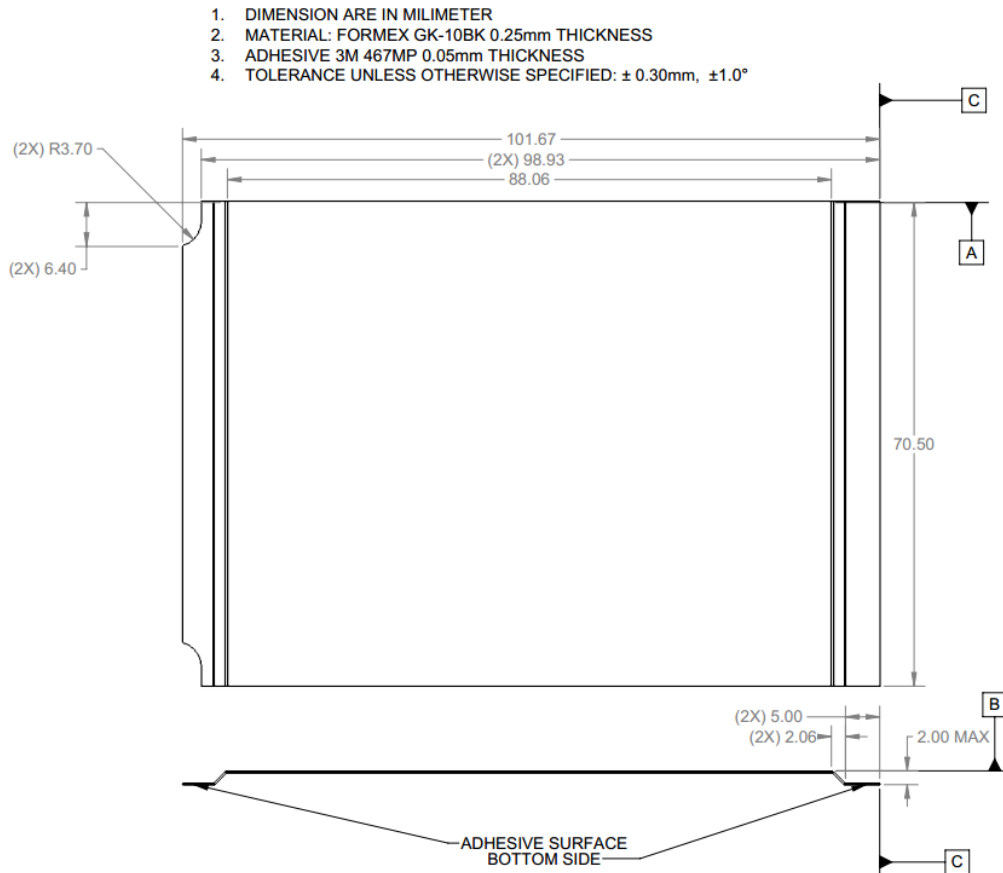
Figure 51: Small Card Bottom Side Insulator (Top and Side View)
