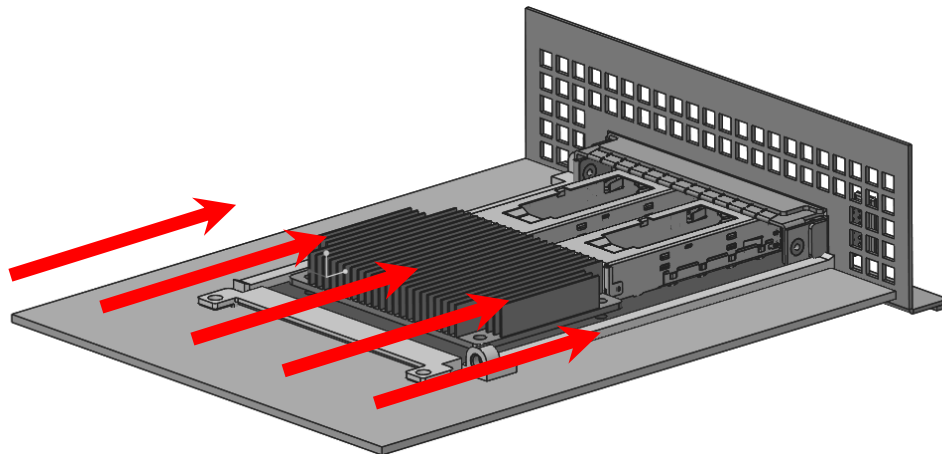
Figure 94: Airflow Direction for Hot Aisle Cooling
