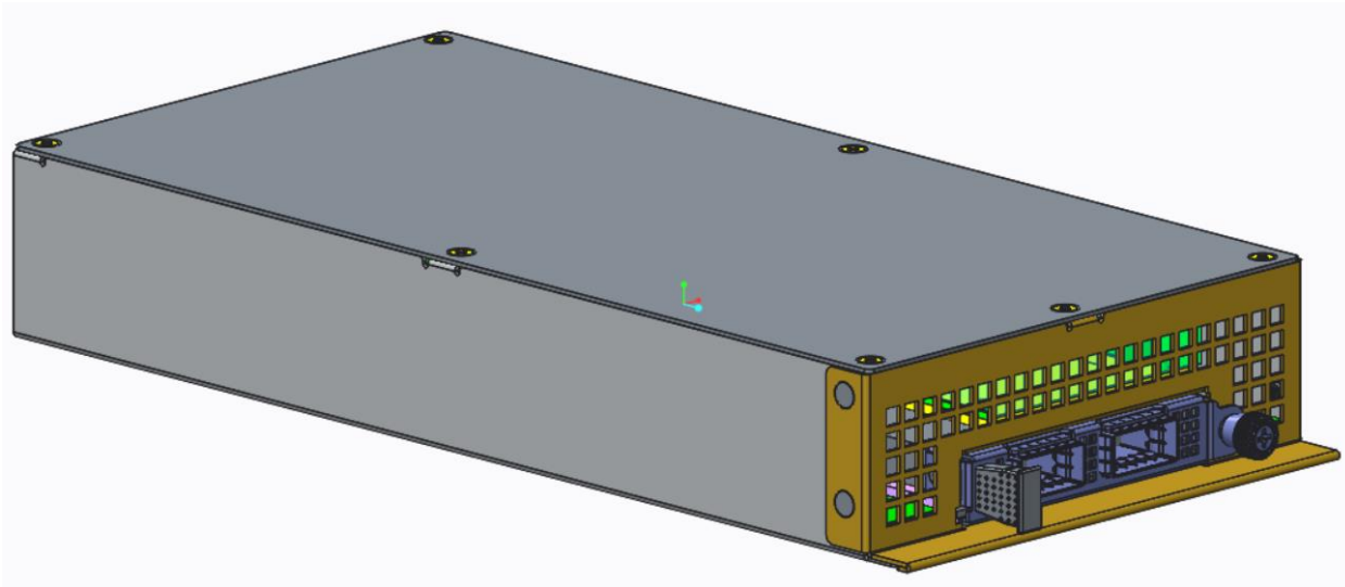
Figure 102: Small Card Thermal Test Fixture Preliminary Design
