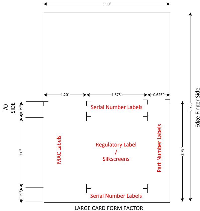
Figure 55: Large Card Label Placement Example
