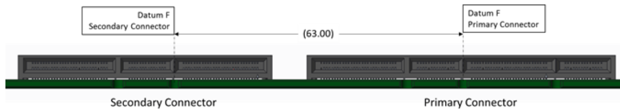
Figure 73: Primary and Secondary Connector Locations for Large Card Support with Right Angle Connectors
