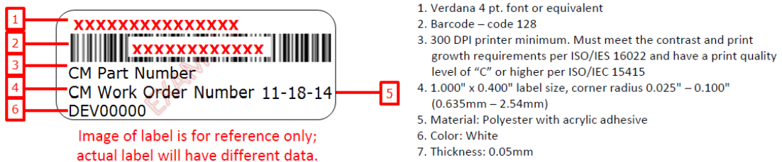
Figure 56: NIC Vendor Factory Label Example
