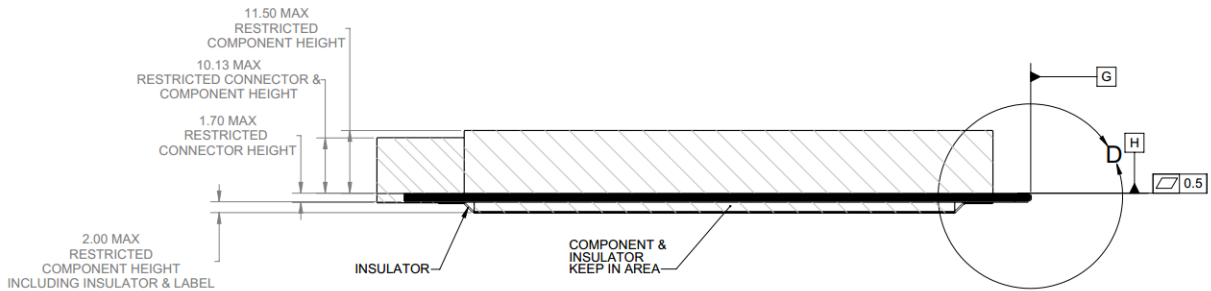
Figure 48: Large Form Factor Keep Out Zone – Side View
