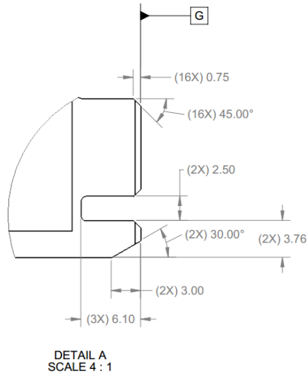
Figure 46: Large Form Factor Keep Out Zone – Top View – Detail A
