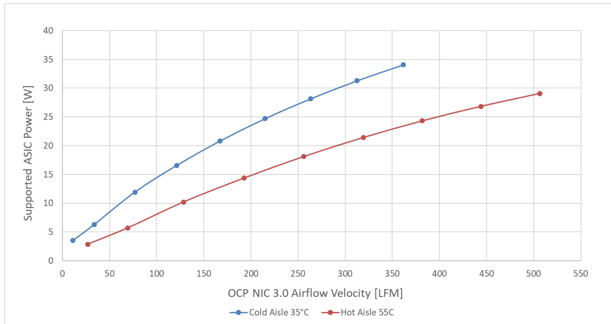
Figure 101: ASIC Supportable Power Comparison – Small Card Form Factor
