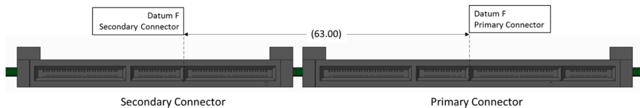
Figure 74: Primary and Secondary Connector Locations for Large Card Support with Straddle Mount Connectors
