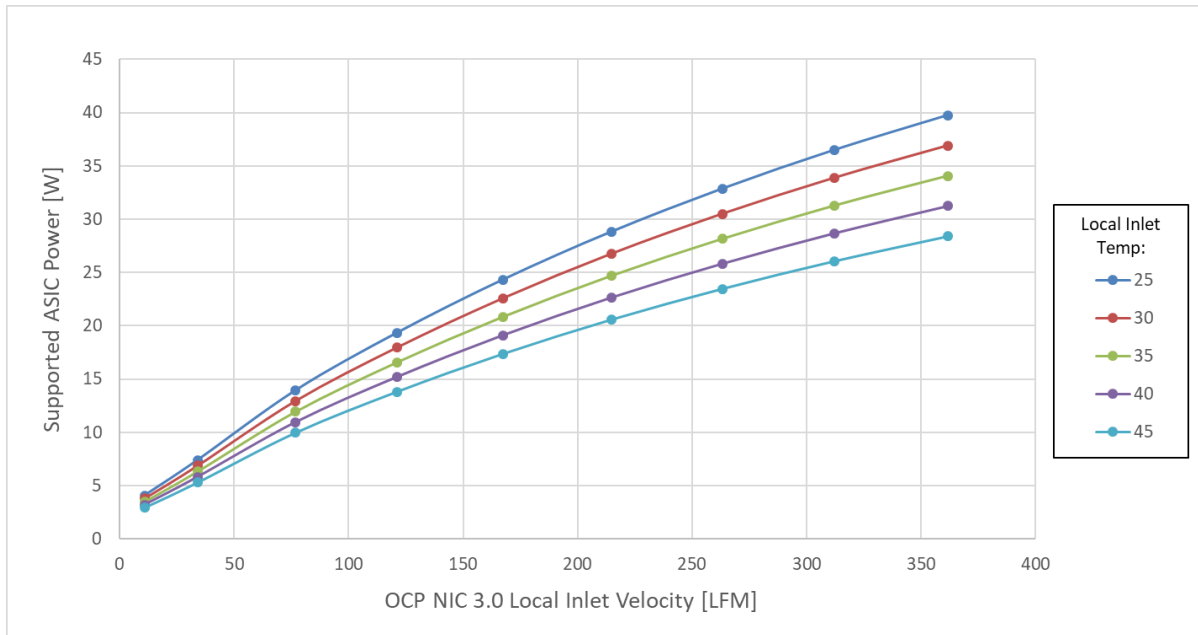
Figure 99: ASIC Supportable Power for Cold Aisle Cooling – Small Card Form Factor
