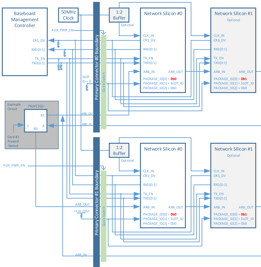
Figure 79: NC-SI Over RBT Connection Example – Dual Primary Connector
