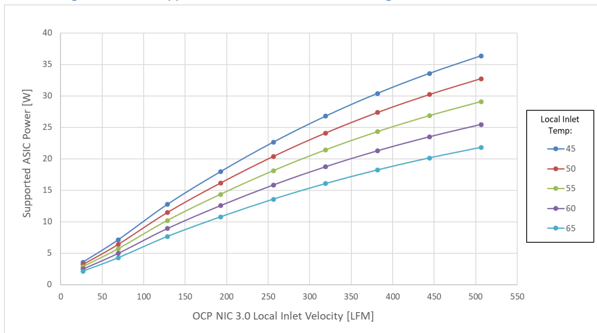
Figure 96: ASIC Supportable Power for Hot Aisle Cooling – Small Card Form Factor
