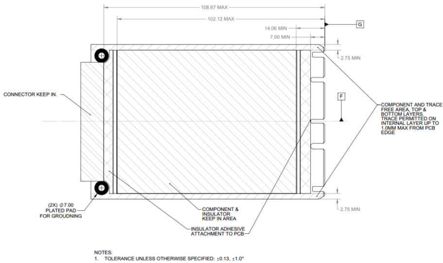
Figure 43: Small Form Factor Keep Out Zone – Bottom View
