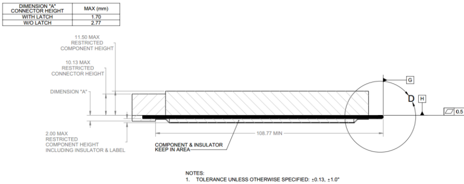
Figure 44: Small Form Factor Keep Out Zone – Side View
